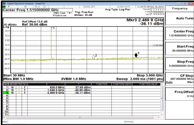
30MHz-3GHz_Band26_Part90s_1_4MHz_QPSK_1_0_HighCH26783-823.3
