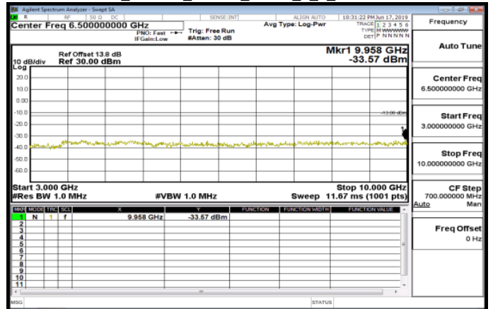
3GHz-10GHz_Band26_15MHz_QPSK_1_0_MidCH26915-836.5
