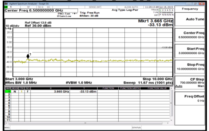
3GHz-10GHz_Band26_Part90s_3MHz_QPSK_1_0_LowCH26705-815.5
