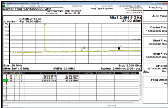
30MHz-3GHz_Band26_15MHz_QPSK_1_0_LowCH26865-831.5
