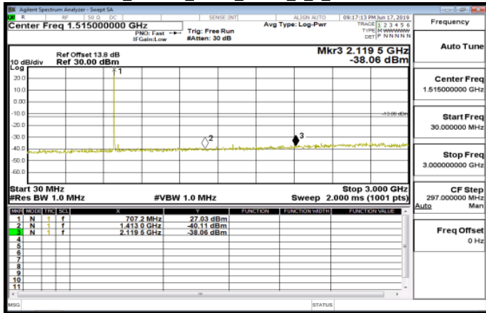
30MHz-3GHz_Band17_5MHz_QPSK_1_0_LowCH23755-706.5
