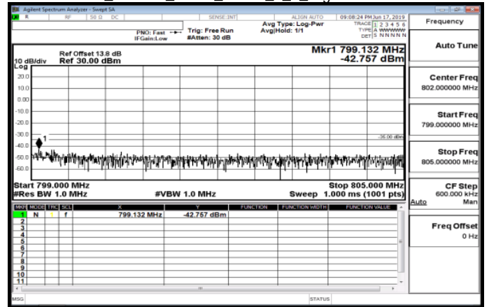
Inband-2_Band14_5MHz_QPSK_1_0_HighCH23355-795.5
