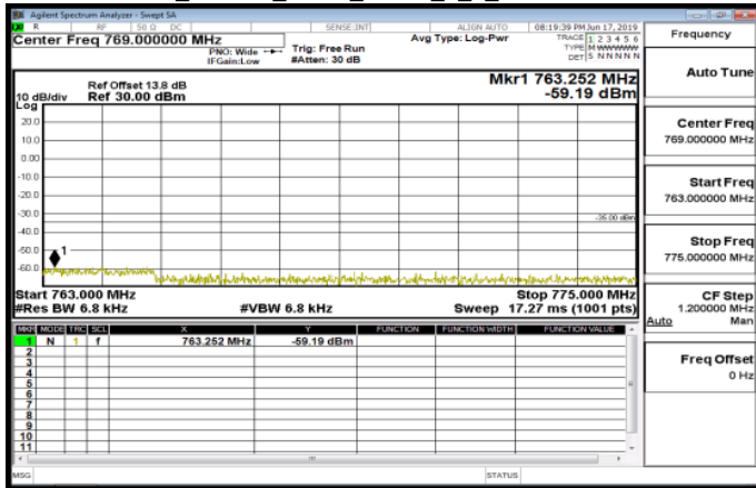
Inband-1_Band14_5MHz_QPSK_1_0_MidCH23330-793
