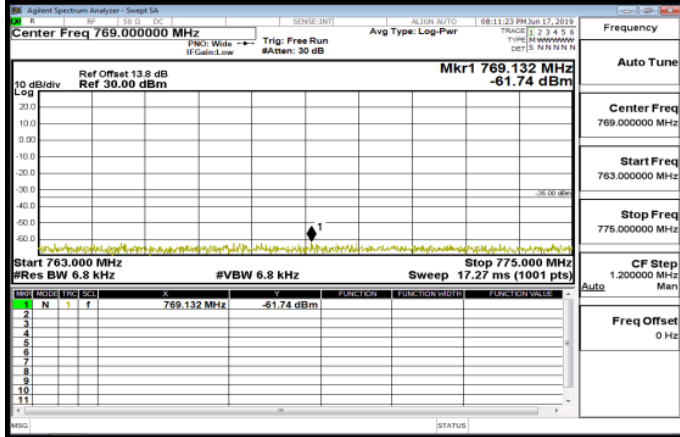
Inband-2_Band14_5MHz_QPSK_1_0_LowCH23305-790.5
