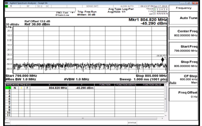
Inband-1_Band14_5MHz_QPSK_1_0_HighCH23355-795.5
