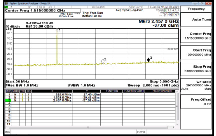
30MHz-3GHz_Band26_Part90s_3MHz_QPSK_1_0_MidCH26740-819
