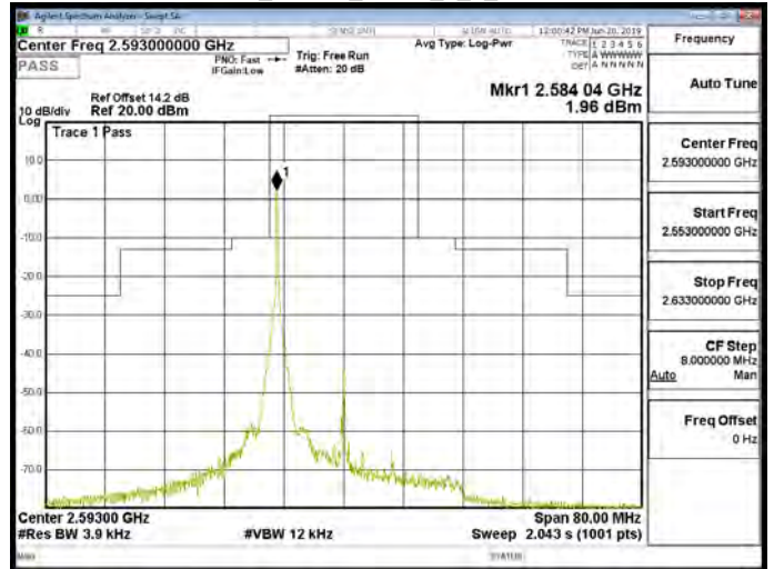
Band41_20MHz_QPSK_1_0_CH41490
