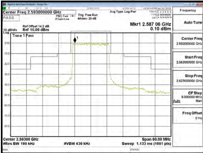
Band41_15MHz_QPSK_75_0_CH41515
