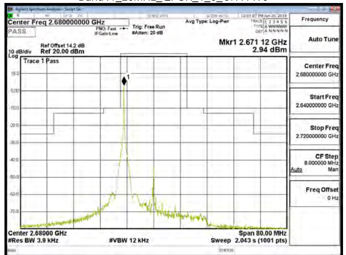
Band41_20MHz_QPSK_1_0_CH41490
