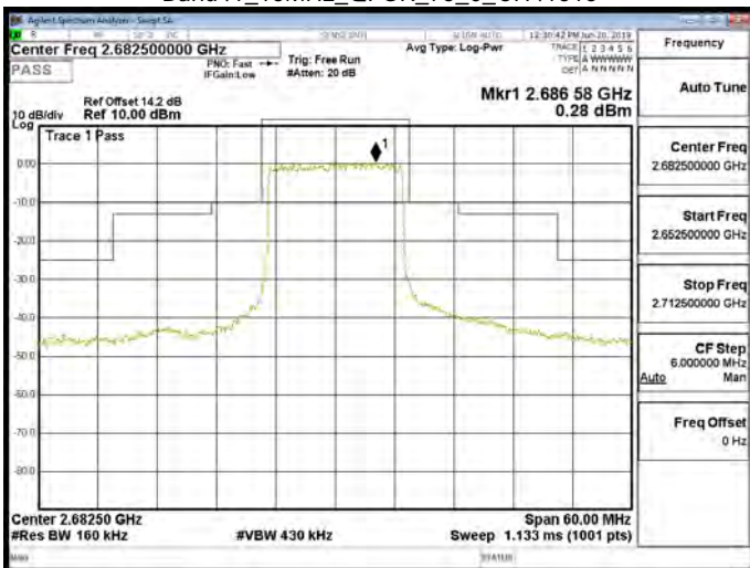
Band41_15MHz_QPSK_75_0_CH41515
