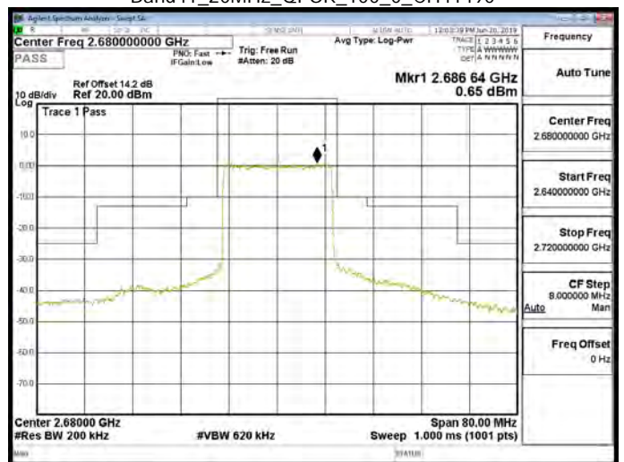
Band41_20MHz_QPSK_100_0_CH41490
