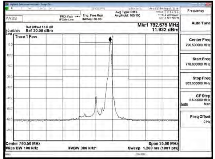
Band14_5MHz_QPSK_1_24_CH23330
