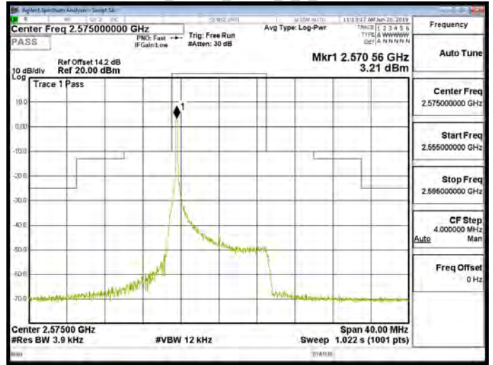
Band38_10MHz_QPSK_1_0_CH38000
