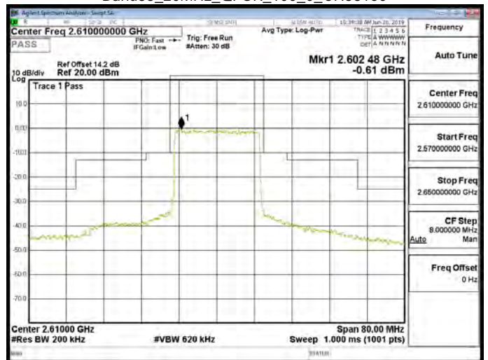
Band38_20MHz_QPSK_100_0_CH38150
