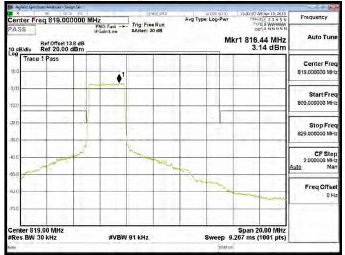
Band26_Part90s_3MHz_QPSK_15_0_CH26740
