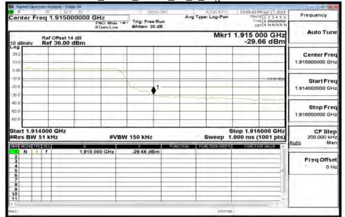
LTE\Band25_5MHz_QPSK_25_0_HighCH26665-1912.5
