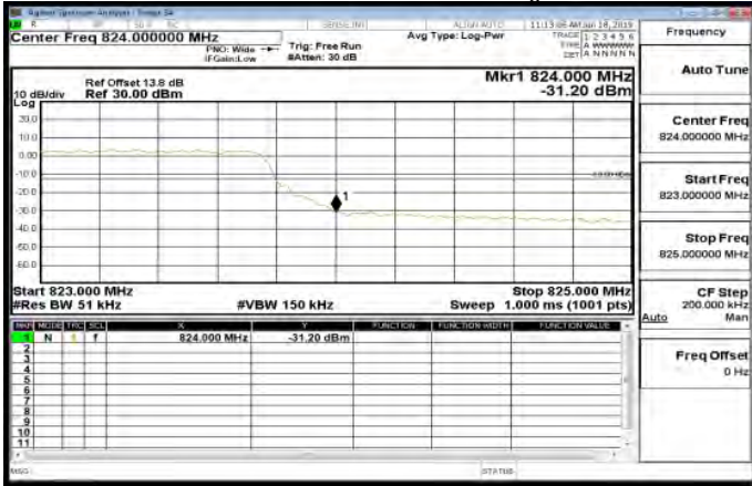
LTE/Band26_Part90s_10MHz_QPSK_1_0_LowCH26740-819
