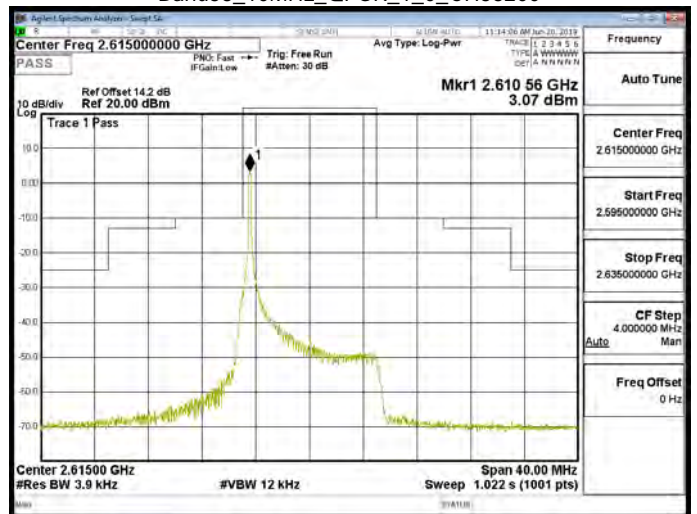
Band38_10MHz_QPSK_1_0_CH38200
