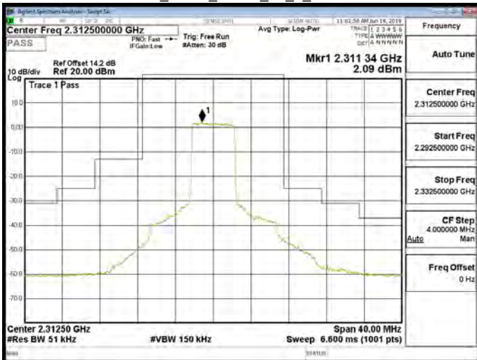
Band30_5MHz_QPSK_25_0_CH27735
