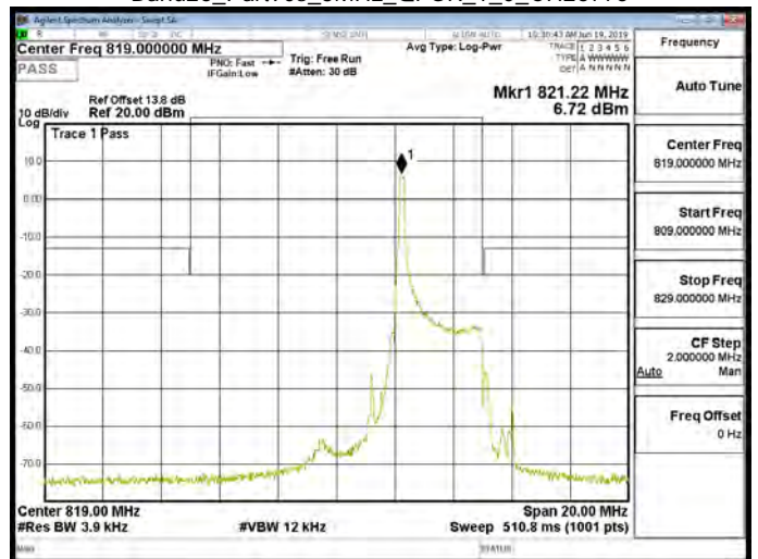
Band26_Part90s_3MHz_QPSK_1_0_CH26775
