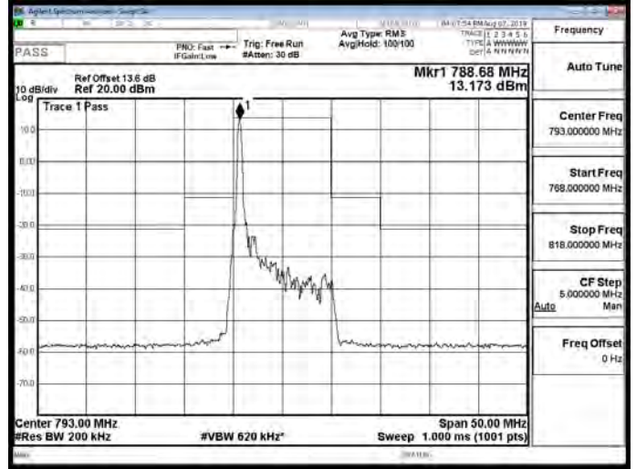
Band14_10MHz_QPSK_1_49_CH23330
