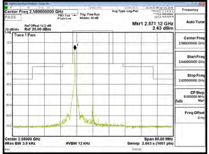
Band38_20MHz_QPSK_1_0_CH38000
