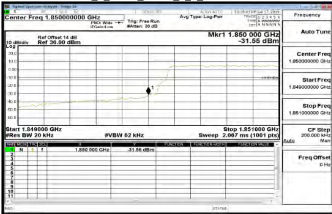
LTE\Band25_1_4MHz_QPSK_6_0_LowCH26047-1850.7
