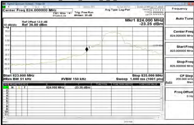
LTE\Band26_5MHz_QPSK_1_0_LowCH26815-826.5
