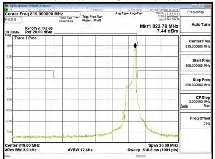
Band26_Part90s_1.4MHz_QPSK_1_5_CH26783
