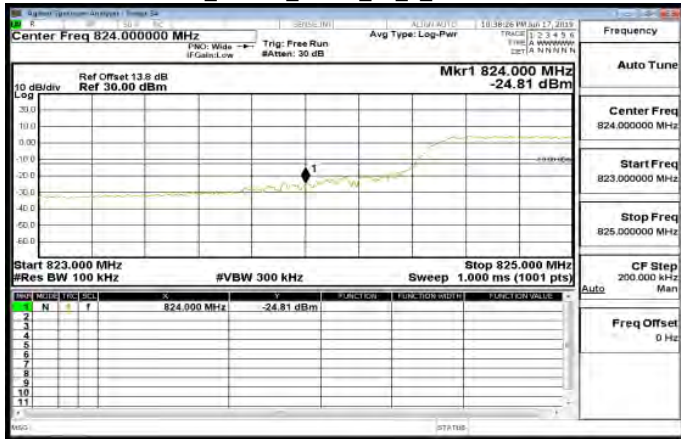
LTE\Band26_10MHz_QPSK_50_0_LowCH26840-829
