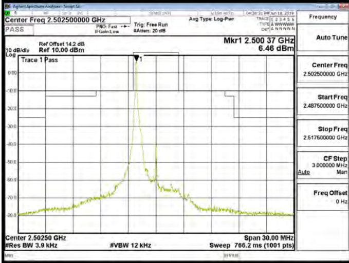
Band7_5MHz_QPSK_1_0_CH21100
