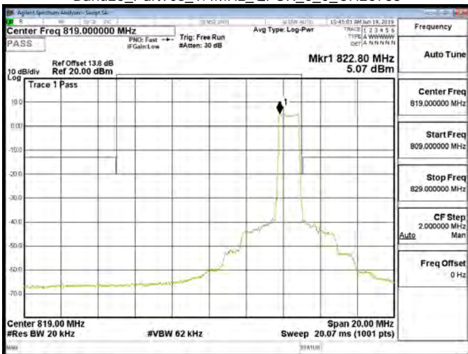
Band26_Part90s_1.4MHz_QPSK_6_0_CH26783
