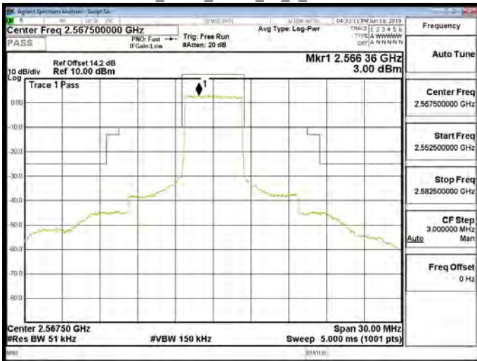
Band7_5MHz_QPSK_25_0_CH21425
