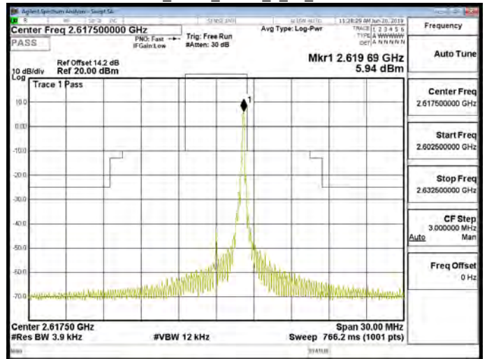
Band38_5MHz_QPSK_1_24_CH38225
