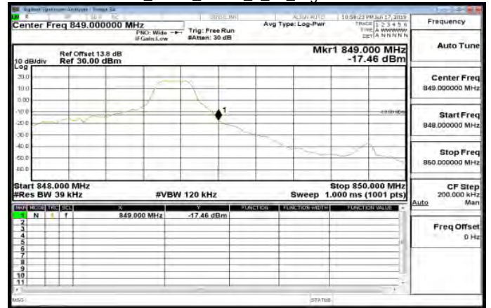
LTE\Band26_3MHz_QPSK_1_14_HighCH27025-847.5
