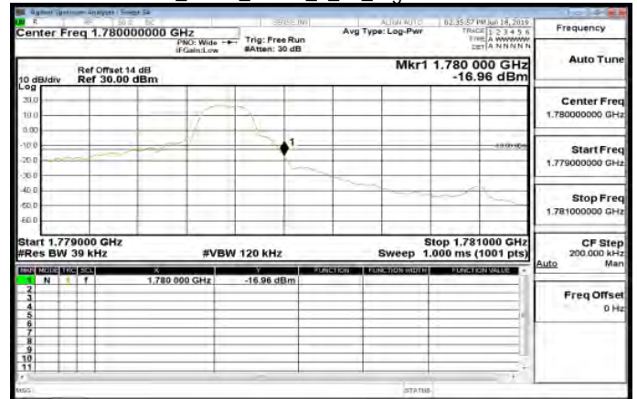
LTEBand66_3MHz_QPSK_1_14_HighCH132657-1778.5
