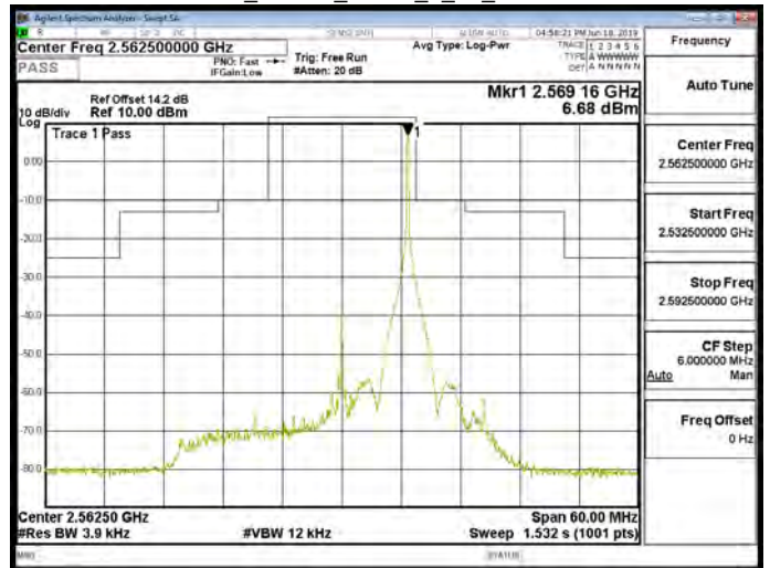
Band7_15MHz_QPSK_1_74_CH21375
