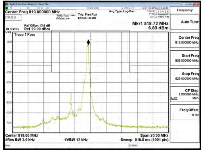
Band26_Part90s_5MHz_QPSK_1_24_CH26740
