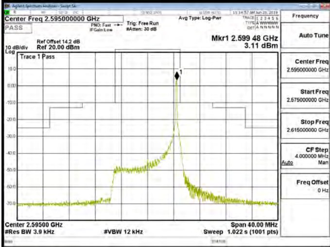
Band38_10MHz_QPSK_1_49_CH38200
