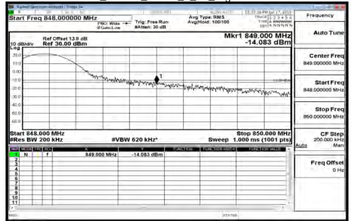
LTE\Band26_15MHz_QPSK_1_74_HighCH26965-841.5
