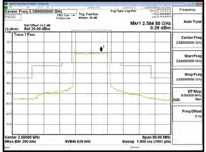
Band38_20MHz_QPSK_100_0_CH38000
