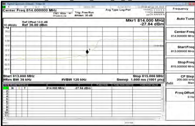
LTEBand26_Part90s_3MHz_QPSK_15_0_LowCH26705-815.5
