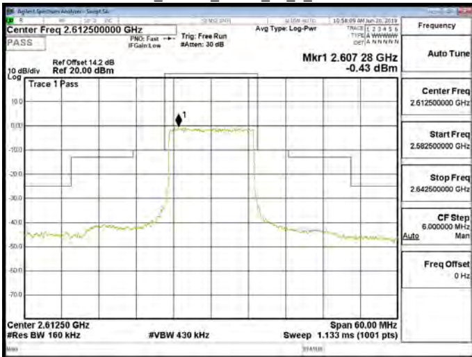
Band38_15MHz_QPSK_75_0_CH38175
