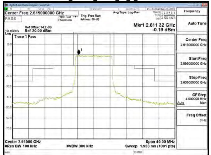
Band38_10MHz_QPSK_50_0_CH38200
