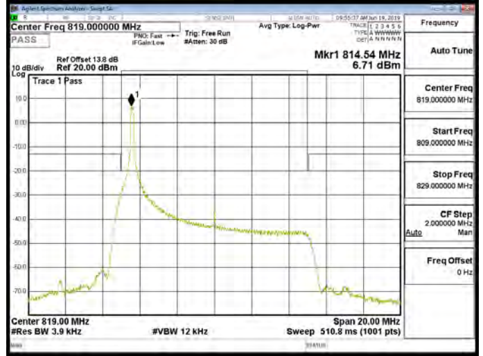
Band26_Part90s_10MHz_QPSK_1_49_CH26740
