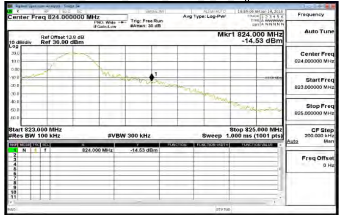
LTE/Band26_Part90s_10MHz_QPSK_50_0_LowCH26740-819
