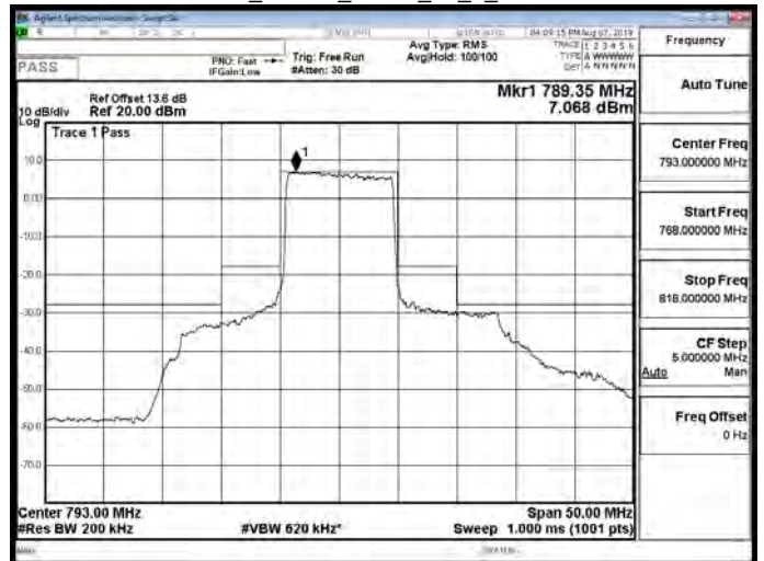
Band14_10MHz_QPSK_50_0_CH23330
