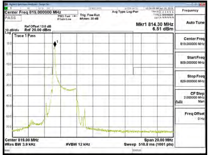
Band26_Part90s_3MHz_QPSK_1_0_CH26740
