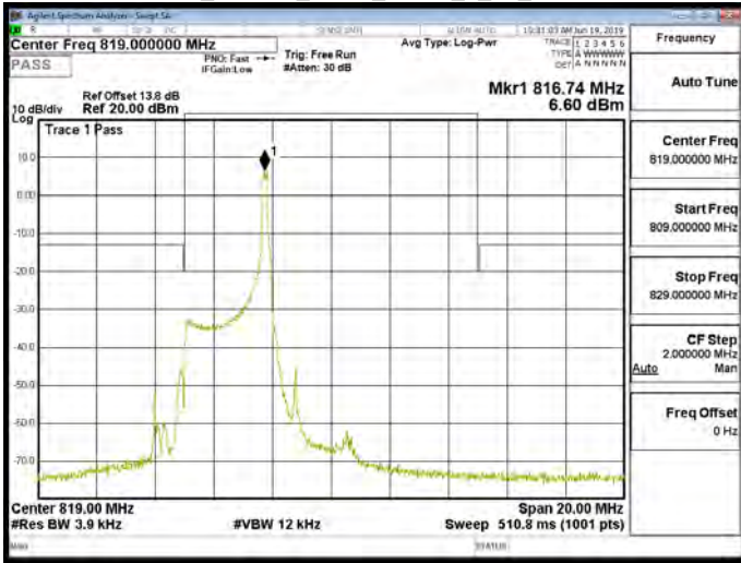
Band26_Part90s_3MHz_QPSK_1_14_CH26740
