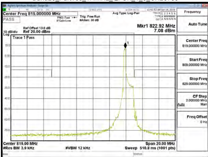
Band26_Part90s_1.4MHz_QPSK_1_0_CH26783
