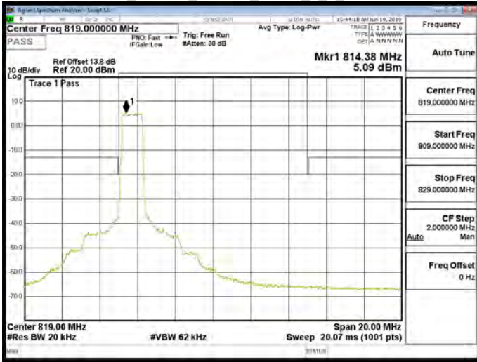
Band26_Part90s_1.4MHz_QPSK_6_0_CH26740
