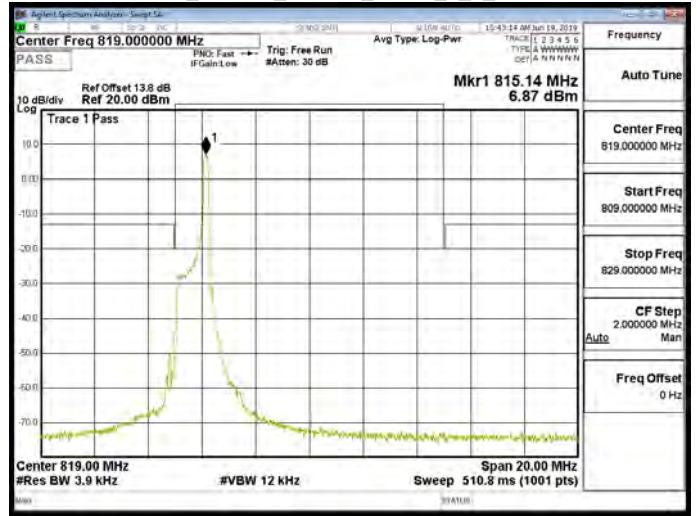
Band26_Part90s_1.4MHz_QPSK_1_5_CH26740
