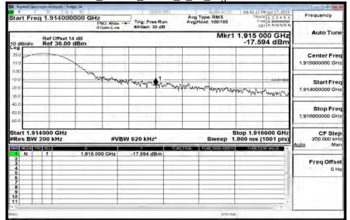
LTE\Band25_15MHz_QPSK_1_74_HighCH26615-1907.5
