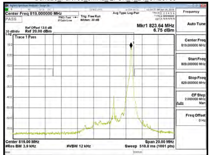
Band26_Part90s_5MHz_QPSK_1_24_CH26765
