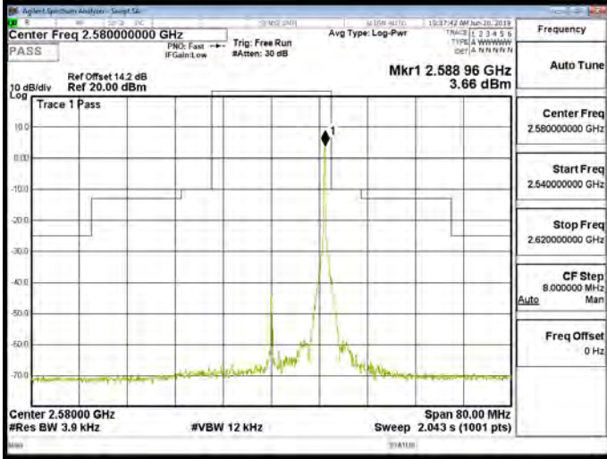
Band38_20MHz_QPSK_1_99_CH38000
