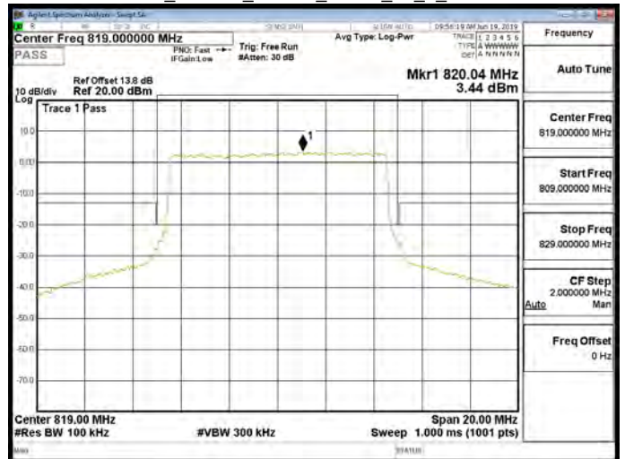
Band26_Part90s_10MHz_QPSK_50_0_CH26740
