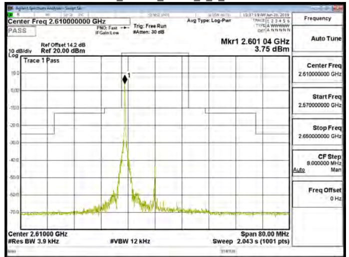
Band38_20MHz_QPSK_1_0_CH38150
