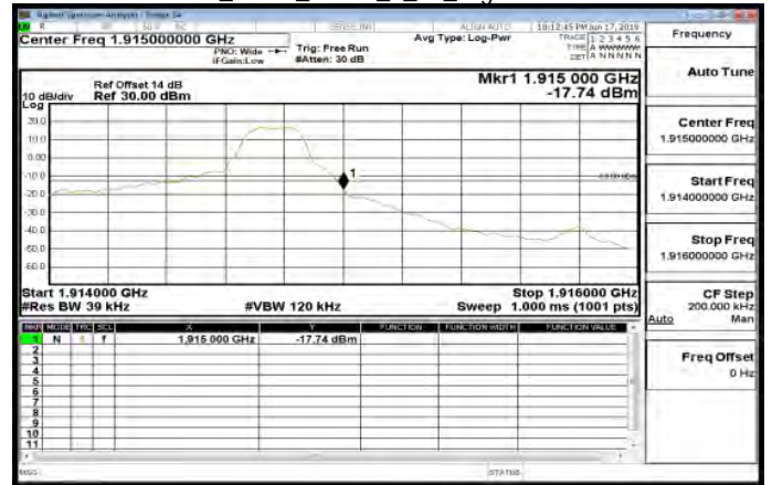
LTE\Band25_3MHz_QPSK_1_14_HighCH26675-1913.5
