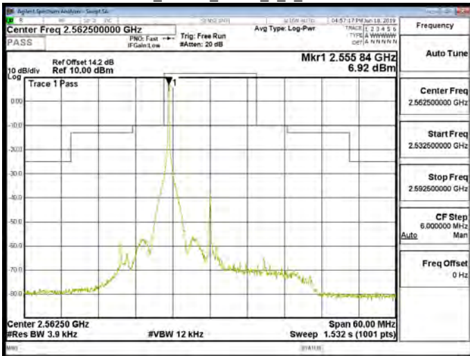
Band7_15MHz_QPSK_1_0_CH21375
