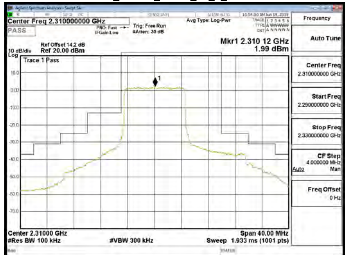
Band30_10MHz_QPSK_50_0_CH27710
