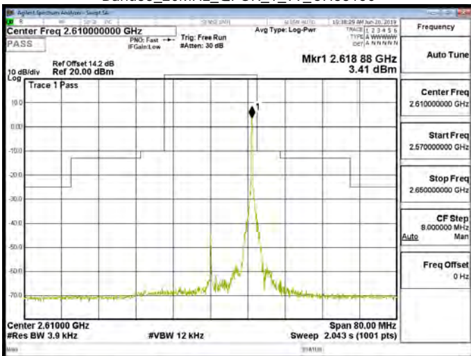
Band38_20MHz_QPSK_1_99_CH38150
