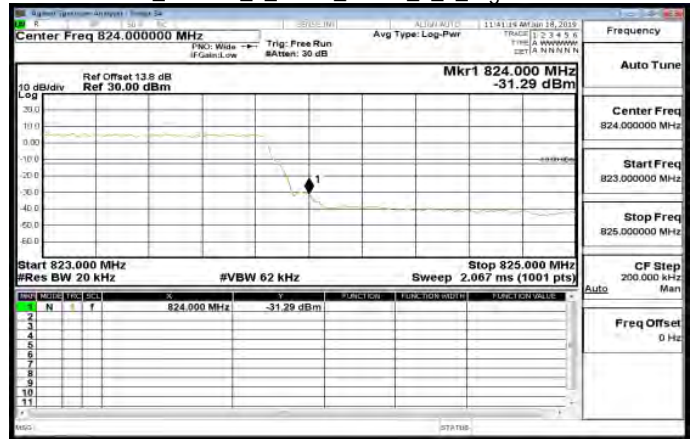
LTE\Band26_Part90s_1_4MHz_QPSK_6_0_HighCH26783-823.3
