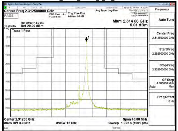
Band30_5MHz_QPSK_1_24_CH27735
