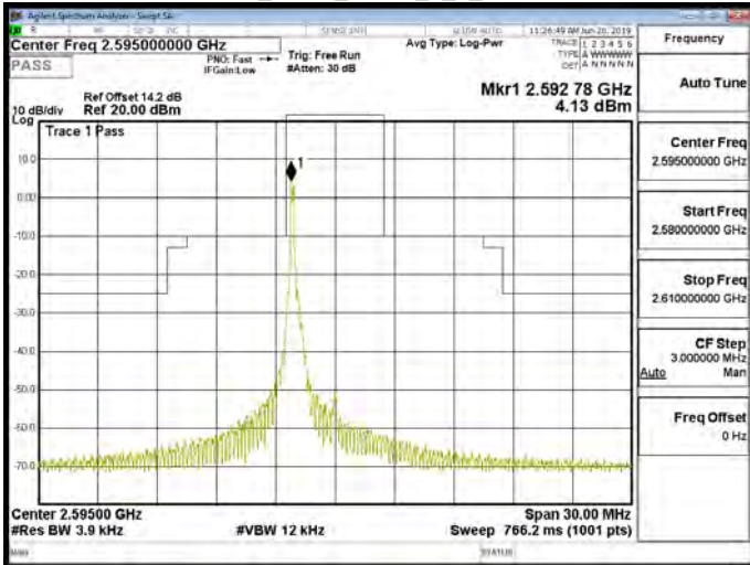
Band38_5MHz_QPSK_1_0_CH38225
