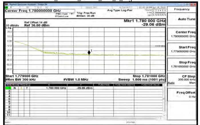
LTEBand66_20MHz_QPSK_100_0_HighCH132572-1770
