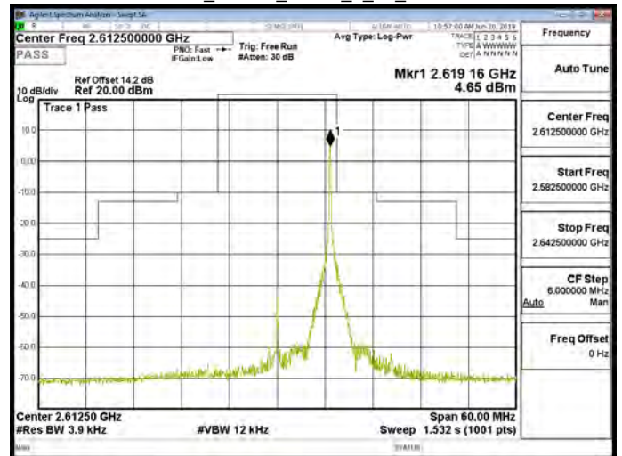
Band38_15MHz_QPSK_1_74_CH38175
