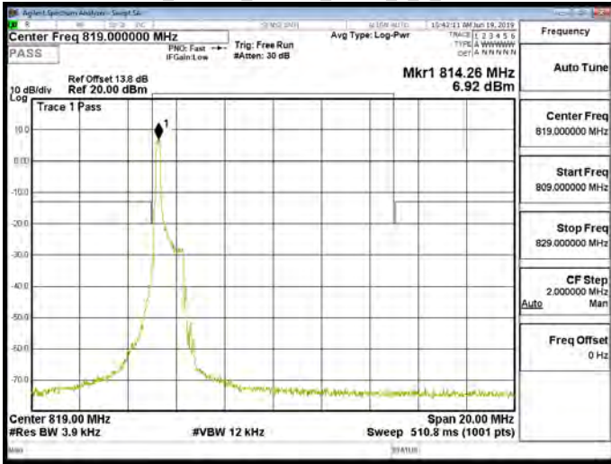
Band26_Part90s_1.4MHz_QPSK_1_0_CH26740
