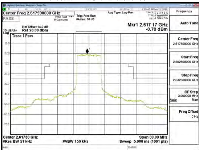
Band38_5MHz_QPSK_25_0_CH38225
