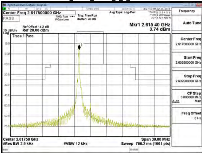
Band38_5MHz_QPSK_1_0_CH38225
