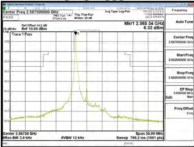
Band7_5MHz_QPSK_1_0_CH21425
