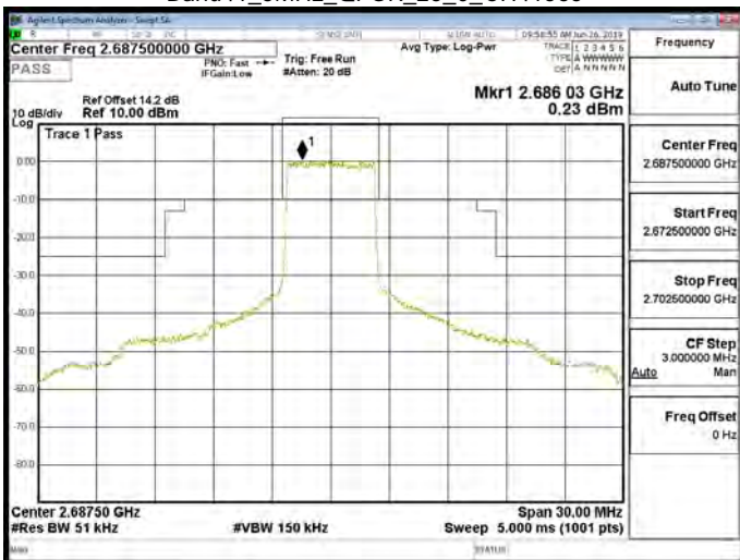
Band41_5MHz_QPSK_25_0_CH41565
