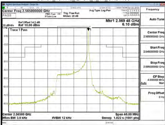
Band7_10MHz_QPSK_1_49_CH21400
