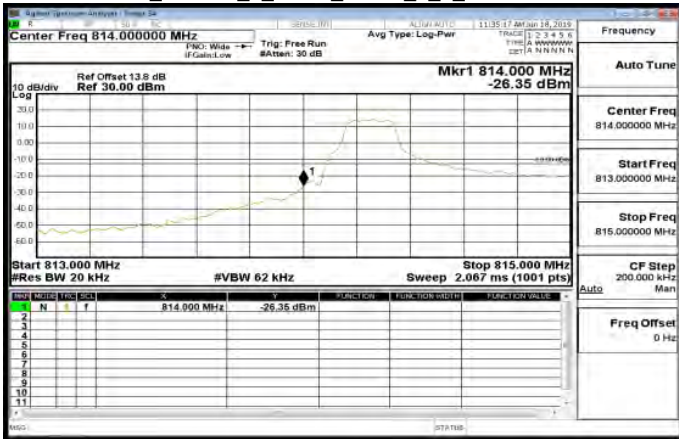
LTE\Band26_Part90s_1_4MHz_QPSK_1_0_LowCH26697-814.7
