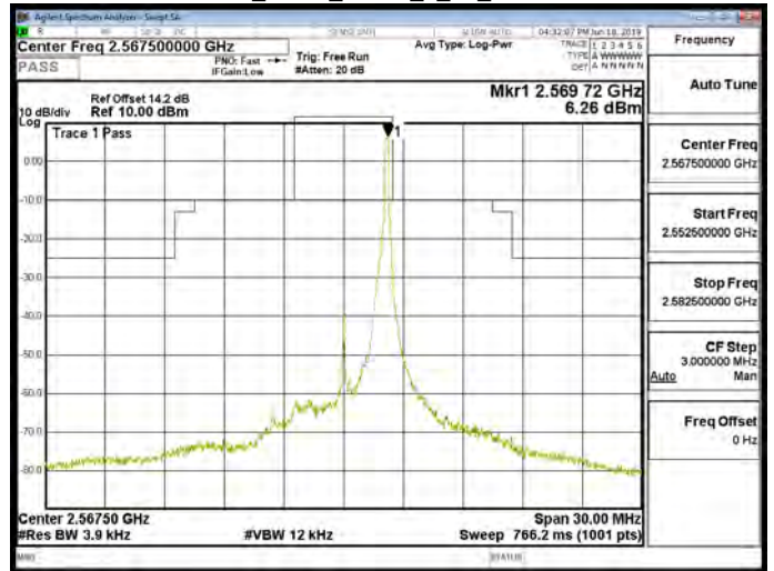
Band7_5MHz_QPSK_1_24_CH21425
