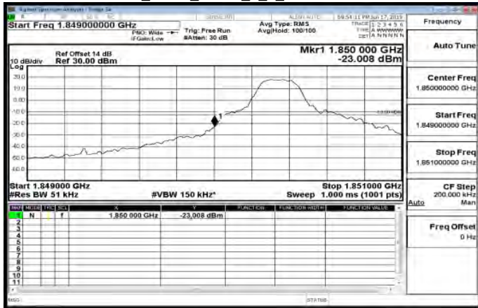
LTE\Band25_5MHz_QPSK_1_0_LowCH26065-1852.5
