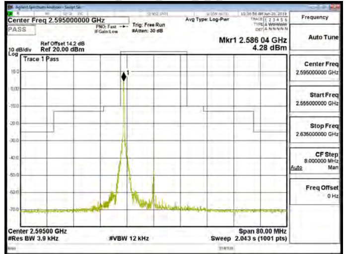
Band38_20MHz_QPSK_1_0_CH38150
