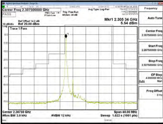
Band30_5MHz_QPSK_1_0_CH27710
