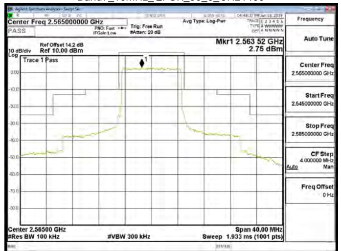
Band7_10MHz_QPSK_50_0_CH21400
