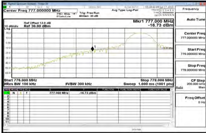
LTE\Band13_10MHz_QPSK_1_49_HighCH23230-782
