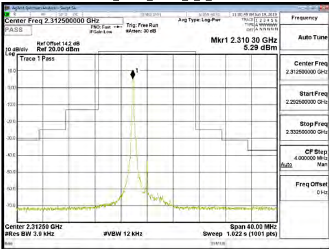
Band30_5MHz_QPSK_1_0_CH27735
