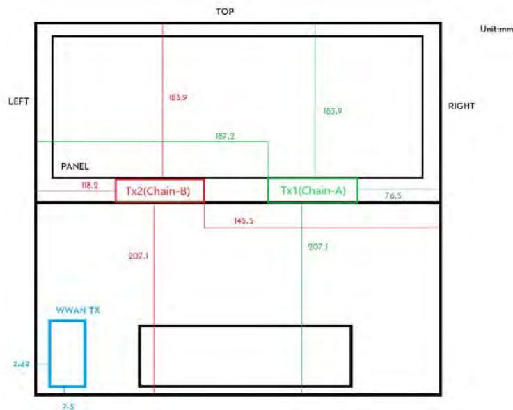
Fig.10 Antenna location of EUT (Laptop mode)
