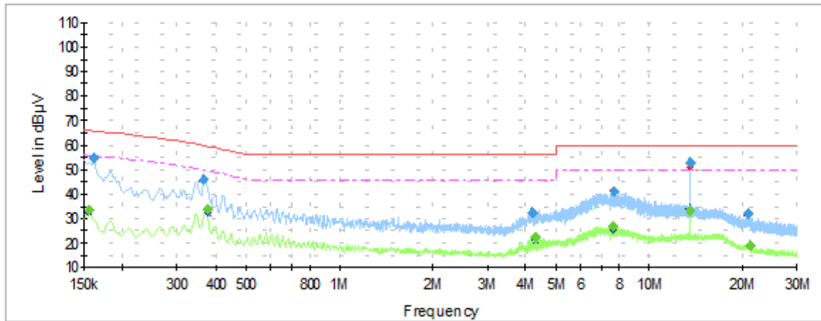
— Peak measurements — Avg measurements — Limit FCC Quasi-Peak - - - Limit FCC Avg
