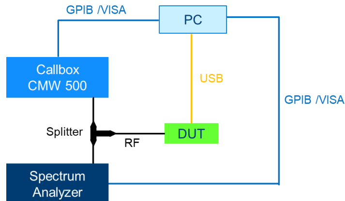
Figure 1 - Test Setup
