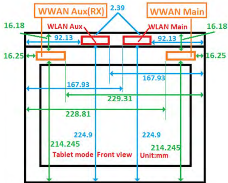
Fig.12 Antenna location (front view of tablet mode)
