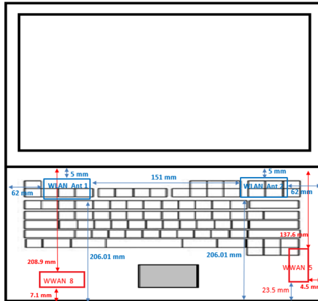
Photograph 7. Antenna position of EUT
