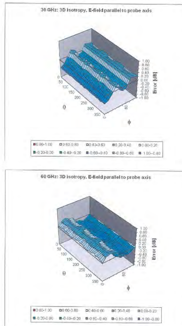
Probe isotropy for E_{\text{eff}} ; probe rotated \psi = 0^\circ to 360^\circ , tilted from field propagation direction \vec{k} Parallel to the field propagation ( \psi = 0^\circ - 90^\circ ) at 30 GHz: deviation within \pm 0.40 dB Parallel to the field propagation ( \psi = 0^\circ - 90^\circ ) at 60 GHz: deviation within \pm 0.38 dB
