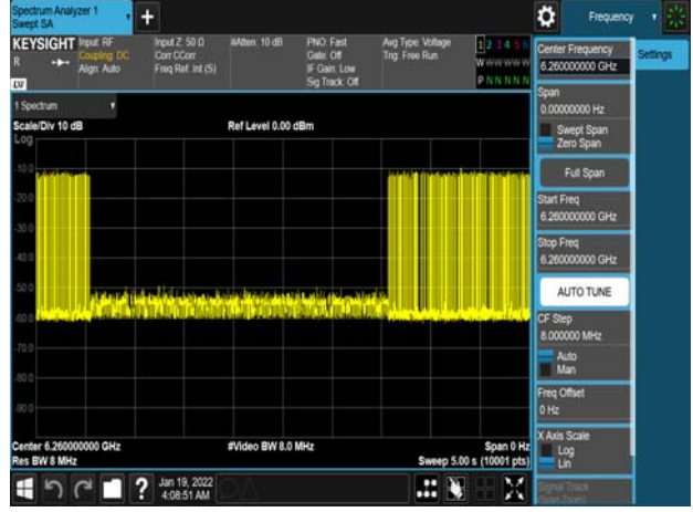
Det LeI_802.11ax_160MHz_6260MHz_-63dBm
