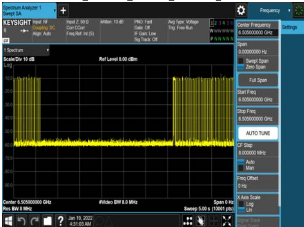
Det Le1_802.11ax_160MHz_6505MHz_-66dBm
