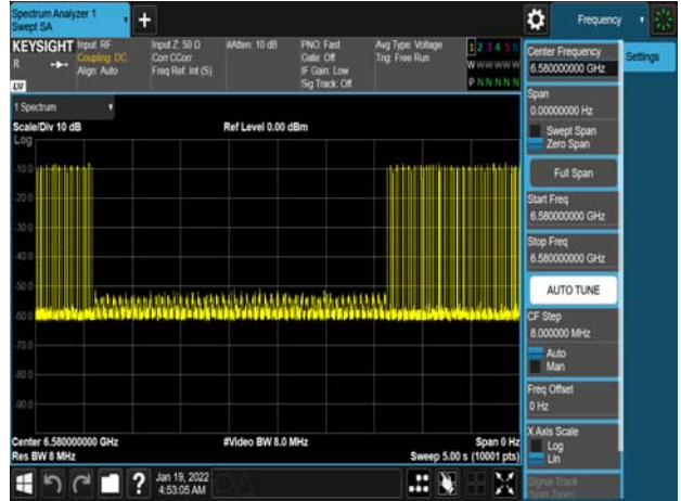
Det Le1_802.11ax_160MHz_6580MHz_-67dBm
