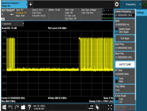
Det LeI_802.11ax_160MHz_6185MHz_-67dBm
