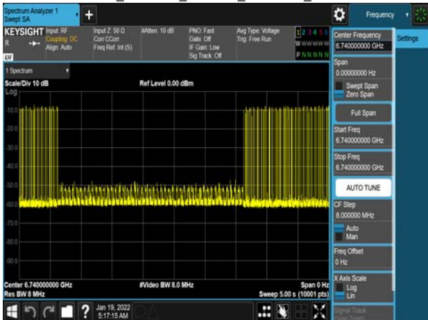
Det Le1_802.11ax_160MHz_6740MHz_-63dBm
