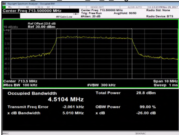
Band12_5MHz_QPSK_25_0_HighCH23155-713.5
