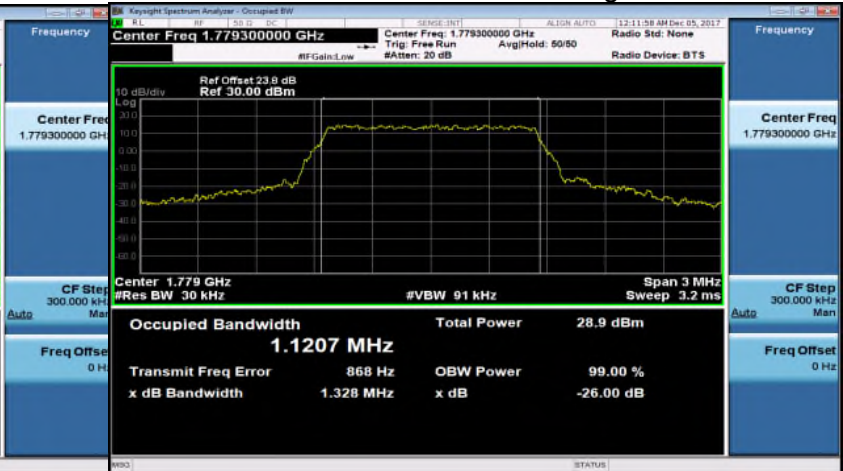
Band66_1_4MHz_16QAM_6_0_HighCH132665
