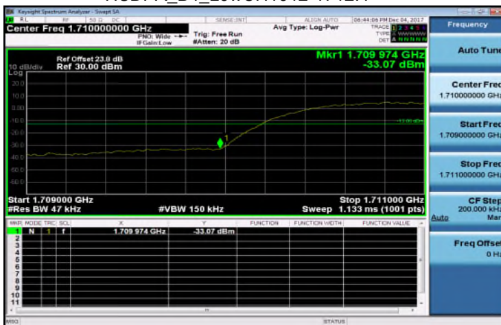
HSDPA_B4_LowCH1312-1712.4
