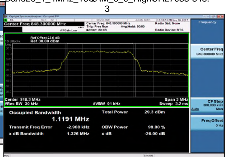
Band26_1_4MHz_16QAM_6_0_HighCH27033-848.3
