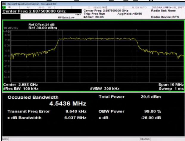
Band41_5MHz_16QAM_25_0_HighCH41565
