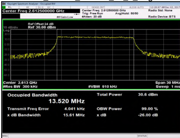
Band38_15MHz_16QAM_75_0_HighCH38175
