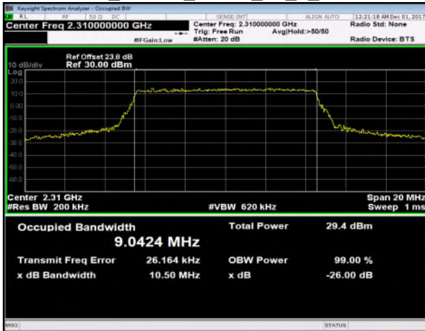
Band30_10MHz_16QAM_50_0_MidCH27710
