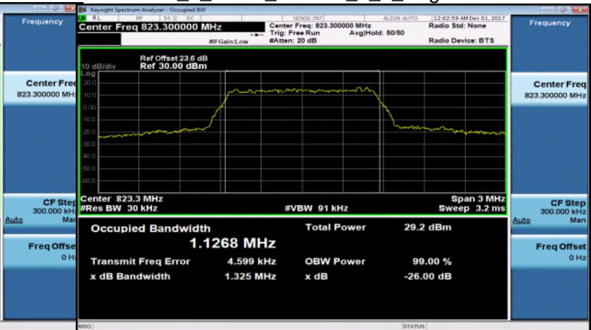
Band26_1_4MHz_16QAM_6_0_HighCH26783
