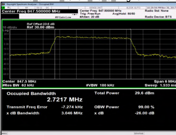
Band26_3MHz_QPSK_15_0_HighCH27025-847.5
