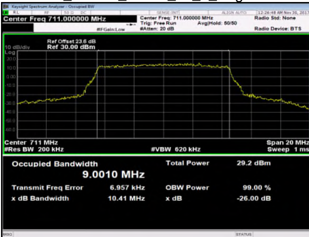
Band17_10MHz_QPSK_50_0_HighCH23800-711
