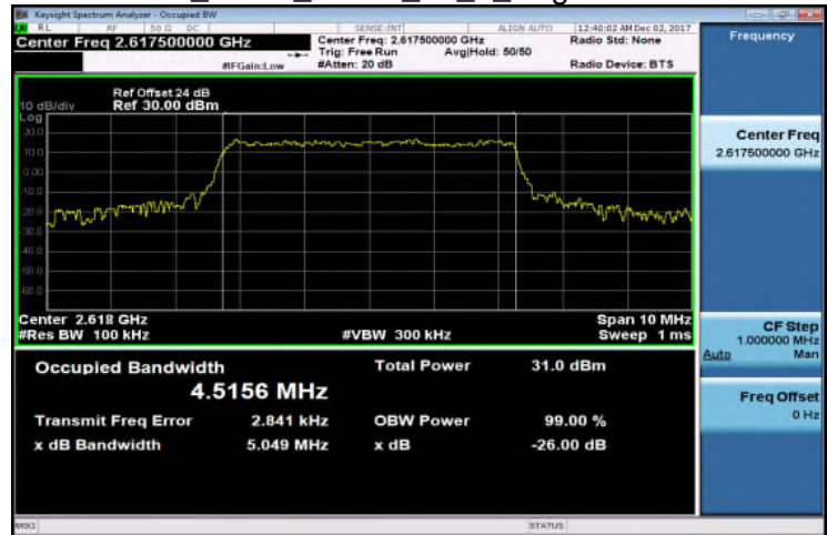
Band38_5MHz_QPSK_25_0_HighCH38225
