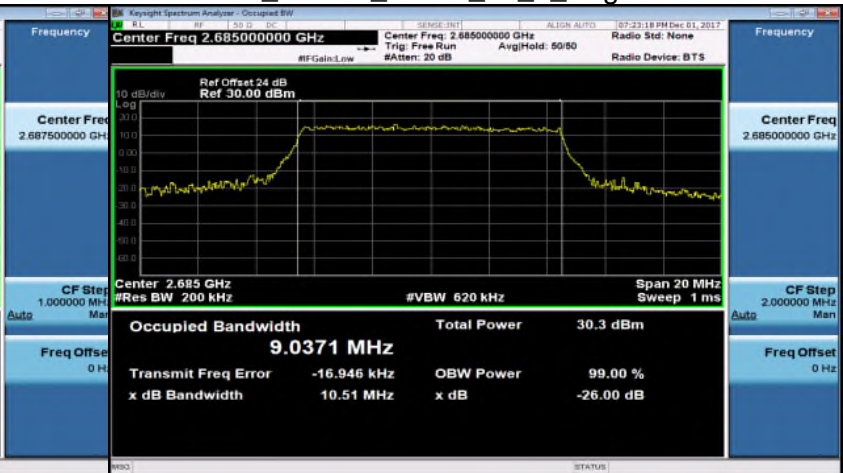
Band41_10MHz_QPSK_50_0_HighCH41540
