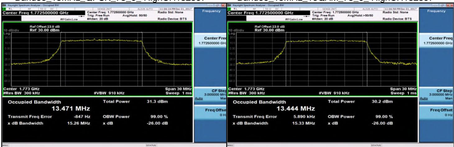
Band66_15MHz_QPSK_75_0_HighCH132597
