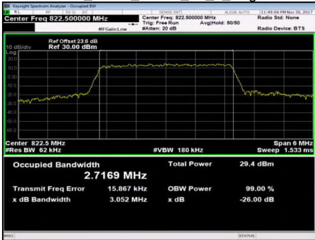
Band26_3MHz_QPSK_15_0_HighCH26775
