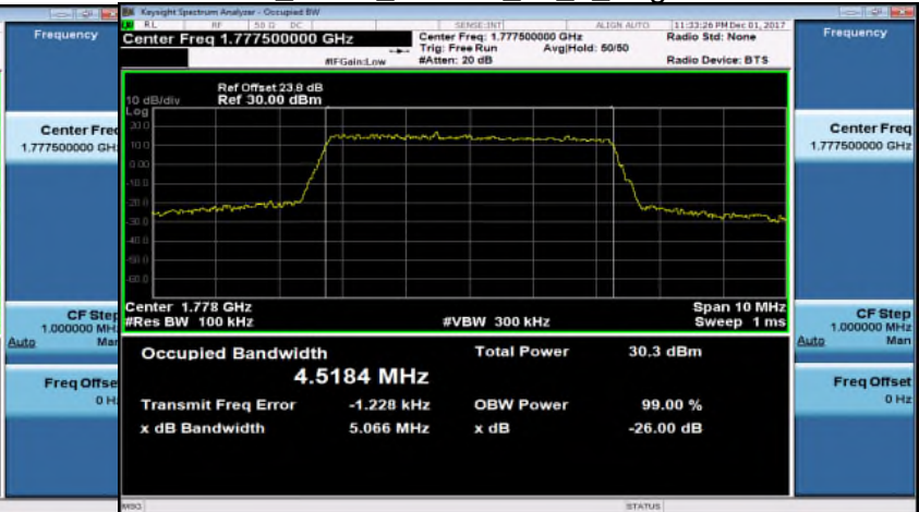
Band66_5MHz_16QAM_25_0_HighCH132647
