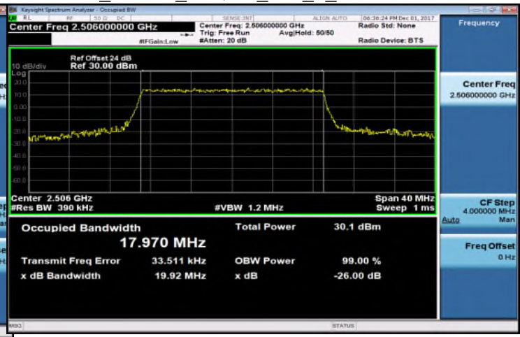
Band41_20MHz_16QAM_100_0_MidCH40620
