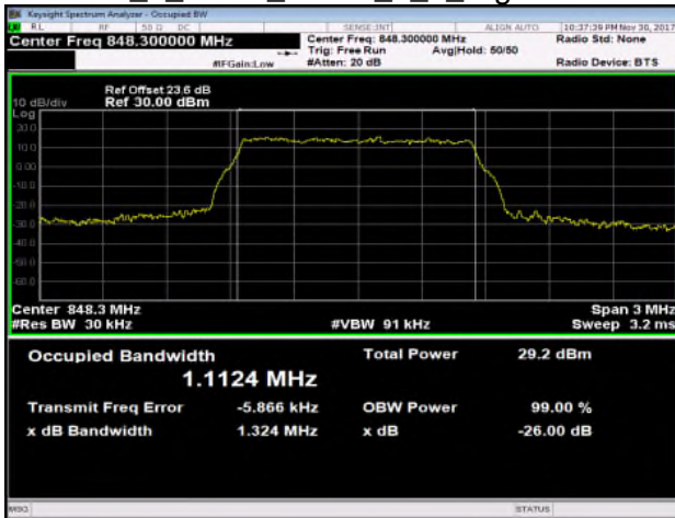
Band26_1_4MHz_QPSK_6_0_HighCH27033-848.3
