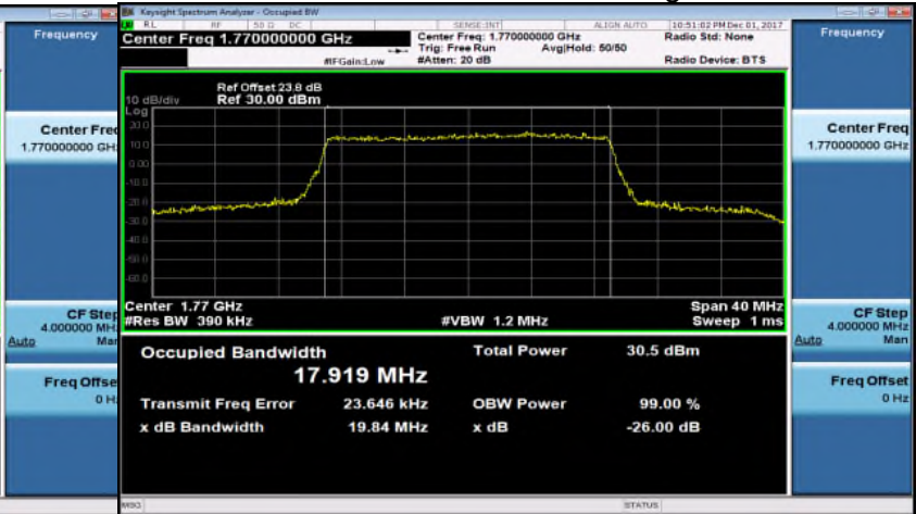
Band66_20MHz_16QAM_100_0_HighCH132572
