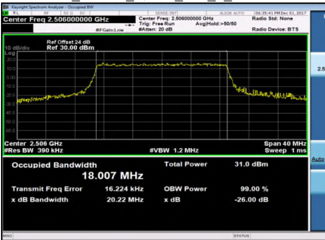
Band41_20MHz_QPSK_100_0_MidCH40620
