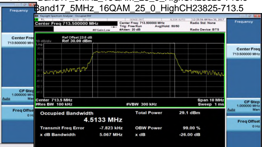
Band17_5MHz_16QAM_25_0_HighCH23825-713.5
