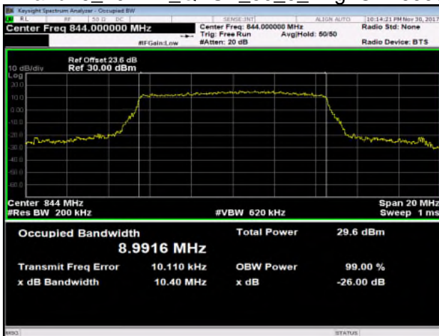
Band26_10MHz_QPSK_50_0_HighCH26990-844
