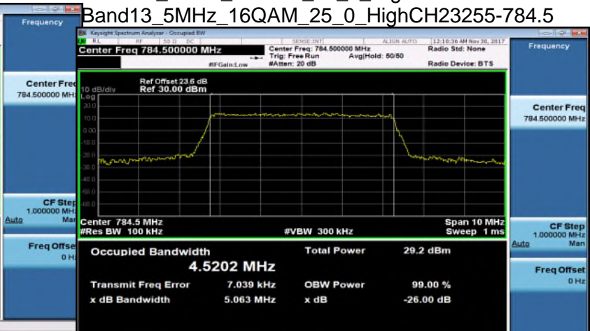
Band13_5MHz_16QAM_25_0_HighCH23255-784.5
