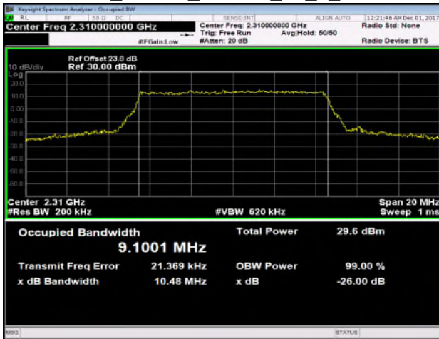
Band30_10MHz_16QAM_50_0_MidCH27710
