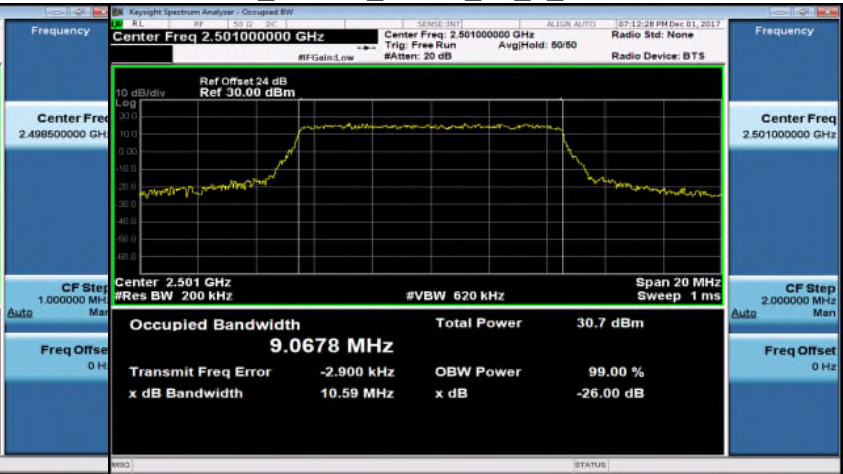
Band41_10MHz_QPSK_50_0_MidCH40620
