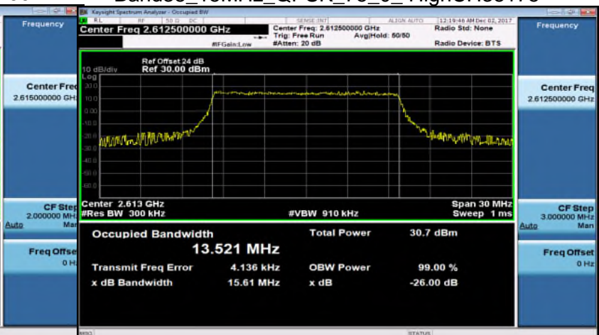
Band38_15MHz_QPSK_75_0_HighCH38175
