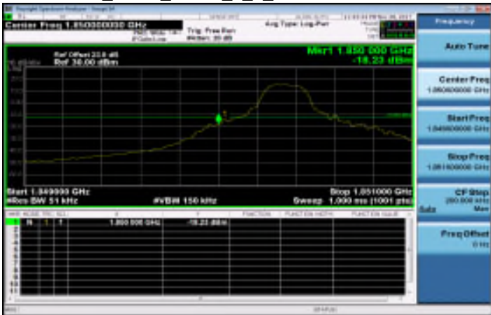
Band2_5MHz_QPSK_1_0_LowCH18625-1852.5
