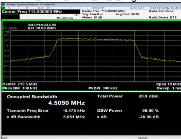
Band17_5MHz_QPSK_25_0_HighCH23825-713.5
