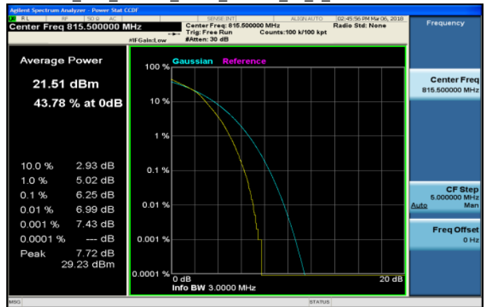
Part 90_LTE_Band26_3MHz_16QAM_15_0_LowCH26705-815.5
