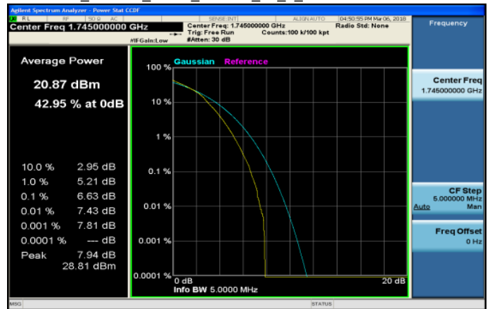
LTE_Band66_5MHz_16QAM_25_0_MidCH132322-1745
