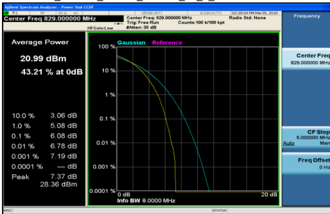
LTE_Band26_10MHz_16QAM_50_0_LowCH26840-829
