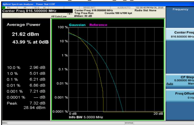
Part 90_LTE_Band26_5MHz_16QAM_25_0_LowCH26715-816.5
