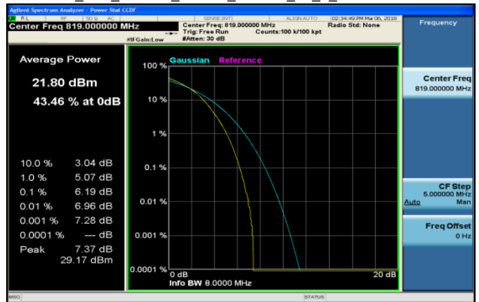
Part 90_LTE_Band26_10MHz_16QAM_50_0_MidCH26740-819
