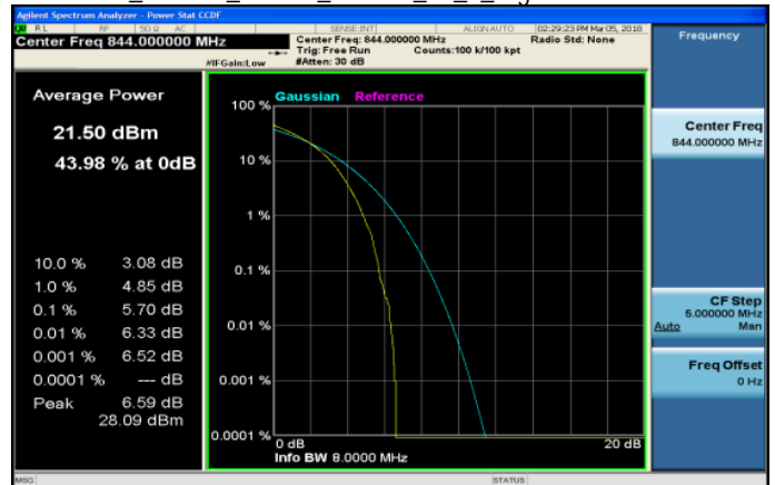
LTE_Band26_10MHz_16QAM_50_0_HighCH26990-844
