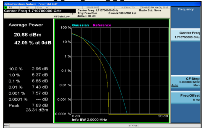
LTE_Band66_1_4MHz_16QAM_6_0_LowCH131979-1710.7
