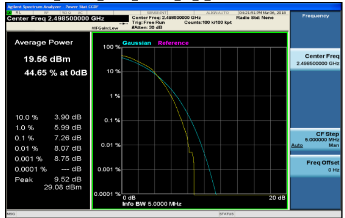
LTE_Band41_5MHz_16QAM_25_0_LowCH39675-2498.5
