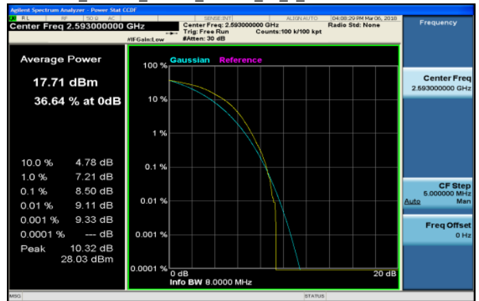
LTE_Band41_15MHz_16QAM_75_0_MidCH40620-2593
