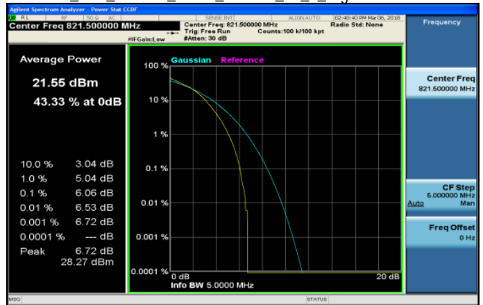
Part 90_LTE_Band26_5MHz_16QAM_25_0_HighCH26765-821.5
