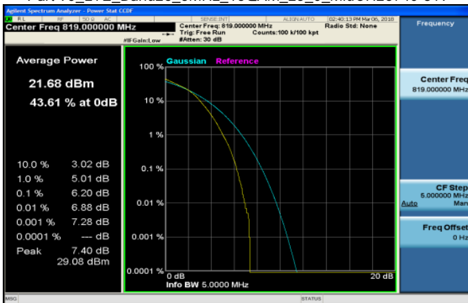
Part 90_LTE_Band26_5MHz_16QAM_25_0_MidCH26740-819
