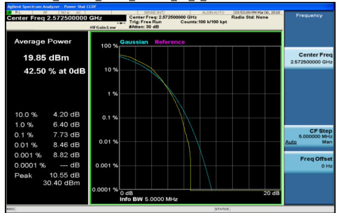
LTE_Band38_5MHz_16QAM_25_0_LowCH37775-2572.5
