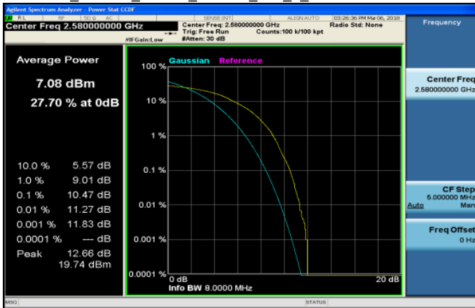
LTE_Band38_20MHz_16QAM_100_0_LowCH37850-2580
