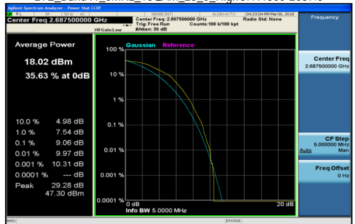
LTE_Band41_5MHz_16QAM_25_0_HighCH41565-2687.5
