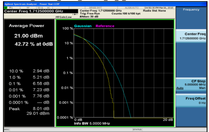
LTE_Band66_5MHz_16QAM_25_0_LowCH131997-1712.5
