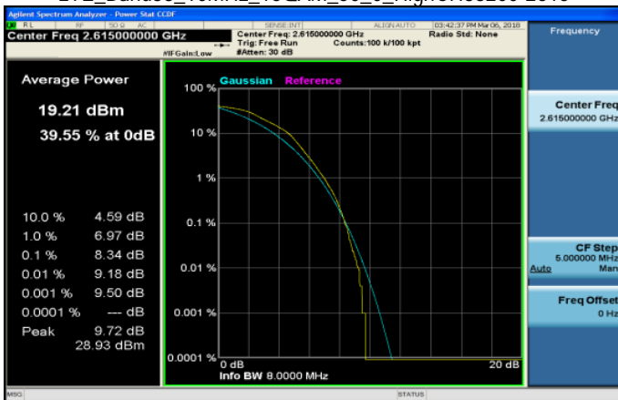
LTE_Band38_10MHz_16QAM_50_0_HighCH38200-2615
