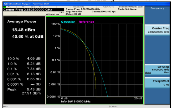
LTE_Band41_15MHz_16QAM_75_0_HighCH41515-2682.5
