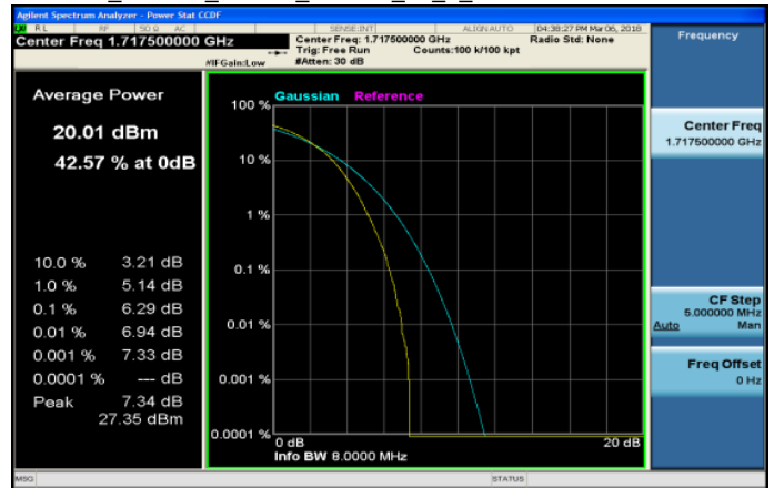
LTE_Band66_15MHz_16QAM_75_0_LowCH132047-1717.5
