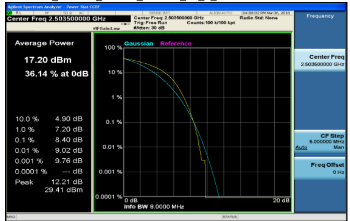
LTE_Band41_15MHz_16QAM_75_0_LowCH39725-2503.5
