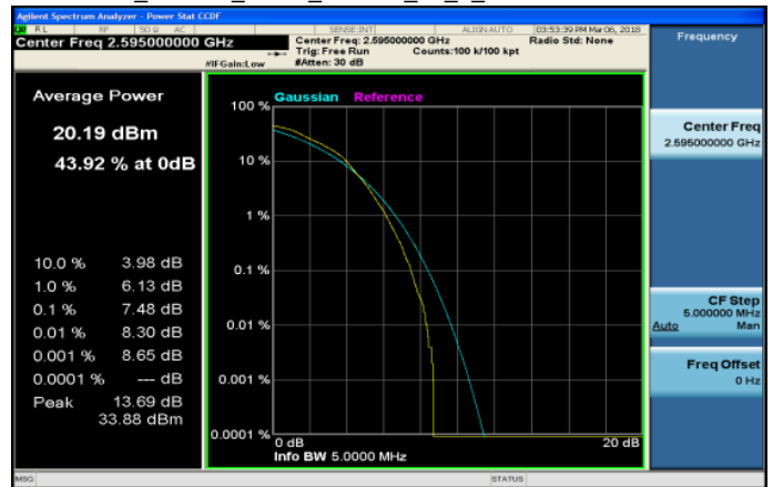
LTE_Band38_5MHz_16QAM_25_0_MidCH38000-2595
