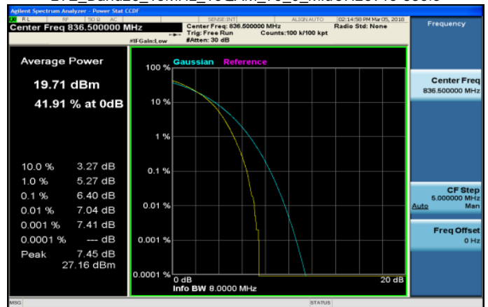
LTE_Band26_15MHz_16QAM_75_0_MidCH26915-836.5
