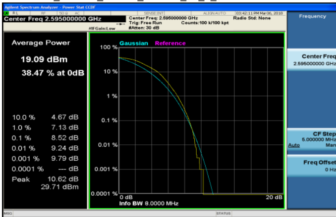
LTE_Band38_10MHz_16QAM_50_0_MidCH38000-2595
