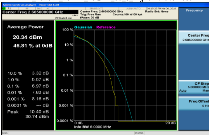
LTE_Band41_10MHz_16QAM_50_0_HighCH41540-2685
