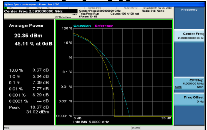
LTE_Band41_5MHz_16QAM_25_0_MidCH40620-2593
