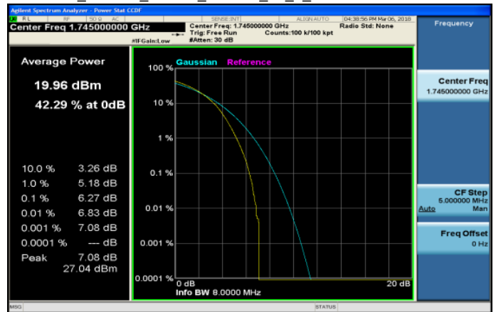
LTE_Band66_15MHz_16QAM_75_0_MidCH132322-1745
