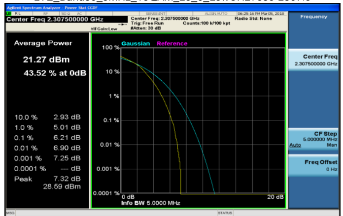
LTE_Band30_5MHz_16QAM_25_0_LowCH27685-2307.5
