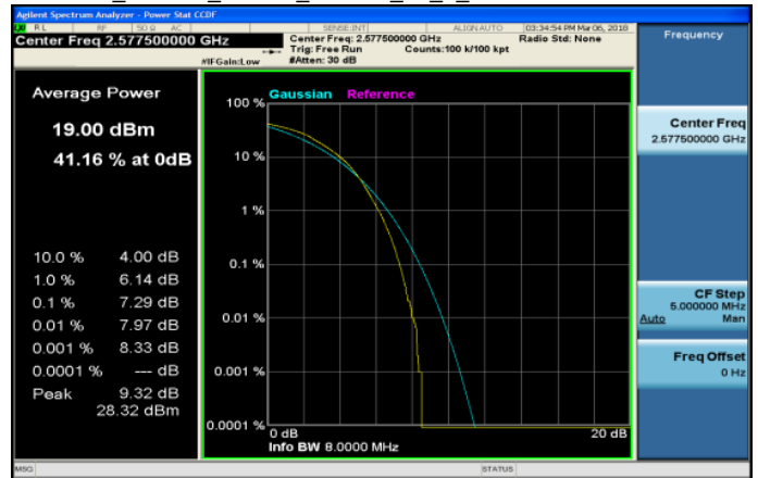
LTE_Band38_15MHz_16QAM_75_0_LowCH37825-2577.5
