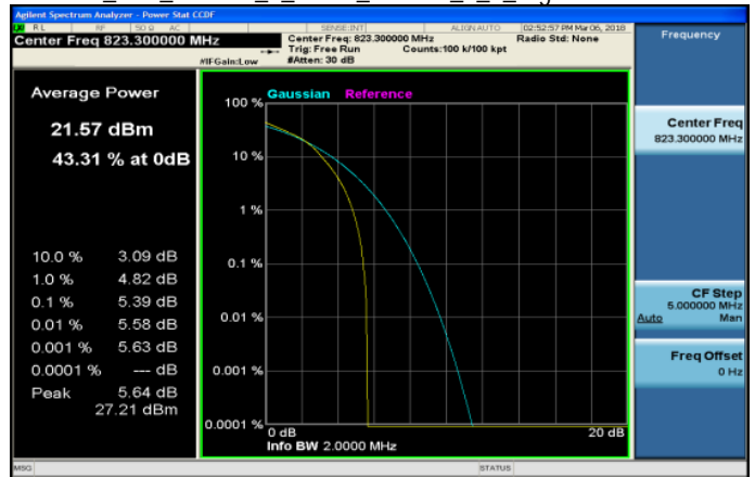
Part 90_LTE_Band26_1_4MHz_16QAM_6_0_HighCH26783-823.3
