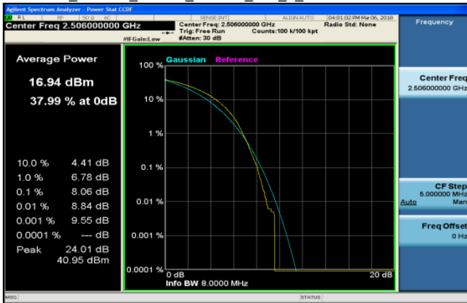
LTE_Band41_20MHz_16QAM_100_0_LowCH39750-2506
