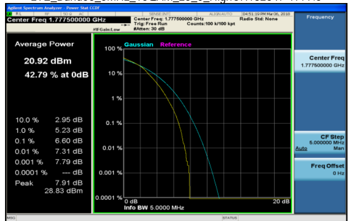
LTE_Band66_5MHz_16QAM_25_0_HighCH132647-1777.5
