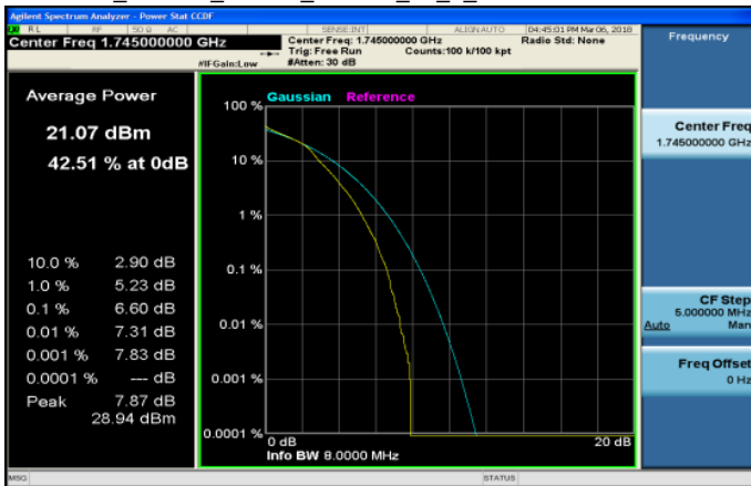
LTE_Band66_10MHz_16QAM_50_0_MidCH132322-1745
