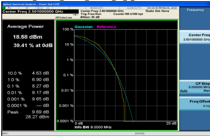
LTE_Band41_10MHz_16QAM_50_0_LowCH39700-2501
