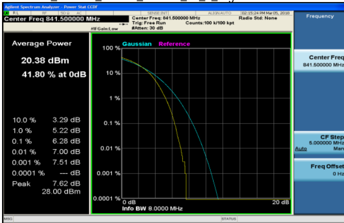
LTE_Band26_15MHz_16QAM_75_0_HighCH26965-841.5
