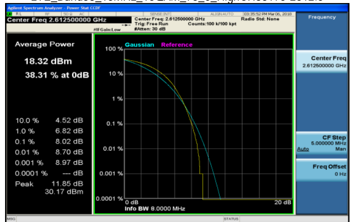
LTE_Band38_15MHz_16QAM_75_0_HighCH38175-2612.5
