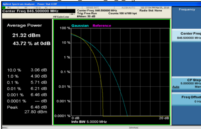
LTE_Band26_5MHz_16QAM_25_0_HighCH27015-846.5
