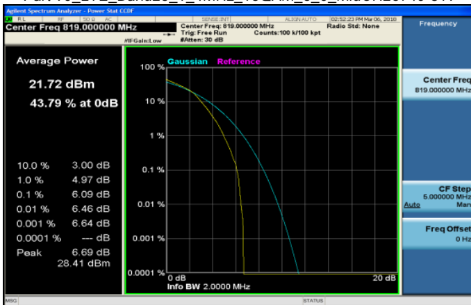
Part 90_LTE_Band26_1_4MHz_16QAM_6_0_MidCH26740-819
