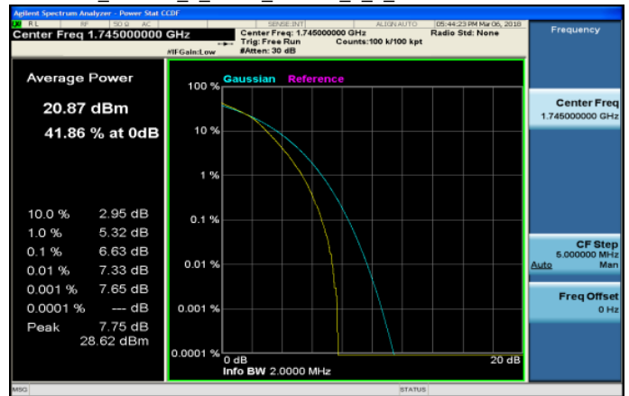
LTE_Band66_1_4MHz_16QAM_6_0_MidCH132322-1745
