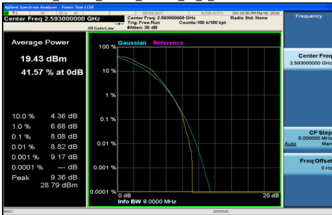
LTE_Band41_10MHz_16QAM_50_0_MidCH40620-2593
