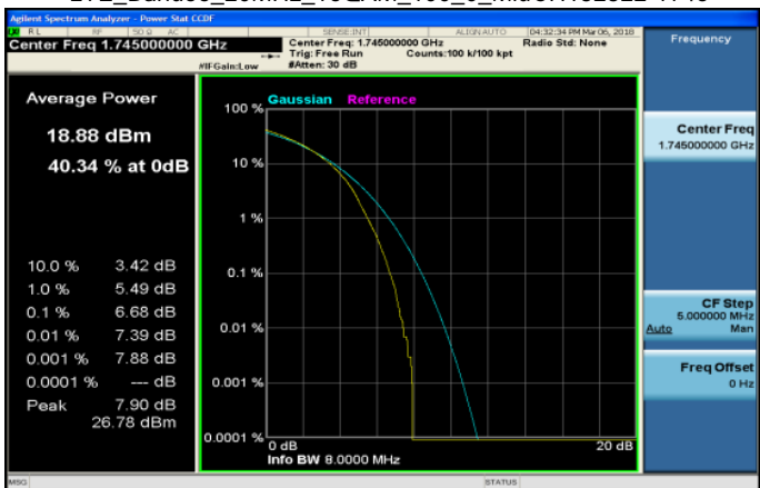
LTE_Band66_20MHz_16QAM_100_0_MidCH132322-1745
