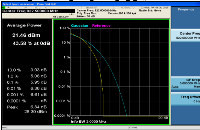
Part 90_LTE_Band26_3MHz_16QAM_15_0_HighCH26775-822.5
