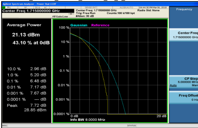
LTE_Band66_10MHz_16QAM_50_0_LowCH132022-1715
