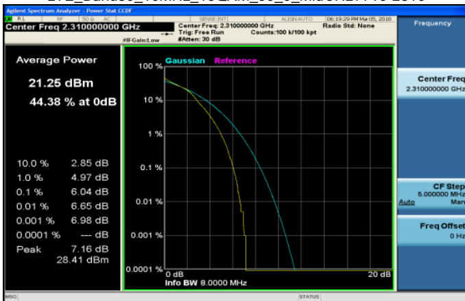
LTE_Band30_10MHz_16QAM_50_0_MidCH27710-2310
