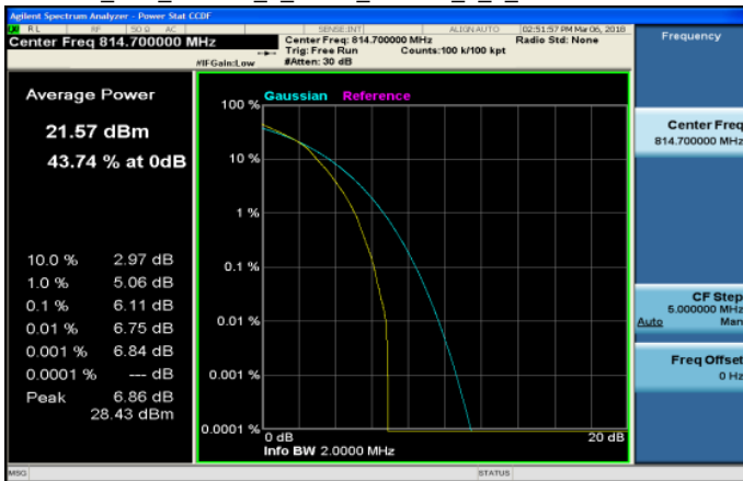
Part 90_LTE_Band26_1_4MHz_16QAM_6_0_LowCH26697-814.7
