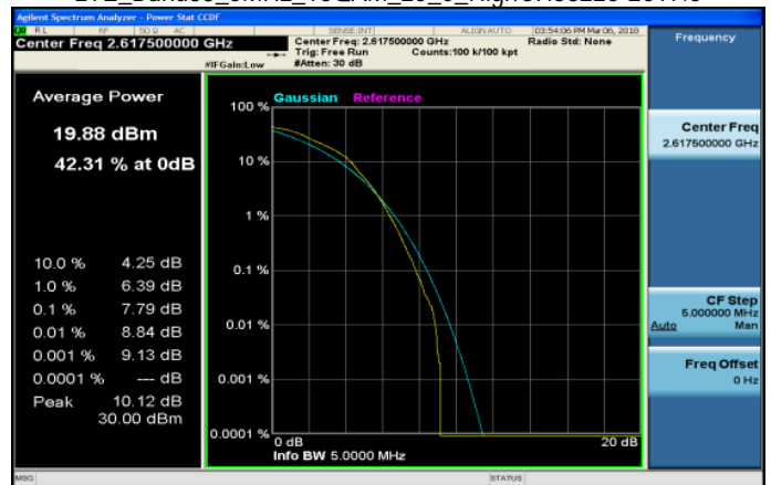
LTE_Band38_5MHz_16QAM_25_0_HighCH38225-2617.5
