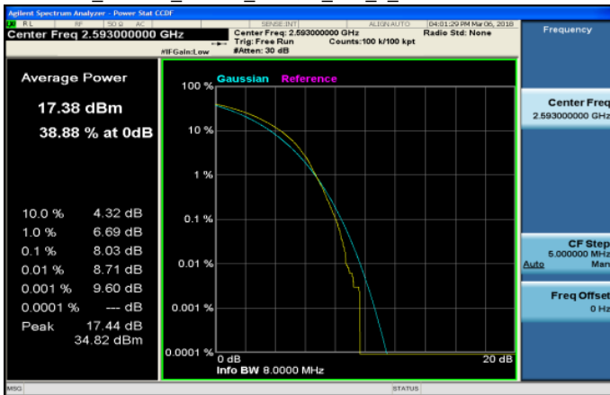
LTE_Band41_20MHz_16QAM_100_0_MidCH40620-2593
