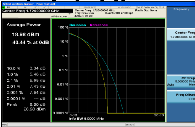
LTE_Band66_20MHz_16QAM_100_0_LowCH132072-1720
