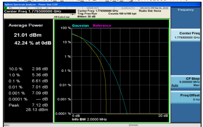
LTE_Band66_1_4MHz_16QAM_6_0_HighCH132665-1779.3
