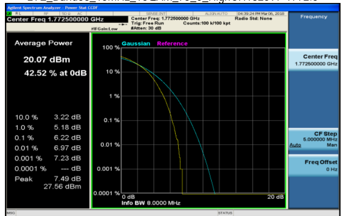
LTE_Band66_15MHz_16QAM_75_0_HighCH132597-1772.5
