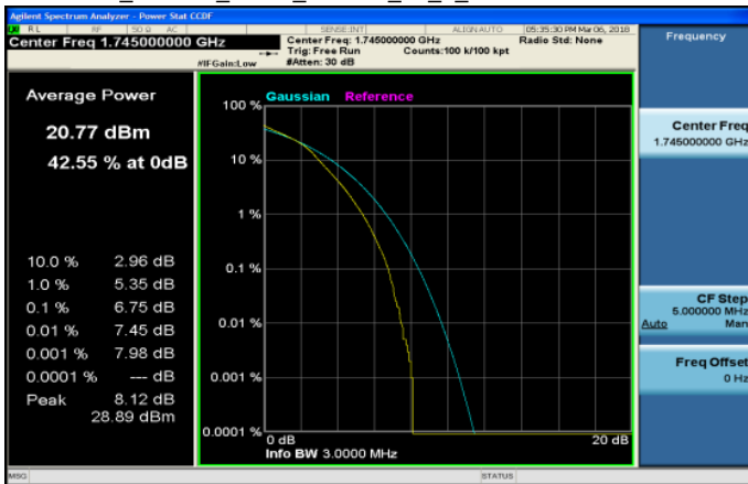
LTE_Band66_3MHz_16QAM_15_0_MidCH132322-1745
