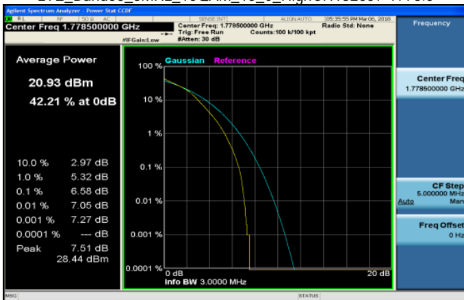
LTE_Band66_3MHz_16QAM_15_0_HighCH132657-1778.5
