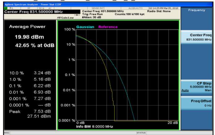
LTE_Band26_15MHz_16QAM_75_0_LowCH26865-831.5
