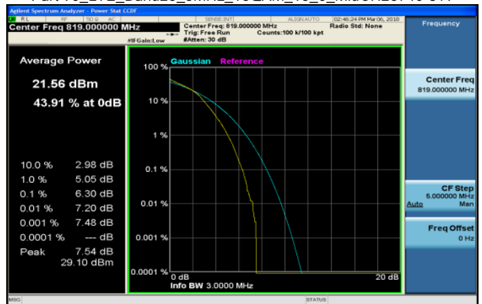
Part 90_LTE_Band26_3MHz_16QAM_15_0_MidCH26740-819
