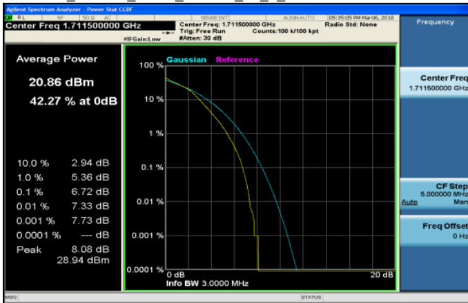
LTE_Band66_3MHz_16QAM_15_0_LowCH131987-1711.5
