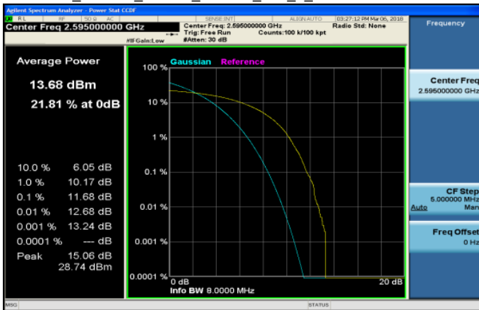
LTE_Band38_20MHz_16QAM_100_0_MidCH38000-2595
