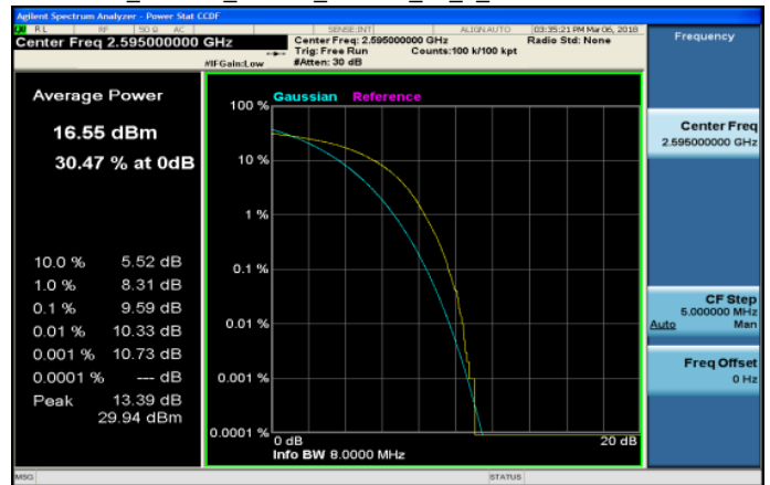
LTE_Band38_15MHz_16QAM_75_0_MidCH38000-2595
