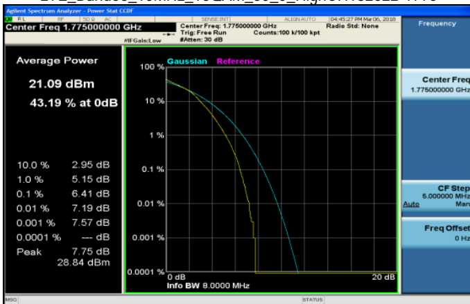
LTE_Band66_10MHz_16QAM_50_0_HighCH132622-1775
