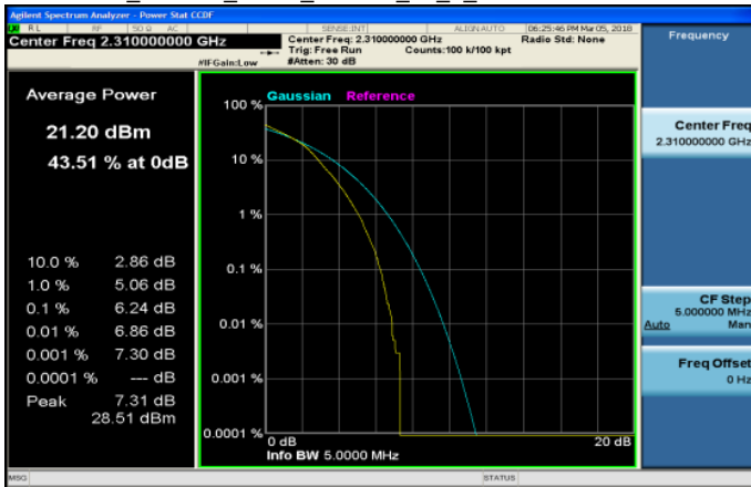
LTE_Band30_5MHz_16QAM_25_0_MidCH27710-2310
