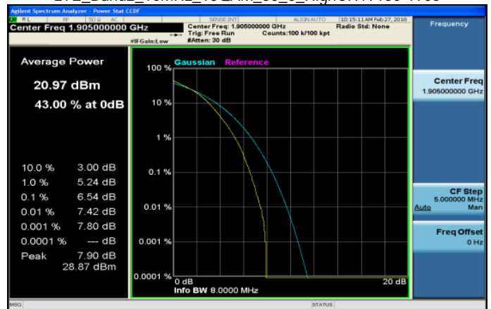
LTE_Band2_10MHz_16QAM_50_0_HighCH19150-1905
