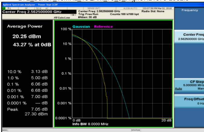
LTE_Band7_15MHz_16QAM_75_0_HighCH21375-2562.5
