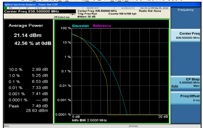
LTE_Band26_1_4MHz_16QAM_6_0_MidCH26915-836.5
