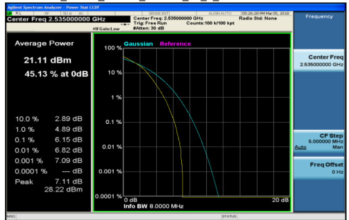
LTE_Band7_10MHz_16QAM_50_0_MidCH21100-2535
