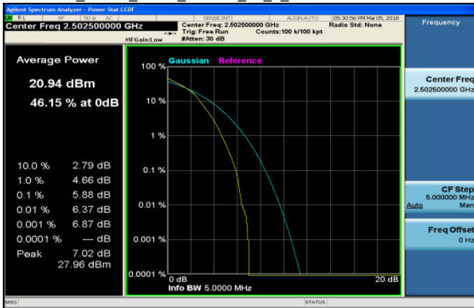
LTE_Band7_5MHz_16QAM_25_0_LowCH20775-2502.5
