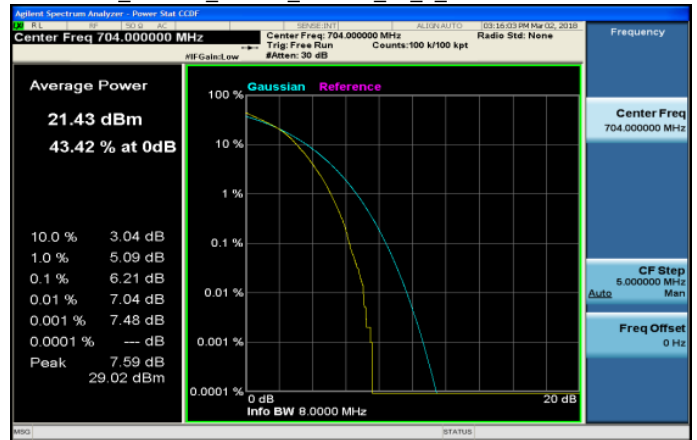
LTE_Band12_10MHz_16QAM_50_0_LowCH23060-704
