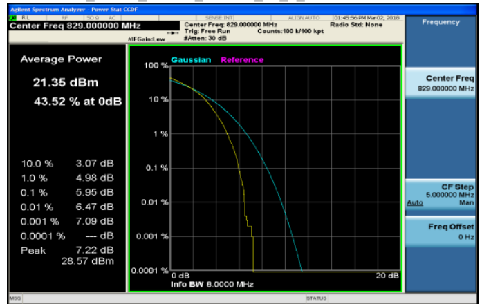
LTE_Band5_10MHz_16QAM_50_0_LowCH20450-829
