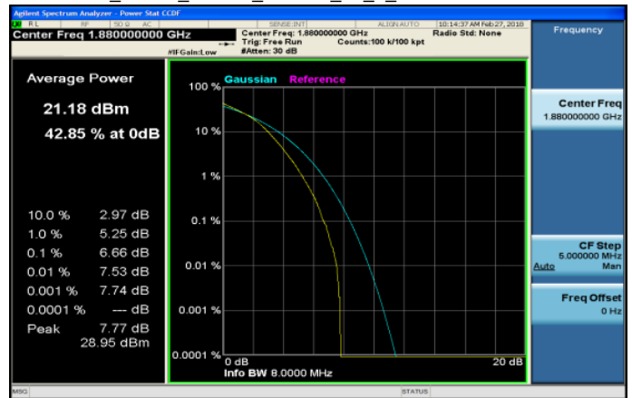
LTE_Band2_10MHz_16QAM_50_0_MidCH18900-1880
