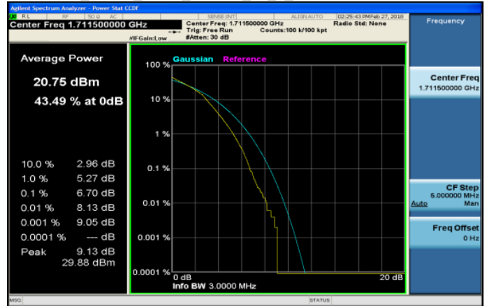
LTE_Band4_3MHz_16QAM_15_0_LowCH19965-1711.5
