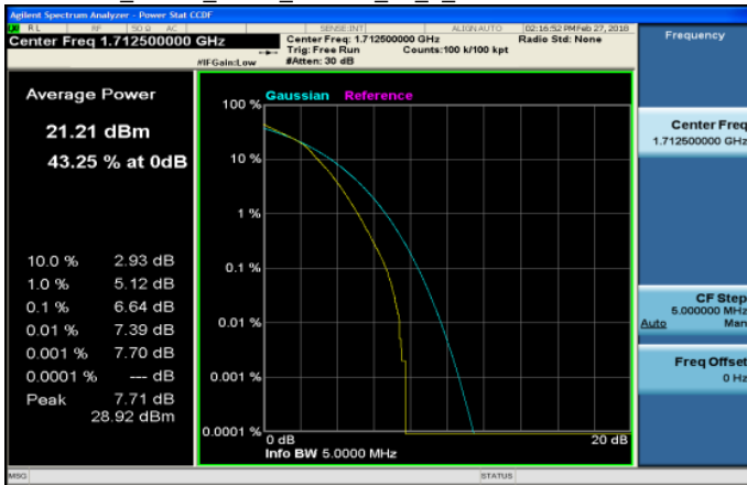
LTE_Band4_5MHz_16QAM_25_0_LowCH19975-1712.5
