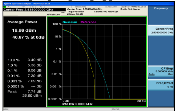
LTE_Band7_20MHz_16QAM_100_0_MidCH21100-2535
