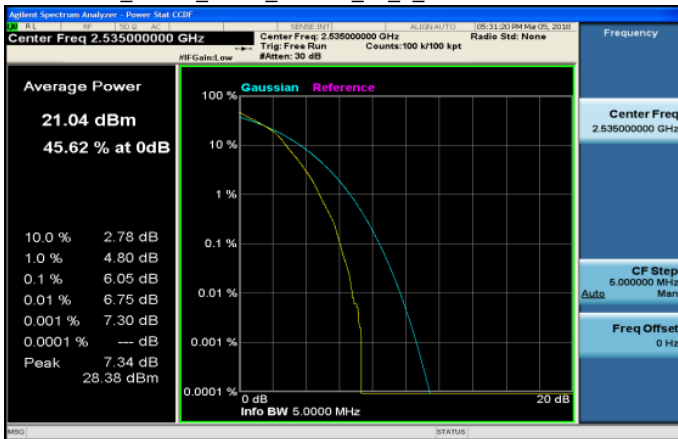
LTE_Band7_5MHz_16QAM_25_0_MidCH21100-2535
