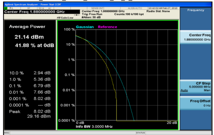
LTE_Band2_3MHz_16QAM_15_0_MidCH18900-1880
