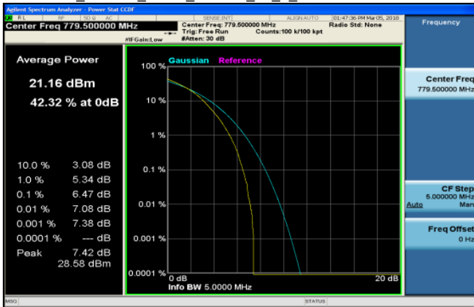
LTE_Band13_5MHz_16QAM_25_0_LowCH23205-779.5
