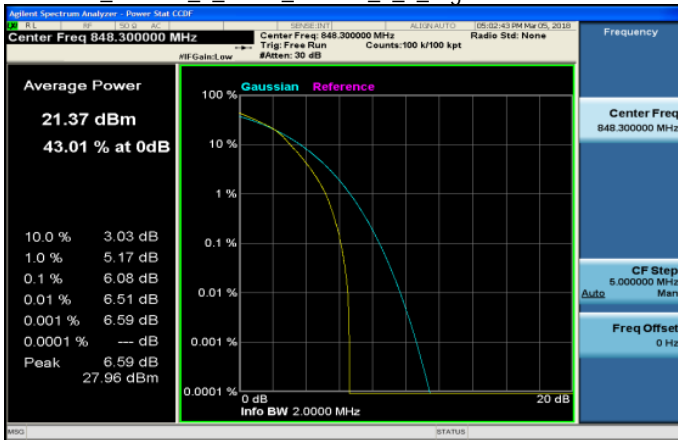
LTE_Band26_1_4MHz_16QAM_6_0_HighCH27033-848.3
