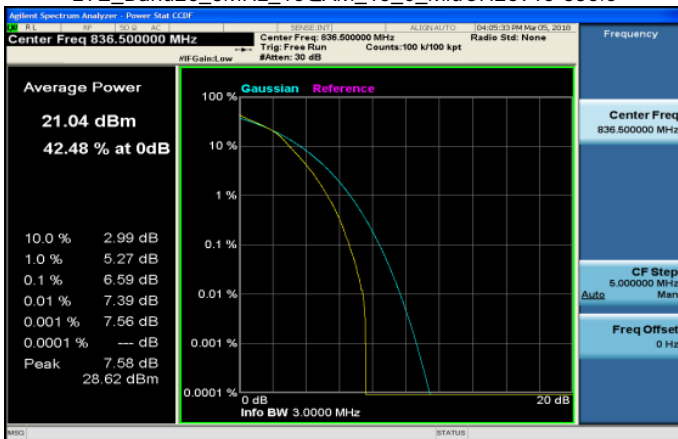
LTE_Band26_3MHz_16QAM_15_0_MidCH26915-836.5
