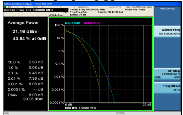
LTE_Band12_3MHz_16QAM_15_0_MidCH23095-707.5
