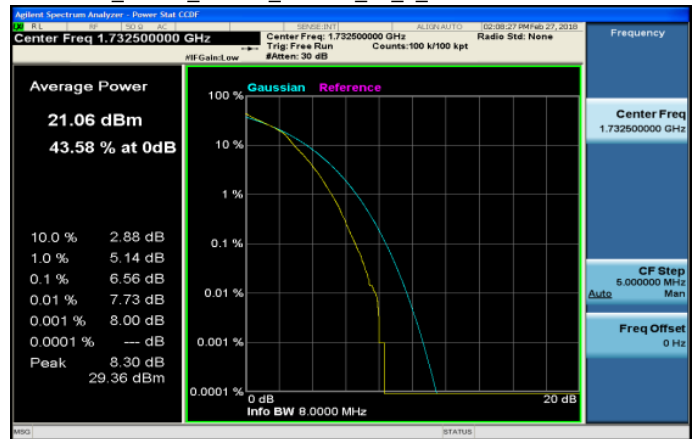
LTE_Band4_10MHz_16QAM_50_0_MidCH20175-1732.5
