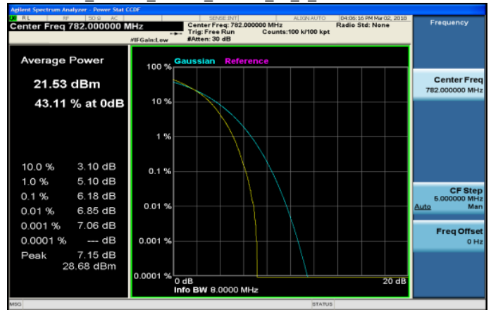
LTE_Band13_10MHz_16QAM_50_0_MidCH23230-782
