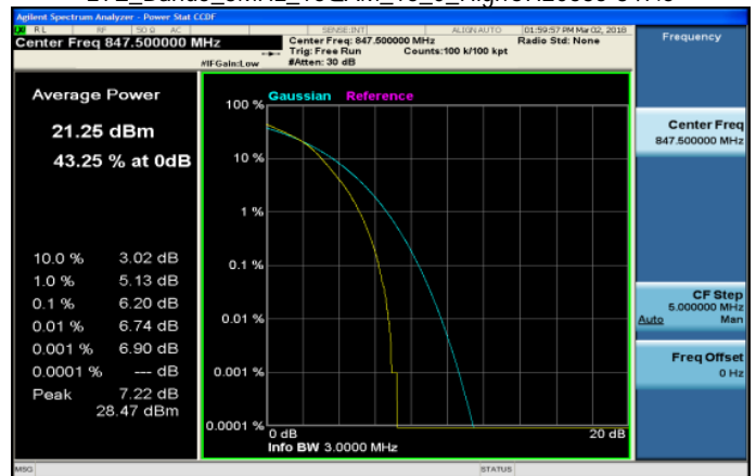
LTE_Band5_3MHz_16QAM_15_0_HighCH20635-847.5
