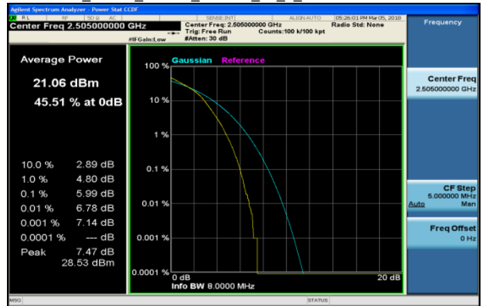
LTE_Band7_10MHz_16QAM_50_0_LowCH20800-2505
