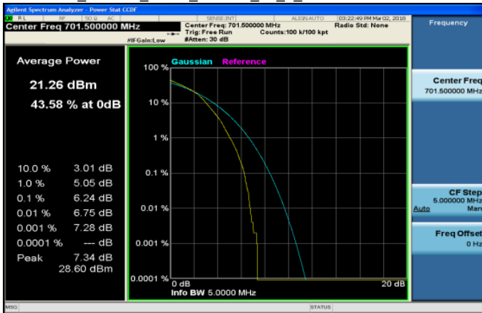
LTE_Band12_5MHz_16QAM_25_0_LowCH23035-701.5
