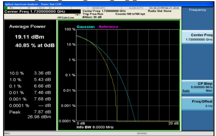
LTE_Band4_20MHz_16QAM_100_0_LowCH20050-1720
