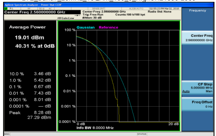
LTE_Band7_20MHz_16QAM_100_0_HighCH21350-2560
