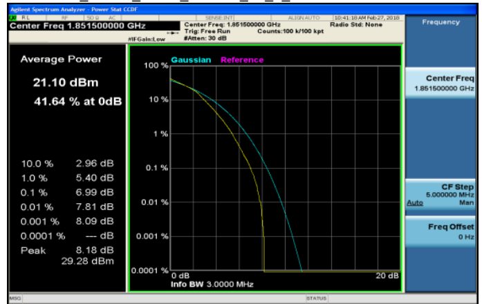
LTE_Band2_3MHz_16QAM_15_0_LowCH18615-1851.5
