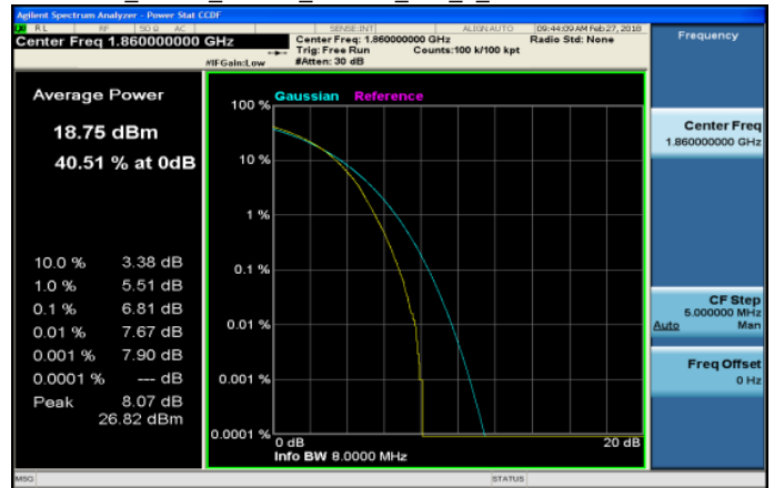
LTE_Band2_20MHz_16QAM_100_0_LowCH18700-1860
