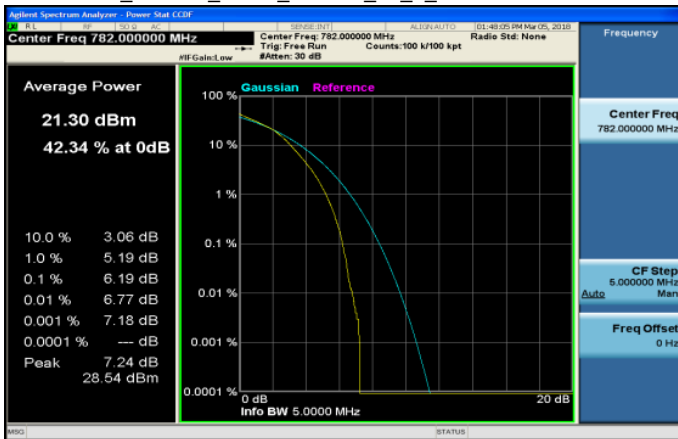
LTE_Band13_5MHz_16QAM_25_0_MidCH23230-782
