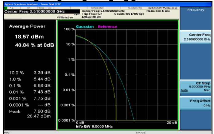
LTE_Band7_20MHz_16QAM_100_0_LowCH20850-2510
