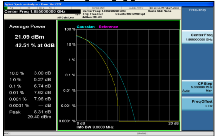
LTE_Band2_10MHz_16QAM_50_0_LowCH18650-1855
