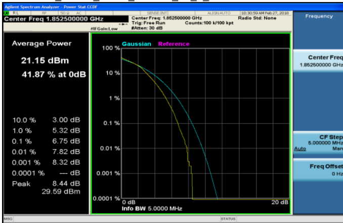
LTE_Band2_5MHz_16QAM_25_0_LowCH18625-1852.5
