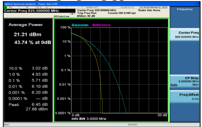
LTE_Band5_3MHz_16QAM_15_0_LowCH20415-825.5
