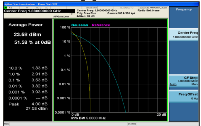
WCDMA_B2_MidCH9400-1880
