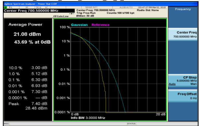
LTE_Band12_3MHz_16QAM_15_0_LowCH23025-700.5
