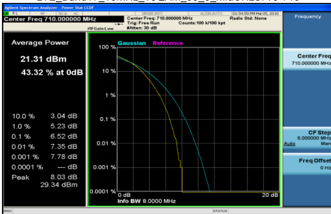
LTE_Band17_10MHz_16QAM_50_0_MidCH23790-710
