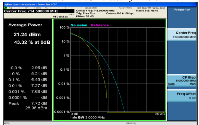
LTE_Band12_3MHz_16QAM_15_0_HighCH23165-714.5
