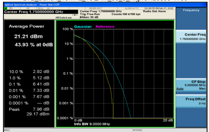
LTE_Band4_10MHz_16QAM_50_0_HighCH20350-1750
