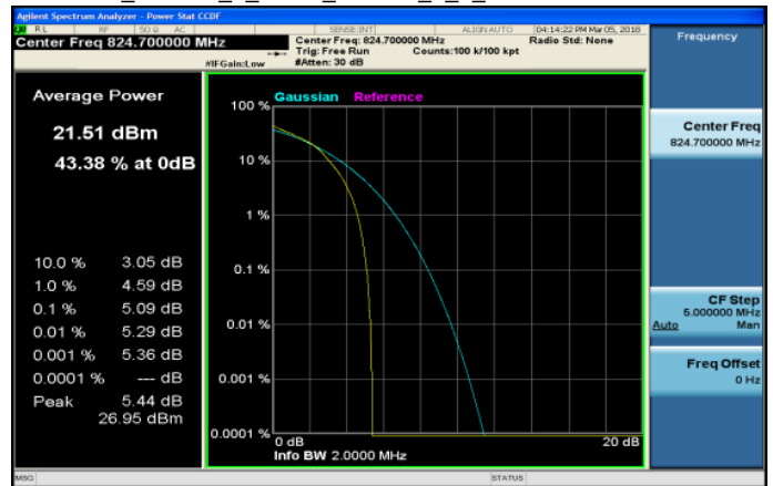
LTE_Band26_1_4MHz_16QAM_6_0_LowCH26797-824.7
