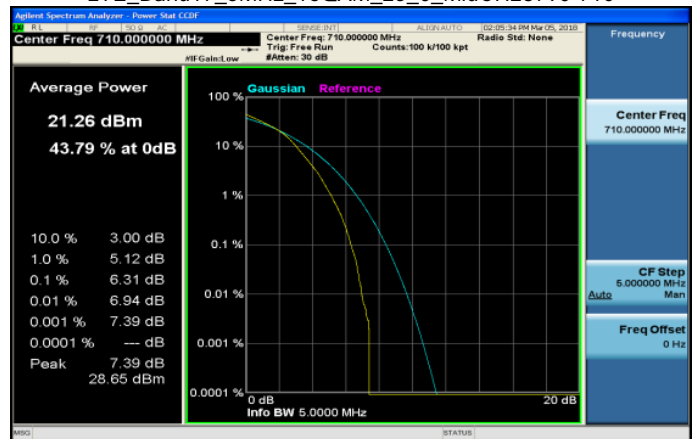
LTE_Band17_5MHz_16QAM_25_0_MidCH23790-710
