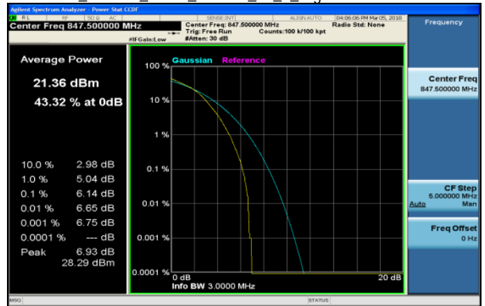
LTE_Band26_3MHz_16QAM_15_0_HighCH27025-847.5
