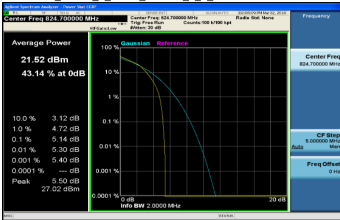
LTE_Band5_1_4MHz_16QAM_6_0_LowCH20407-824.7
