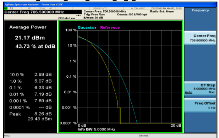
LTE_Band17_5MHz_16QAM_25_0_LowCH23755-706.5
