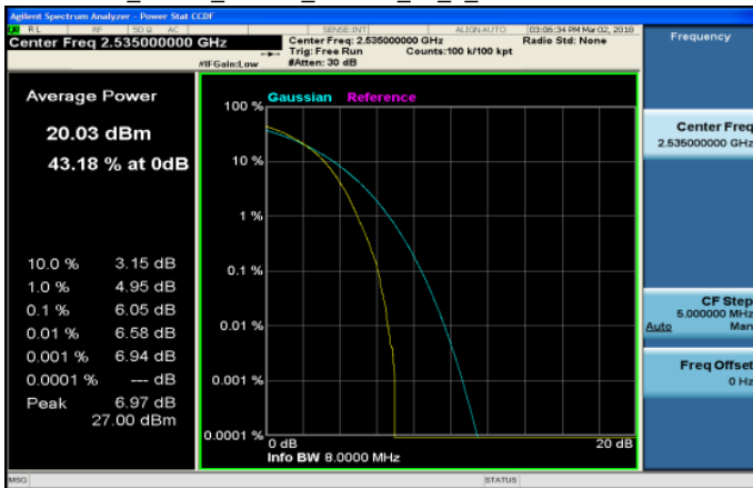
LTE_Band7_15MHz_16QAM_75_0_MidCH21100-2535
