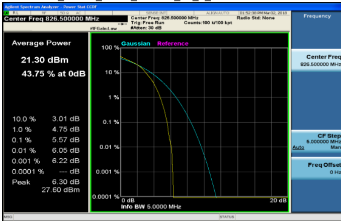
LTE_Band5_5MHz_16QAM_25_0_LowCH20425-826.5
