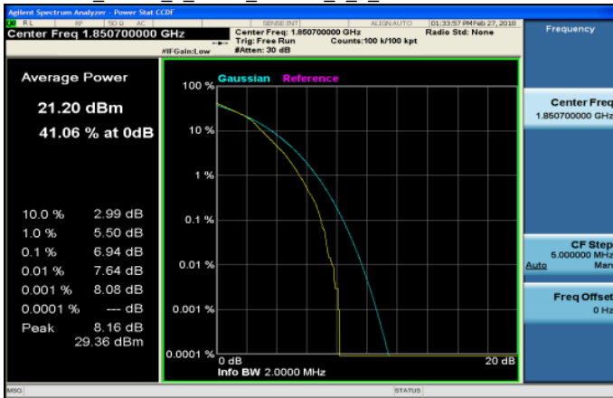
LTE_Band2_1_4MHz_16QAM_6_0_LowCH18607-1850.7
