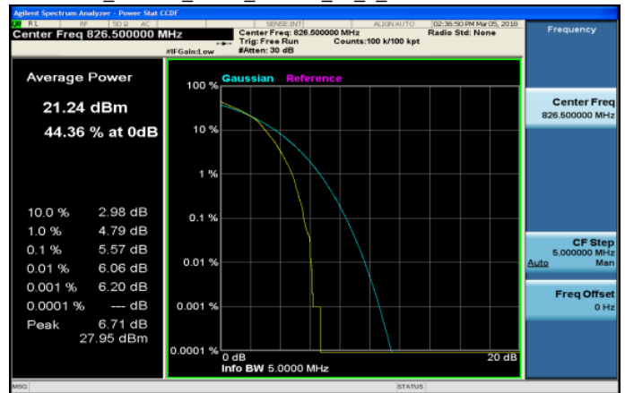
LTE_Band26_5MHz_16QAM_25_0_LowCH26815-826.5
