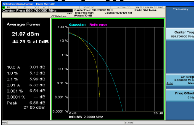
LTE_Band12_1_4MHz_16QAM_6_0_LowCH23017-699.7
