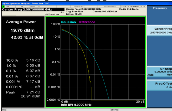
LTE_Band7_15MHz_16QAM_75_0_LowCH20825-2507.5
