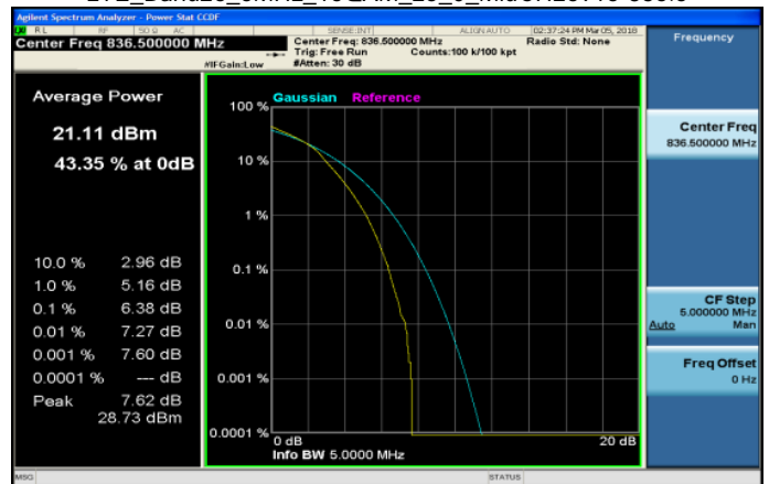
LTE_Band26_5MHz_16QAM_25_0_MidCH26915-836.5
