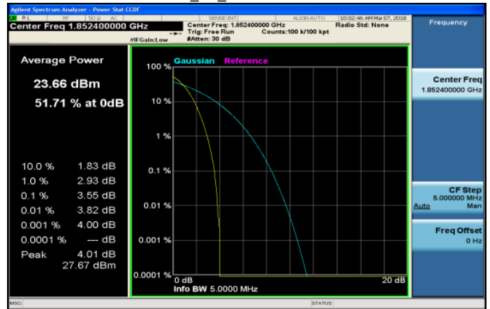
WCDMA_B2_LowCH9262-1852.4
