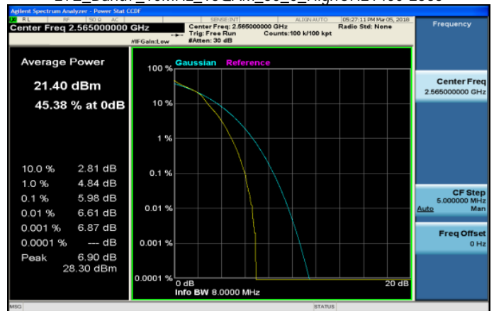
LTE_Band7_10MHz_16QAM_50_0_HighCH21400-2565
