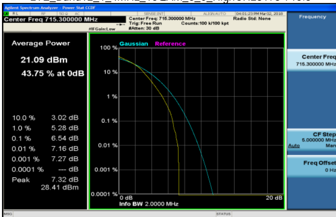
LTE_Band12_1_4MHz_16QAM_6_0_HighCH23173-715.3
