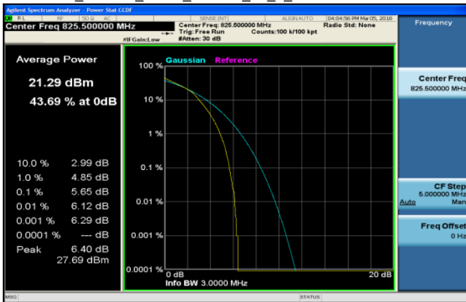
LTE_Band26_3MHz_16QAM_15_0_LowCH26805-825.5
