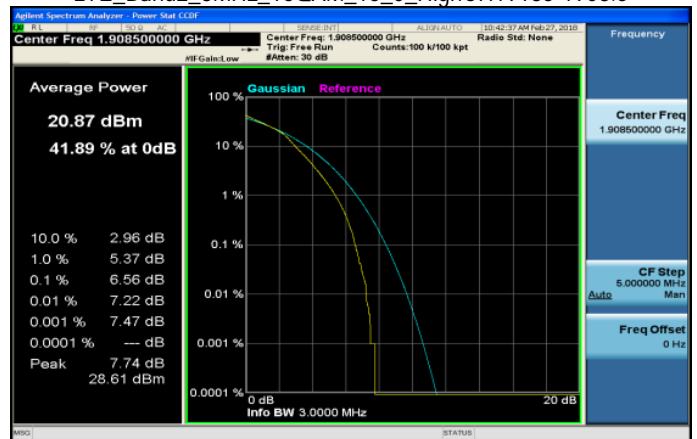
LTE_Band2_3MHz_16QAM_15_0_HighCH19185-1908.5
