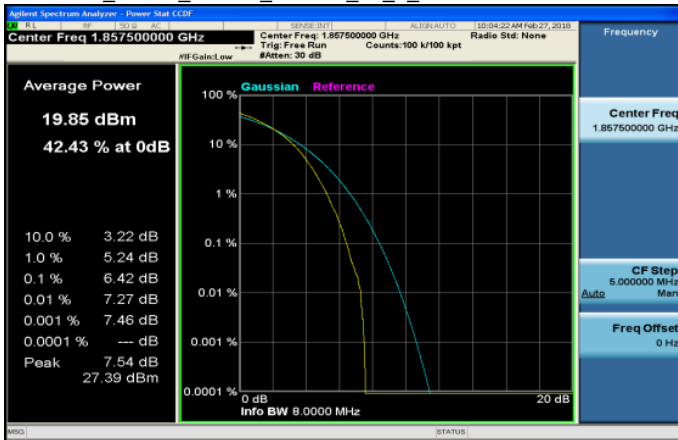
LTE_Band2_15MHz_16QAM_75_0_LowCH18675-1857.5
