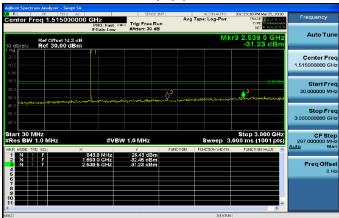
30MHz~3GHz_Band26_5MHz_QPSK_1_0_HighCH27015-846.5
