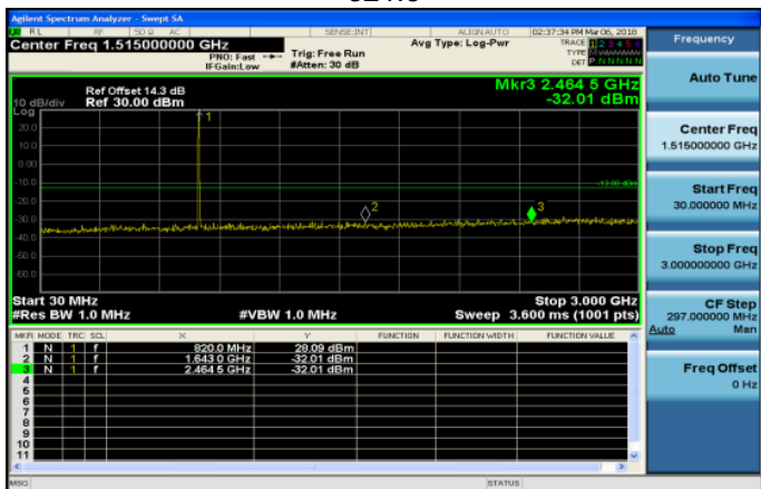
30MHz~3GHz_Band26_5MHz_QPSK_1_0_HighCH26765-821.5
