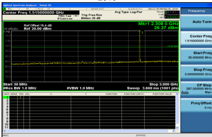
30MHz~3GHz_Band30_5MHz_QPSK_1_0_MidCH27710-2310
