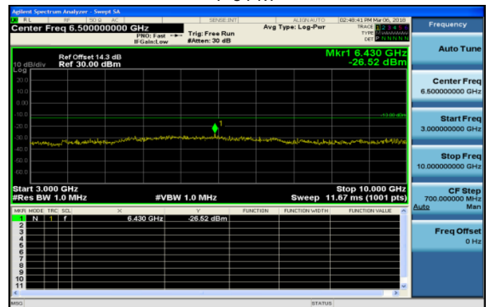
3GHz~10GHz_Band26_1_4MHz_QPSK_1_0_LowCH2669 7-814.7
