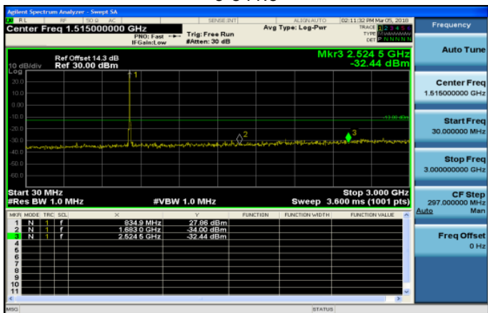
30MHz~3GHz_Band26_15MHz_QPSK_1_0_HighCH2696 5-841.5
