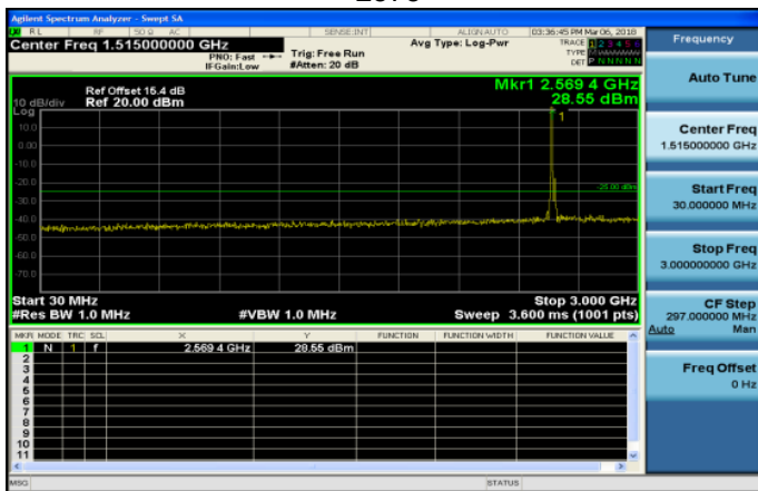
30MHz~3GHz_Band38_10MHz_QPSK_1_0_LowCH37800-2575
