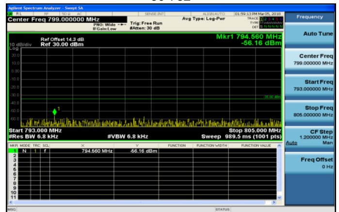
793MHz~805MHz_Band13_5MHz_QPSK_1_0_MidCH23230-782
