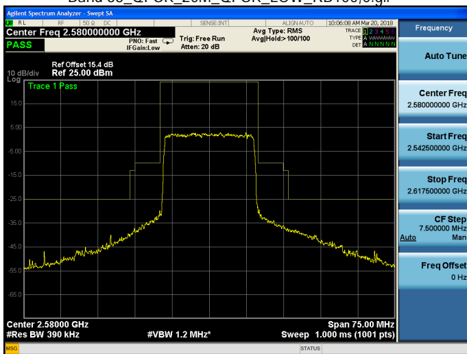
Band 38_QPSK_20M_QPSK_LOW_RB100,0.gif
