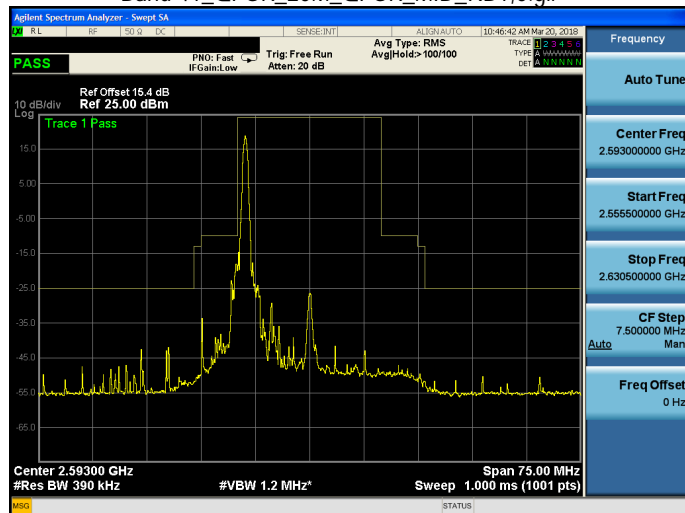
Band 41_QPSK_20M_QPSK_MID_RB1,99.gif
