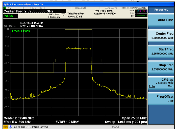
Band 38_QPSK_15M_QPSK_MID_RB75,0.gif
