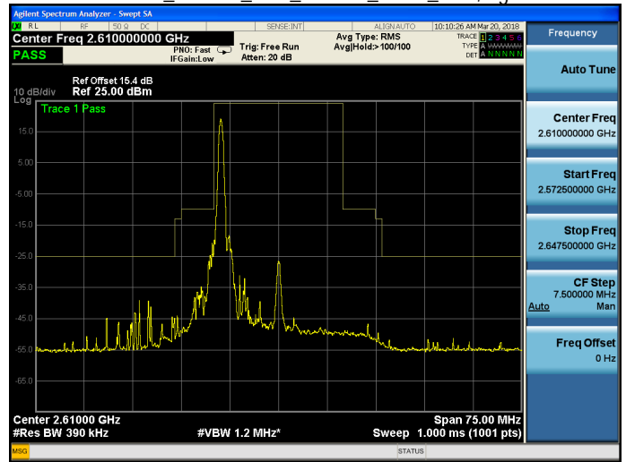
Band 38_16QAM_20M_16QAM_HIGH_RB1,99.gif
