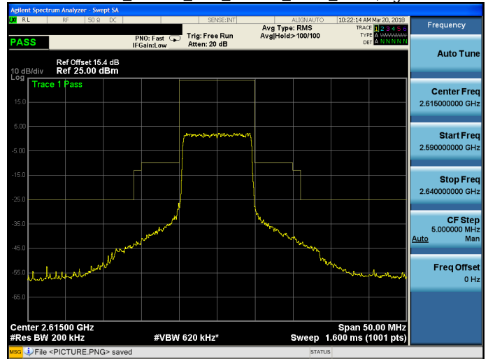
Band 38_16QAM_10M_16QAM_HIGH_RB50,0.gif
