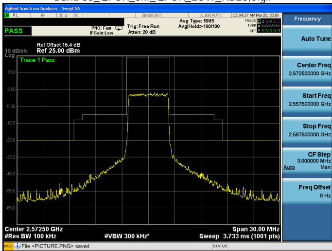
Band 38_QPSK_5M_QPSK_LOW_RB25,0.gif
