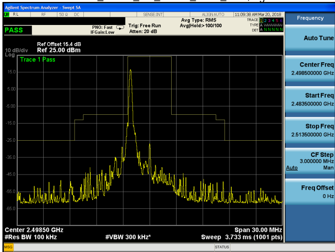
Band 41_QPSK_5M_QPSK_LOW_RB1,24.gif
