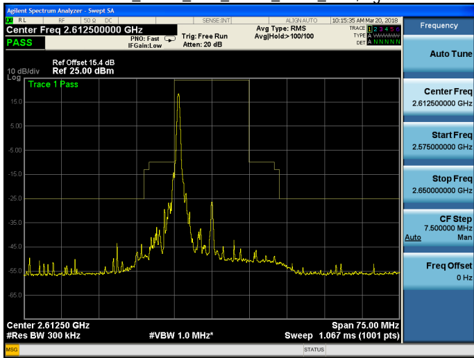
Band 38_QPSK_15M_QPSK_HIGH_RB1,74.qif
