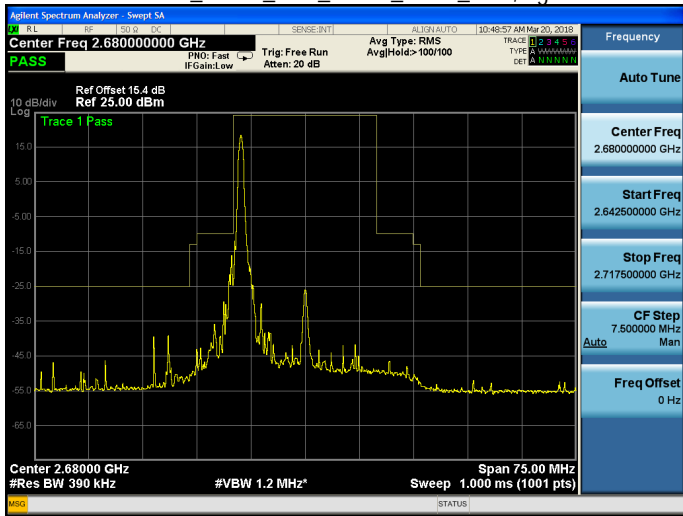
Band 41_QPSK_20M_QPSK_HIGH_RB1,99.gif
