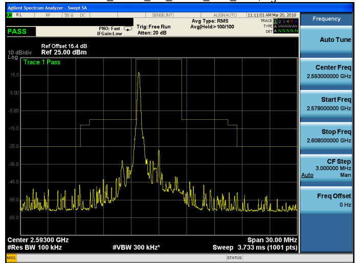
Band 41_QPSK_5M_QPSK_MID_RB1,24.gif
