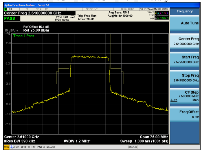
Band 38_16QAM_20M_16QAM_HIGH_RB100,0.gif
