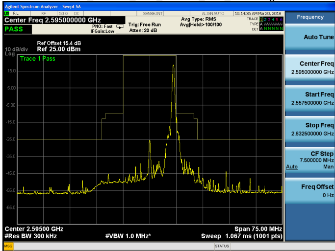
Band 38_16QAM_15M_16QAM_MID_RB75,0.gif
