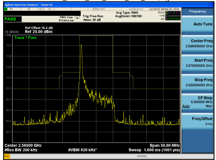
Band 38_QPSK_10M_QPSK_MID_RB1,49.gif
