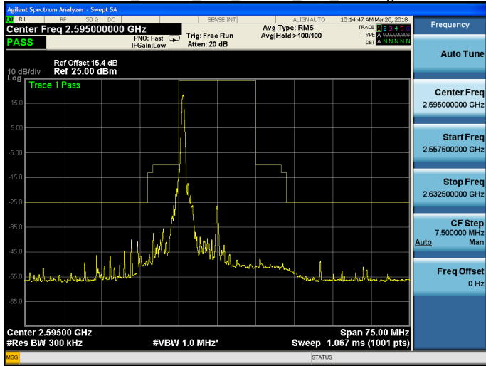
Band 38_16QAM_15M_16QAM_MID_RB1,74.gif
