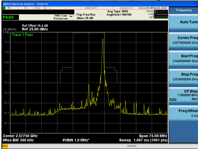
Band 38_QPSK_15M_QPSK_LOW_RB75,0.gif
