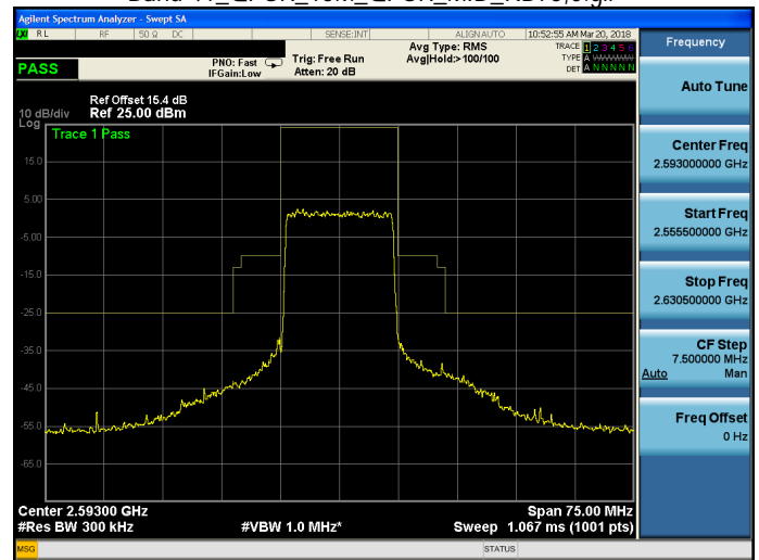
Band 41_QPSK_15M_QPSK_MID_RB75,0.gif
