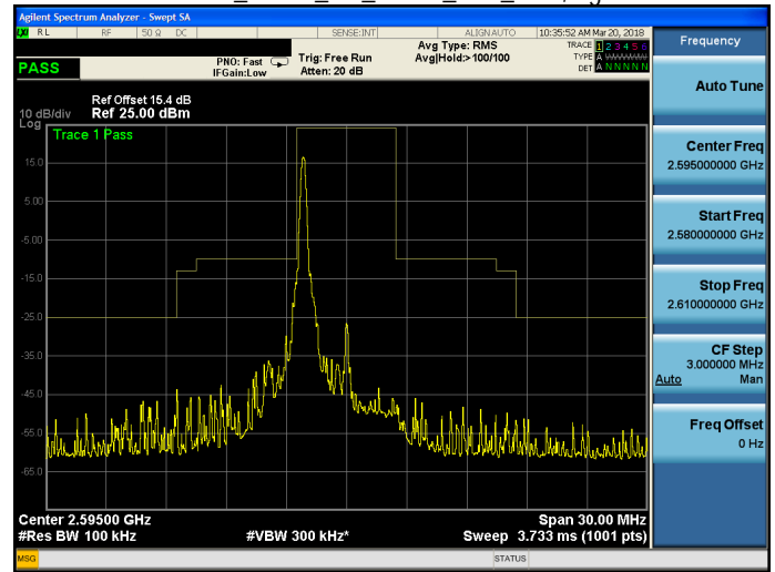
Band 38_QPSK_5M_QPSK_MID_RB1,24.gif
