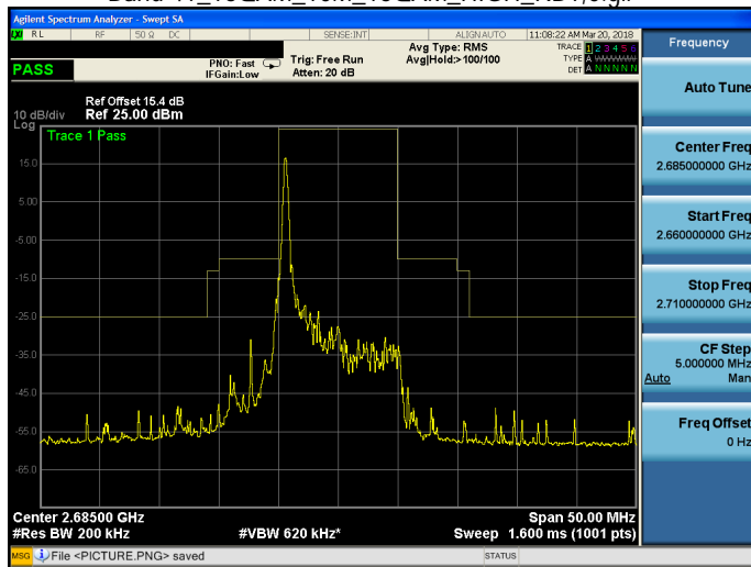
Band 41_16QAM_10M_16QAM_HIGH_RB1,49.gif
