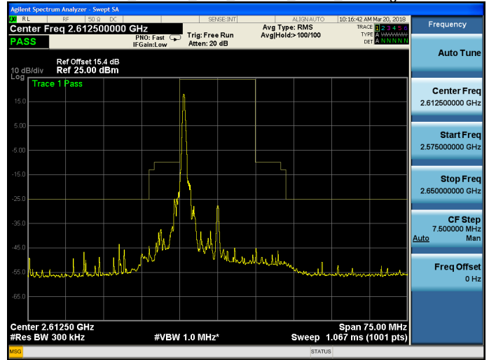
Band 38_16QAM_15M_16QAM_HIGH_RB1,74.gif
