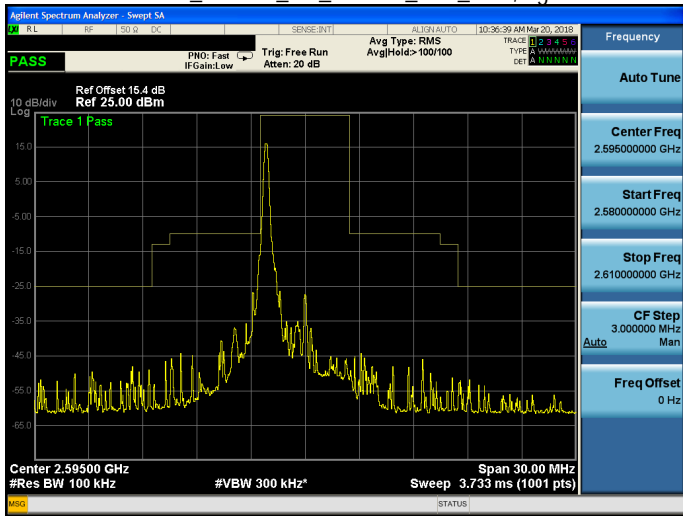
Band 38_16QAM_5M_16QAM_MID_RB1,24.gif
