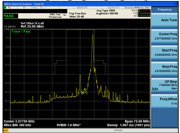
Band 38_16QAM_15M_16QAM_LOW_RB75,0.qif
