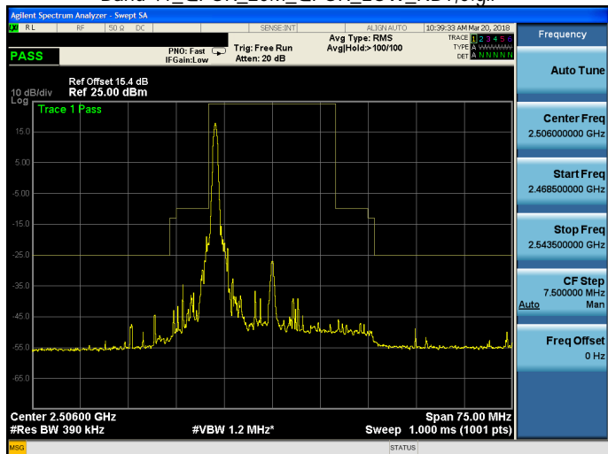
Band 41_QPSK_20M_QPSK_LOW_RB1,99.gif
