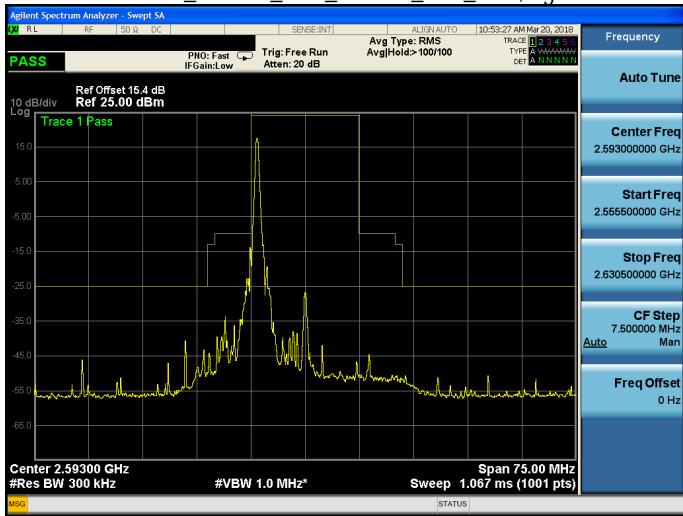
Band 41_16QAM_15M_16QAM_MID_RB1,74.gif
