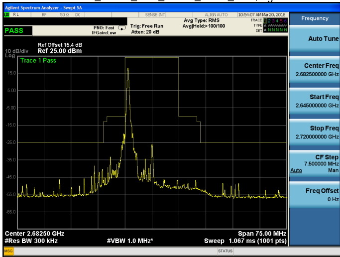
Band 41_QPSK_15M_QPSK_HIGH_RB1,74.qif
