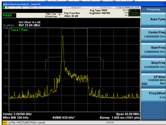
Band 41_16QAM_10M_16QAM_MID_RB1,49.gif
