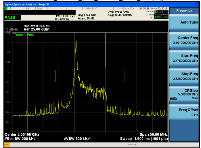
Band 41_16QAM_10M_16QAM_LOW_RB1,49.gif
