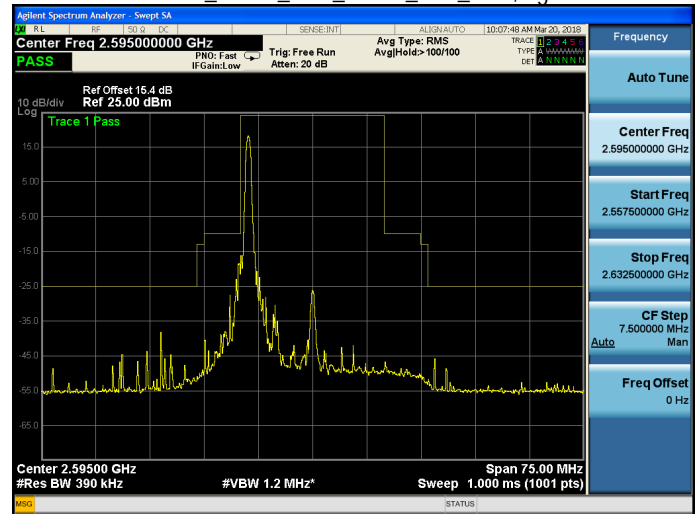
Band 38_QPSK_20M_QPSK_MID_RB1,99.gif
