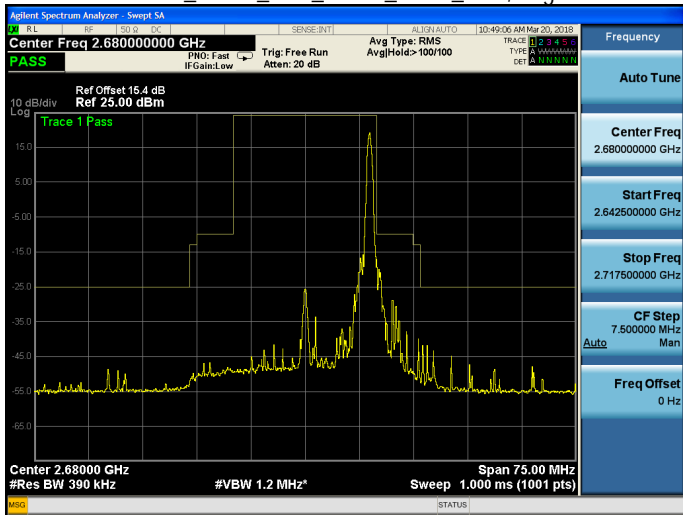
Band 41_QPSK_20M_QPSK_HIGH_RB100,0.gif
