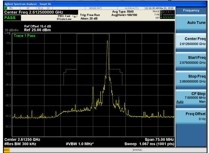
Band 38_16QAM_15M_16QAM_HIGH_RB75,0.gif
