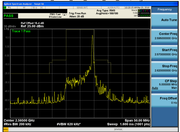
Band 38_QPSK_10M_QPSK_MID_RB50,0.gif
