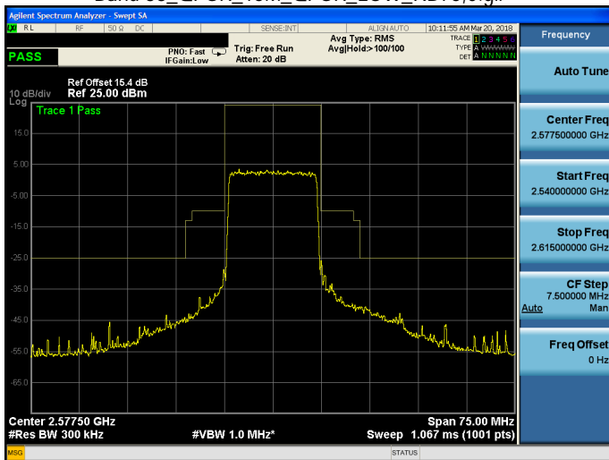
Band 38_QPSK_15M_QPSK_LOW_RB75,0.gif
