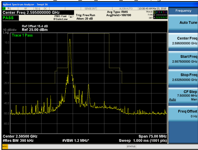
Band 38_16QAM_20M_16QAM_MID_RB1,99.gif
