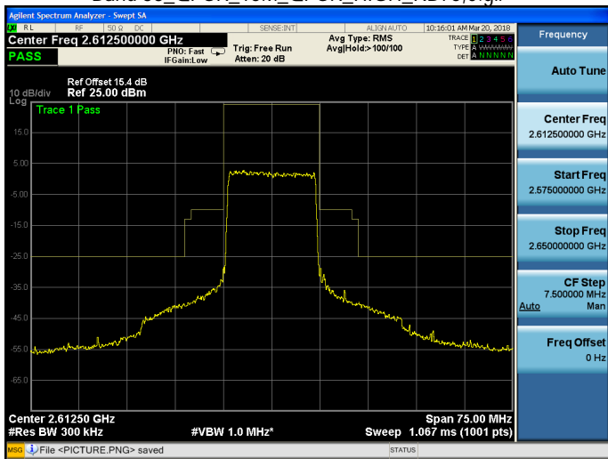
Band 38_QPSK_15M_QPSK_HIGH_RB75,0.qif
