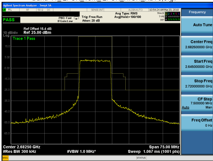
Band 41_QPSK_15M_QPSK_HIGH_RB75,0.qif
