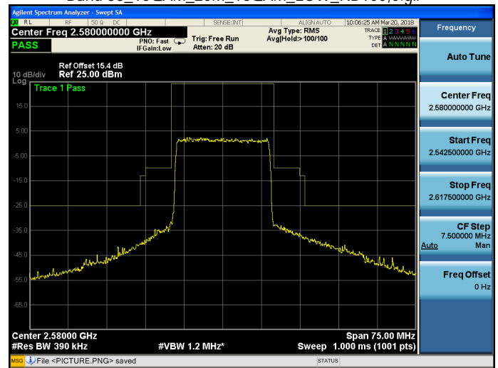
Band 38_16QAM_20M_16QAM_LOW_RB100,0.gif
