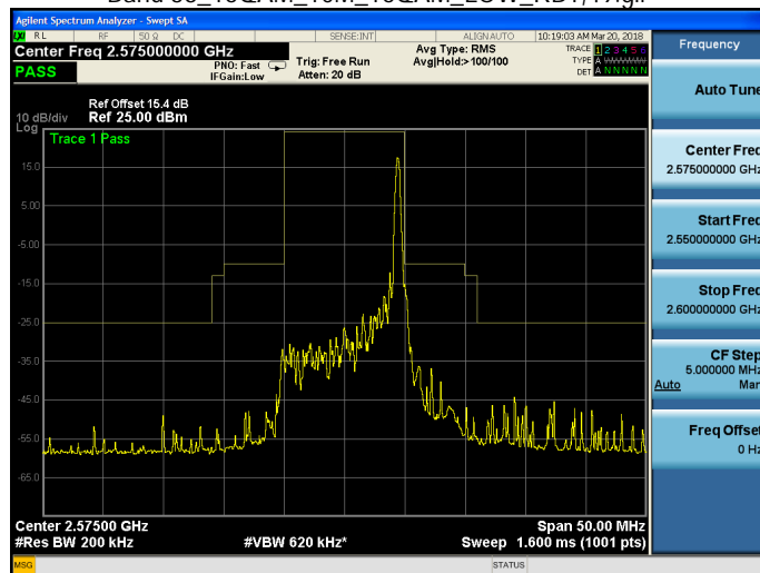
Band 38_16QAM_10M_16QAM_LOW_RB50,0.gif
