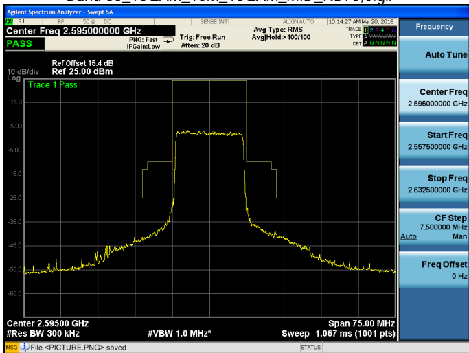
Band 38_16QAM_15M_16QAM_MID_RB75,0.gif
