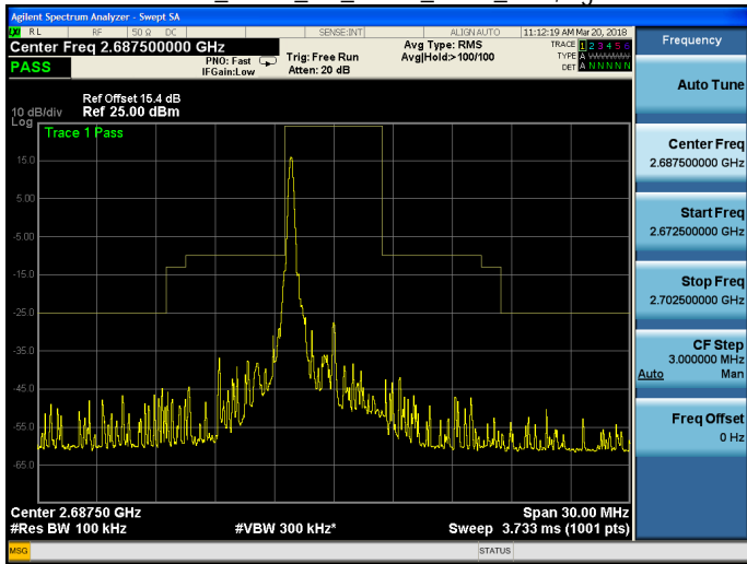
Band 41_QPSK_5M_QPSK_HIGH_RB1,24.gif
