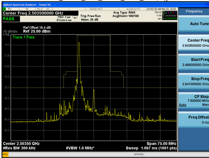
Band 41_QPSK_15M_QPSK_LOW_RB1,74.gif
