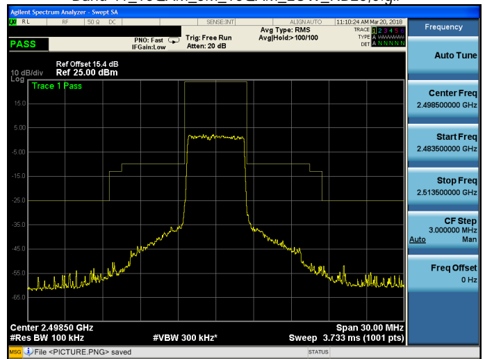
Band 41_16QAM_5M_16QAM_LOW_RB25,0.gif
