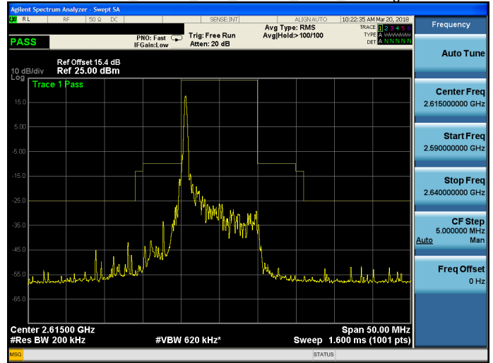
Band 38_16QAM_10M_16QAM_HIGH_RB1,49.gif
