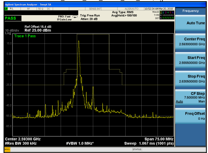
Band 41_QPSK_15M_QPSK_MID_RB1,74.gif
