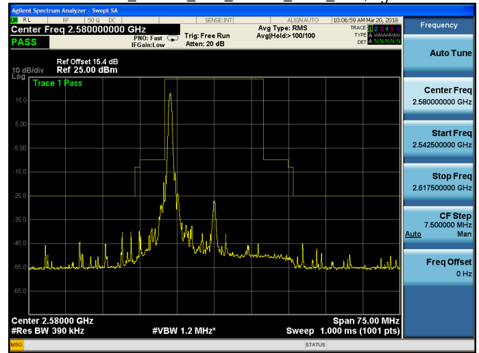
Band 38_16QAM_20M_16QAM_LOW_RB1,99.gif
