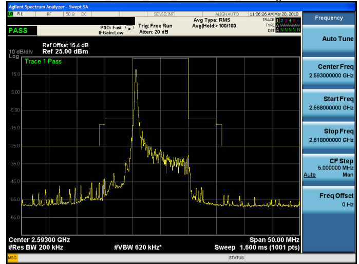
Band 41_QPSK_10M_QPSK_MID_RB1,49.gif
