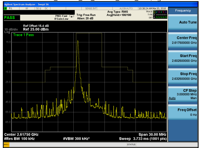
Band 38_16QAM_5M_16QAM_HIGH_RB1,24.gif
