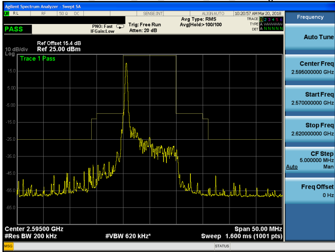
Band 38_16QAM_10M_16QAM_MID_RB1,49.gif
