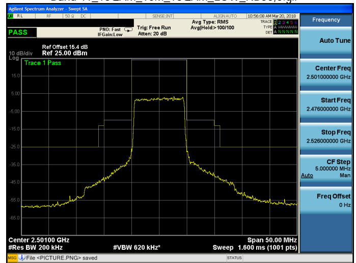
Band 41_16QAM_10M_16QAM_LOW_RB50,0.gif
