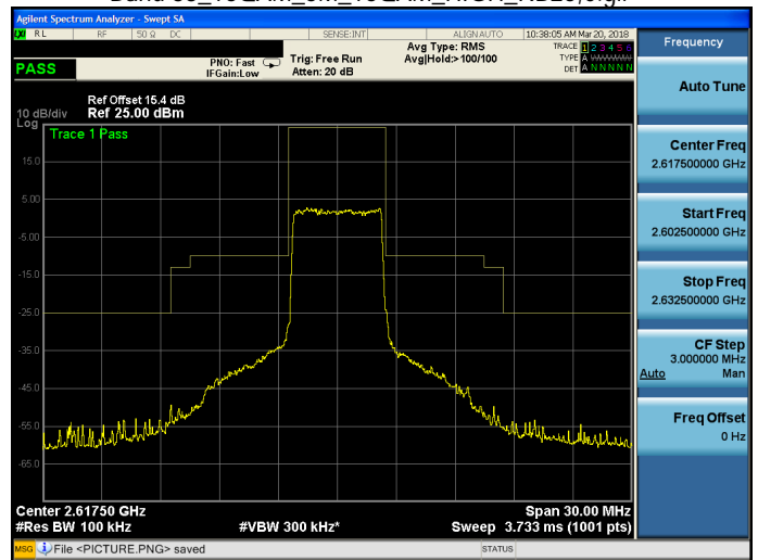
Band 38_16QAM_5M_16QAM_HIGH_RB25,0.gif
