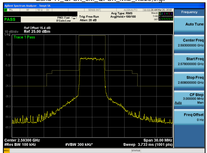
Band 41_QPSK_5M_QPSK_MID_RB25,0.gif
