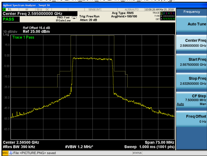
Band 38_16QAM_20M_16QAM_MID_RB100,0.gif
