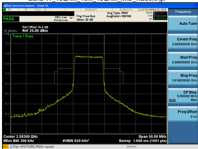
Band 41_16QAM_10M_16QAM_MID_RB50,0.gif
