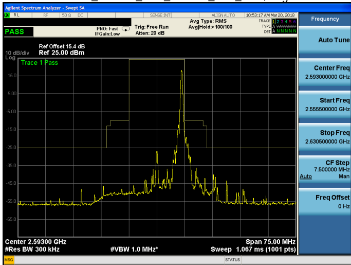
Band 41_16QAM_15M_16QAM_MID_RB75,0.gif
