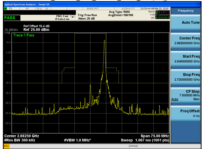
Band 41_16QAM_15M_16QAM_HIGH_RB75,0.gif
