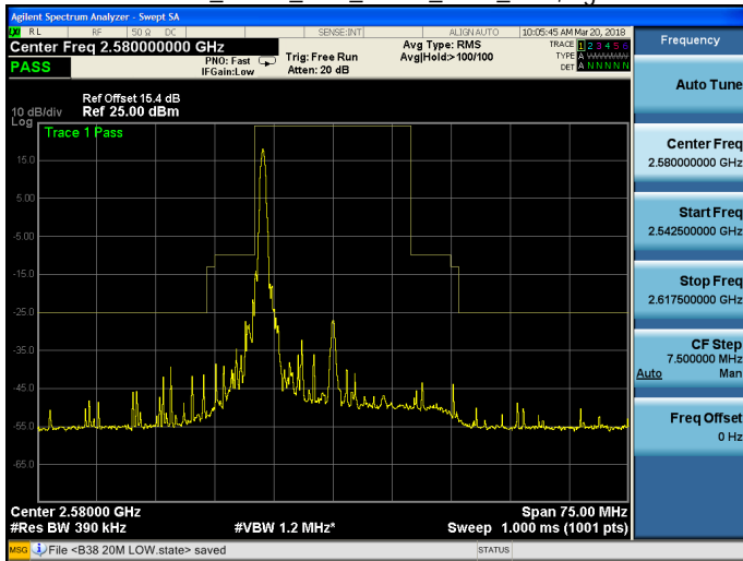
Band 38_QPSK_20M_QPSK_LOW_RB1,99.gif
