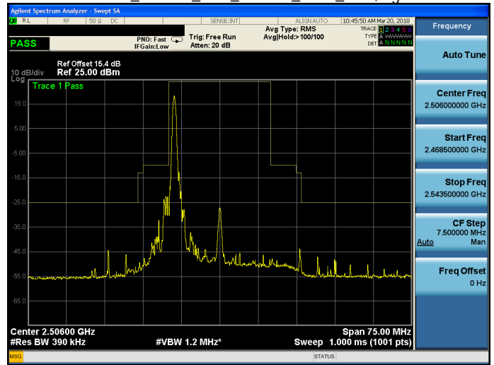
Band 41_16QAM_20M_16QAM_LOW_RB1,99.gif
