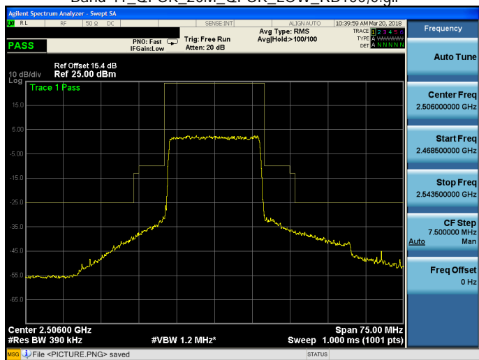
Band 41_QPSK_20M_QPSK_LOW_RB100,0.gif
