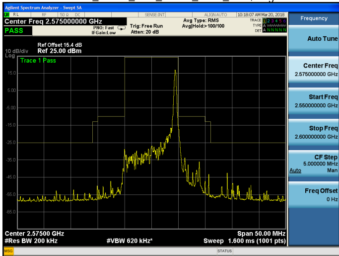
Band 38_QPSK_10M_QPSK_LOW_RB50,0.gif
