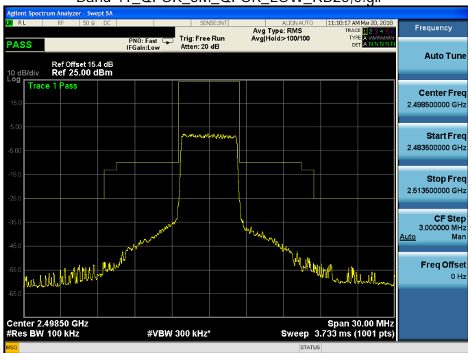
Band 41_QPSK_5M_QPSK_LOW_RB25,0.gif
