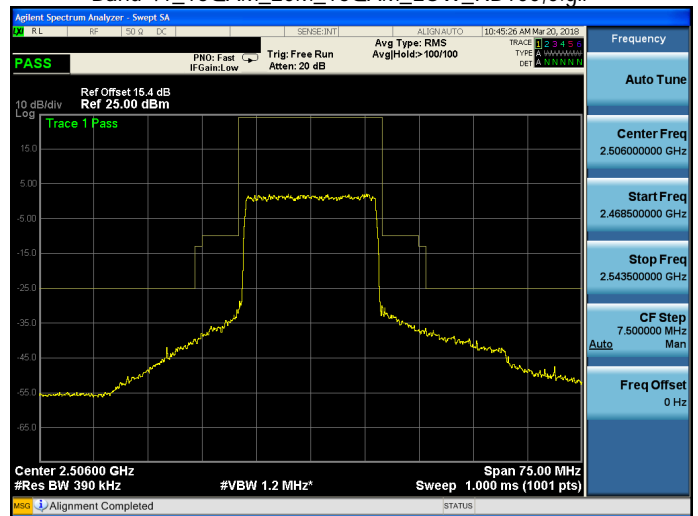
Band 41_16QAM_20M_16QAM_LOW_RB100,0.gif
