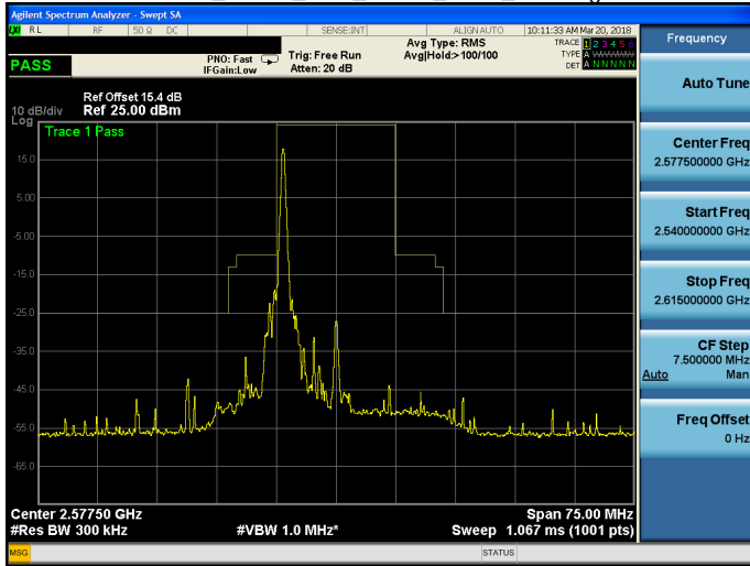
Band 38_QPSK_15M_QPSK_LOW_RB1,74.gif
