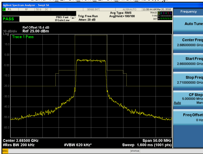
Band 41_QPSK_10M_QPSK_HIGH_RB50,0.gif
