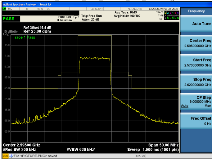
Band 38_16QAM_10M_16QAM_MID_RB50,0.gif
