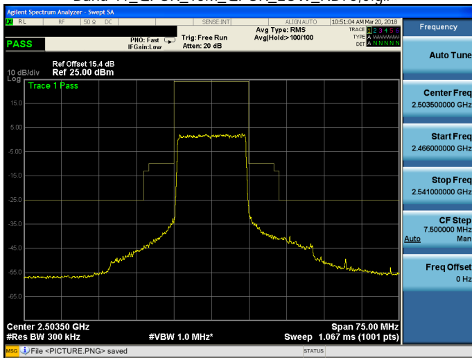
Band 41_QPSK_15M_QPSK_LOW_RB75,0.gif
