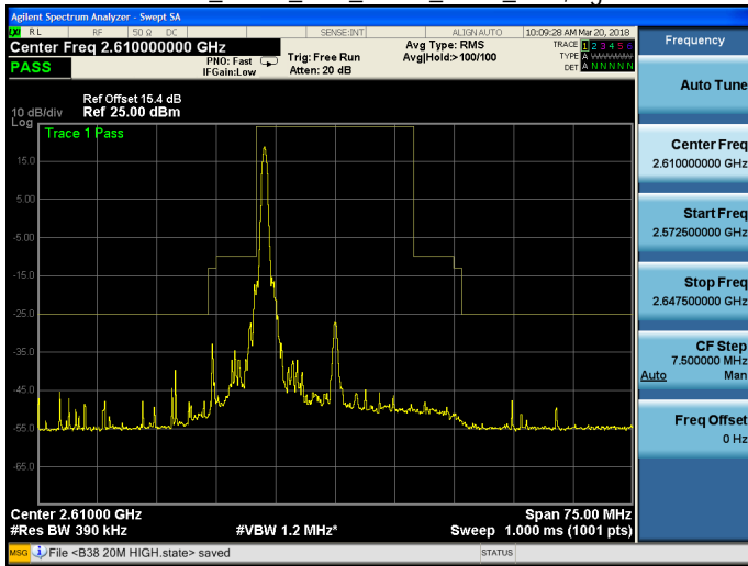
Band 38_QPSK_20M_QPSK_HIGH_RB1,99.gif
