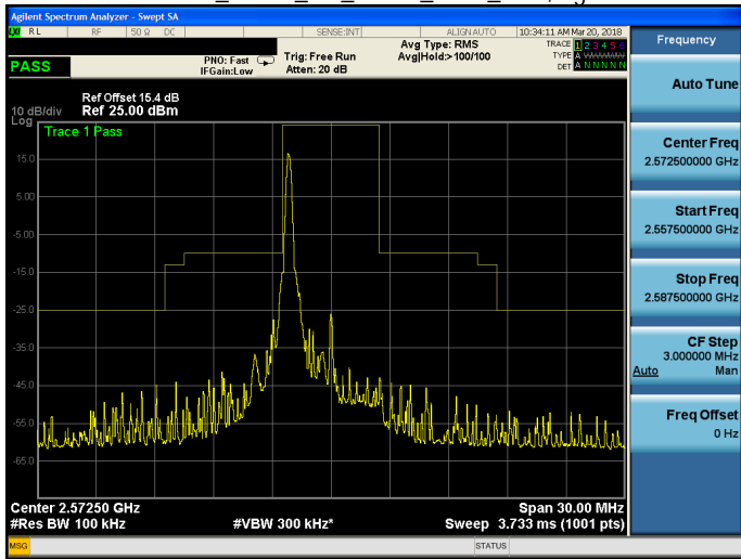
Band 38_QPSK_5M_QPSK_LOW_RB1,24.gif
