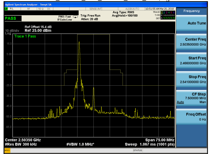
Band 41_16QAM_15M_16QAM_LOW_RB1,74.qif
