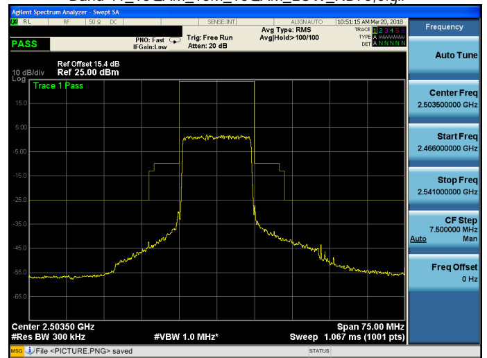
Band 41_16QAM_15M_16QAM_LOW_RB75,0.qif
