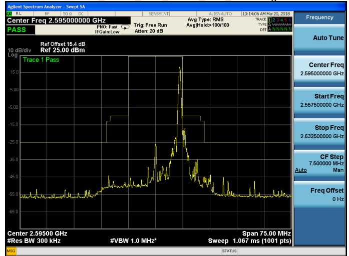
Band 38_QPSK_15M_QPSK_MID_RB75,0.gif
