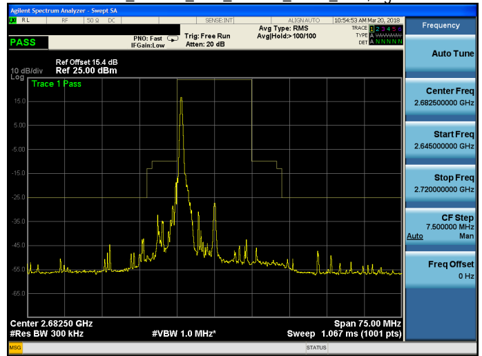
Band 41_16QAM_15M_16QAM_HIGH_RB1,74.gif
