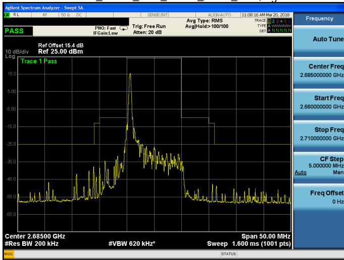
Band 41_QPSK_10M_QPSK_HIGH_RB1,49.gif
