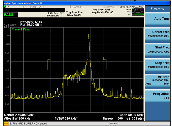
Band 41_QPSK_10M_QPSK_MID_RB50,0.gif
