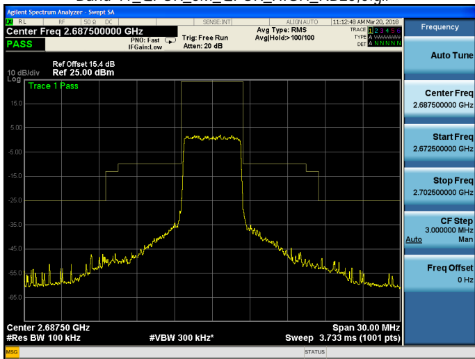
Band 41_QPSK_5M_QPSK_HIGH_RB25,0.gif
