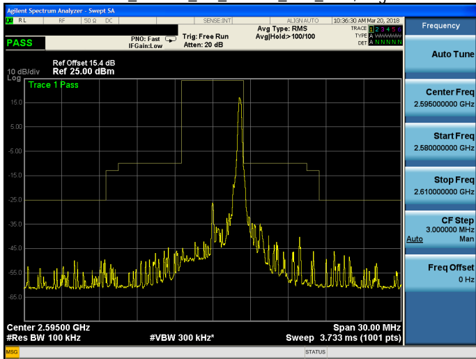
Band 38_16QAM_5M_16QAM_MID_RB25,0.gif
