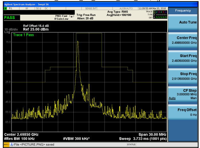
Band 41_16QAM_5M_16QAM_LOW_RB1,24.gif
