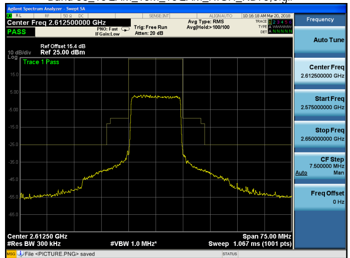
Band 38_16QAM_15M_16QAM_HIGH_RB75,0.gif
