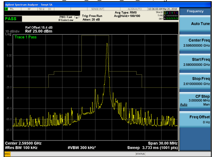
Band 38_QPSK_5M_QPSK_MID_RB25,0.gif
