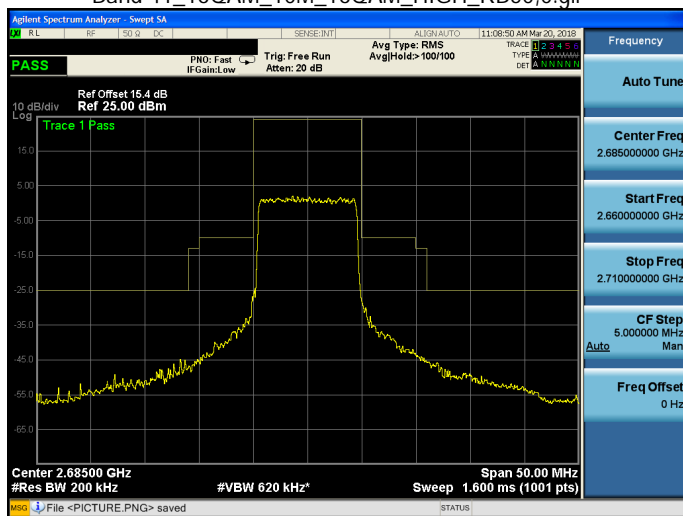
Band 41_16QAM_10M_16QAM_HIGH_RB50,0.gif
