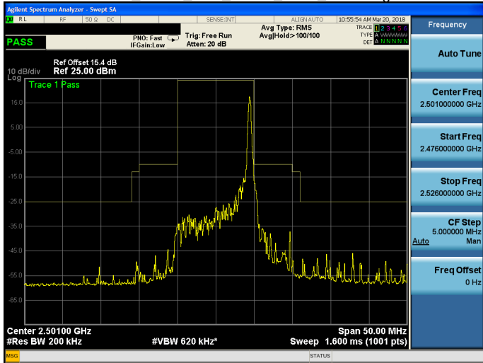
Band 41_QPSK_10M_QPSK_LOW_RB50,0.gif
