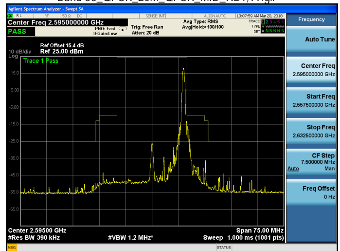
Band 38_QPSK_20M_QPSK_MID_RB100,0.gif
