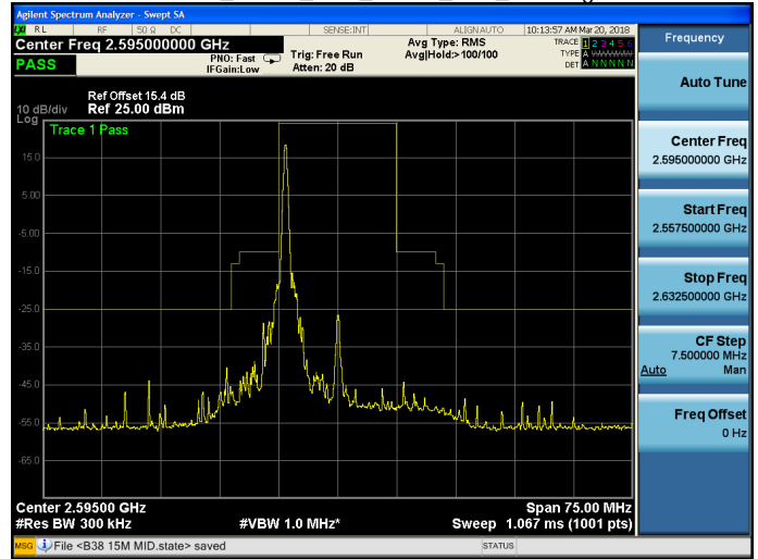
Band 38_QPSK_15M_QPSK_MID_RB1,74.gif
