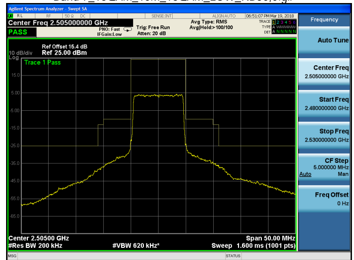
Band 7_16QAM_10M_16QAM_LOW_RB50,0.gif
