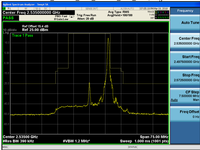
Band 7_16QAM_20M_16QAM_MID_RB100,0.gif
