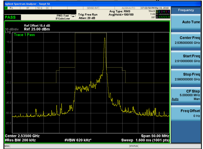
Band 7_QPSK_10M_QPSK_MID_RB50,0.gif
