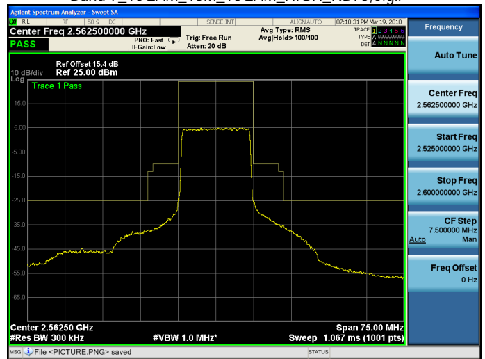
Band 7_16QAM_15M_16QAM_HIGH_RB75,0.gif
