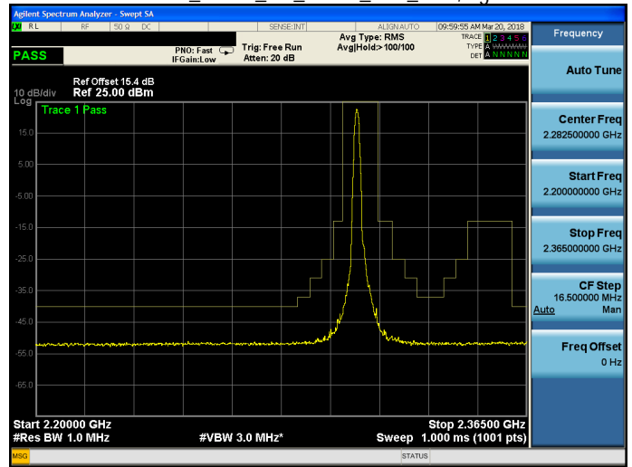
Band 30_QPSK_5M_QPSK_MID_RB1,24.gif
