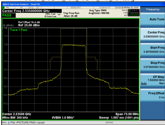
Band 7_16QAM_15M_16QAM_MID_RB75,0.gif
