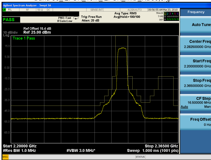
Band 30_QPSK_10M_QPSK_MID_RB50,0.gif
