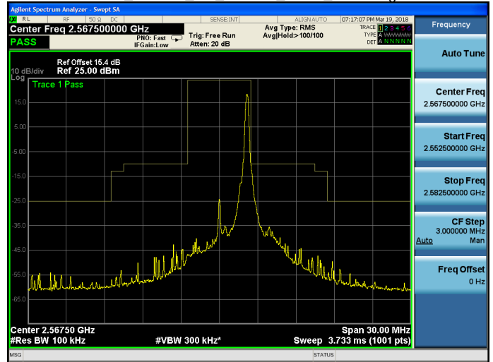
Band 7_16QAM_5M_16QAM_HIGH_RB25,0.gif
