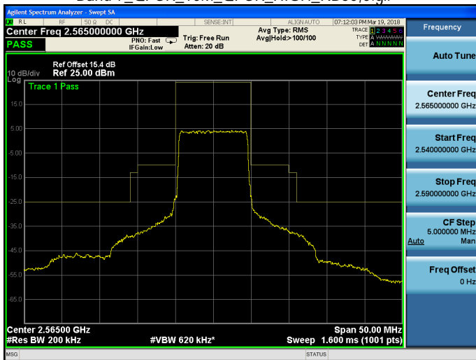
Band 7_QPSK_10M_QPSK_HIGH_RB50,0.gif
