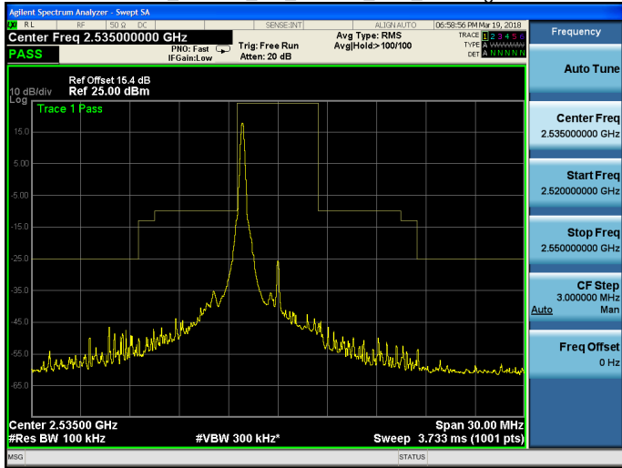
Band 7_16QAM_5M_16QAM_MID_RB1,24.gif
