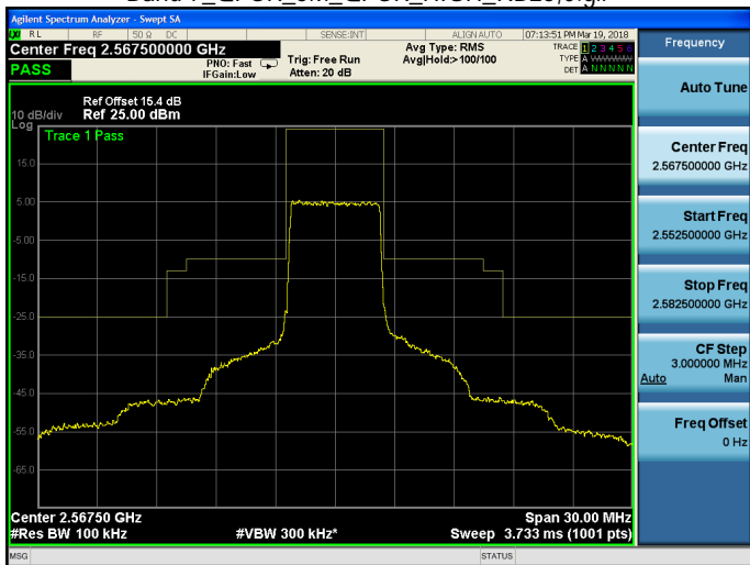
Band 7_QPSK_5M_QPSK_HIGH_RB25,0.gif
