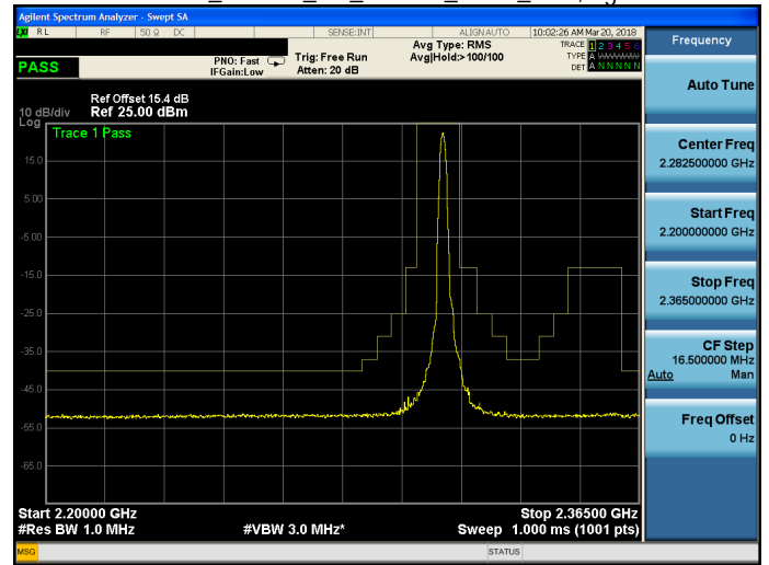
Band 30_16QAM_5M_16QAM_HIGH_RB1,24.gif
