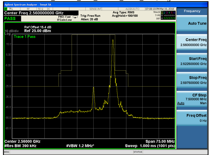
Band 7_16QAM_20M_16QAM_HIGH_RB100,0.gif
