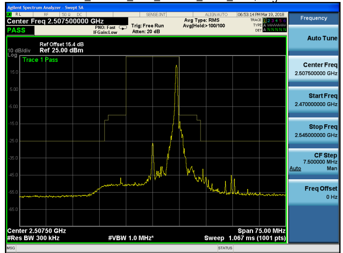
Band 7_16QAM_15M_16QAM_LOW_RB75,0.gif
