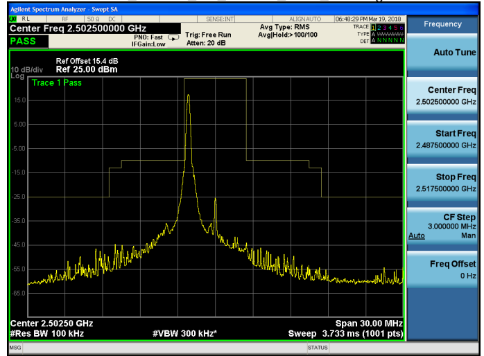
Band 7_16QAM_5M_16QAM_LOW_RB1,24.gif
