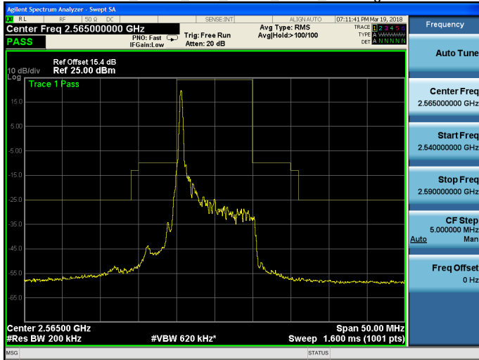
Band 7_QPSK_10M_QPSK_HIGH_RB1,49.gif
