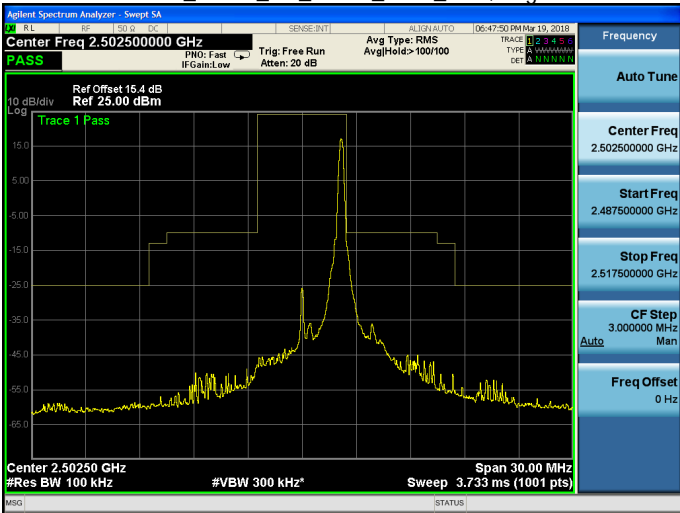
Band 7_QPSK_5M_QPSK_LOW_RB25,0.qjf
