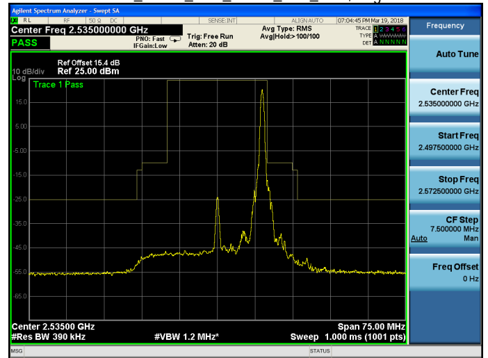
Band 7_QPSK_20M_QPSK_MID_RB100,0.gif
