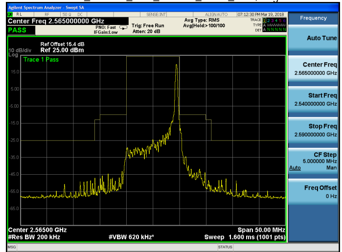
Band 7_16QAM_10M_16QAM_HIGH_RB50,0.qif
