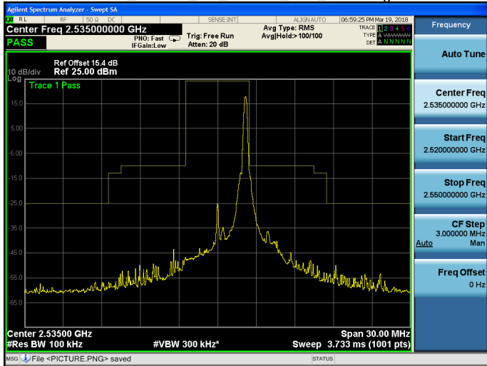
Band 7_16QAM_5M_16QAM_MID_RB25,0.gif
