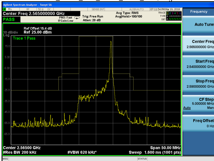
Band 7_QPSK_10M_QPSK_HIGH_RB50,0.gif
