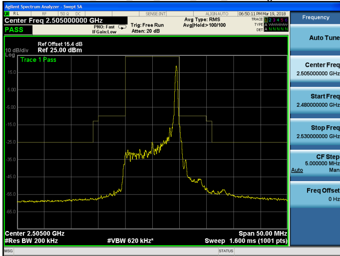
Band 7_QPSK_10M_QPSK_LOW_RB50,0.gif
