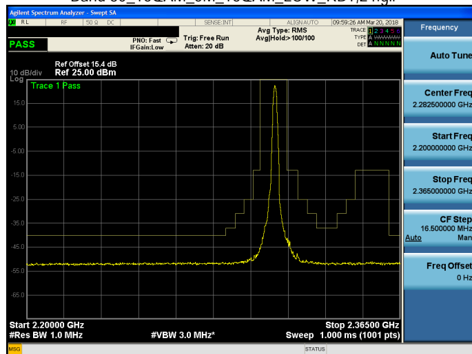
Band 30_16QAM_5M_16QAM_LOW_RB25,0.gif
