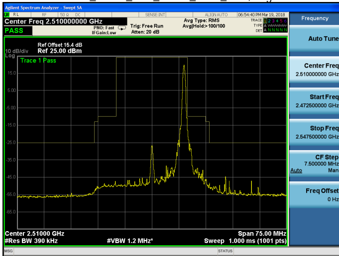
Band 7_QPSK_20M_QPSK_LOW_RB100,0.gif
