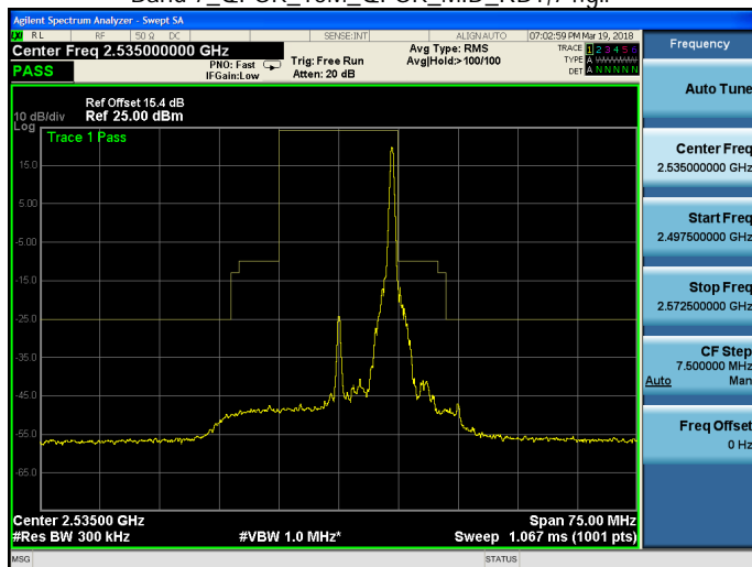
Band 7_QPSK_15M_QPSK_MID_RB75,0.gif
