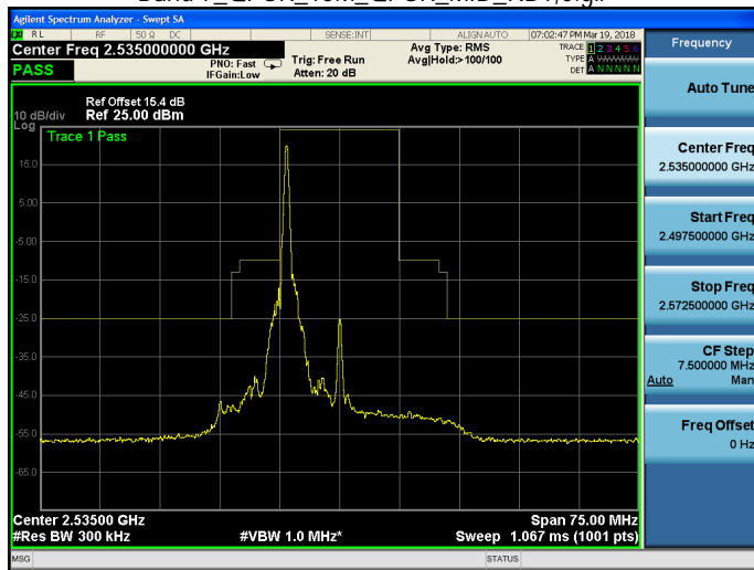
Band 7_QPSK_15M_QPSK_MID_RB1,74.gif
