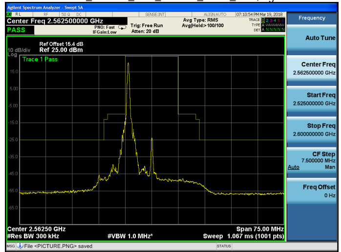
Band 7_16QAM_15M_16QAM_HIGH_RB1,74.gif
