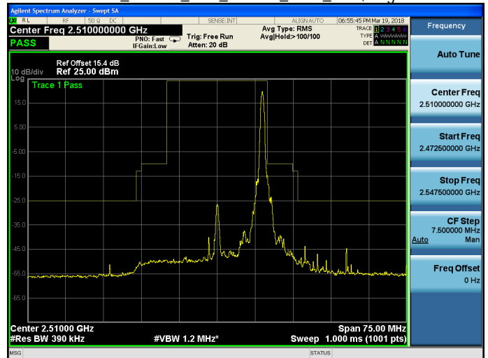
Band 7_16QAM_20M_16QAM_LOW_RB100,0.gif
