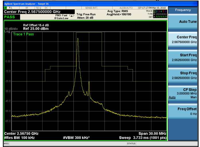
Band 7_16QAM_5M_16QAM_HIGH_RB1,24.gif
