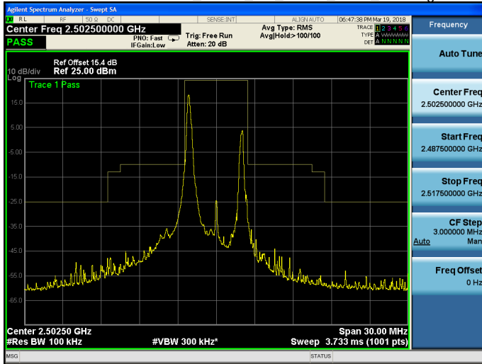
Band 7_QPSK_5M_QPSK_LOW_RB1,24.qjf
