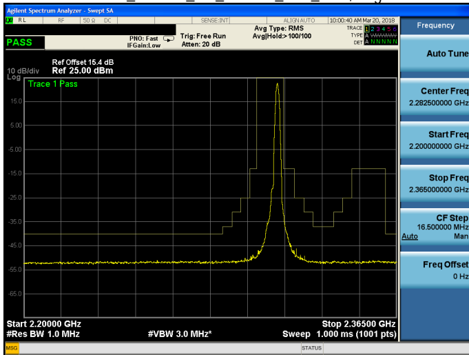
Band 30_16QAM_5M_16QAM_MID_RB25,0.gif
