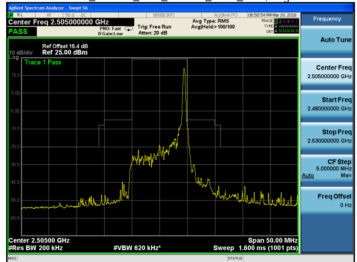
Band 7_16QAM_10M_16QAM_LOW_RB50,0.gif
