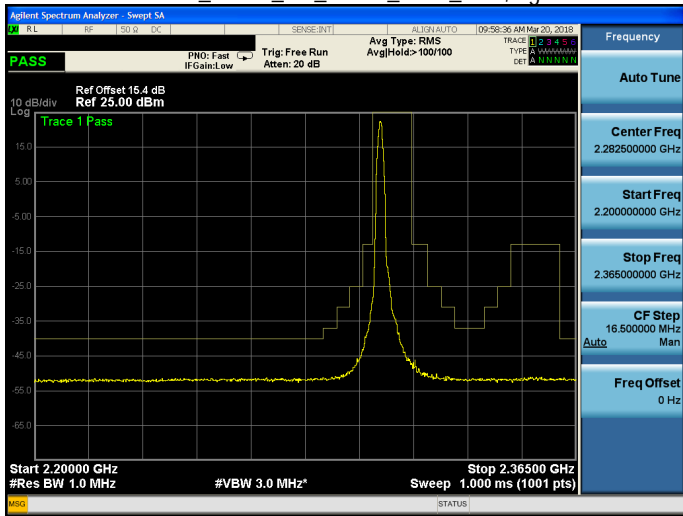
Band 30_QPSK_5M_QPSK_LOW_RB1,24.gif
