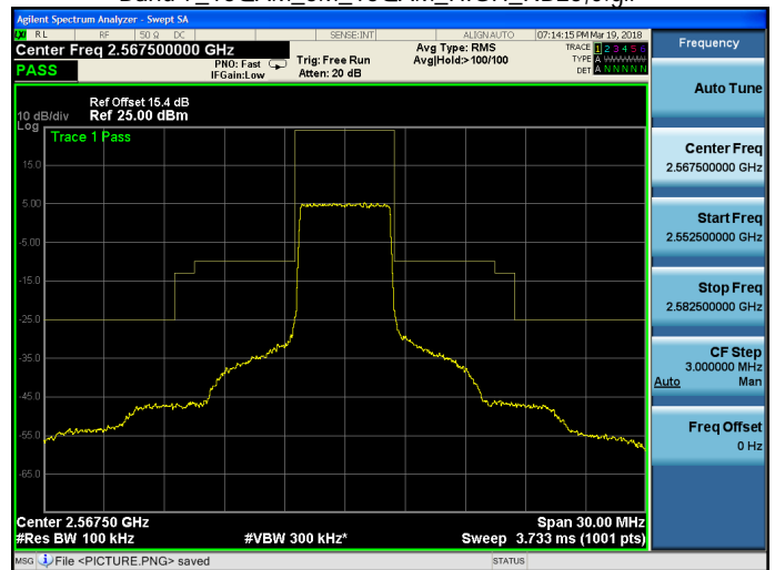
Band 7_16QAM_5M_16QAM_HIGH_RB25,0.gif
