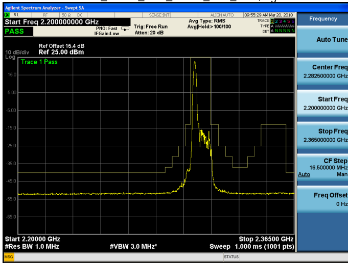
Band 30_QPSK_10M_QPSK_MID_RB1,49.gif
