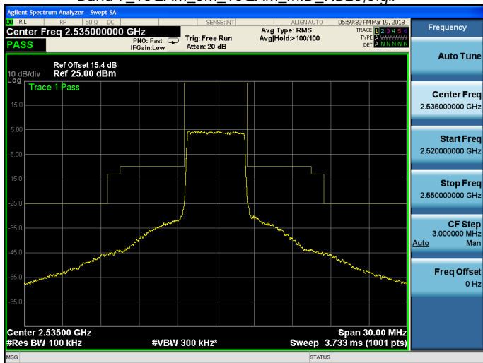
Band 7_16QAM_5M_16QAM_MID_RB25,0.gif
