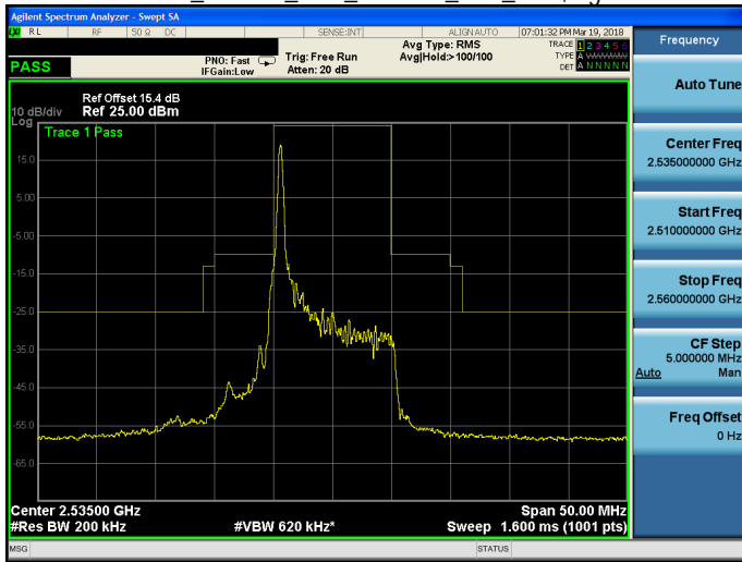
Band 7_16QAM_10M_16QAM_MID_RB1,49.qif
