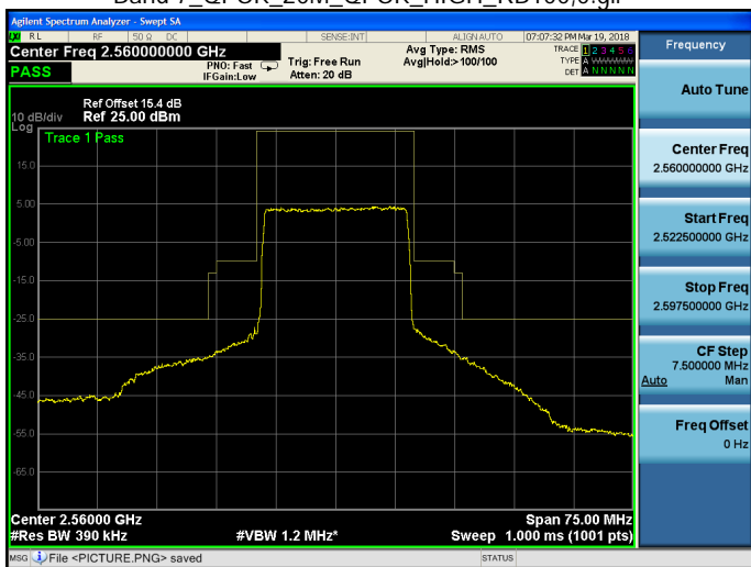
Band 7_QPSK_20M_QPSK_HIGH_RB100,0.gif
