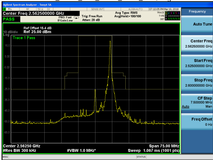
Band 7_QPSK_15M_QPSK_HIGH_RB75,0.gif
