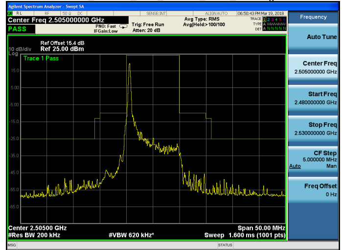
Band 7_16QAM_10M_16QAM_LOW_RB1,49.gif
