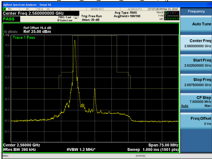
Band 7_QPSK_20M_QPSK_HIGH_RB1,99.gif
