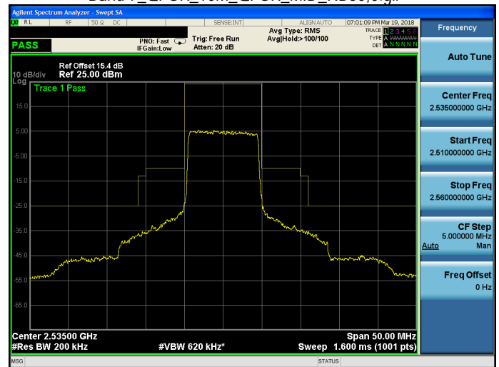
Band 7_QPSK_10M_QPSK_MID_RB50,0.gif
