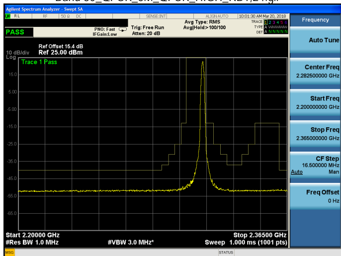
Band 30_QPSK_5M_QPSK_HIGH_RB25,0.gif
