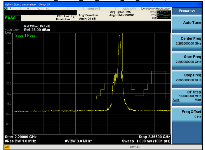
Band 30_16QAM_10M_16QAM_MID_RB50,0.gif
