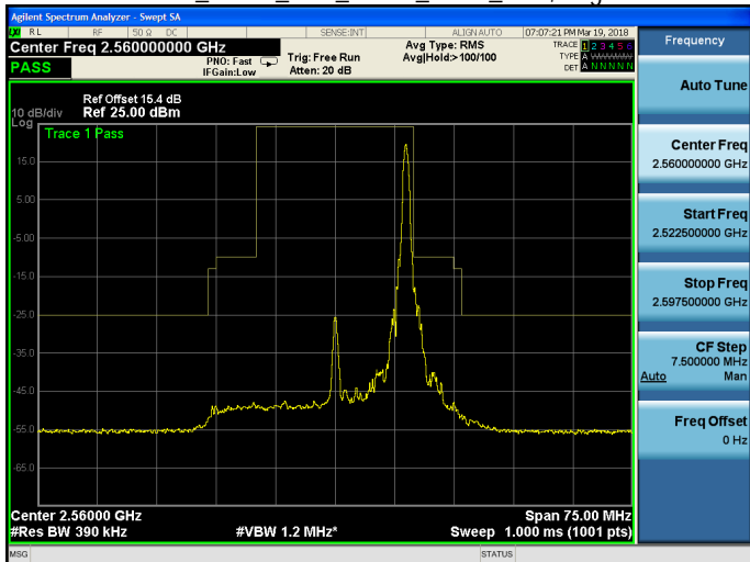
Band 7_QPSK_20M_QPSK_HIGH_RB100,0.gif
