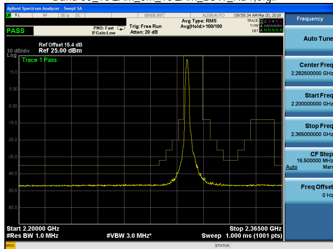
Band 30_16QAM_5M_16QAM_LOW_RB1,24.gif
