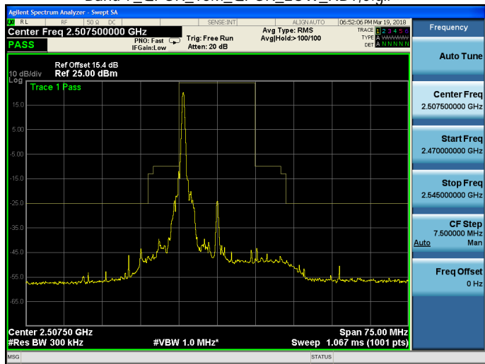
Band 7_QPSK_15M_QPSK_LOW_RB1,74.gif
