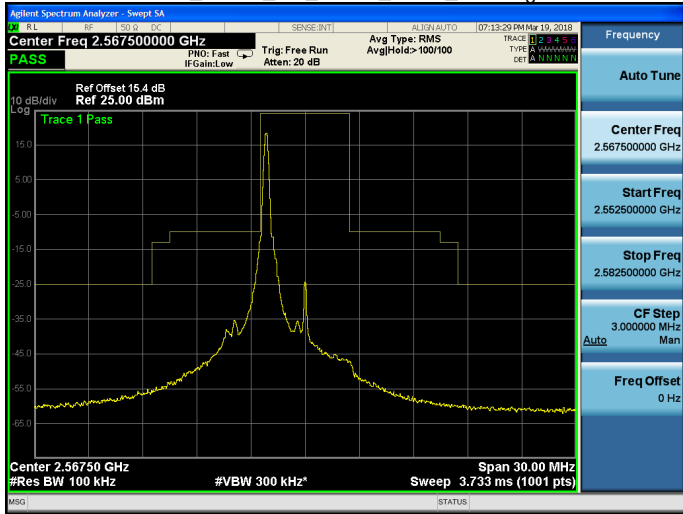
Band 7_QPSK_5M_QPSK_HIGH_RB1,24.gif
