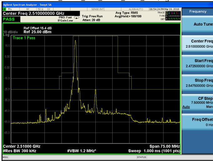
Band 7_QPSK_20M_QPSK_LOW_RB1,99.gif
