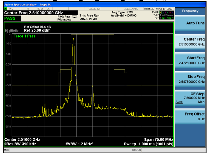
Band 7_16QAM_20M_16QAM_LOW_RB1,99.gif
