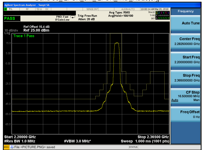
Band 30_QPSK_5M_QPSK_MID_RB25,0.gif
