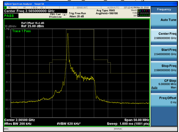
Band 7_16QAM_10M_16QAM_HIGH_RB1,49.qif
