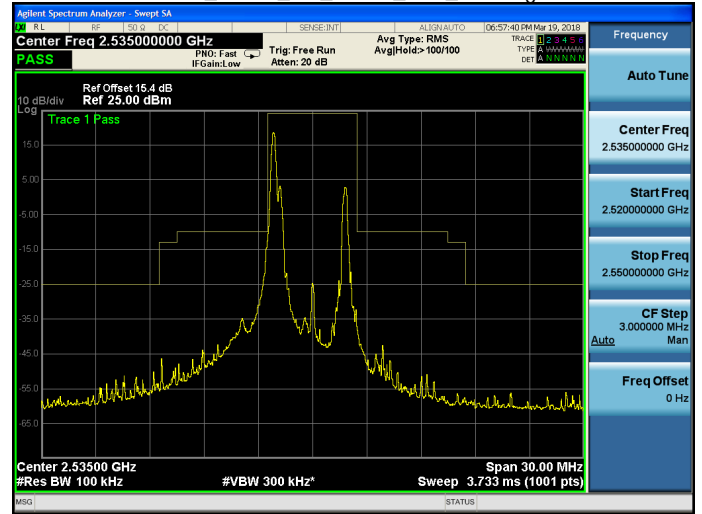
Band 7_QPSK_5M_QPSK_MID_RB1,24.qjf
