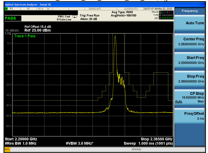
Band 30_16QAM_10M_16QAM_MID_RB1,49.gif
