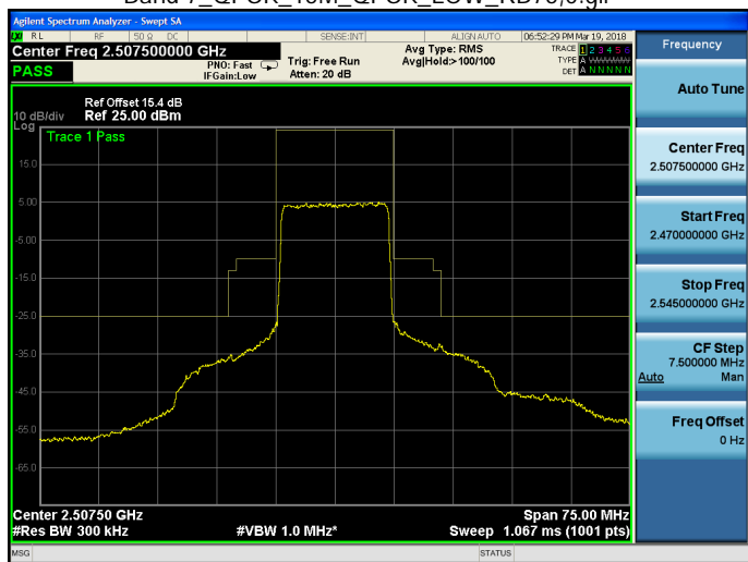
Band 7_QPSK_15M_QPSK_LOW_RB75,0.gif
