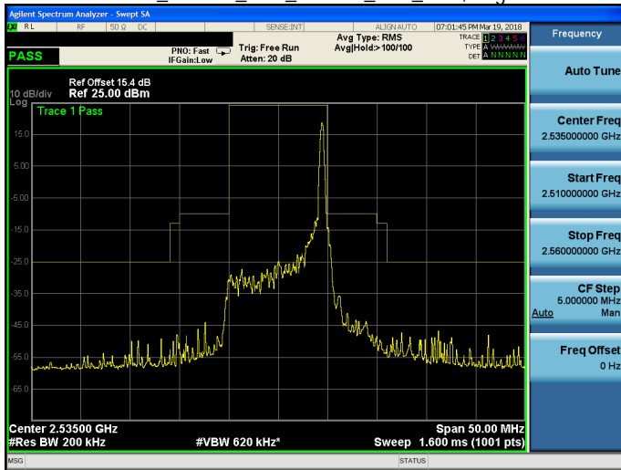
Band 7_16QAM_10M_16QAM_MID_RB50,0.qif
