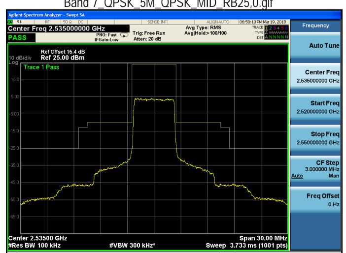
Band 7_QPSK_5M_QPSK_MID_RB25,0.qjf
