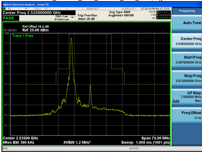
Band 7_16QAM_20M_16QAM_MID_RB1,99.gif
