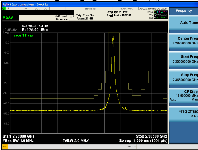
Band 30_16QAM_5M_16QAM_MID_RB1,24.gif
