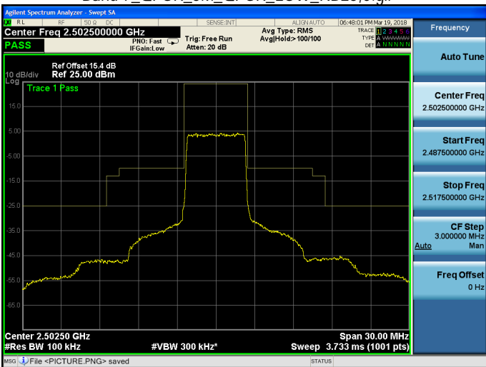
Band 7_QPSK_5M_QPSK_LOW_RB25,0.qjf
