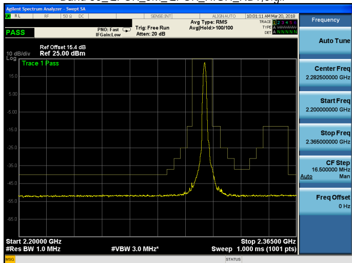
Band 30_QPSK_5M_QPSK_HIGH_RB1,24.gif
