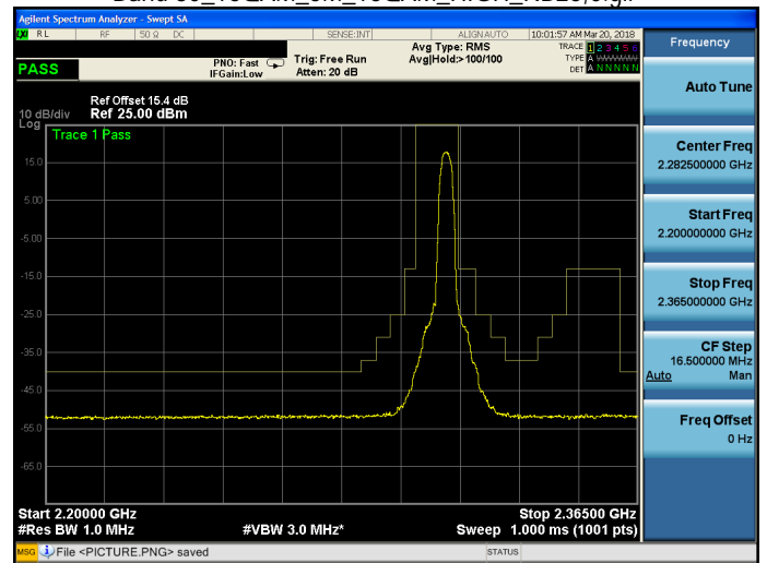
Band 30_16QAM_5M_16QAM_HIGH_RB25,0.gif
