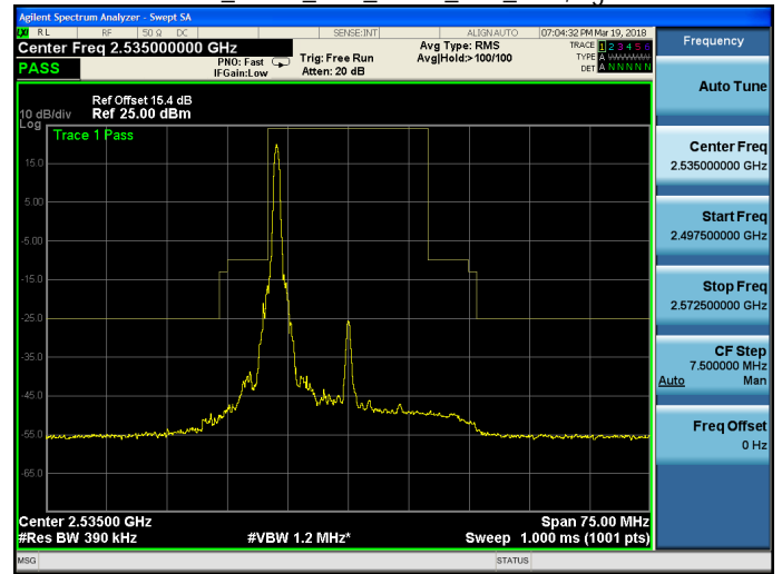
Band 7_QPSK_20M_QPSK_MID_RB1,99.gif
