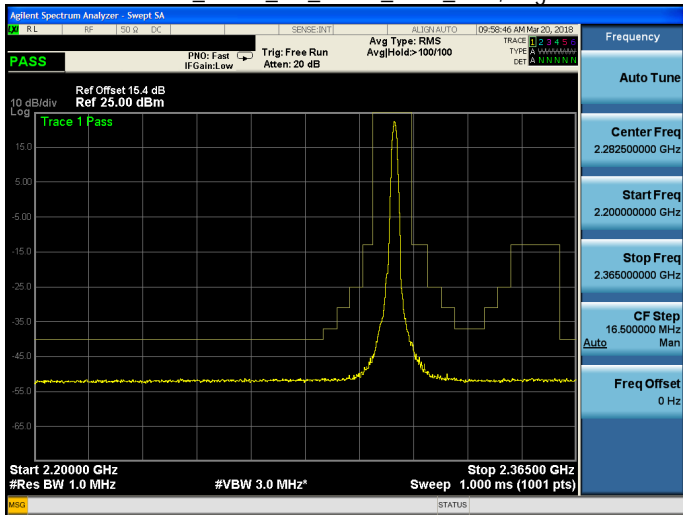
Band 30_QPSK_5M_QPSK_LOW_RB25,0.gif
