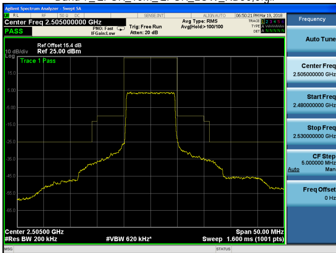
Band 7_QPSK_10M_QPSK_LOW_RB50,0.gif
