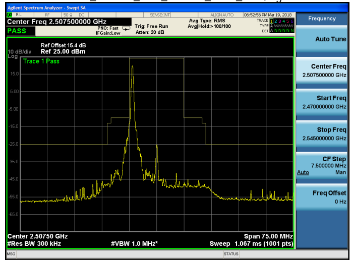
Band 7_16QAM_15M_16QAM_LOW_RB1,74.gif
