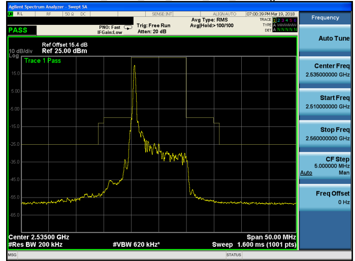
Band 7_QPSK_10M_QPSK_MID_RB1,49.gif
