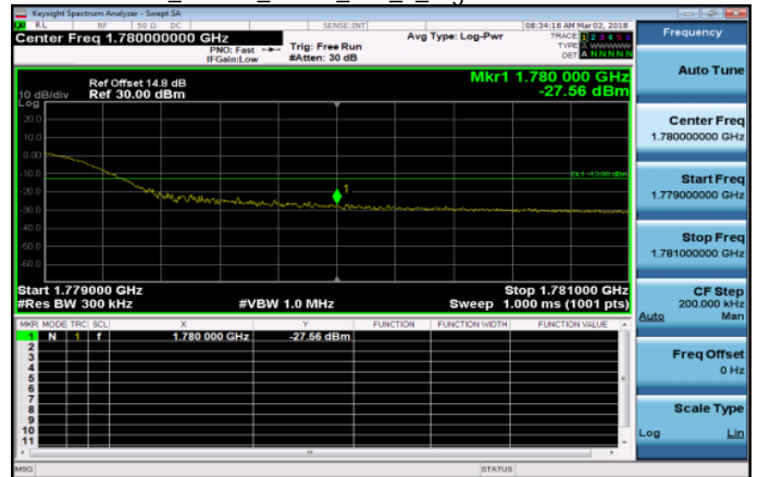
Band66_20MHz_QPSK_100_0_HighCH132572-1770
