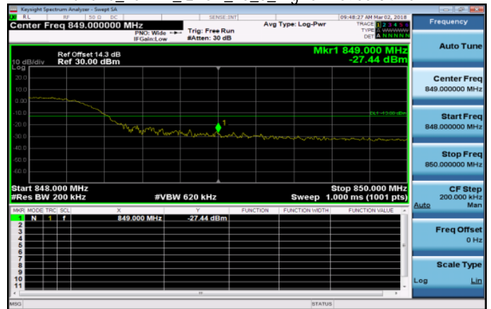
Band26_15MHz_QPSK_75_0_HighCH26965-841.5
