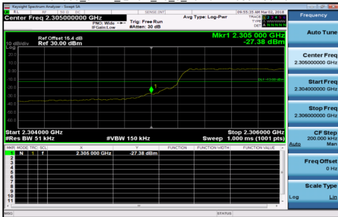
Band30_5MHz_QPSK_25_0_LowCH27685-2307.5
