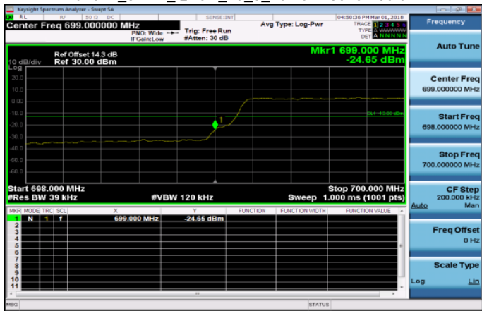
Band12_3MHz_QPSK_15_0_LowCH23025-700.5
