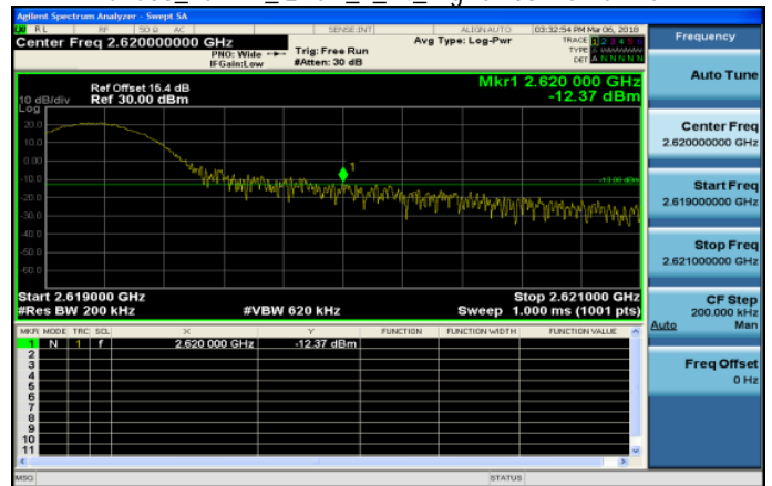
Band38_15MHz_QPSK_1_74_HighCH38175-2612.5
