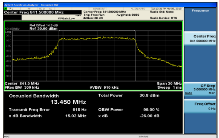
Band26_15MHz_QPSK_75_0_HighCH26965-841.5
