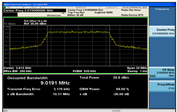
Band38_10MHz_16QAM_50_0_HighCH38200-2615
