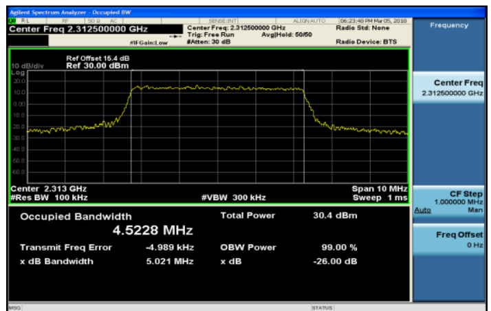
Band30_5MHz_QPSK_25_0_HighCH27735-2312.5
