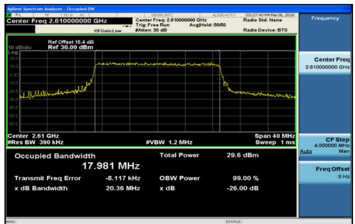
Band38_20MHz_16QAM_100_0_HighCH38150-2610
