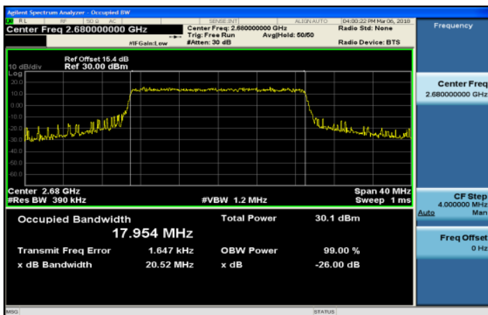
Band41_20MHz_QPSK_100_0_HighCH41490-2680
