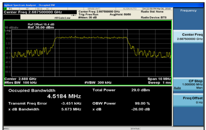
Band41_5MHz_16QAM_25_0_HighCH41565-2687.5
