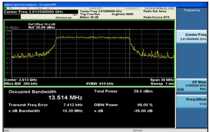
Band38_15MHz_16QAM_75_0_HighCH38175-2612.5
