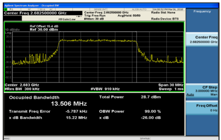
Band41_15MHz_16QAM_75_0_HighCH41515-2682.5
