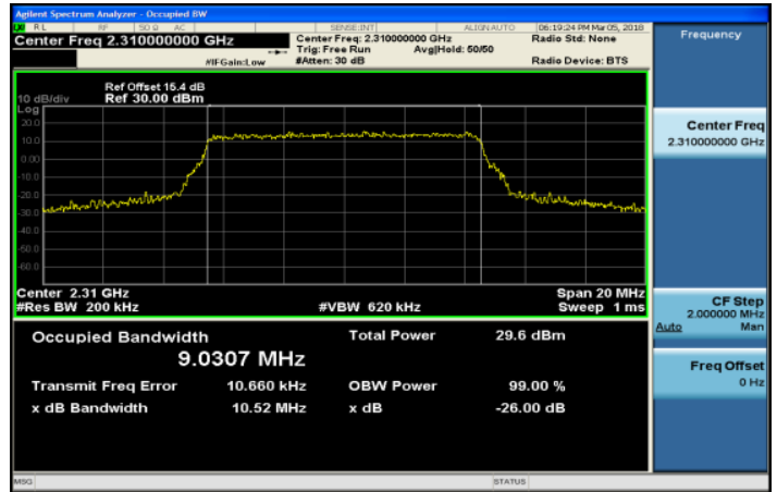
Band30_10MHz_16QAM_50_0_MidCH27710-2310
