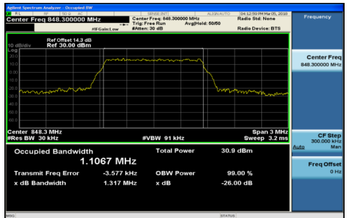
Band26_1_4MHz_QPSK_6_0_HighCH27033-848.3
