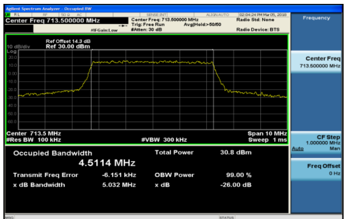
Band17_5MHz_QPSK_25_0_HighCH23825-713.5
