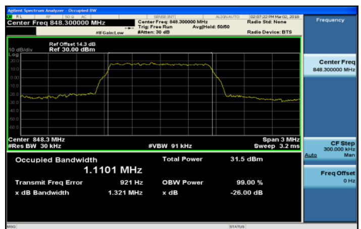
Band5_1_4MHz_QPSK_6_0_HighCH20643-848.3
