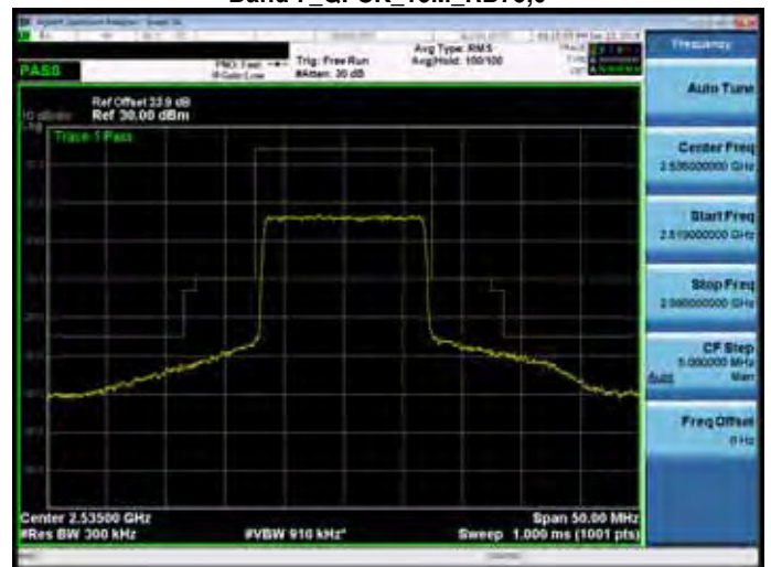
Band 7_QPSK_15M_RB75,0
