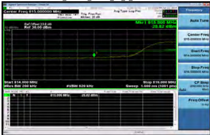
Band26_15MHz_QPSK_75_0_LowCH26775
