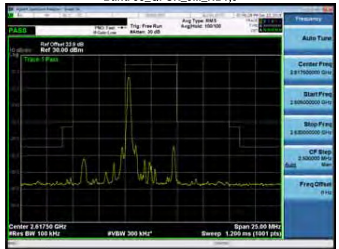
Band 38_QPSK_5M_RB1,24
