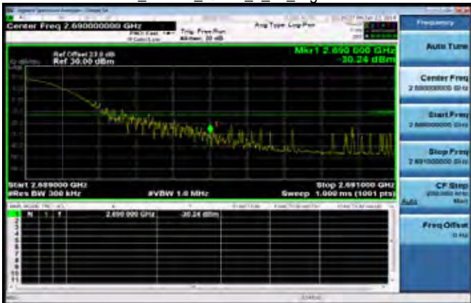
Band41_20MHz_QPSK_1_99_HighCH41490
