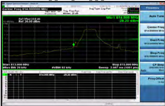
Band26_1_4MHz_QPSK_1_0_LowCH26697
