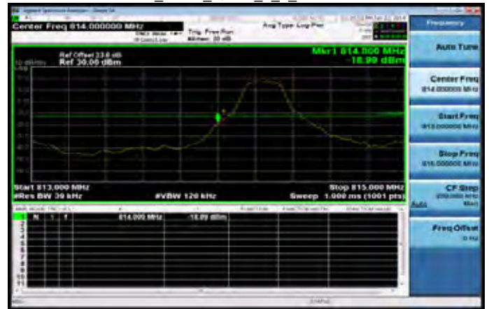
Band26_3MHz_QPSK_1_0_LowCH26705
