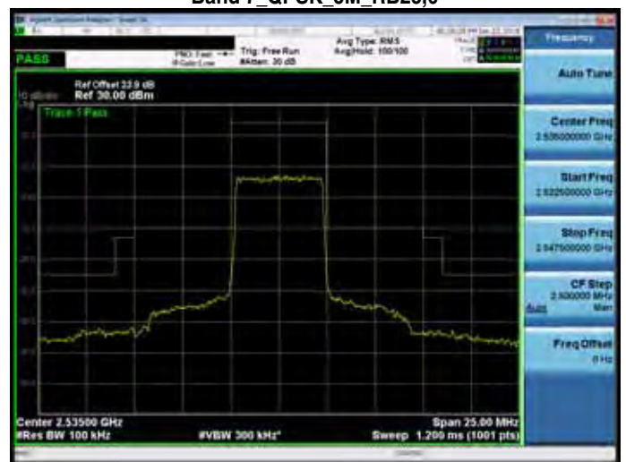
Band 7_QPSK_5M_RB25,0
