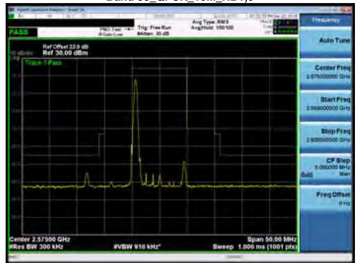
Band 38_QPSK_10M_RB1,49
