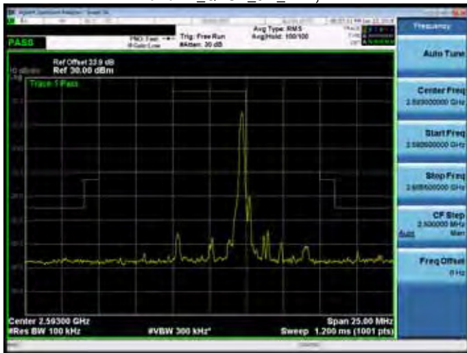
Band 41_QPSK_5M_RB1,24
