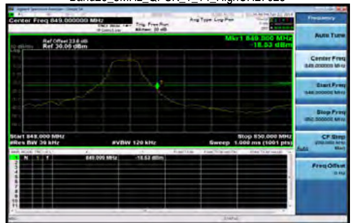
Band26_3MHz_QPSK_1_14_HighCH27025
