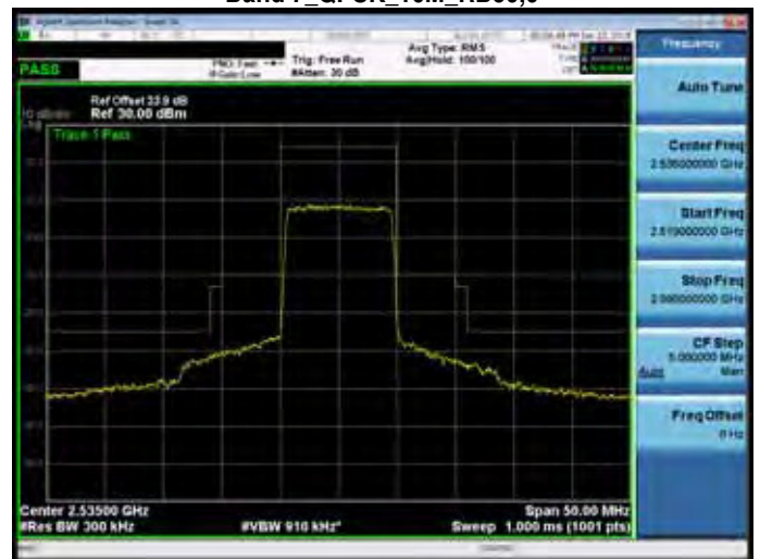
Band 7_QPSK_10M_RB50,0
