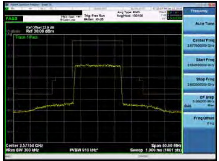
Band 38_16QAM_15M_RB1,0
