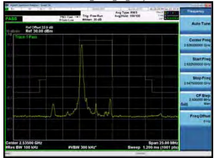
Band 7_QPSK_5M_RB1,24
