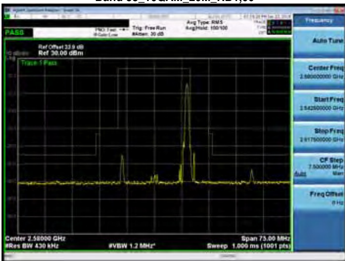
Band 38_16QAM_20M_RB1,99
