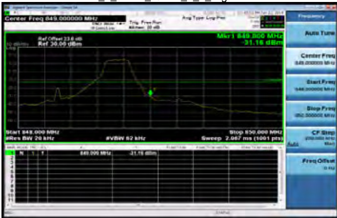
Band26_1_4MHz_QPSK_1_5_HighCH27033
