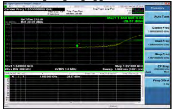
Band25_20MHz_QPSK_100_0_LowCH26140-1860
