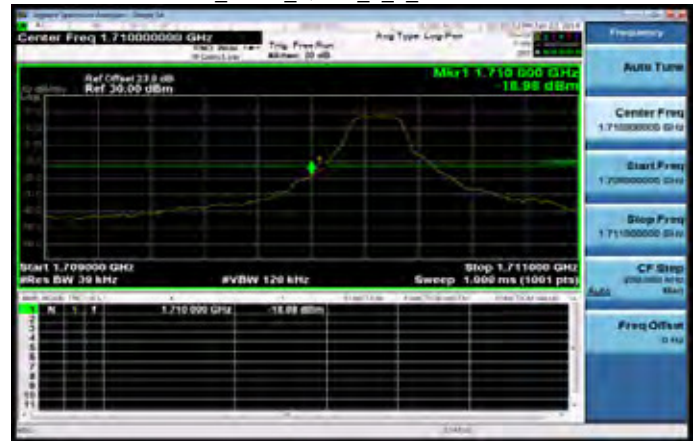
Band66_3MHz_QPSK_1_0_LowCH131987
