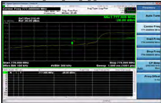
Band13_10MHz_QPSK_50_0_LowCH23230-782
