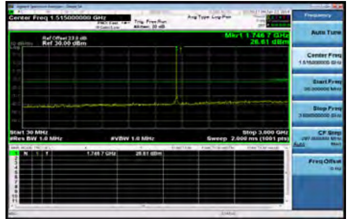
30MHz~3GHz_Band66_1_4MHz_QPSK_1_0_MidCH132322
