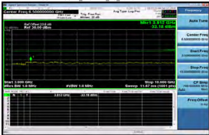
3GHz~10GHz_WCDMA_B5_LowCH4132-826.4
