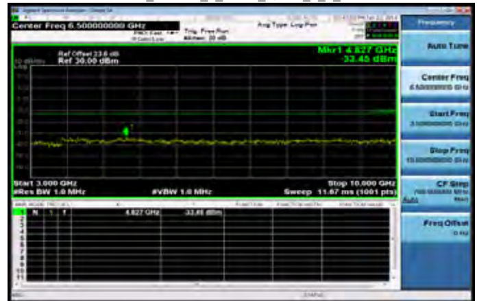
3GHz~10GHz_Band26_1_4MHz_QPSK_1_0_MidCH26865
