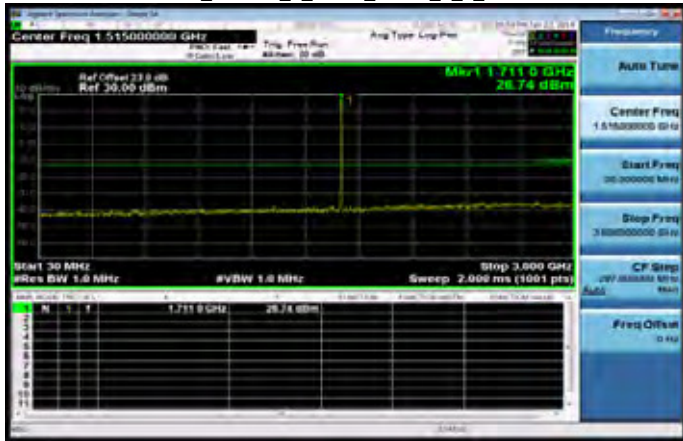
30MHz~3GHz_Band66_1_4MHz_QPSK_1_0_LowCH131979
