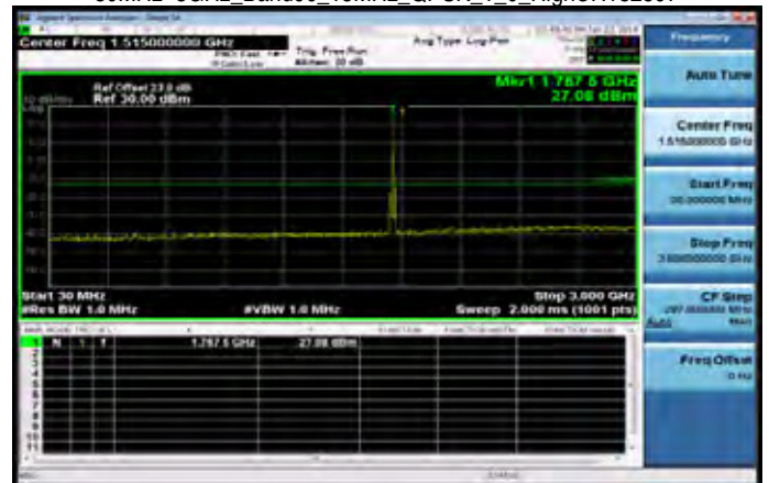
30MHz~3GHz_Band66_15MHz_QPSK_1_0_HighCH132597
