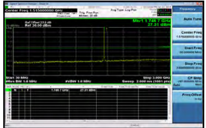
30MHz~3GHz_Band66_3MHz_QPSK_1_0_MidCH132322
