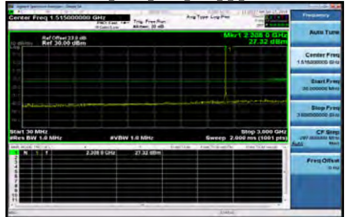
30MHz~3GHz_Band30_10MHz_QPSK_1_0_MidCH27710
