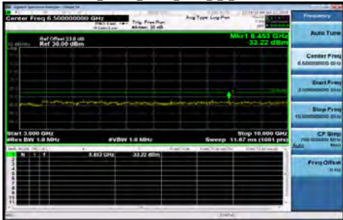
3GHz~10GHz_Band13_10MHz_QPSK_1_0_MidCH23230-782
