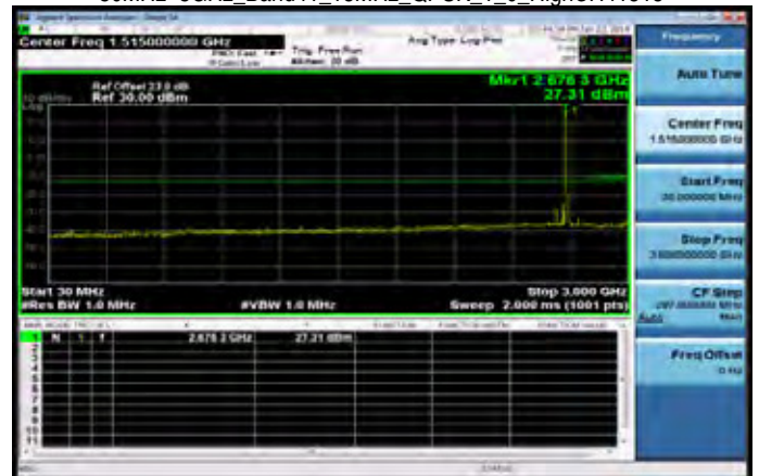
30MHz~3GHz_Band41_15MHz_QPSK_1_0_HighCH41515
