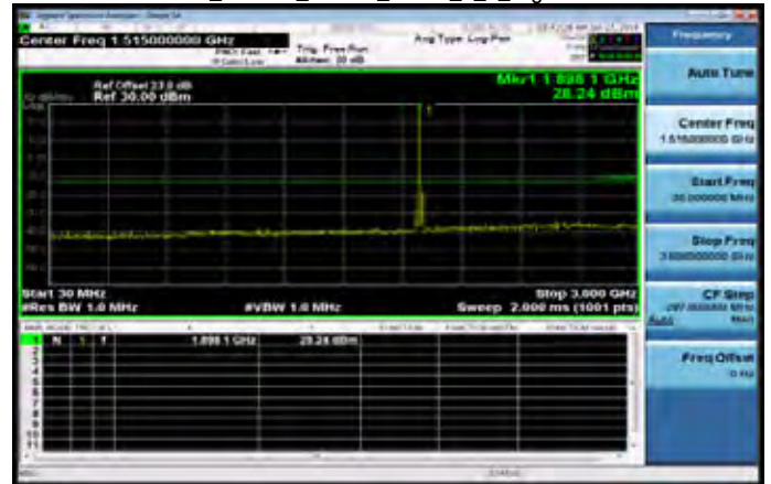
30MHz~3GHz_Band25_20MHz_QPSK_1_0_HighCH26590-1905
