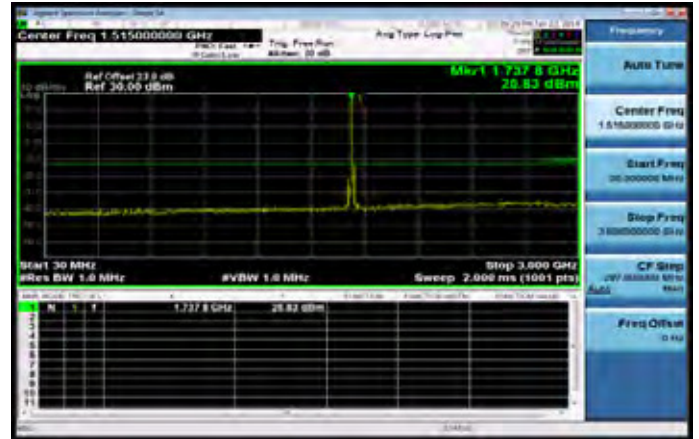
30MHz~3GHz_Band66_20MHz_QPSK_1_0_MidCH132322
