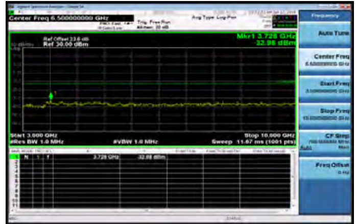
3GHz~10GHz_Band5_1_4MHz_QPSK_1_0_MidCH20525-836.5
