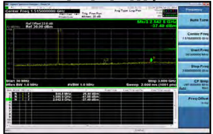
30MHz~3GHz_Band26_3MHz_QPSK_1_0_HighCH27025
