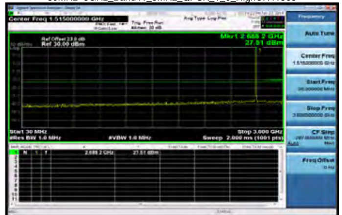
30MHz~3GHz_Band41_5MHz_QPSK_1_0_HighCH41565
