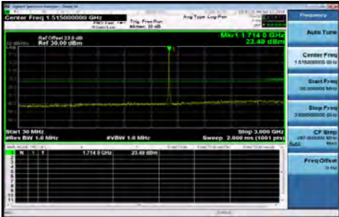
30MHz-3GHz_HSDPA_B4_LowCH1312-1712.4
