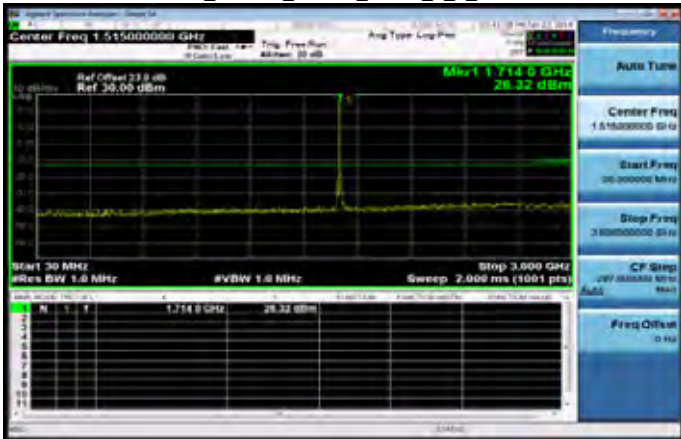
30MHz~3GHz_Band66_15MHz_QPSK_1_0_LowCH132047
