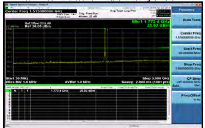
30MHz~3GHz_Band66_10MHz_QPSK_1_0_HighCH132622
