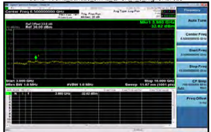
3GHz~10GHz_Band26_3MHz_QPSK_1_0_HighCH27025
