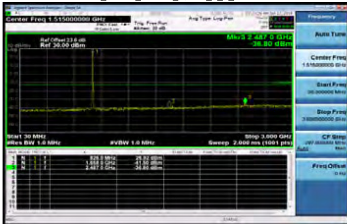
30MHz~3GHz_Band5_10MHz_QPSK_1_0_LowCH20450-829
