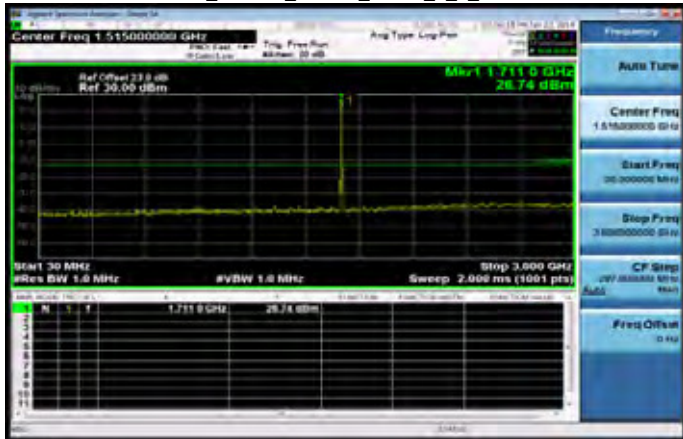
30MHz~3GHz_Band66_10MHz_QPSK_1_0_LowCH132022
