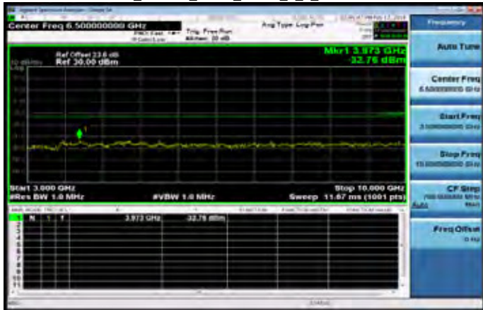
3GHz~10GHz_Band12_5MHz_QPSK_1_0_LowCH23035-701.5
