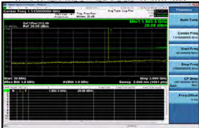
30MHz~3GHz_Band25_1_4MHz_QPSK_1_0_MidCH26365-1882.5
