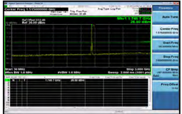
30MHz~3GHz_Band66_15MHz_QPSK_1_0_MidCH132322
