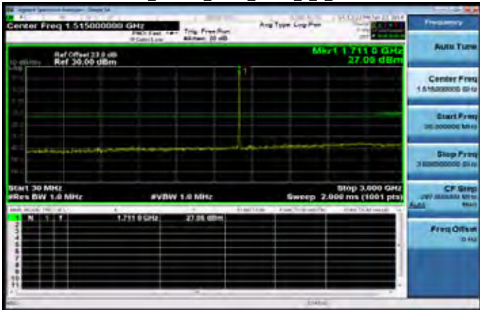
30MHz~3GHz_Band66_5MHz_QPSK_1_0_LowCH131997
