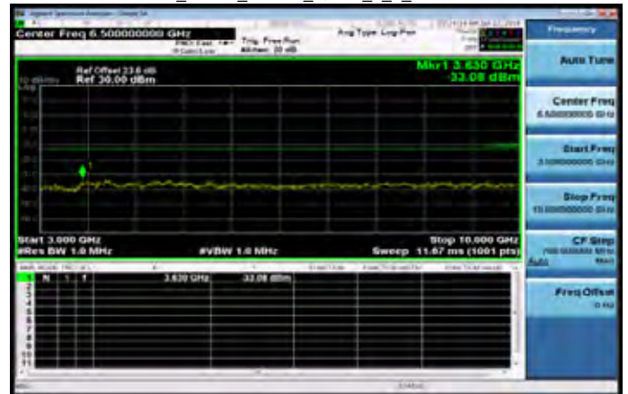
3GHz~10GHz_Band5_10MHz_QPSK_1_0_MidCH20525-836.5
