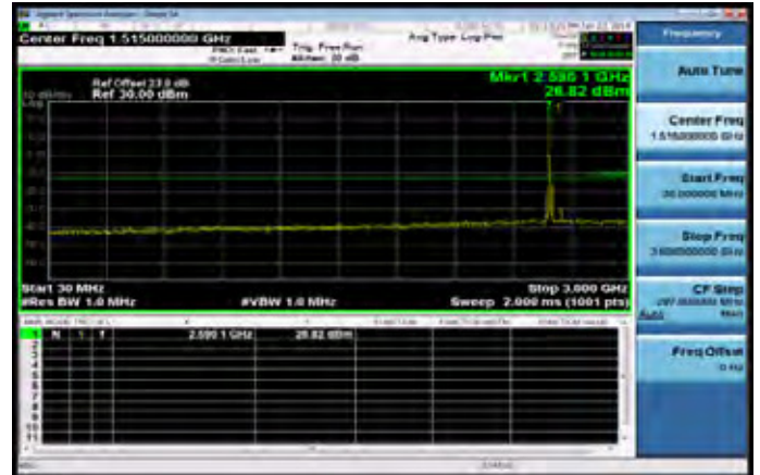
30MHz~3GHz_Band38_15MHz_QPSK_1_0_MidCH38000-2595
