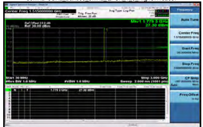
30MHz~3GHz_Band66_3MHz_QPSK_1_0_HighCH132657
