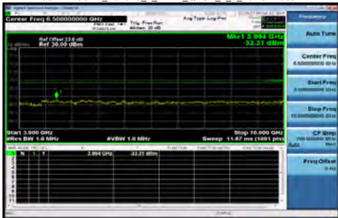
3GHz~10GHz_Band26_1_4MHz_QPSK_1_0_LowCH26697
