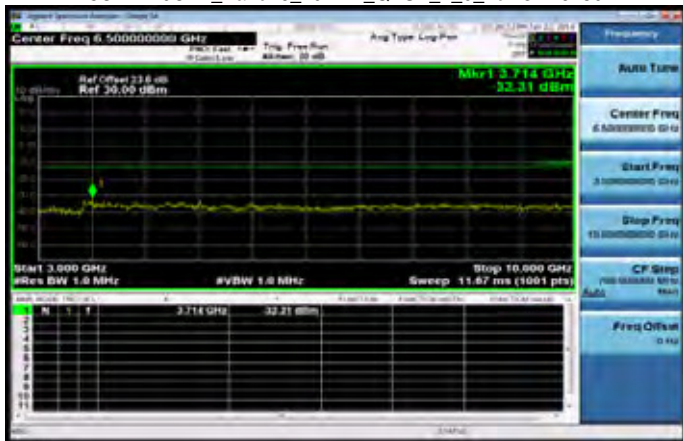
3GHz~10GHz_Band26_10MHz_QPSK_1_0_LowCH26750
