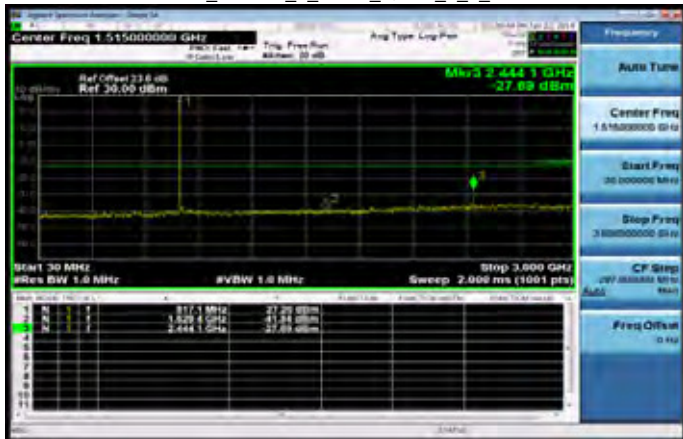
30MHz~3GHz_Band26_1_4MHz_QPSK_1_0_LowCH26697
