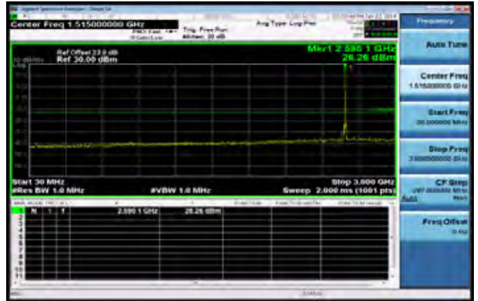
30MHz~3GHz_Band41_10MHz_QPSK_1_0_MidCH40620
