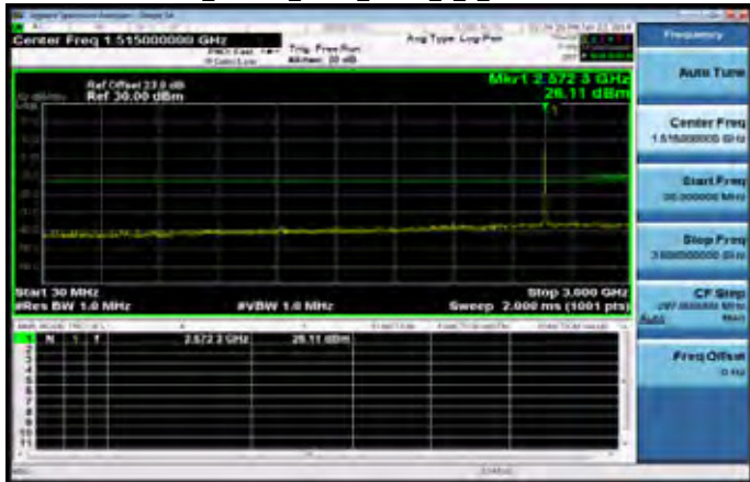
30MHz~3GHz_Band38_5MHz_QPSK_1_0_LowCH37775-2572.5
