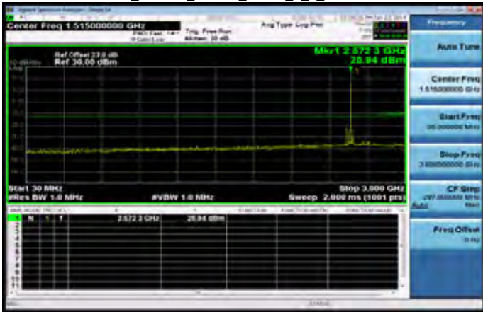
30MHz~3GHz_Band38_20MHz_QPSK_1_0_LowCH37850-2580
