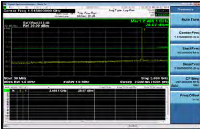
30MHz~3GHz_Band41_5MHz_QPSK_1_0_LowCH39675
