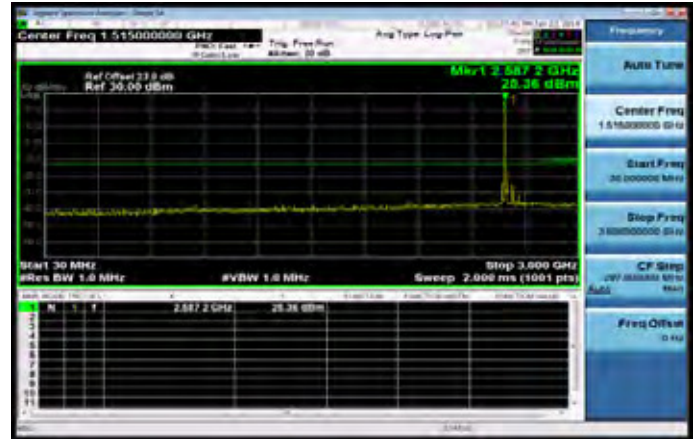
30MHz~3GHz_Band41_15MHz_QPSK_1_0_MidCH40620
