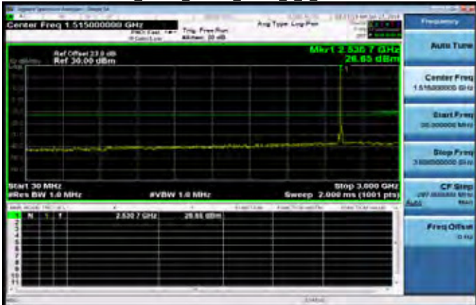
30MHz~3GHz_Band7_15MHz_QPSK_1_0_MidCH21100-2535
