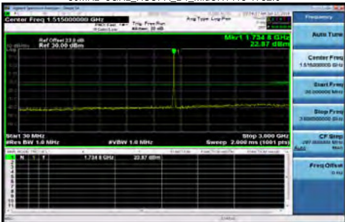
30MHz-3GHz_HSUPA_B4_MidCH1413-1732.6
