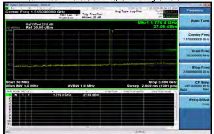
30MHz~3GHz_Band66_5MHz_QPSK_1_0_HighCH132647
