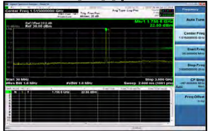
30MHz-3GHz_HSUPA_B4_HighCH1513-1752.6
