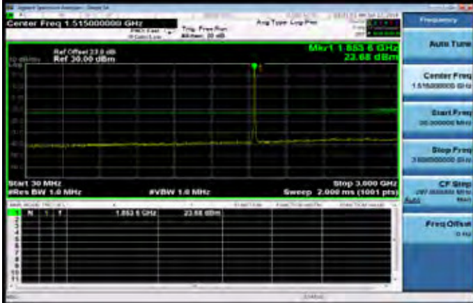
Out of Band Emission30MHz~3GHz_WCDMA_B2_LowCH9262-1852.4
