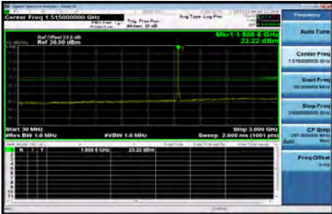
30MHz~3GHz_HSUPA_B2_LowCH9262-1852.4
