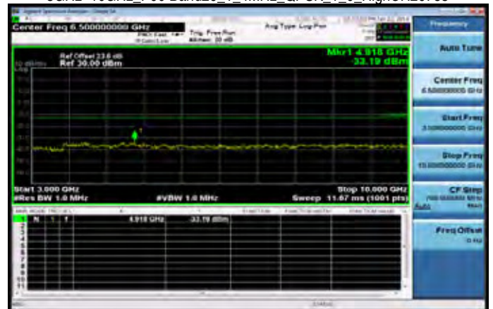
3GHz~10GHz_P90 Band26_1_4MHz_QPSK_1_0_HighCH26783
