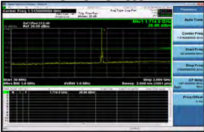
30MHz~3GHz_Band66_20MHz_QPSK_1_0_LowCH132072
