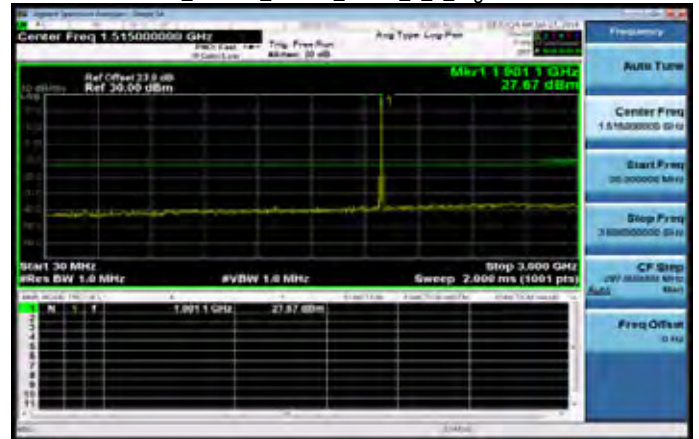
30MHz~3GHz_Band25_15MHz_QPSK_1_0_HighCH26615-1907.5
