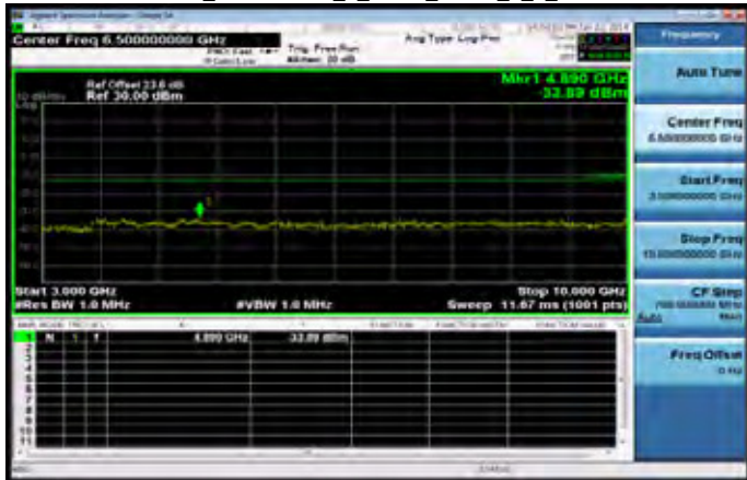
3GHz~10GHz_P90 Band26_1_4MHz_QPSK_1_0_LowCH26697
