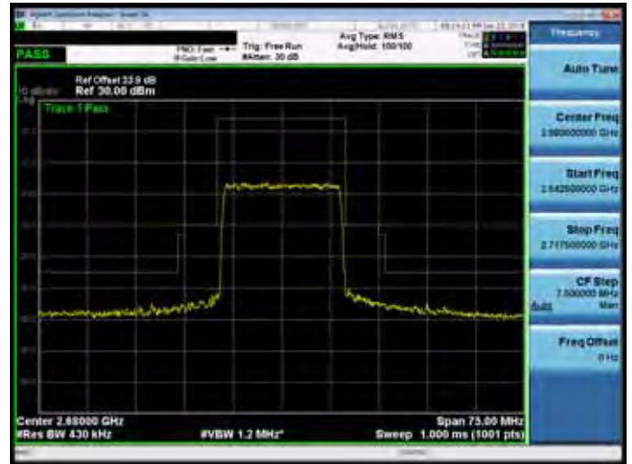
Band 41_16QAM_20M_RB100,0
