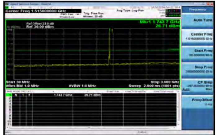
30MHz~3GHz_Band66_10MHz_QPSK_1_0_MidCH132322
