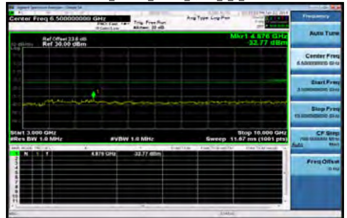
3GHz~10GHz_Band26_15MHz_QPSK_1_0_MidCH26865
