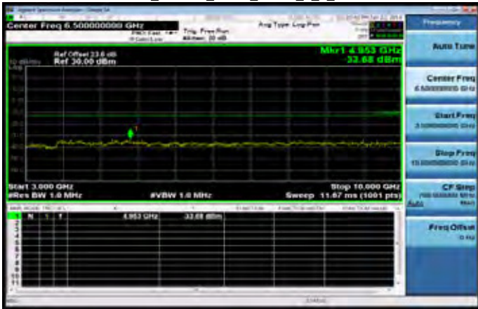
3GHz~10GHz_Band26_3MHz_QPSK_1_0_LowCH26705
