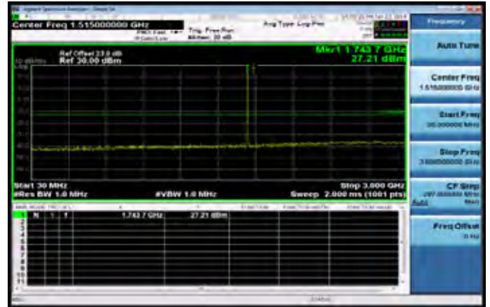
30MHz~3GHz_Band66_5MHz_QPSK_1_0_MidCH132322
