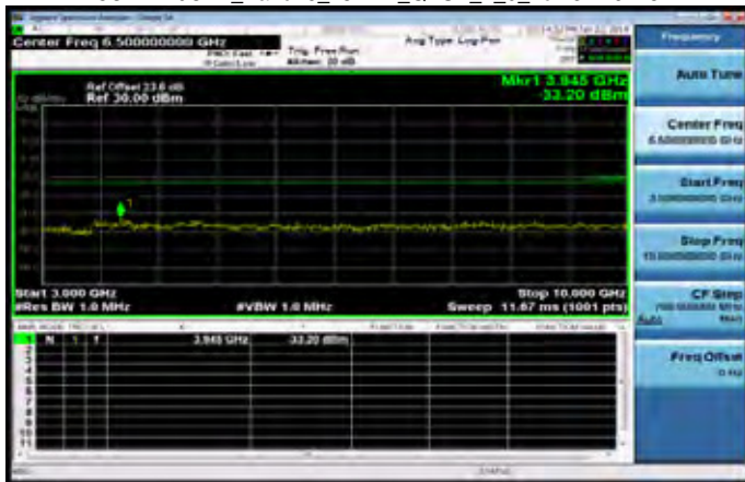
3GHz~10GHz_Band26_15MHz_QPSK_1_0_LowCH26775
