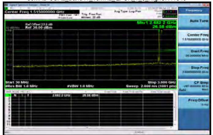
30MHz~3GHz_Band41_10MHz_QPSK_1_0_HighCH41540
