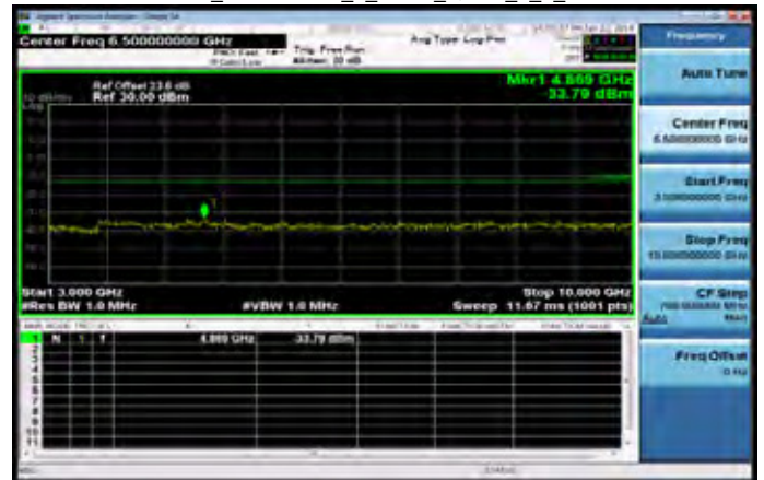
3GHz~10GHz_P90 Band26_1_4MHz_QPSK_1_0_MidCH26740
