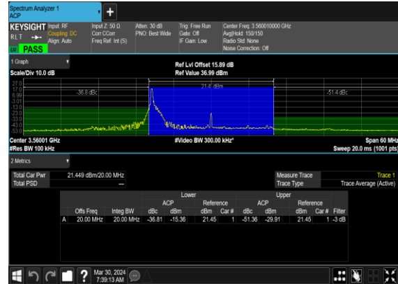
N48(20M)_DFT-s-OFDM_PI_2- BPSK_Edge_1RB_Left_Low_CH
