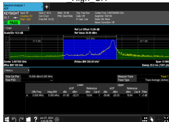
B2_N48(5M)_DFT-s-OFDM_QPSK_Edge_1RB_Right_High_CH
