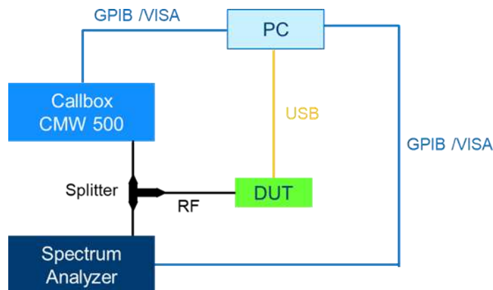
Figure 4-1 - Test Setup
