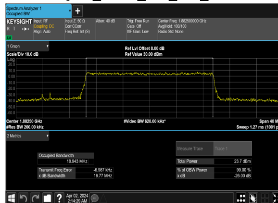
N25(20M)_CP-OFDM_256 QAM_Outer_Full_Mid_CH
