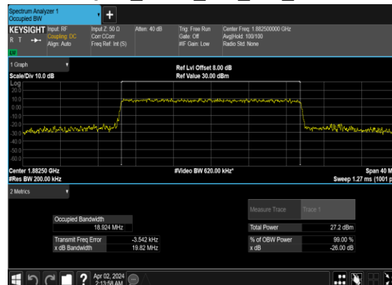
N25(20M)_CP-OFDM_16 QAM_Outer_Full_Mid_CH
