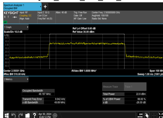
B2_N41(50M)_CP-OFDM_256 QAM_Outter_Full_Mid_CH
