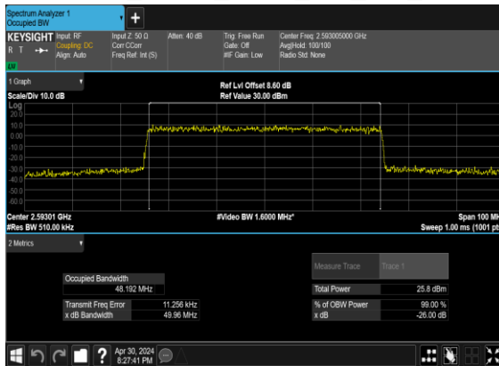
B2_N41(50M)_CP- OFDM_QPSK_Outter_Full_Mid_CH
