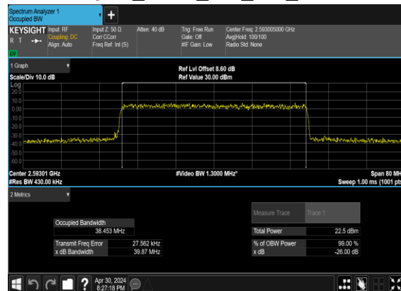
B2_N41(40M)_CP-OFDM_256 QAM_Outter_Full_Mid_CH
