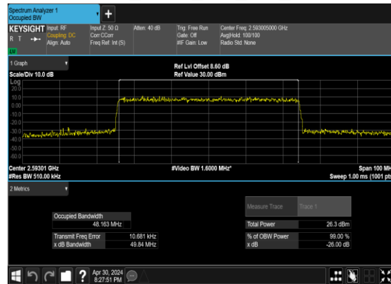
B2_N41(50M)_CP-OFDM_16 QAM_Outter_Full_Mid_CH
