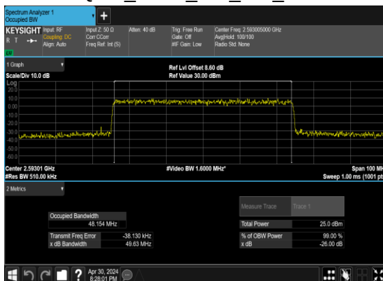
B2_N41(50M)_CP-OFDM_64 QAM_Outter_Full_Mid_CH
