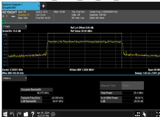
B2_N41(40M)_CP-OFDM_64 QAM_Outter_Full_Mid_CH
