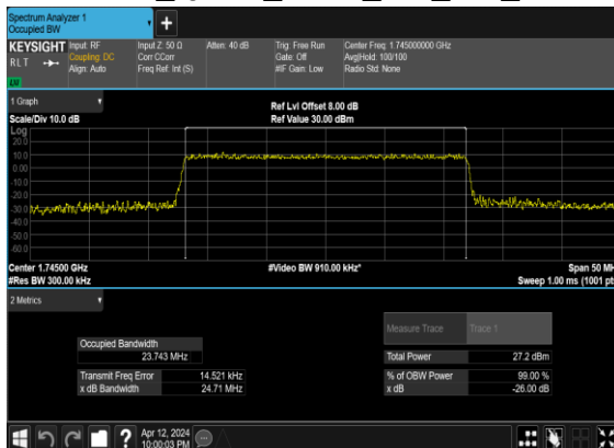
B5_N66(25M)_CP- OFDM_QPSK_Outer_Full_Mid_CH
