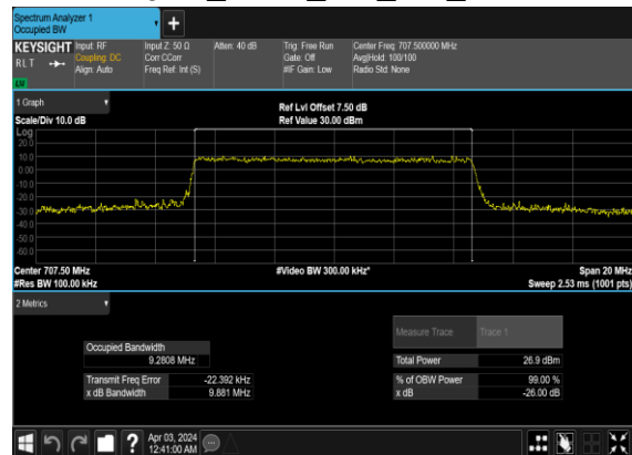
N12(10M)_CP-OFDM_16 QAM_Outer_Full_Mid_CH
