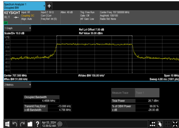
N12(5M)_CP-OFDM_16 QAM_Outer_Full_Mid_CH
