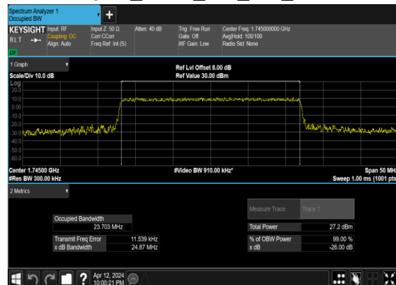
B5_N66(25M)_CP-OFDM_16 QAM_Outer_Full_Mid_CH
