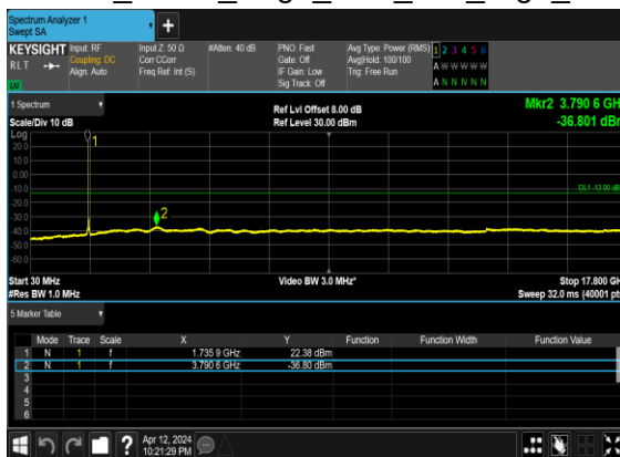
B5_N66(45M)_DFT-s- OFDM_BPSK_Edge_1RB_Left_High_CH
