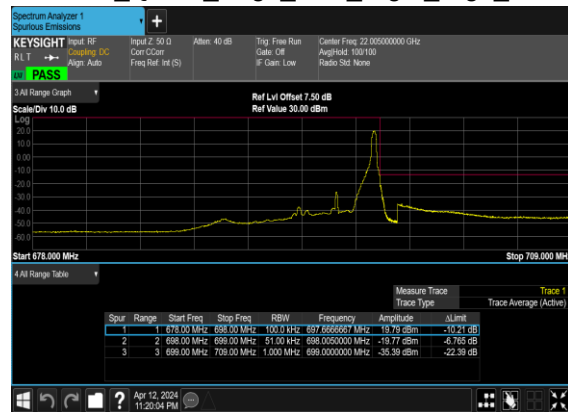
B2_N71(5M)_DFT-s- OFDM_QPSK_Edge_1RB_Right_High_CH
