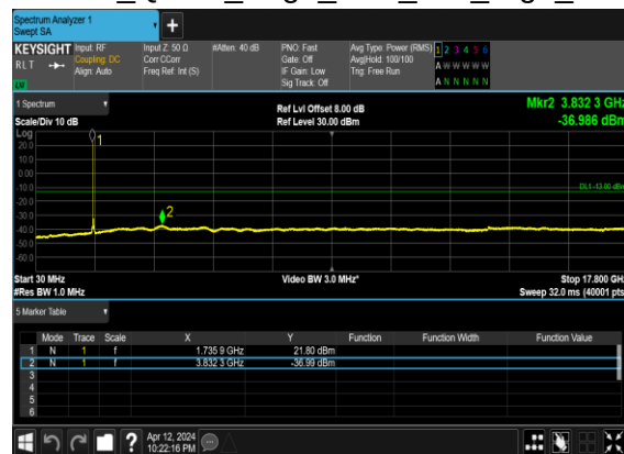
B5_N66(45M)_DFT-s- OFDM_QPSK_Edge_1RB_Left_High_CH
