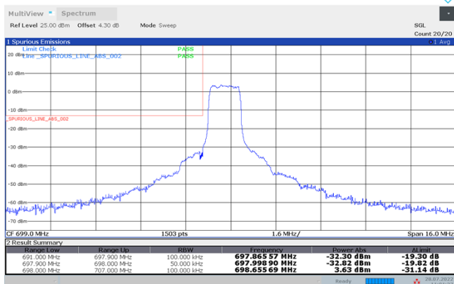
Band85-5MHz-QPSK-L-6RB#0
