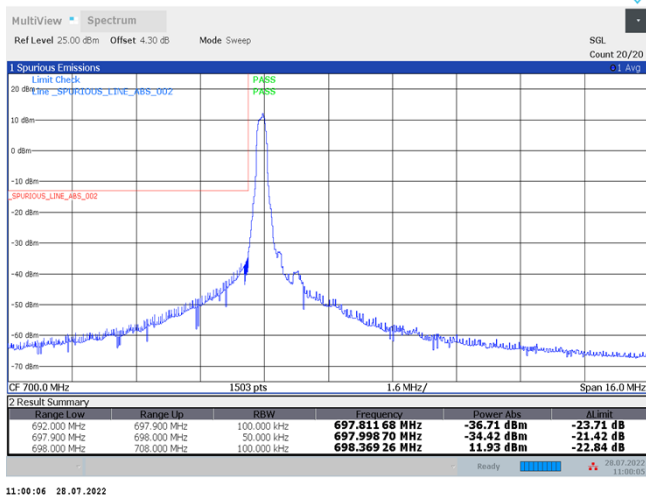
Band85-5MHz-QPSK-L-6RB#0
