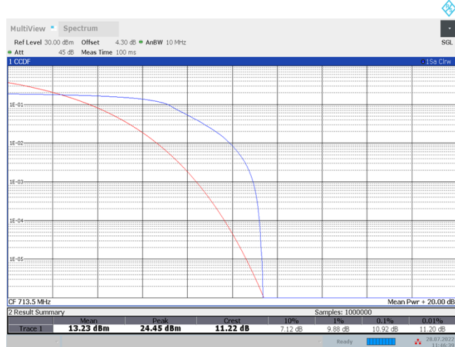
Band85-5MHz-QPSK-23095-50RB#0
