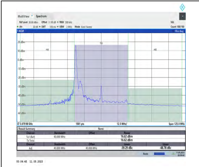
1-N48-PC3-30-40-H-CP-QPSK-Edge_1RB_Left-1@ 0-Ant1-1--PASS-see graph
