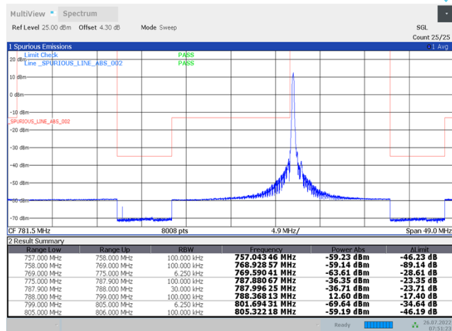
Band14-5MHz-QPSK-23305-6RB#0
