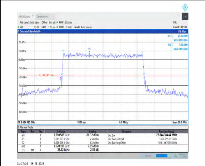
1-N48-PC3-30-30-M-6-CP-QPSK-Outer_Full-78@0- Ant1-27.845-28.920-≤30-PASS
