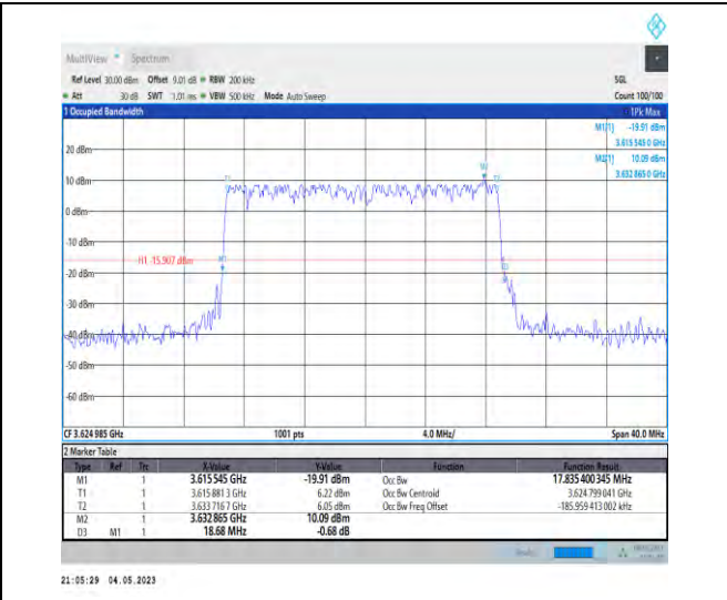
1-N48-PC3-30-20-M-3-DFT-16QAM-Outer_Full-50@ 0-Ant1-17.835-18.680-<=20-PASS
