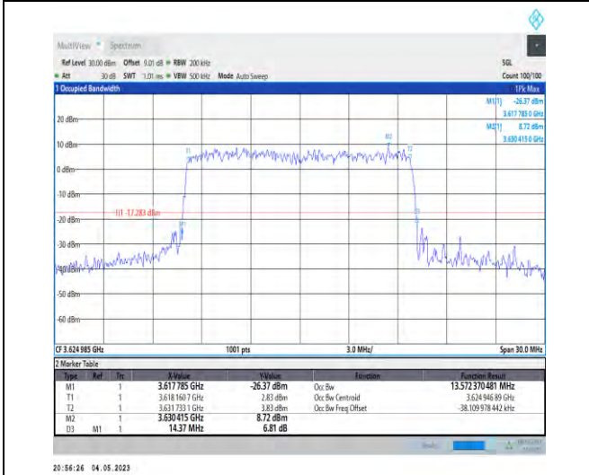
1-N48-PC3-30-15-M-7-CP-16QAM-Outer_Full-38@0 -Ant1-13.572-14.370-≤15-PASS
