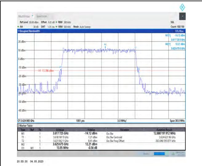
1-N48-PC3-30-15-M-2-DFT-PI2BPSK-Outer_Full-36@0-Ant1-12.88-13.950-≤15-PASS
