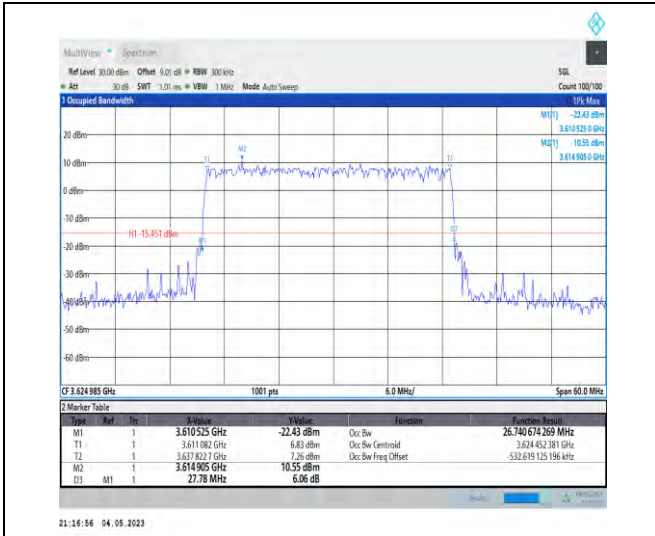
1-N48-PC3-30-30-M-3-DFT-16QAM-Outer_Full-75@ 0-Ant1-26.741-27.780-≤30-PASS
