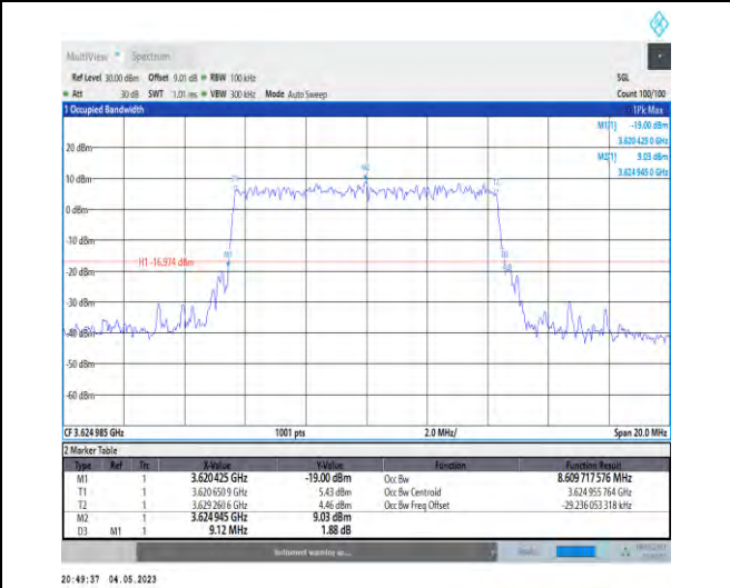
1-N48-PC3-30-10-M-3-DFT-16QAM-Outer_Full-24@ 0-Ant1-8.61-9.120-≤10-PASS
