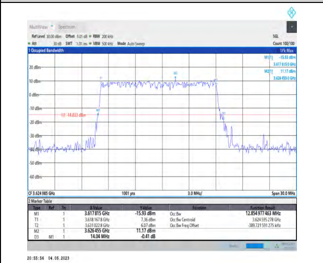
1-N48-PC3-30-15-M-4-DFT-64QAM-Outer_Full-36@0-Ant1-12.855-14.040-≤15-PASS
