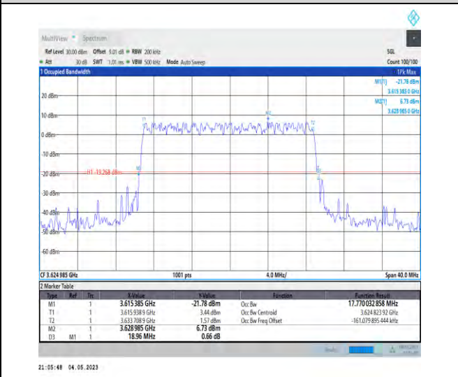
1-N48-PC3-30-20-M-5-DFT-256QAM-Outer_Full-50 @0-Ant1-17.77-18.960-<=20-PASS
