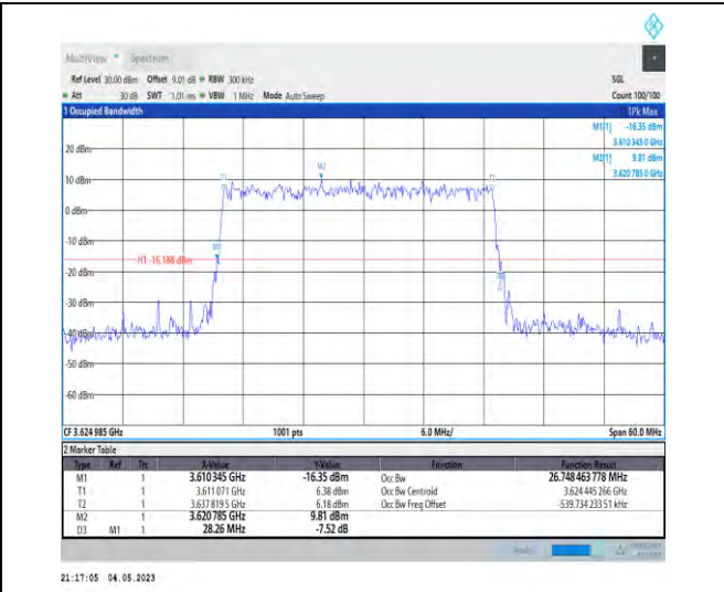
1-N48-PC3-30-30-M-4-DFT-64QAM-Outer_Full-75@ 0-Ant1-26.748-28.260-≤30-PASS
