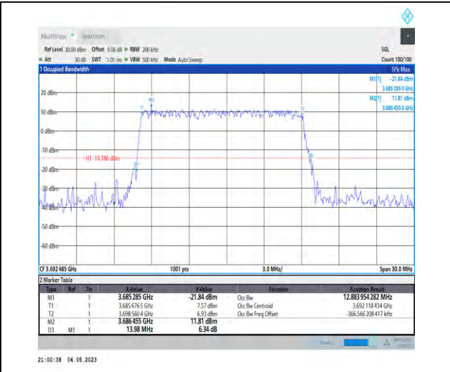
1-N48-PC3-30-15-H-1-DFT-QPSK-Outer_Full-36@0 -Ant1-12.884-13.980-≤15-PASS
