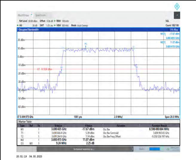
1-N48-PC3-30-10-H-2-DFT-PI2BPSK-Outer_Full-24@0-Ant1-8.598-9.240-≤10-PASS
