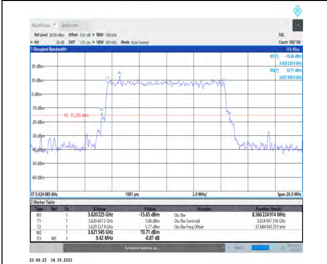
1-N48-PC3-30-10-M-2-DFT-PI2BPSK-Outer_Full-24 @0-Ant1-8.56-9.420-≤10-PASS
