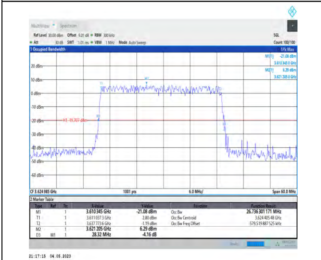
1-N48-PC3-30-30-M-5-DFT-256QAM-Outer_Full-75 @0-Ant1-26.736-28.320-≤30-PASS
