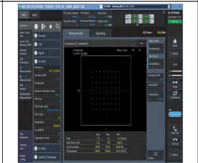
1-N48-PC3-30-40-M-4-DFT-64QAM-Outter_Full-100 @0-Ant1-see graph-PASS
