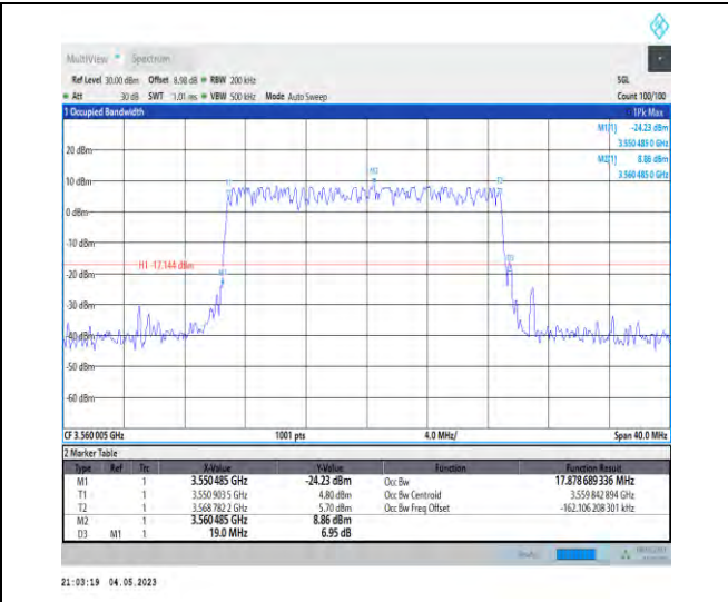
1-N48-PC3-30-20-L-4-DFT-64QAM-Outer_Full-50@ 0-Ant1-17.879-19.000-<=20-PASS
