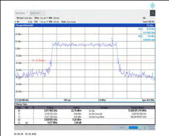
1-N48-PC3-30-15-M-8-CP-64QAM-Outer_Full-38@0 -Ant1-13.601-14.370-≤15-PASS
