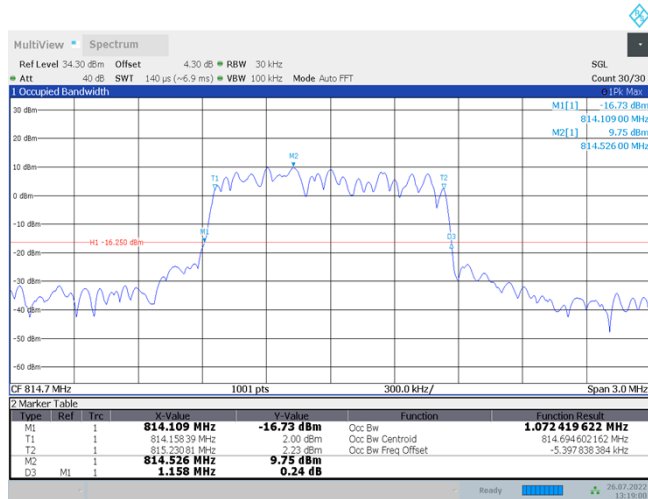
Band26-1.4MHz-QPSK-26697-6RB#0
