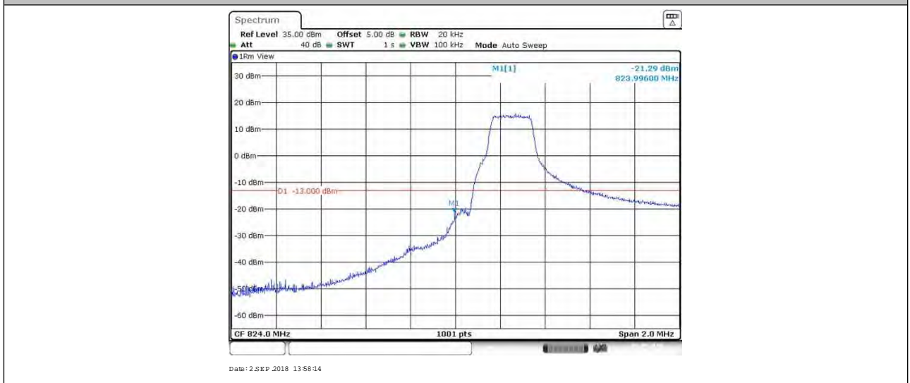
BAND 26_1.4MHz_16QAM_26797_6RB#0
