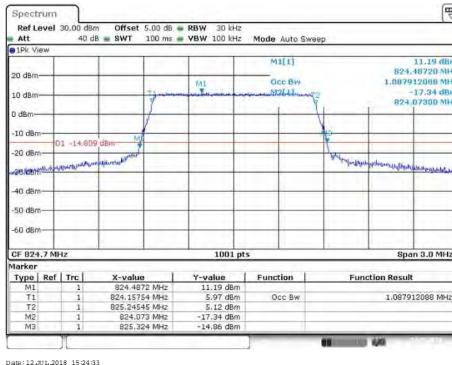
BAND26_1.4MHz_64QAM_26915_6RB#0
