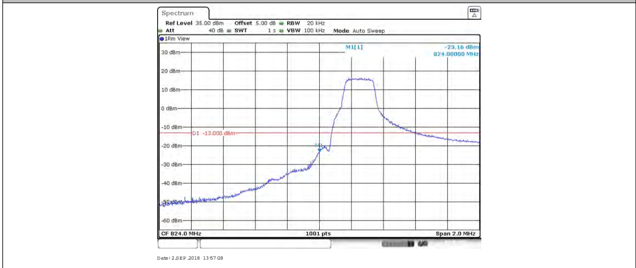
BAND 26_10MHz_QPSK_26840_50RB#0
