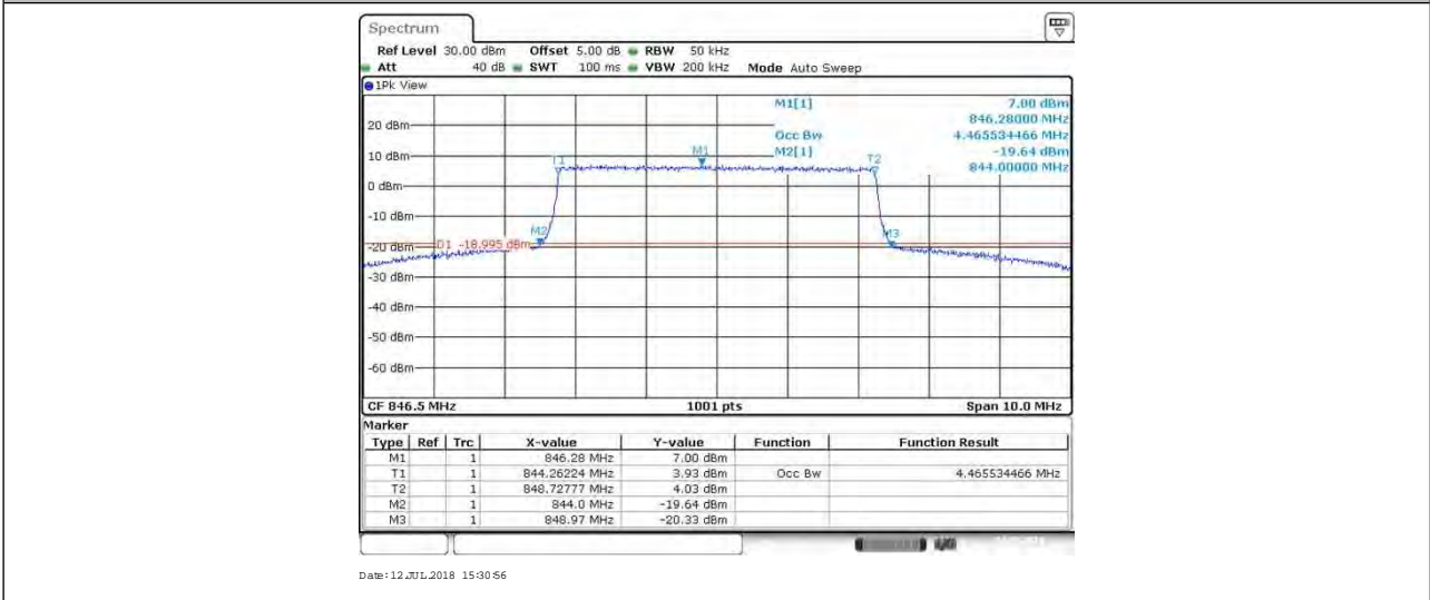
BAND26_5MHz_16QAM_26815_25RB#0
