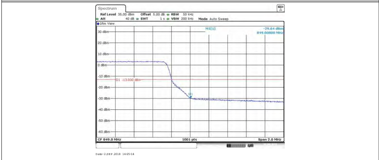
BAND 26_5MHz_64QAM_26815_1RB#0
