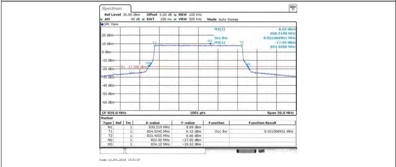
BAND26_10MHz_16QAM_26915_50RB#0
