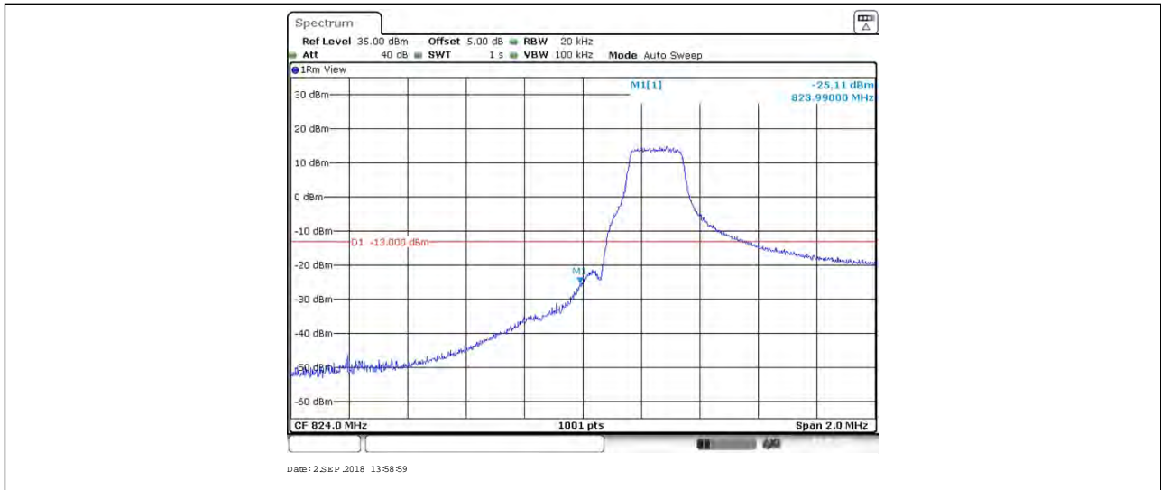
BAND 26_10MHz_64QAM_26840_50RB#0
