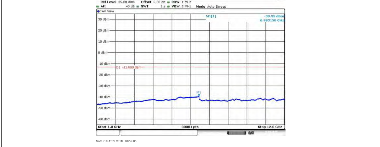
BAND 26_15MHz_64QAM_26915_1RB#0
