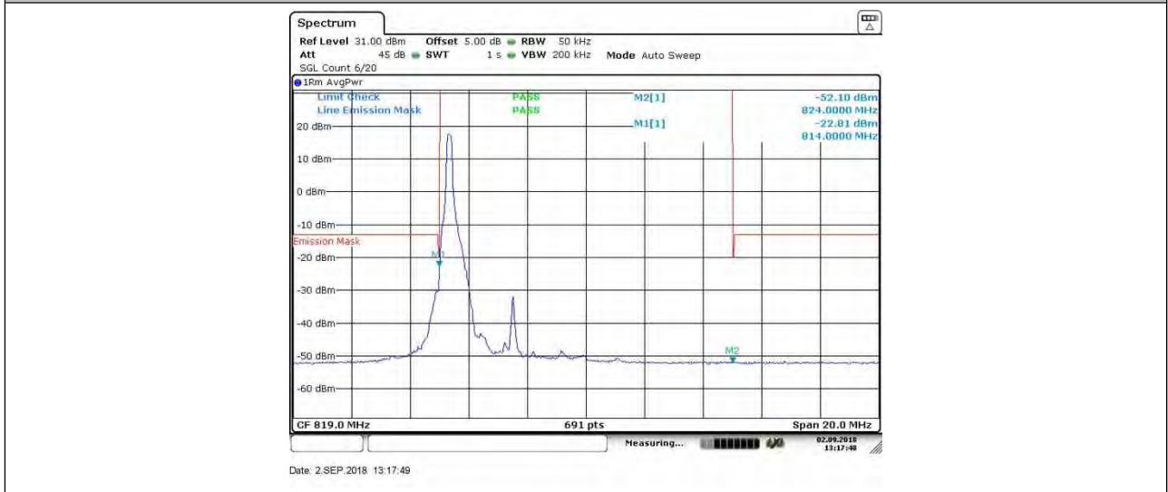
BAND 26_5MHz_16QAM_26715_25RB#0
