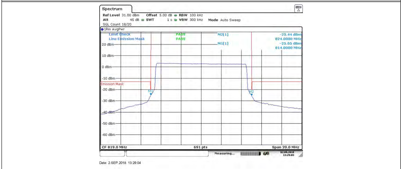
BAND 26_10MHz_16QAM_26740_1RB#0
