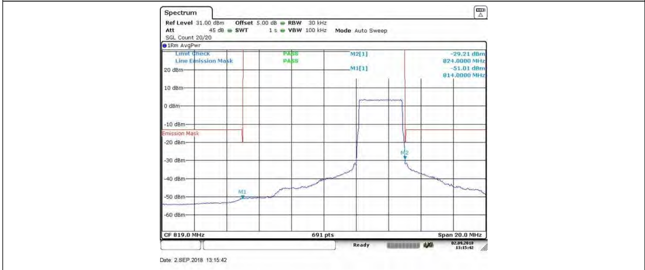
BAND 26_3MHz_16QAM_26705_1RB#0
