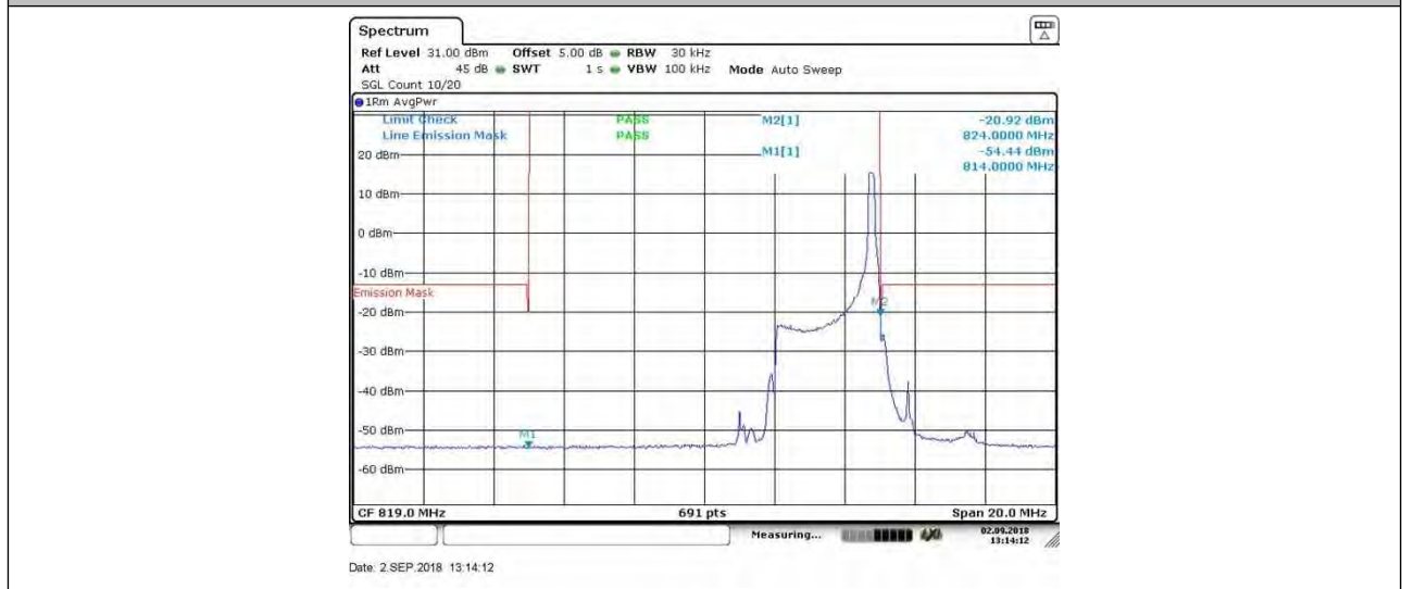
BAND 26_3MHz_16QAM_26775_15RB#0
