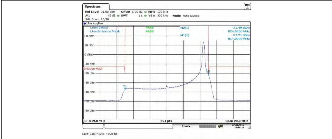
BAND 26_10MHz_16QAM_26740_50RB#0
