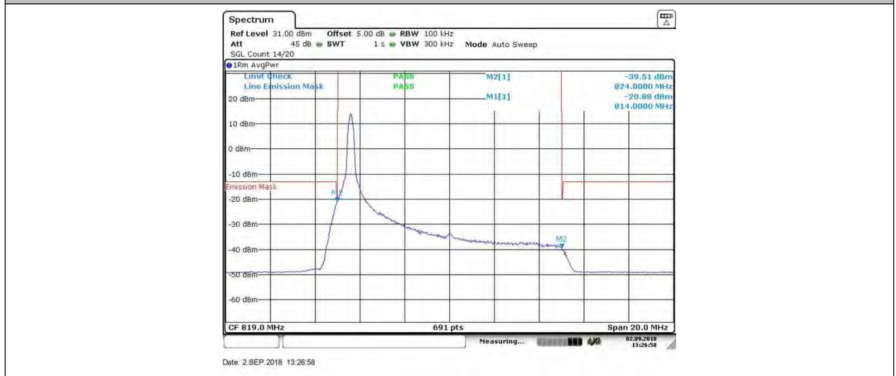
BAND 26_10MHz_QPSK_26740_50RB#0
