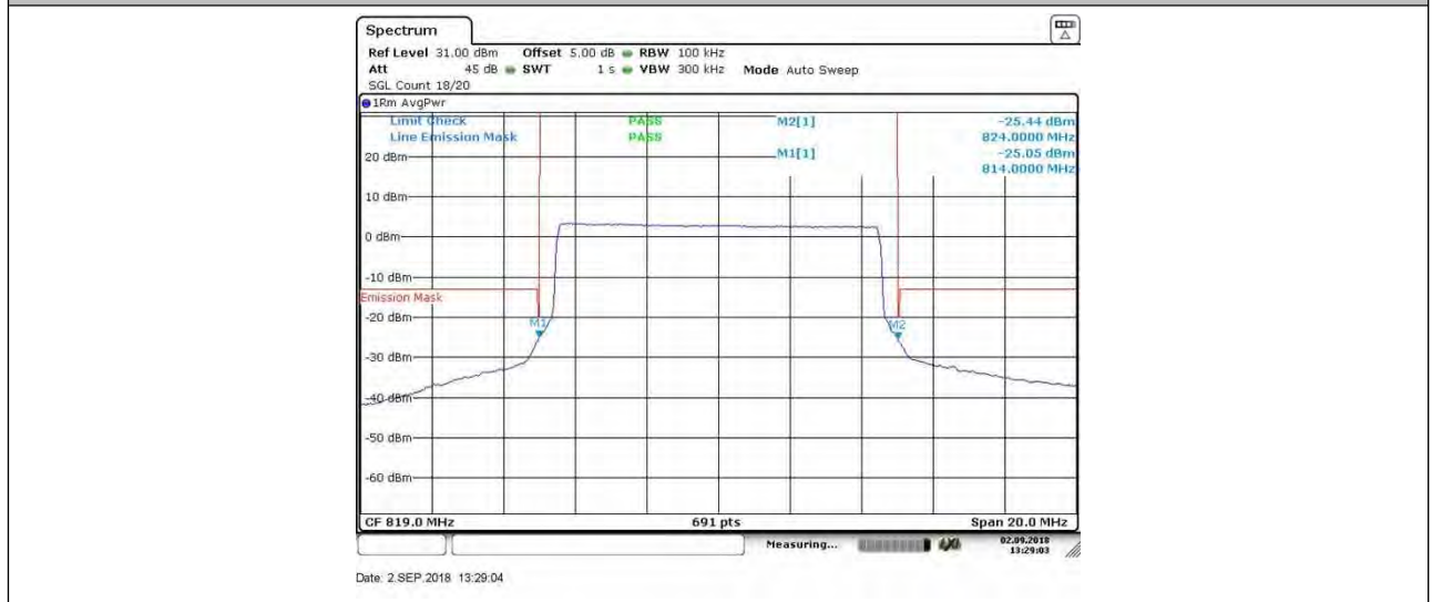
BAND 26_10MHz_QPSK_26740_1RB#49
