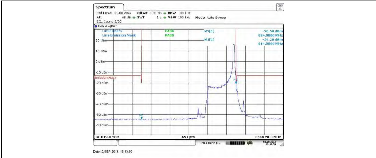
BAND 26_3MHz_QPSK_26775_15RB#0
