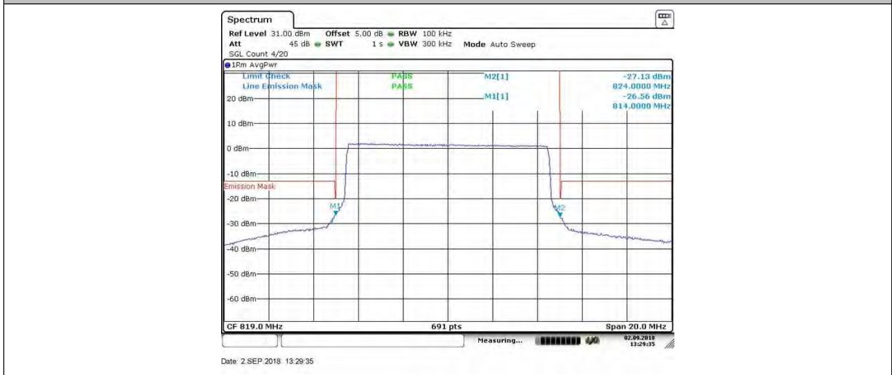
BAND 26_10MHz_64QAM_26740_1RB#49
