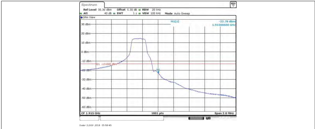
BAND25_1.4MHz_QPSK_26683_6RB#0
