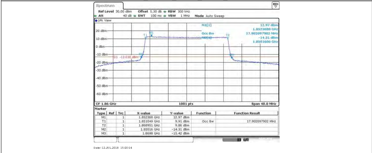
BAND25_20MHz_QPSK_26365_100RB#0
