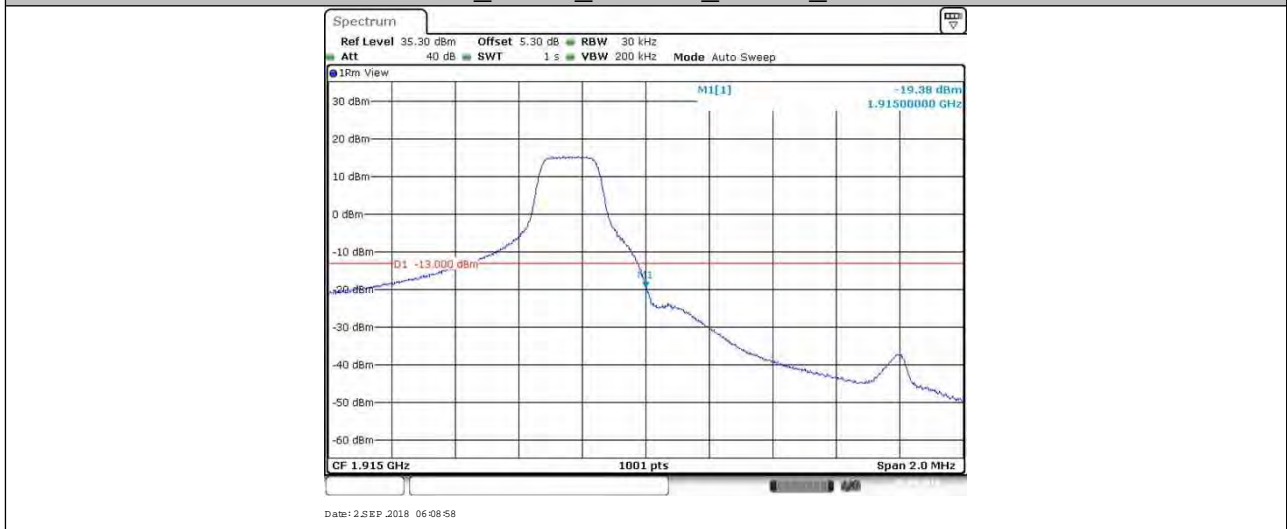
BAND25_3MHz_16QAM_26675_15RB#0
