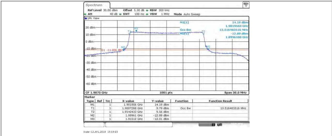
BAND25_15MHz_64QAM_26115_75RB#0
