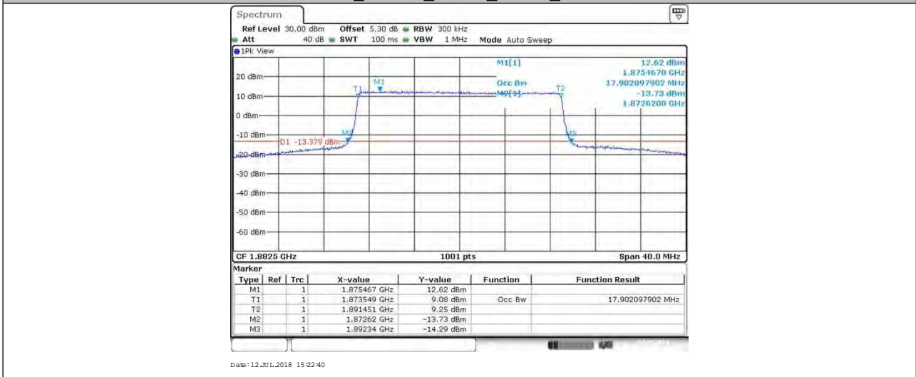
BAND25_20MHz_QPSK_26590_100RB#0
