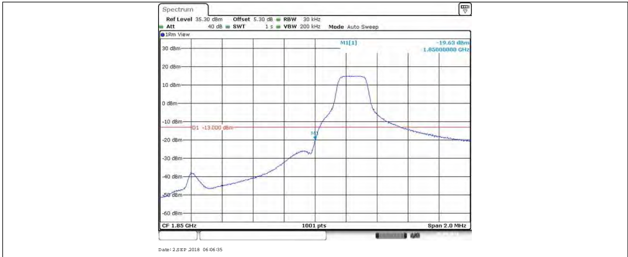
BAND25_3MHz_16QAM_26055_15RB#0
