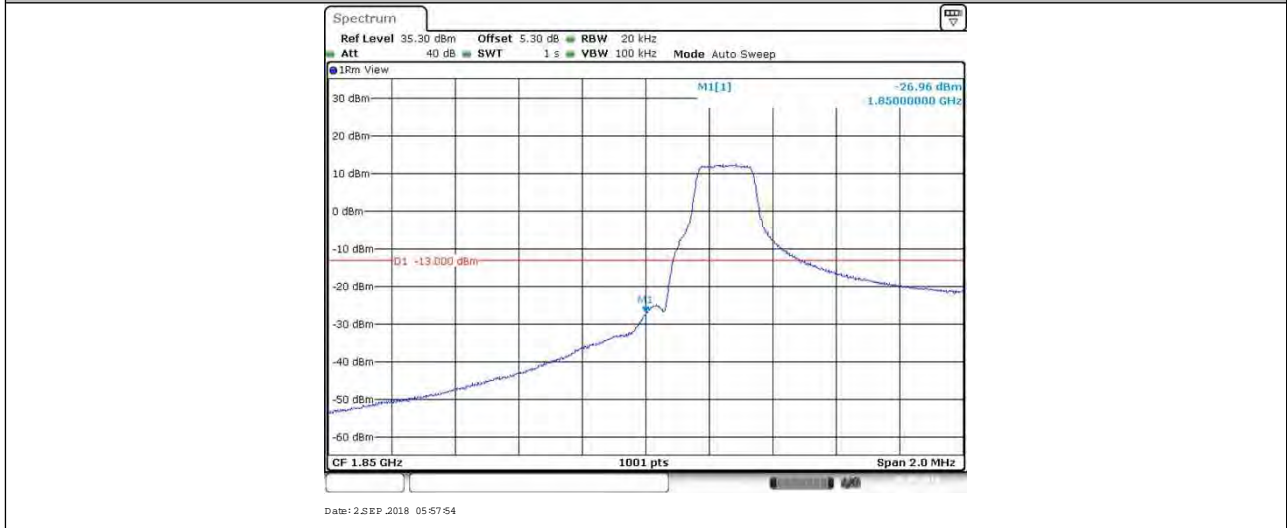
BAND25_1.4MHz_64QAM_26047_6RB#0
