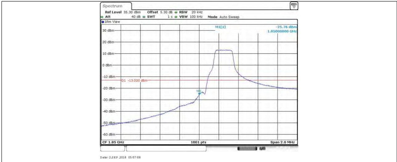
BAND25_1.4MHz_16QAM_26047_6RB#0
