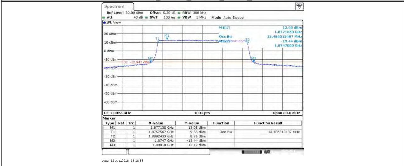
BAND25_15MHz_16QAM_26615_75RB#0
