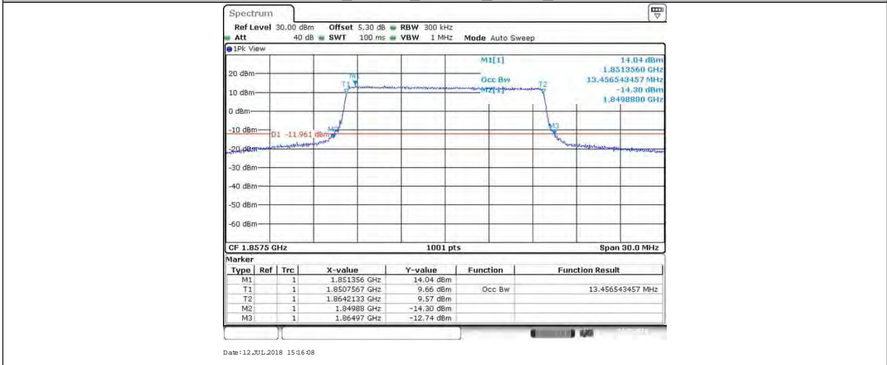
BAND25_15MHz_16QAM_26365_75RB#0
