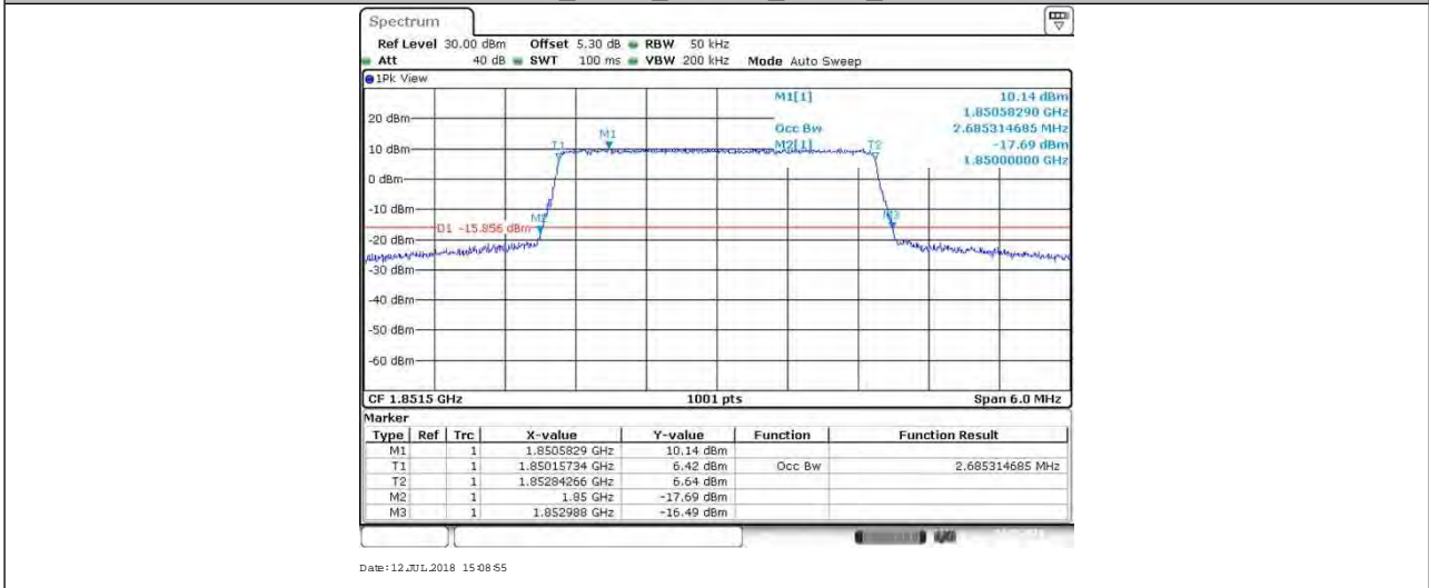
BAND25_3MHz_16QAM_26365_15RB#0
