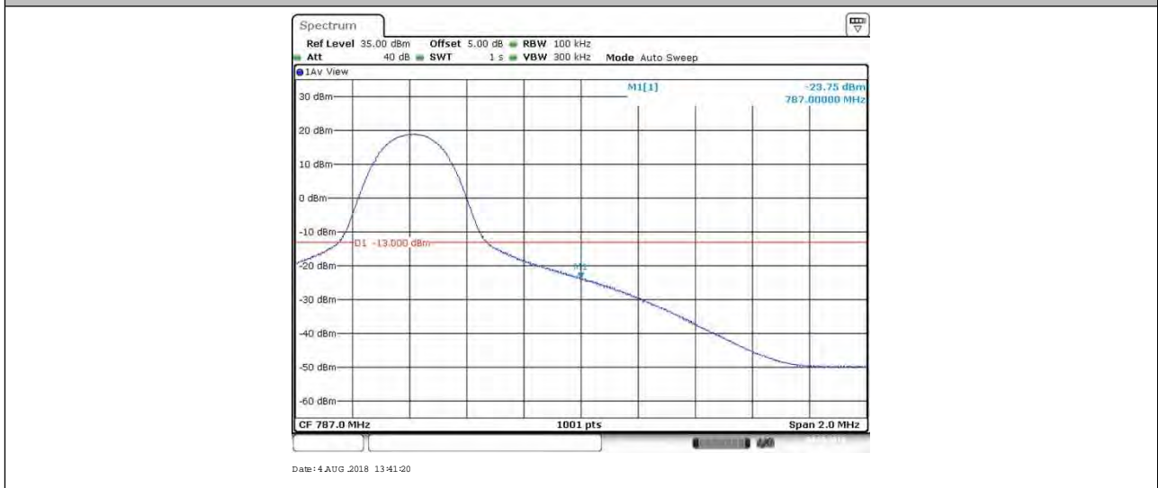
BAND13_10MHz_64QAM_23230_50RB#0
