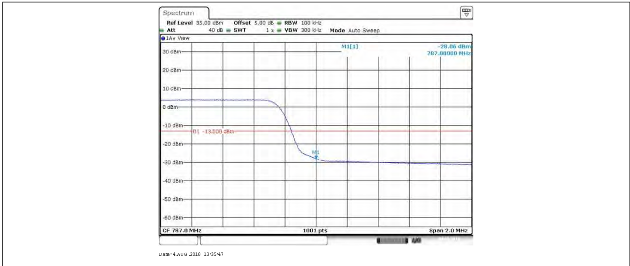
BAND13_10MHz_QPSK_23230_1RB#0
