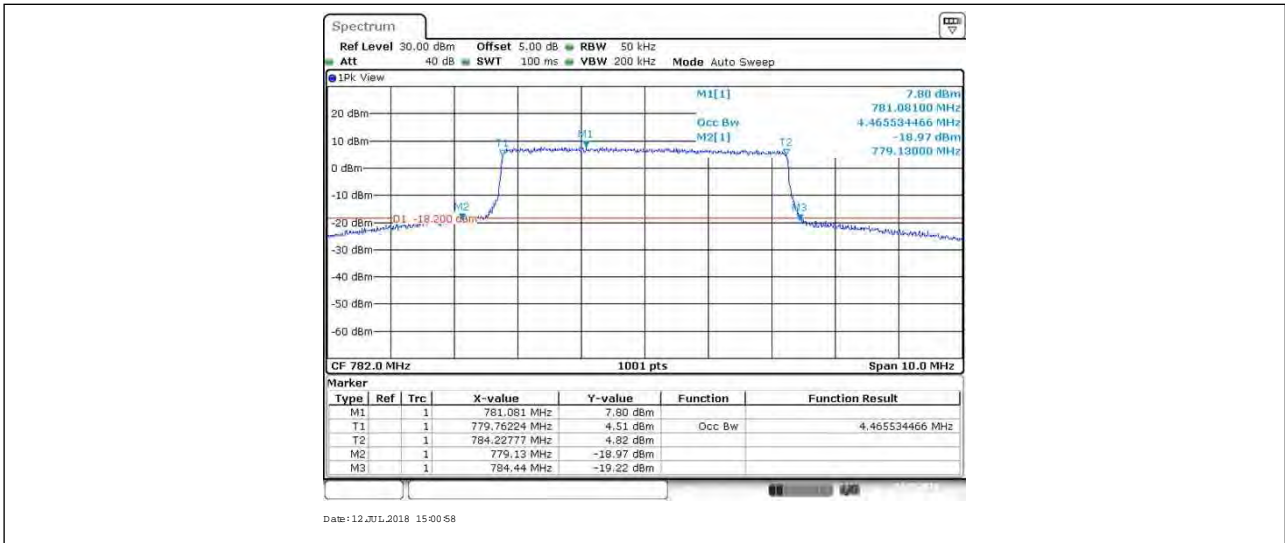
BAND13_5MHz_64QAM_23255_25RB#0
