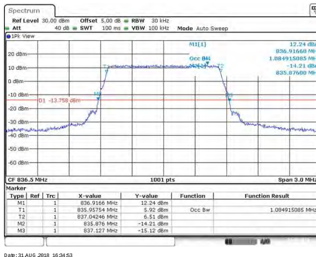
BAND5_1.4MHz_QPSK_20643_6RB#0
