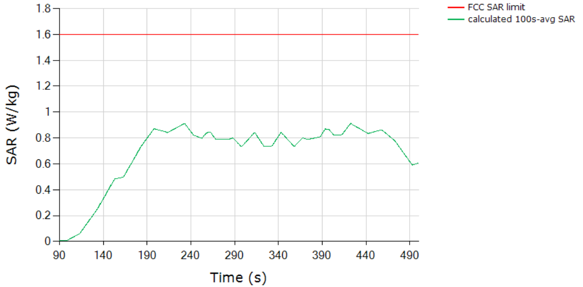
SAR (Test Sequence 2) Tech: LTE, Band 12
