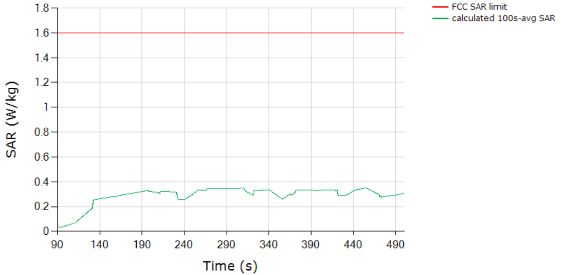
SAR (Test Sequence 2) Tech: NRSUB6, Band 41
