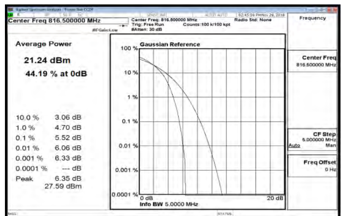
LTE_Band26_Part90s_5MHz_64QAM_25_0_LowCH26715
