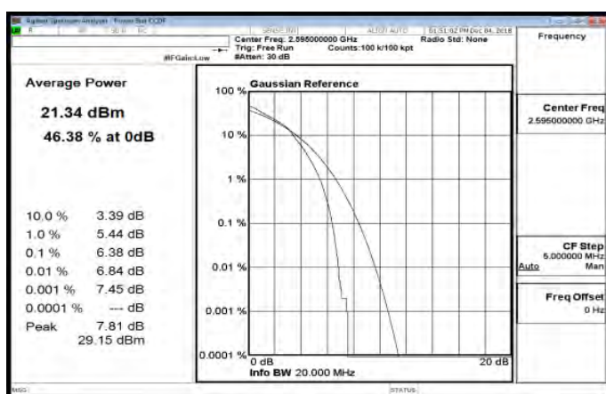
LTE_Band38_15MHz_64QAM_75_0_MidCH38000-2595
