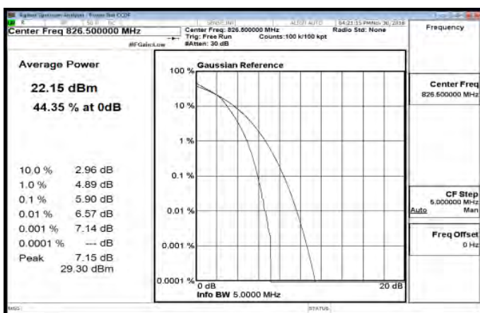
LTE_Band26_5MHz_64QAM_25_0_LowCH26815-826.5
