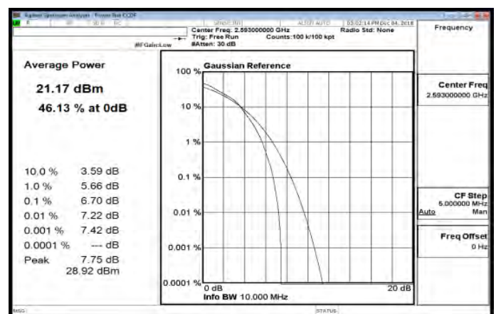
LTE_Band41_10MHz_64QAM_50_0_MidCH40620-2593
