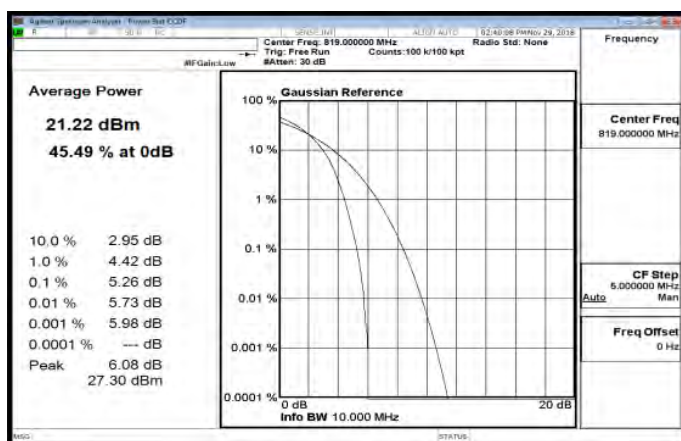
LTE_Band26_Part90s_10MHz_64QAM_50_0_MidCH26740
