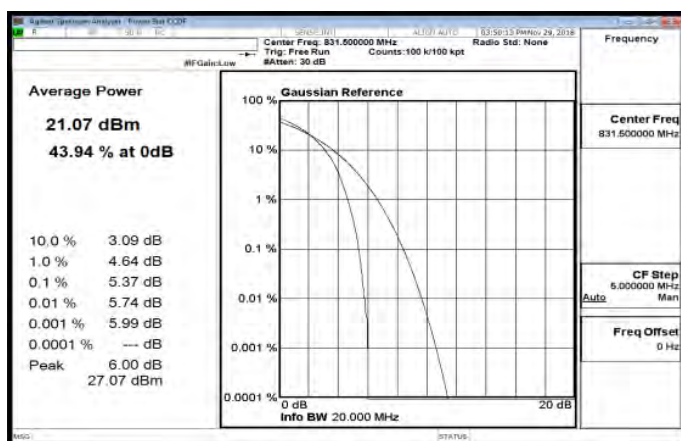
LTE_Band26_15MHz_64QAM_75_0_LowCH26865
