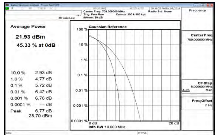
LTE_Band17_10MHz_64QAM_50_0_LowCH23780-709
