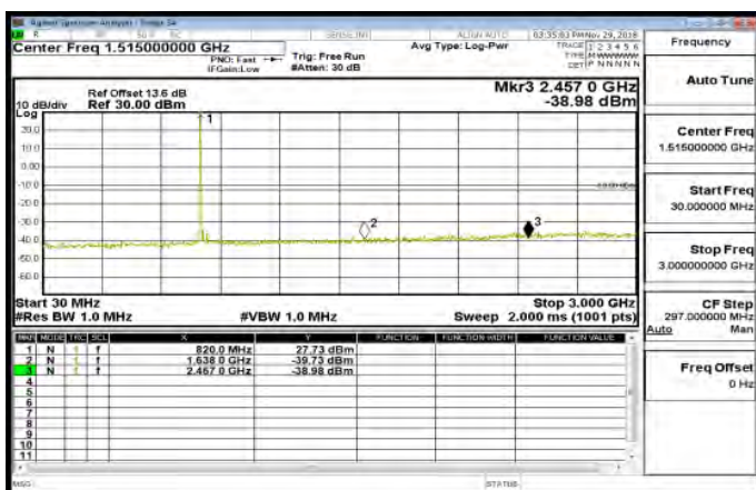
30MHz~3GHz_Band26_Part90s_1_4MHz_QPSK_1_0_MidCH26740
