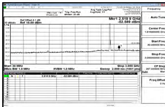
30MHz~3GHz_Band30_5MHz_QPSK_1_0_LowCH27685
