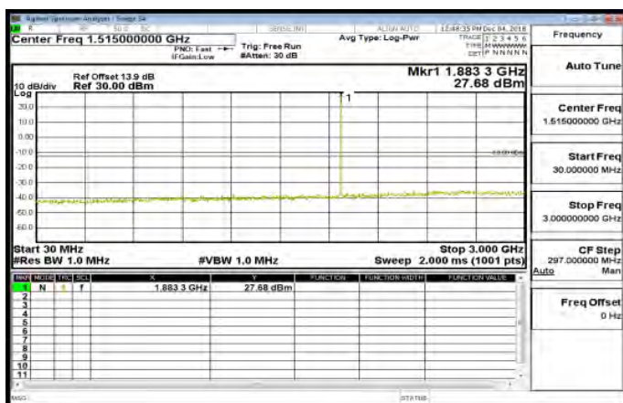
30MHz~3GHz_Band25_1_4MHz_QPSK_1_0_MidCH26365-1882.5
