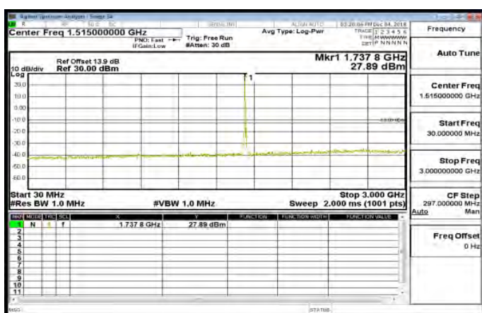
30MHz-3GHz_Band66_20MHz_QPSK_1_0_MidCH132322-1745
