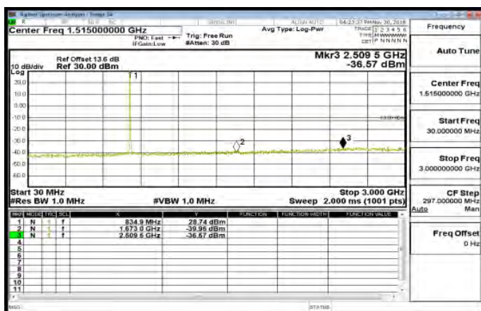
30MHz~3GHz_Band26_5MHz_QPSK_1_0_MidCH26915-836.5
