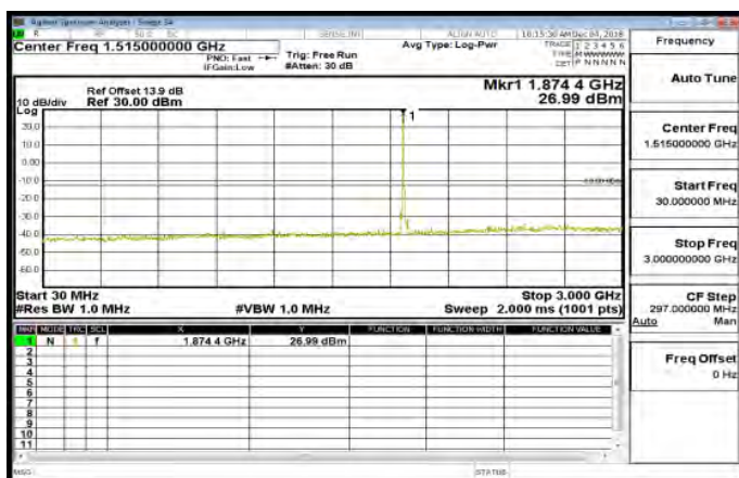
30MHz~3GHz_Band25_20MHz_QPSK_1_0_MidCH26365-1882.5
