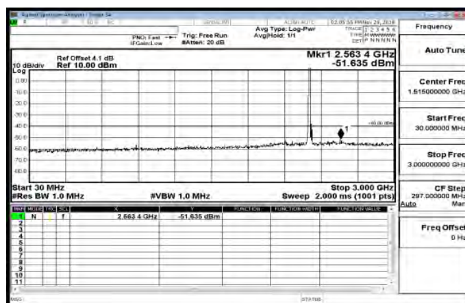
30MHz~3GHz_Band30_5MHz_QPSK_1_0_MidCH27710
