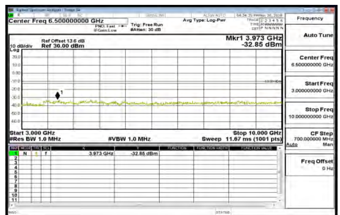
3GHz~10GHz_Band26_3MHz_QPSK_1_0_HighCH27025-847.5
