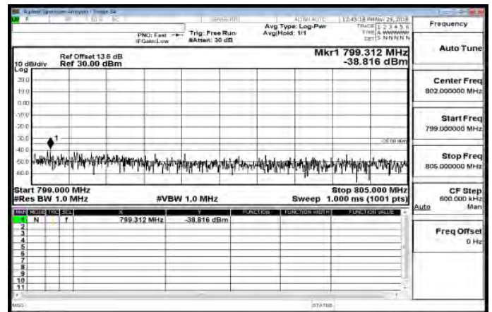
799MHz-805MHz_Band14_10MHz_QPSK_1_0_MidCH23330
