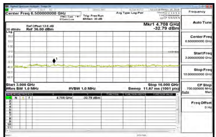
3GHz~10GHz_Band26_Part90s_3MHz_QPSK_1_0_HighCH26775
