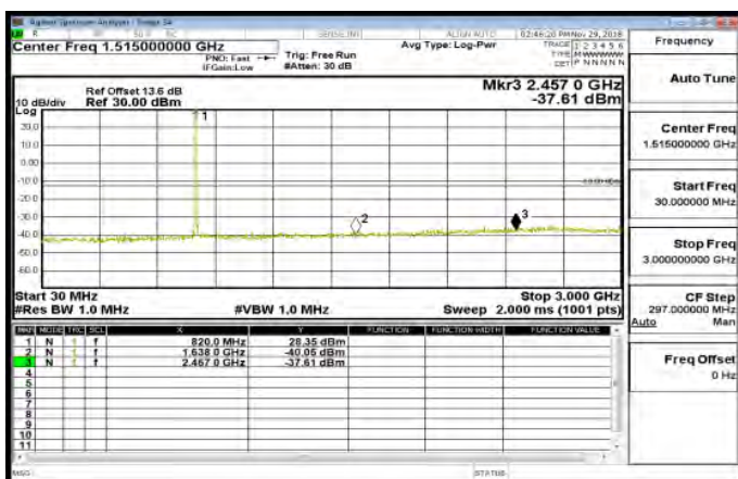
30MHz~3GHz_Band26_Part90s_5MHz_QPSK_1_0_MidCH26740
