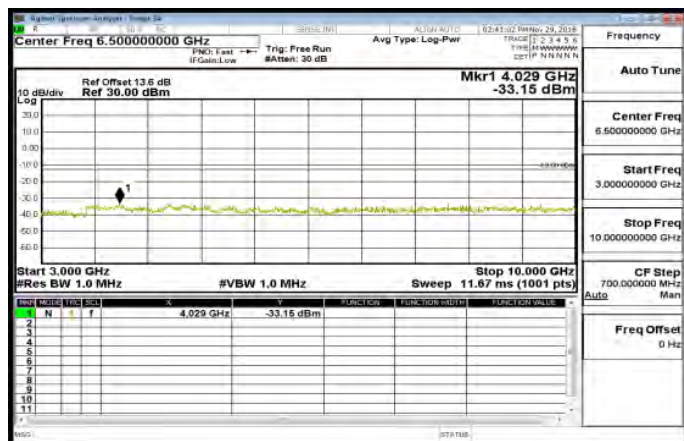
3GHz~10GHz_Band26_Part90s_10MHz_QPSK_1_0_MidCH26740
