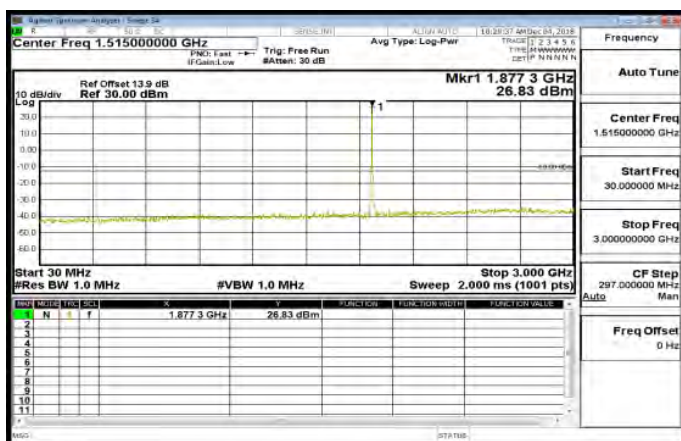
30MHz~3GHz_Band25_15MHz_QPSK_1_0_MidCH26365-1882.5
