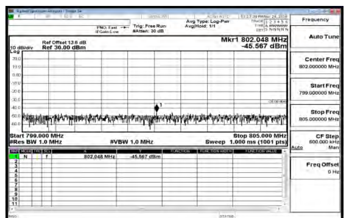
799MHz-805MHz_Band14_5MHz_QPSK_1_0_MidCH23330
