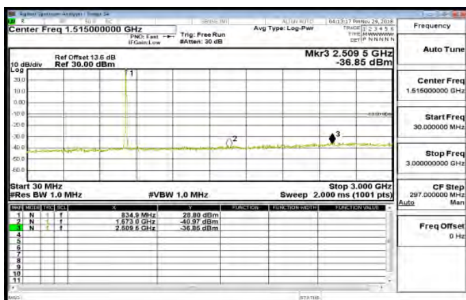
30MHz~3GHz_Band26_10MHz_QPSK_1_0_MidCH26915
