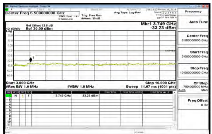
3GHz~10GHz_Band14_5MHz_QPSK_1_0_HighCH23355
