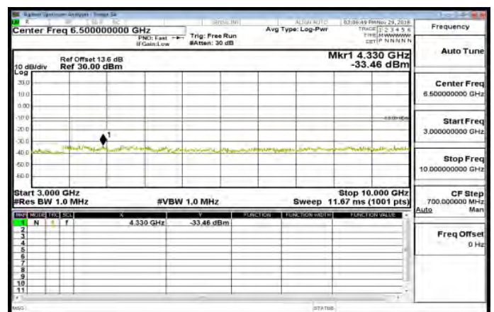
3GHz~10GHz_Band26_Part90s_5MHz_QPSK_1_0_HighCH26765
