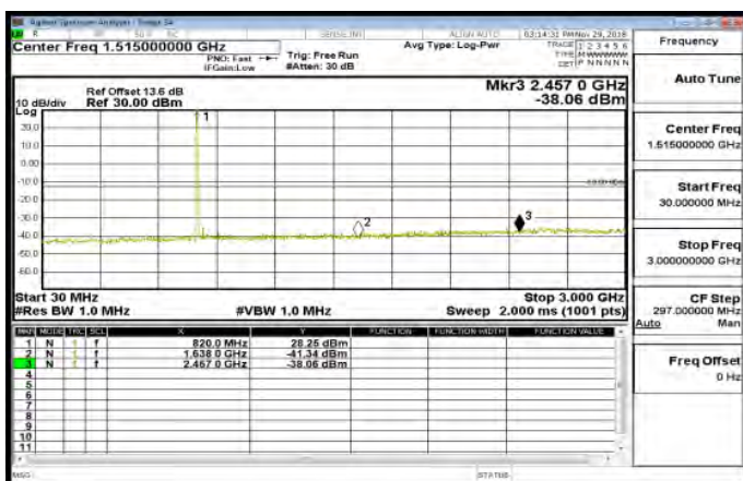
30MHz~3GHz_Band26_Part90s_3MHz_QPSK_1_0_MidCH26740
