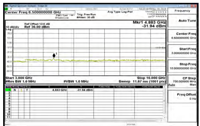
3GHz~10GHz_Band26_5MHz_QPSK_1_0_HighCH27015-846.5
