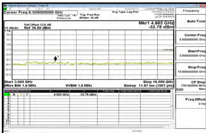
769MHz-775MHz_Band14_5MHz_QPSK_1_0_LowCH23305
