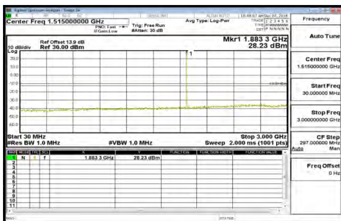
30MHz~3GHz_Band25_5MHz_QPSK_1_0_MidCH26365-1882.5
