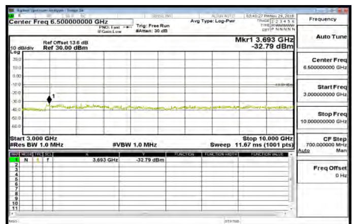
3GHz~10GHz_Band26_Part90s_1_4MHz_QPSK_1_0_HighCH26783
