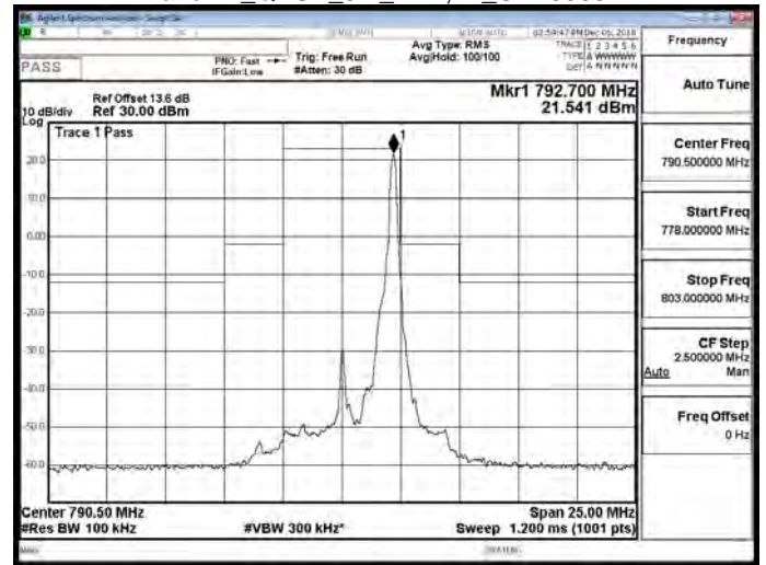
Band 14_QPSK_5M_RB1,24_CH23330
