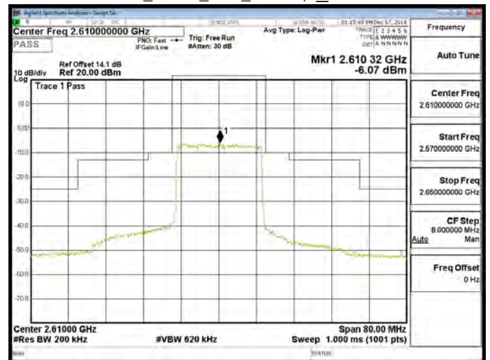
Band 38_QPSK_20M_RB100,0_CH38150
