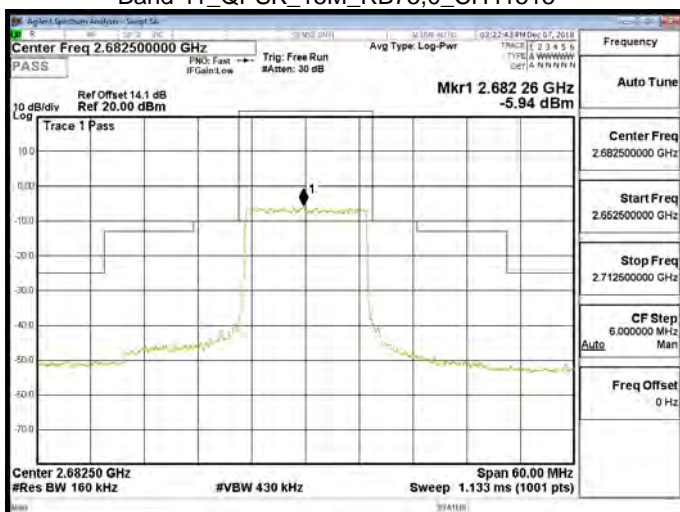
Band 41_QPSK_15M_RB75.0_CH41515
