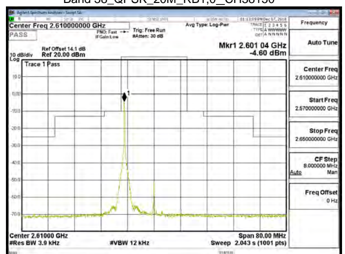
Band 38_QPSK_20M_RB1,0_CH38150
