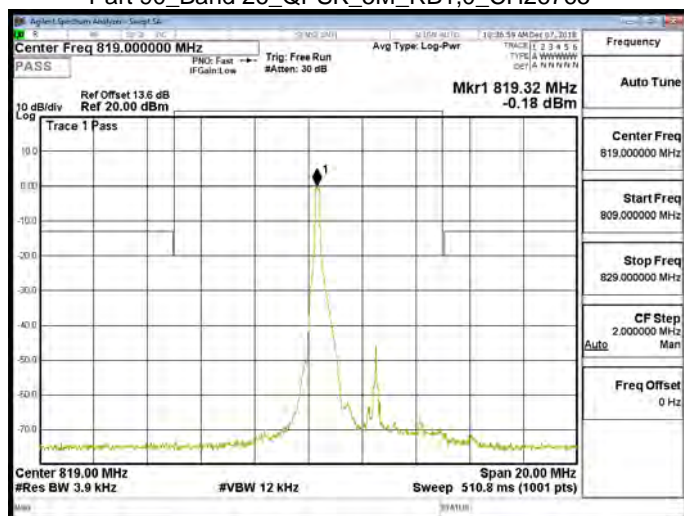
Part 90_Band 26_QPSK_5M_RB1,0_CH26765
