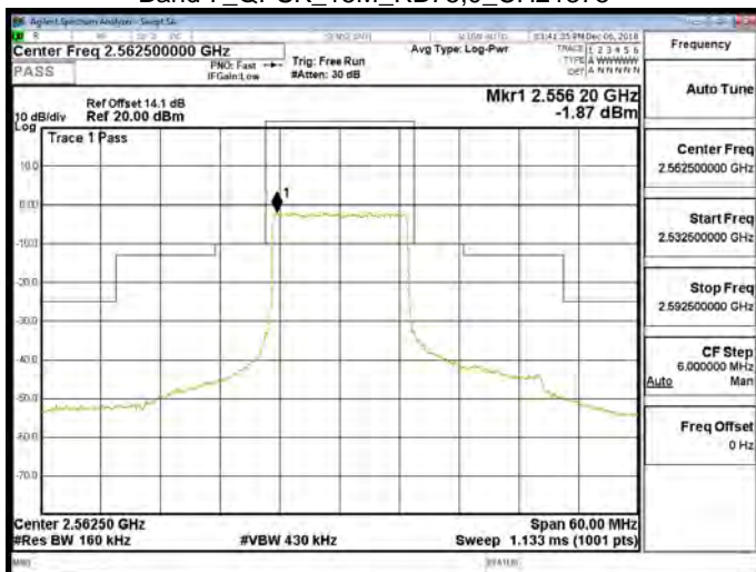
Band 7_QPSK_15M_RB75,0_CH21375
