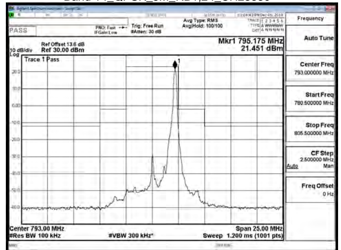
Band 14_QPSK_5M_RB1,24_CH23355
