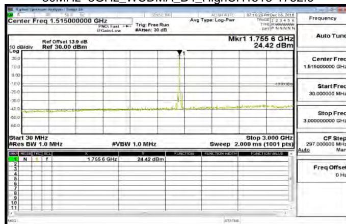
30MHz~3GHz_WCDMA_B4_HighCH1513-1752.6
