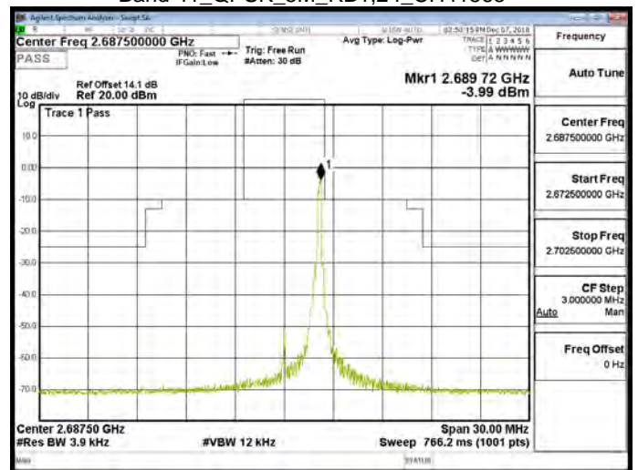
Band 41_QPSK_5M_RB1,24_CH41565
