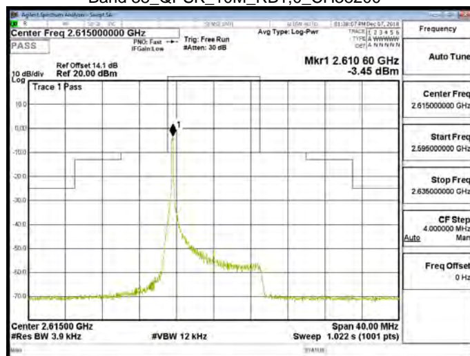
Band 38_QPSK_10M_RB1,0_CH38200
