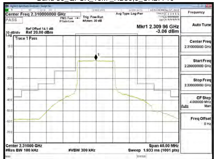
Band 30_QPSK_10M_RB50,0_CH27710
