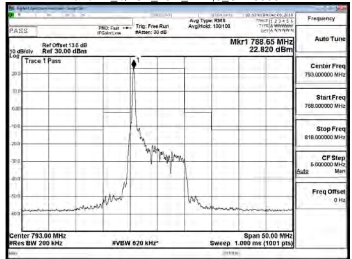
Band 14_QPSK_10M_RB1,49_CH23330
