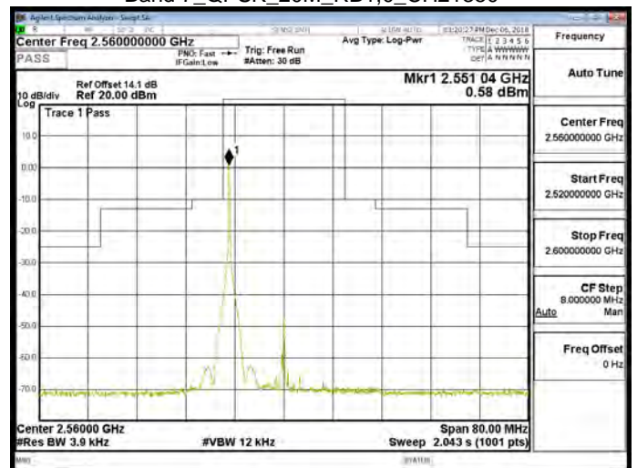
Band 7_QPSK_20M_RB1,0_CH21350
