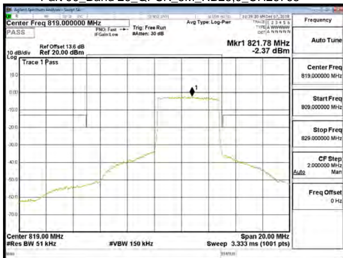
Part 90_Band 26_QPSK_5M_RB25,0_CH26765
