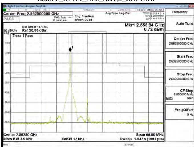
Band 7_QPSK_15M_RB1,0_CH21375
