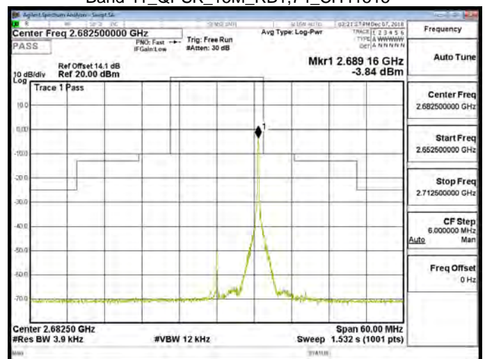
Band 41_QPSK_15M_RB1,74_CH41515
