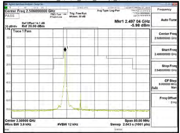
Band 41_QPSK_20M_RB1.0_CH40620
