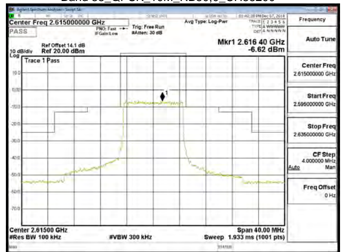
Band 38_QPSK_10M_RB50,0_CH38200
