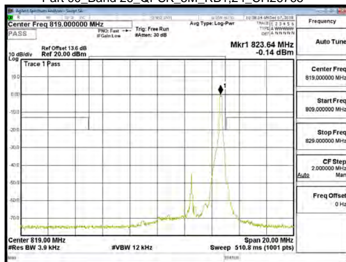
Part 90_Band 26_QPSK_5M_RB1,24_CH26765
