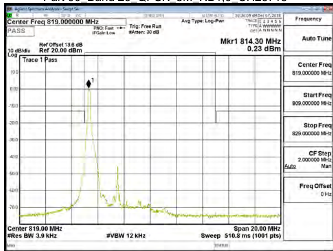
Part 90_Band 26_QPSK_5M_RB1,0_CH26740
