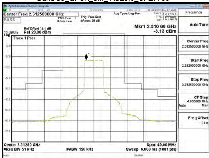
Band 30_QPSK_5M_RB25,0_CH27735
