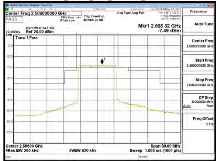
Band 41_QPSK_20M_RB100,0_CH40620
