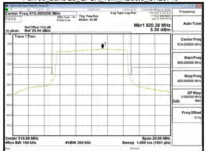
Part 90_Band 26_QPSK_10M_RB50,0_CH26740
