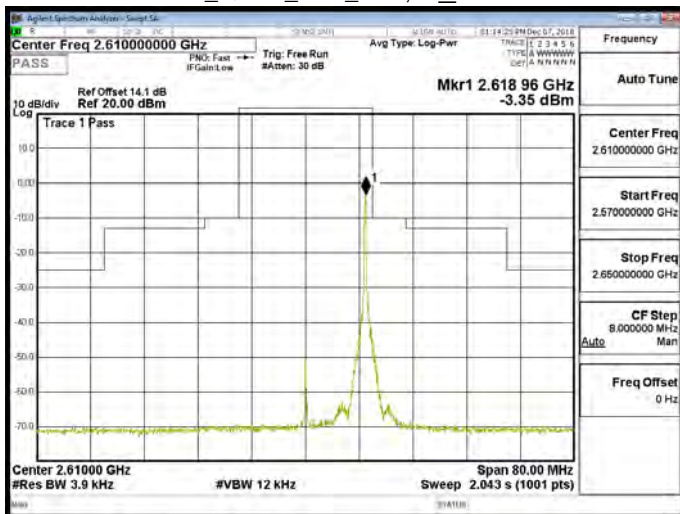
Band 38_QPSK_20M_RB1,99_CH38150
