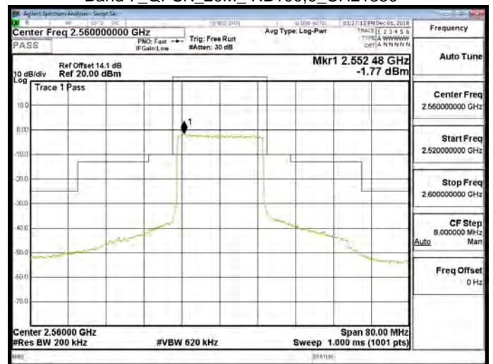
Band 7_QPSK_20M_RB100,0_CH21350
