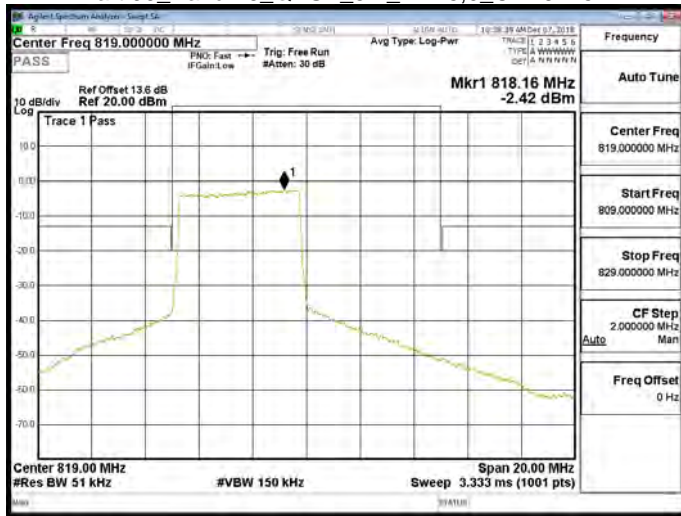
Part 90_Band 26_QPSK_5M_RB25,0_CH26740
