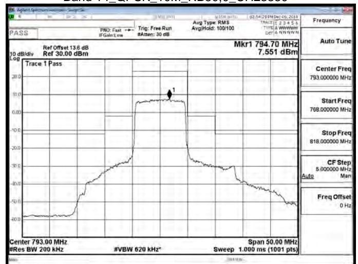
Band 14_QPSK_10M_RB50,0_CH23330
