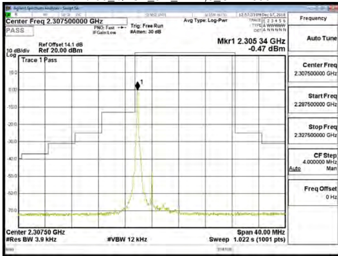
Band 30_QPSK_5M_RB1,0_CH27710
