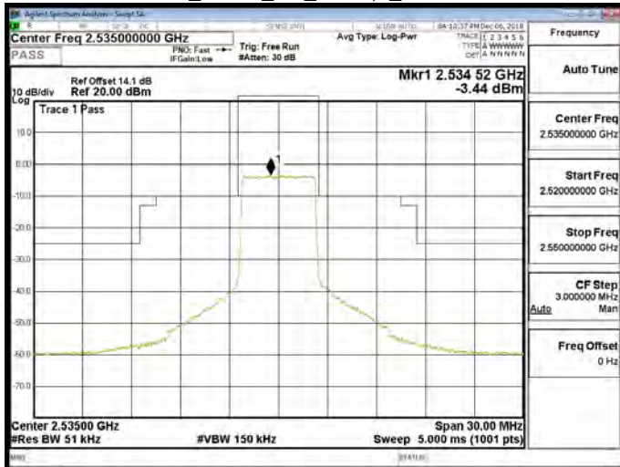
Band 7_QPSK_5M_RB25,0_CH21425
