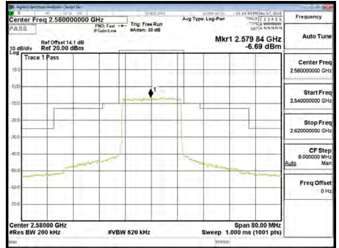
Band 38_QPSK_20M_RB100,0_CH38000
