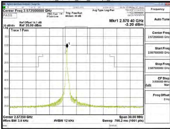
Band 38_QPSK_5M_RB1,0_CH38000
