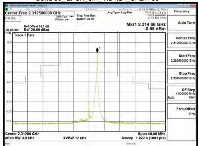
Band 30_QPSK_5M_RB1,24_CH27735
