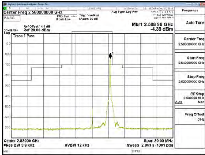
Band 38_QPSK_20M_RB1,99_CH38000
