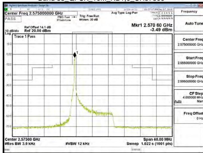
Band 38_QPSK_10M_RB1,0_CH38000
