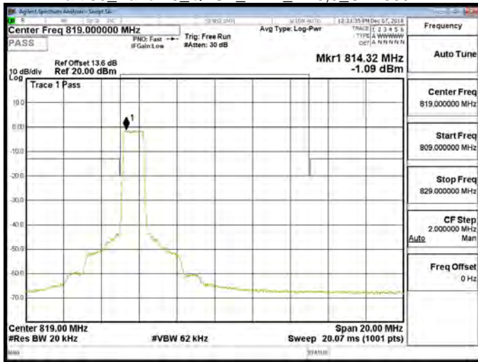
Part 90 Band 26 QPSK 1.4M_RB6,0_CH26740
