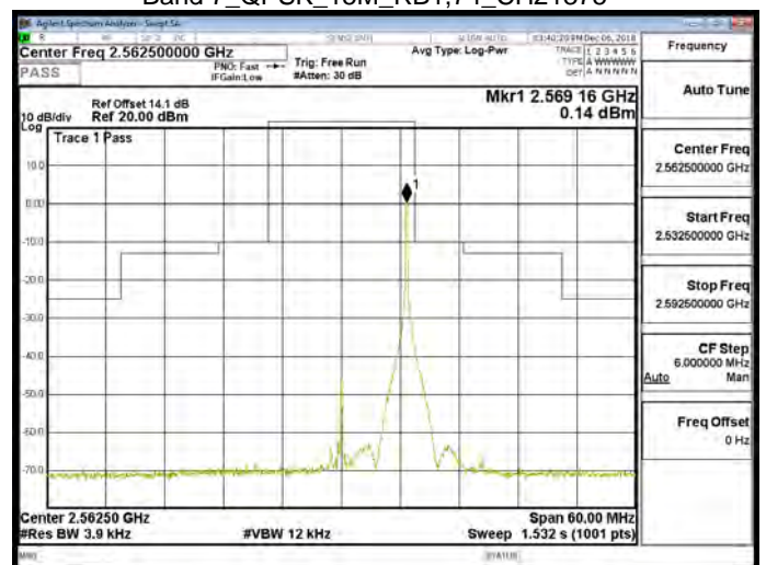
Band 7_QPSK_15M_RB1,74_CH21375
