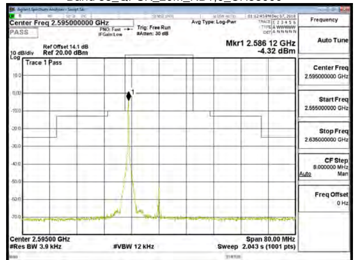
Band 38_QPSK_20M_RB1,0_CH38150
