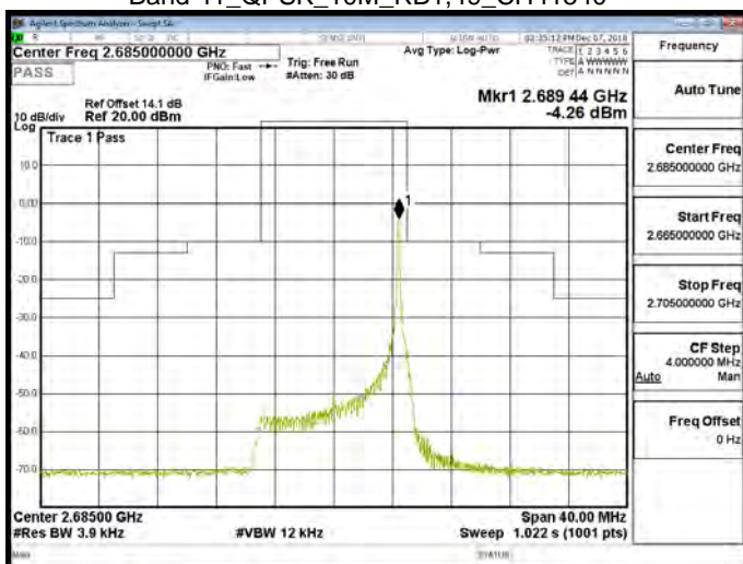
Band 41_QPSK_10M_RB1,49_CH41540
