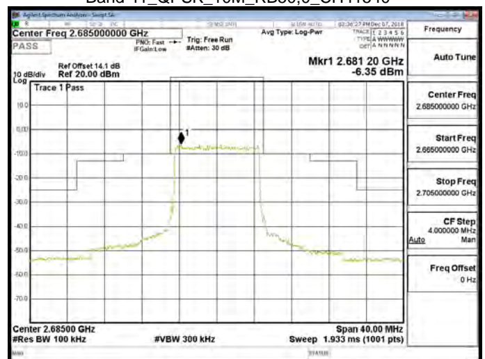
Band 41_QPSK_10M_RB50,0_CH41540
