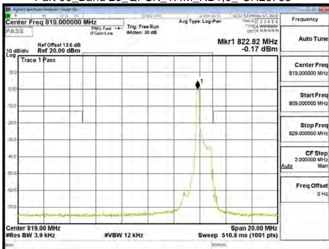
Part 90_Band 26_QPSK_1.4M_RB1,0_CH26783
