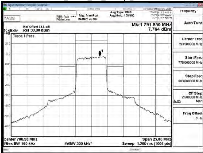
Band 14_QPSK_5M_RB25,0_CH23330
