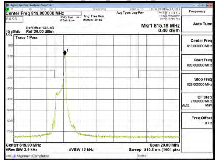
Part 90_Band 26_QPSK_1.4M_RB1,5_CH26740
