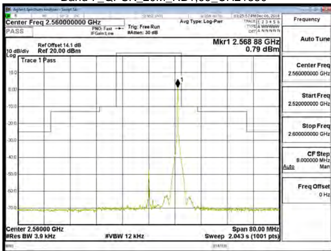
Band 7_QPSK_20M_RB1,99_CH21350
