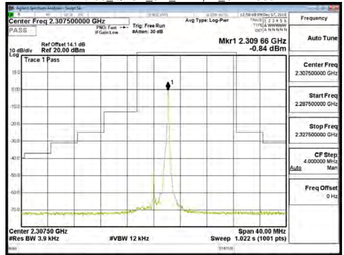
Band 30_QPSK_5M_RB1,24_CH27710
