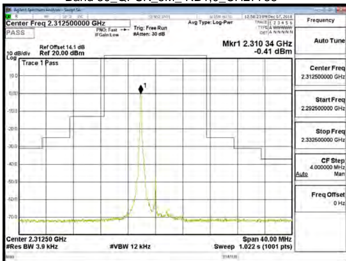
Band 30_QPSK_5M_RB1,0_CH27735
