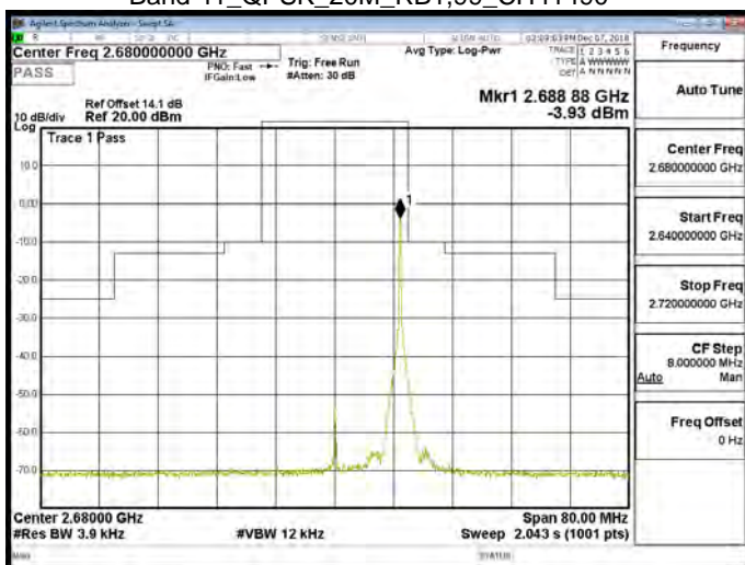
Band 41_QPSK_20M_RB1,99_CH41490
