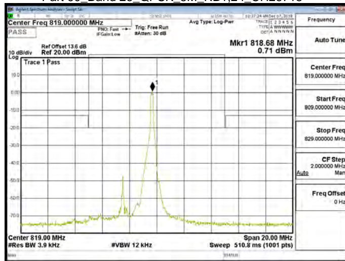
Part 90_Band 26_QPSK_5M_RB1,24_CH26740
