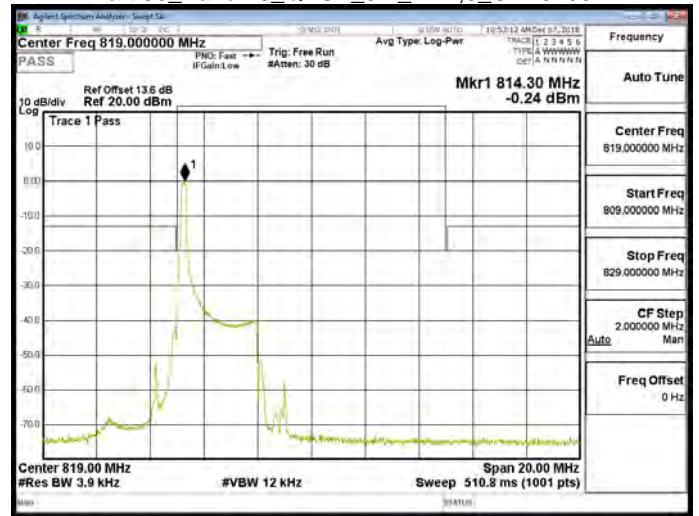
Part 90 Band 26 QPSK 3M_RB1,0_CH26740
