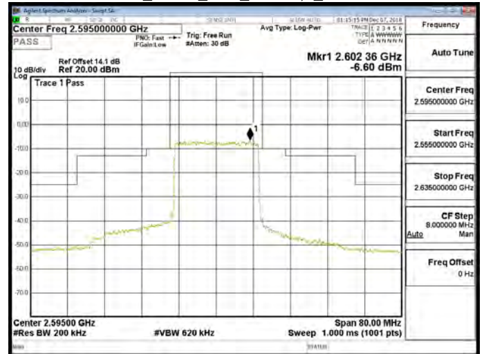
Band 38_QPSK_20M_RB100,0_CH38150
