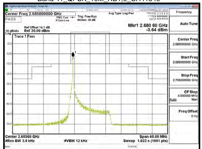
Band 41_QPSK_10M_RB1,0_CH41540
