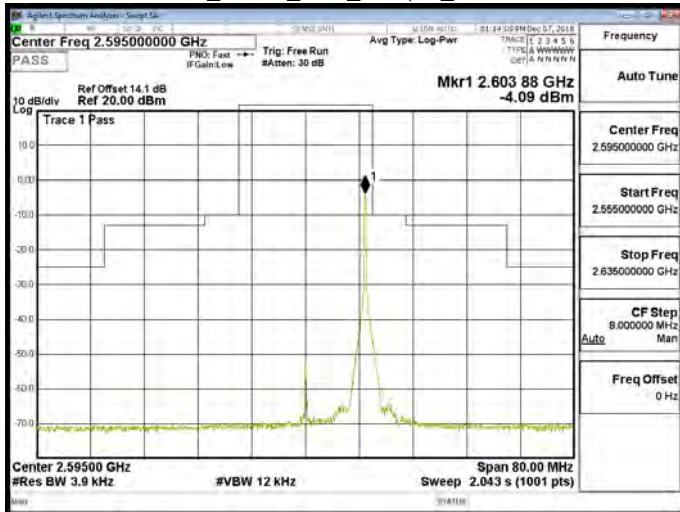
Band 38_QPSK_20M_RB1,99_CH38150
