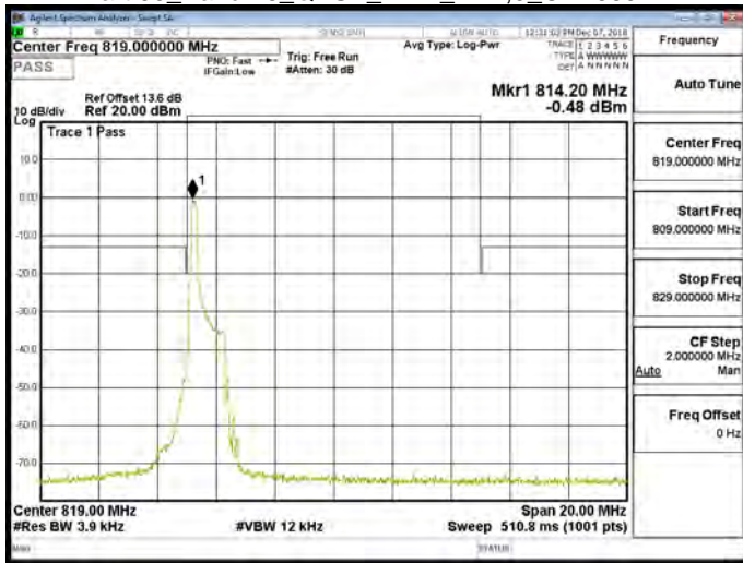
Part 90_Band 26_QPSK_1.4M_RB1,0_CH26740
