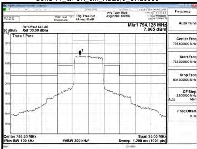
Band 14_QPSK_5M_RB25,0_CH23355
