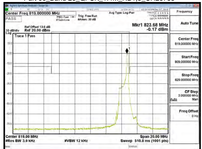
Part 90_Band 26_QPSK_1.4M_RB1,5_CH26783
