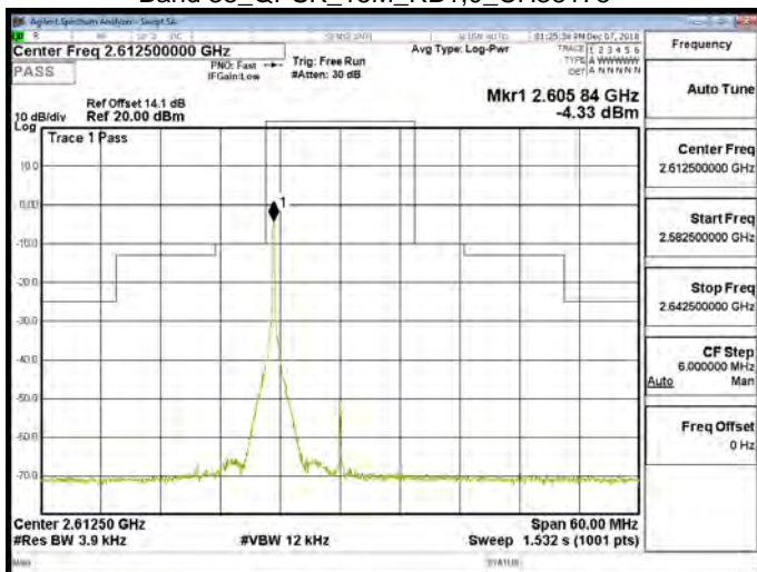
Band 38_QPSK_15M_RB1,0_CH38175
