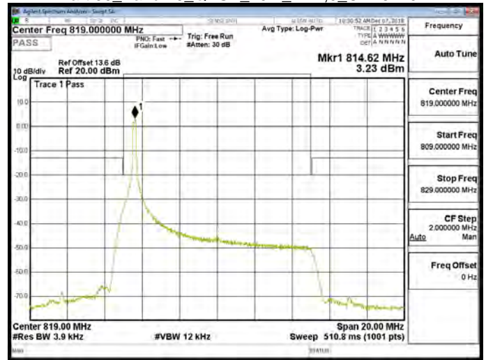
Part 90_Band 26_QPSK_10M_RB1,49_CH26740
