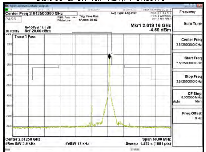
Band 38_QPSK_15M_RB1,74_CH38175
