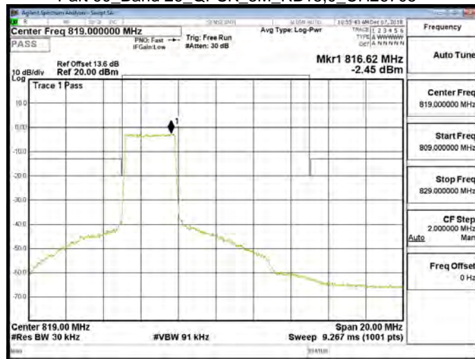
Part 90_Band 26_QPSK_3M_RB15,0_CH26740
