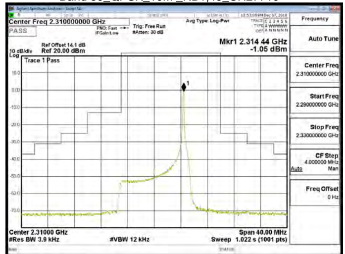
Band 30_QPSK_10M_RB50,0_CH27710
