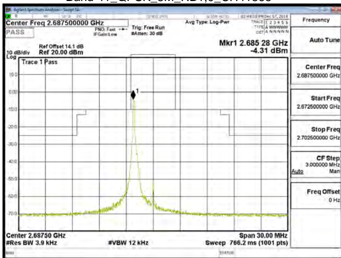
Band 41_QPSK_5M_RB1,0_CH41565
