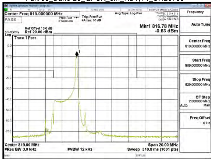
Part 90_Band 26_QPSK_3M_RB1,14_CH26740
