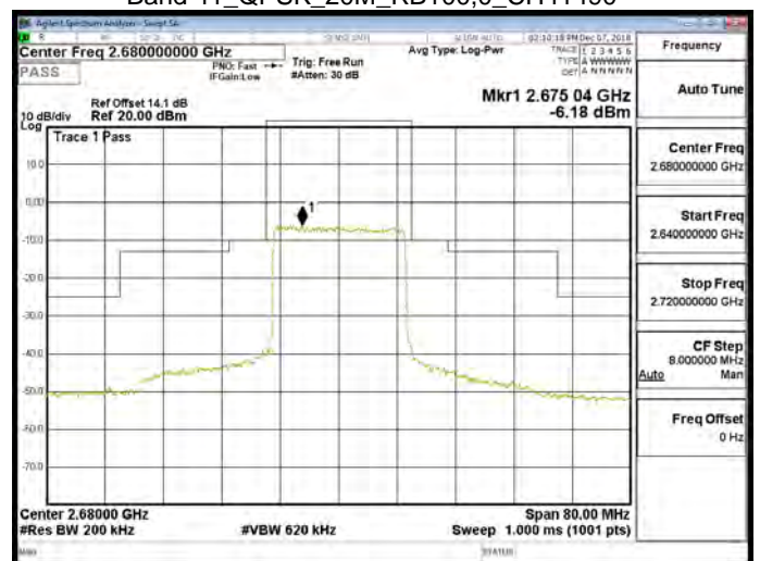
Band 41_QPSK_20M_RB100,0_CH41490
