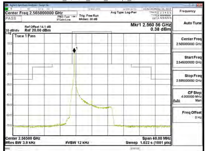
Band 7_QPSK_10M_RB1,0_CH21400
