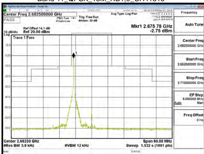
Band 41_QPSK_15M_RB1,0_CH41515
