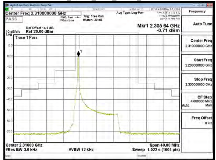
Band 30_QPSK_10M_RB1,49_CH27710
