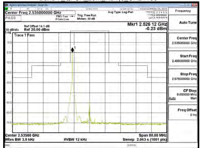
Band 7_QPSK_20M_RB1,0_CH21350
