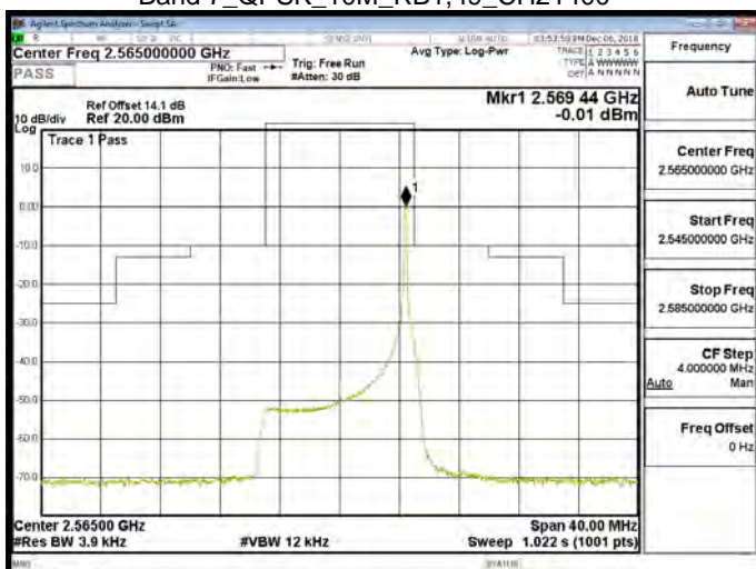
Band 7_QPSK_10M_RB1,49_CH21400
