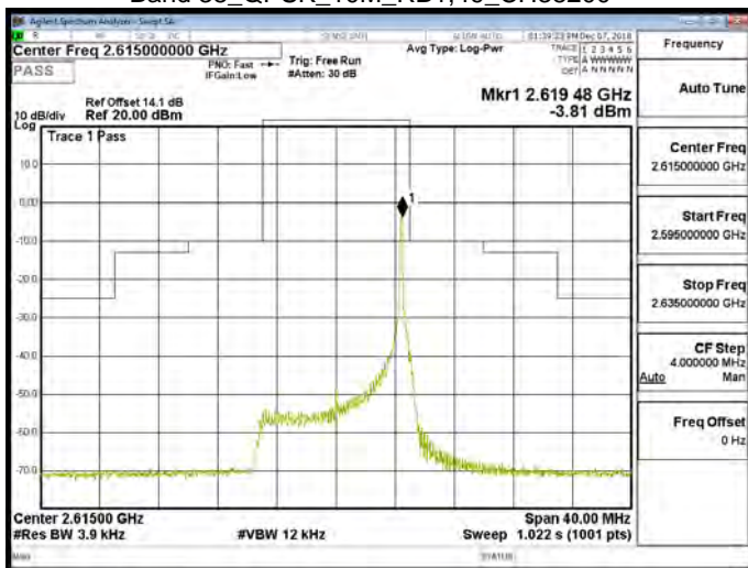
Band 38_QPSK_10M_RB1,49_CH38200
