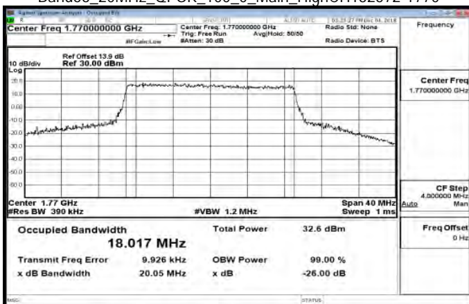
Band66_20MHz_QPSK_100_0_Main_HighCH132572-1770
