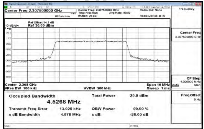
Band30_5MHz_QPSK_25_0_Main_LowCH27685-2307.5
