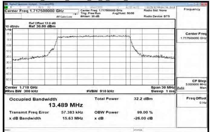
Band66_15MHz_QPSK_75_0_Main_LowCH132047-1717.5
