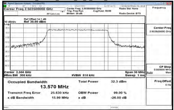
Band41_15MHz_QPSK_75_0_Main_LowCH39725-2503.5
