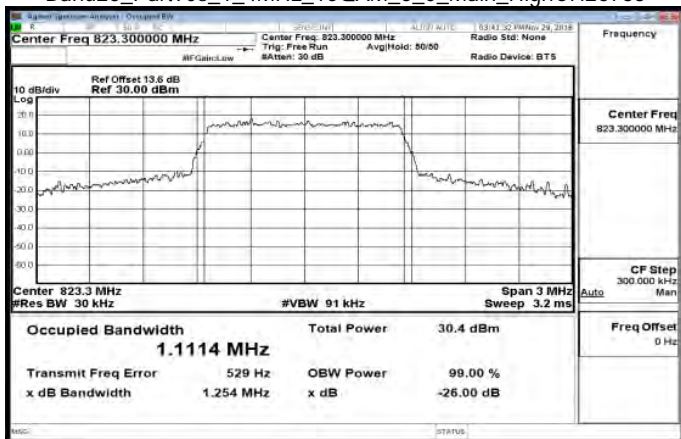
Band26_Part90s_1_4MHz_16QAM_6_0_Main_HighCH26783
