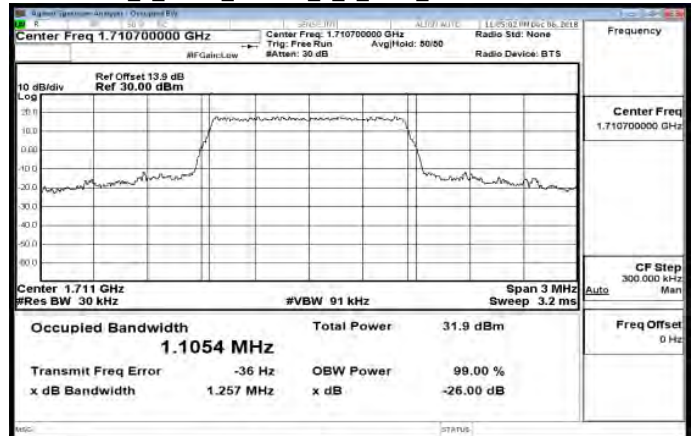
Band66_1_4MHz_64QAM_6_0_Main_LowCH131979-1710.7
