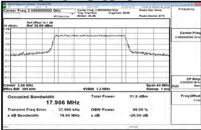
Band38_20MHz_64QAM_100_0_Main_LowCH37850-2580
