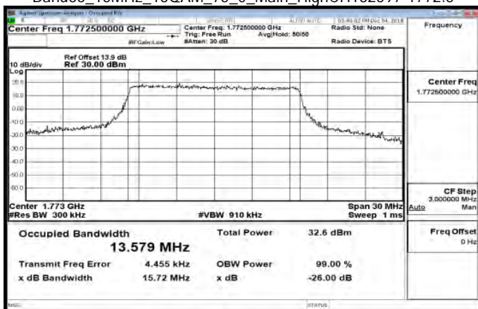
Band66_15MHz_16QAM_75_0_Main_HighCH132597-1772.5
