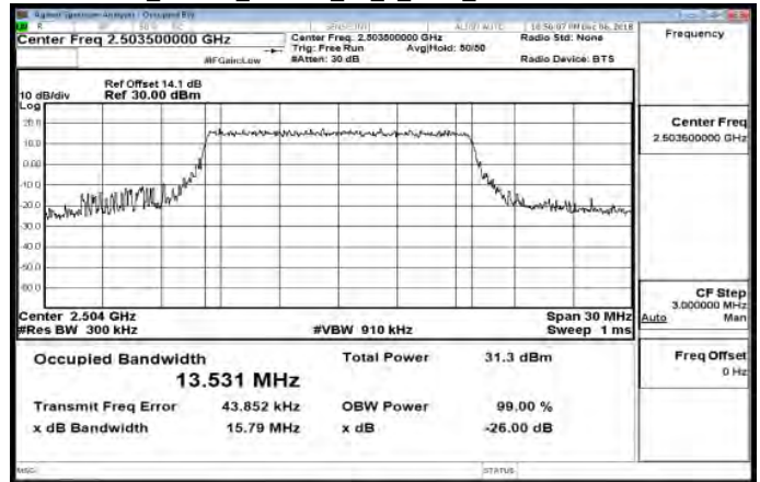
Band41_15MHz_64QAM_75_0_Main_LowCH39725-2503.5
