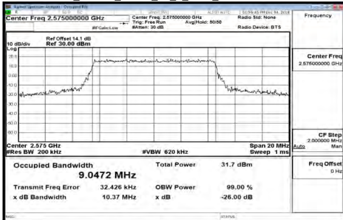
Band38_10MHz_QPSK_50_0_Main_LowCH37800-2575
