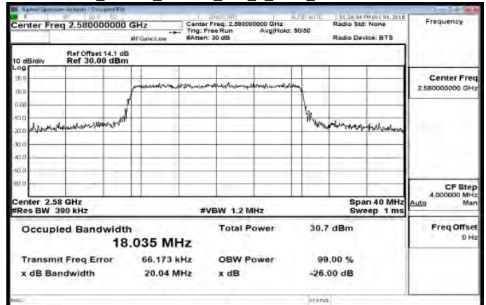
Band38_20MHz_16QAM_100_0_Main_LowCH37850-2580
