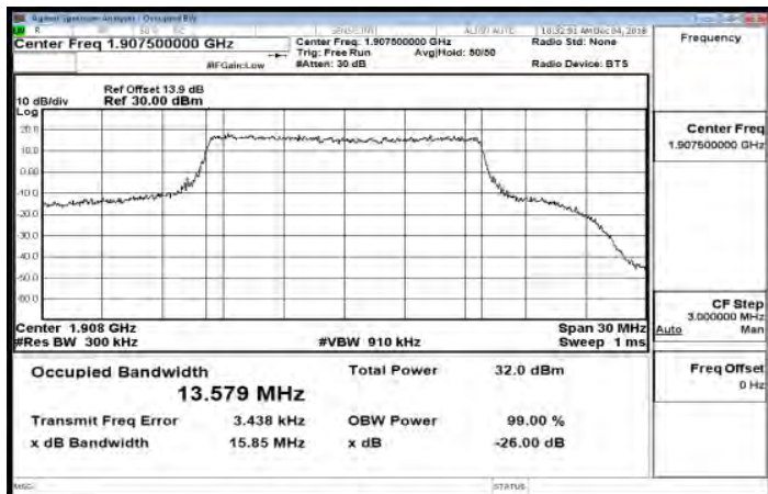
Band25_15MHz_QPSK_75_0_HighCH26615-1907.5
