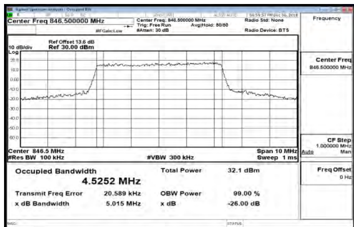
Band26_5MHz_64QAM_25_0_HighCH27015-846.5
