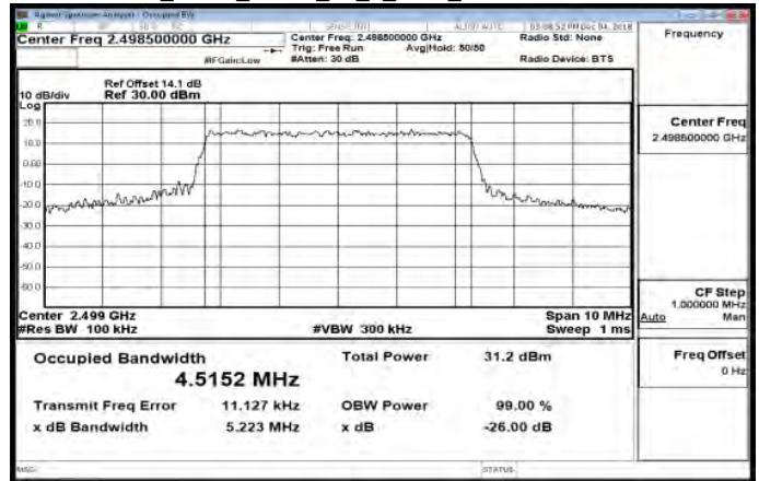
Band41_5MHz_QPSK_25_0_Main_LowCH39675-2498.5
