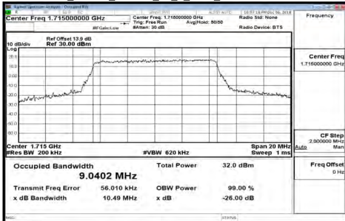
Band66_10MHz_64QAM_50_0_Main_LowCH132022-1715
