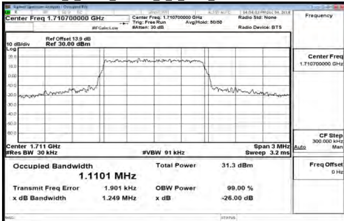
Band66_1_4MHz_16QAM_6_0_Main_LowCH131979-1710.7
