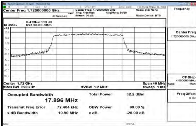
Band66_20MHz_QPSK_100_0_Main_LowCH132072-1720
