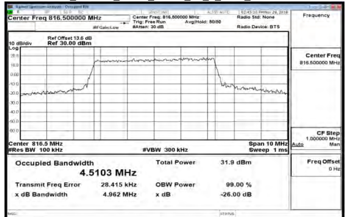
Band26_Part90s_5MHz_QPSK_25_0_Main_LowCH26715
