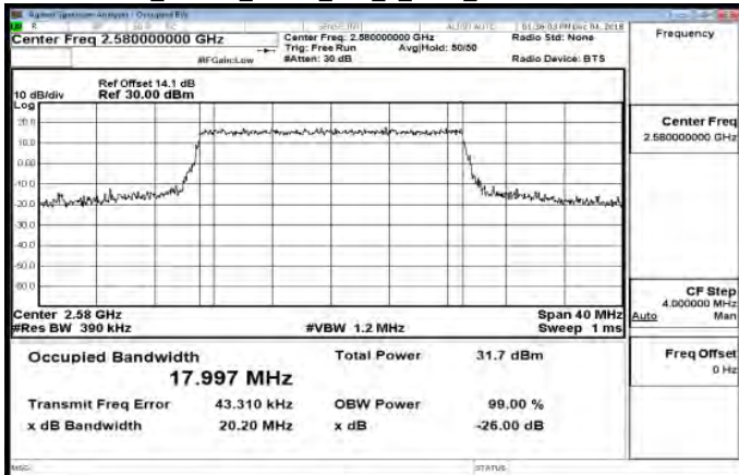
Band38_20MHz_QPSK_100_0_Main_LowCH37850-2580
