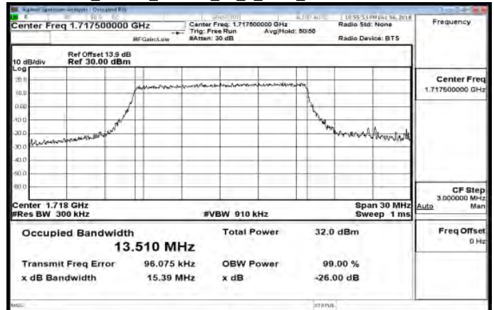
Band66_15MHz_64QAM_75_0_Main_LowCH132047-1717.5
