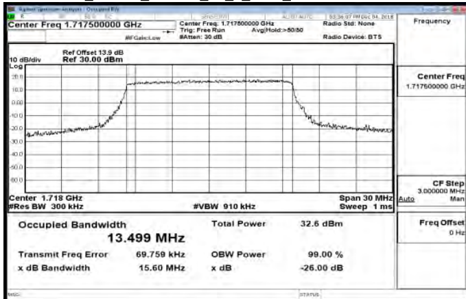
Band66_15MHz_16QAM_75_0_Main_LowCH132047-1717.5
