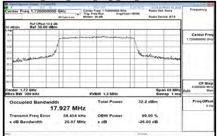
Band66_20MHz_16QAM_100_0_Main_LowCH132072-1720
