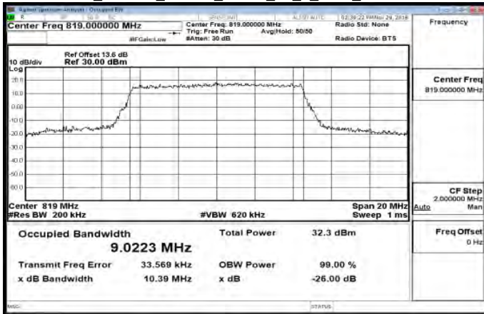
Band26_Part90s_10MHz_QPSK_50_0_Main_MidCH26740
