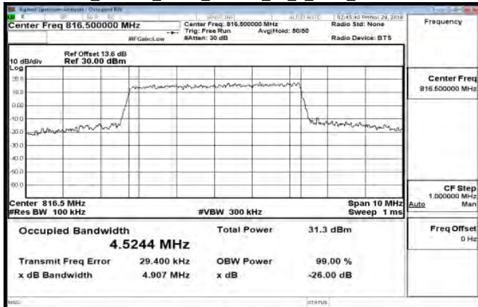
Band26_Part90s_5MHz_16QAM_25_0_Main_LowCH26715
