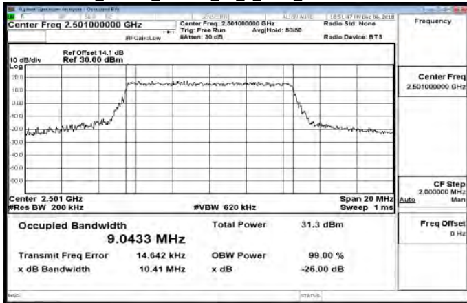
Band41_10MHz_64QAM_50_0_Main_LowCH39700-2501
