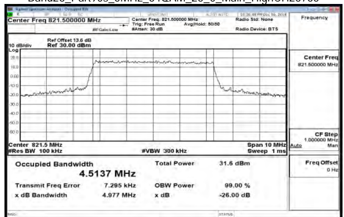
Band26_Part90s_5MHz_64QAM_25_0_Main_HighCH26765
