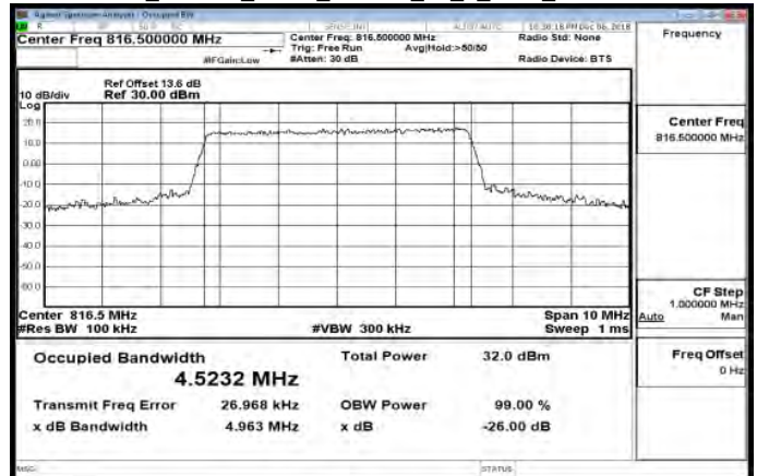
Band26_Part90s_5MHz_64QAM_25_0_Main_LowCH26715
