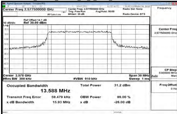
Band38_15MHz_16QAM_75_0_Main_LowCH37825-2577.5
