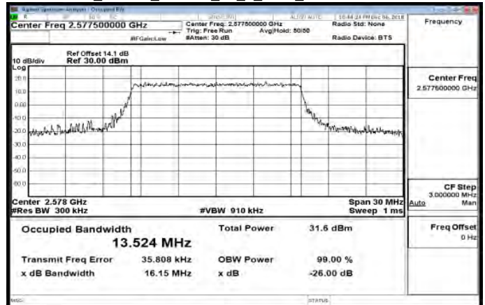
Band38_15MHz_64QAM_75_0_Main_LowCH37825-2577.5
