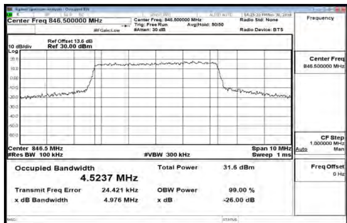
Band26_5MHz_QPSK_25_0_HighCH27015-846.5
