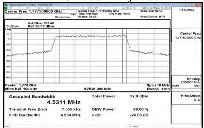
Band66_5MHz_QPSK_25_0_Main_HighCH132647-1777.5
