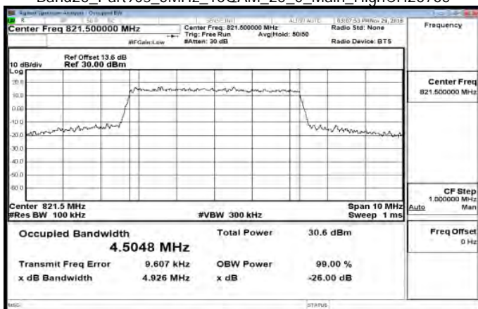
Band26_Part90s_5MHz_16QAM_25_0_Main_HighCH26765
