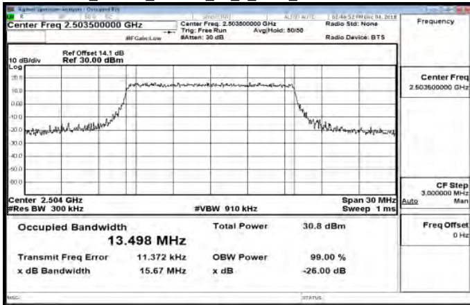
Band41_15MHz_16QAM_75_0_Main_LowCH39725-2503.5
