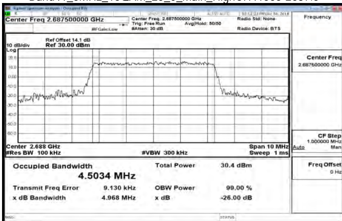
Band41_5MHz_16QAM_25_0_Main_HighCH41565-2687.5
