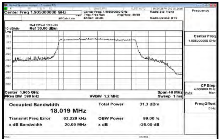
Band25_20MHz_64QAM_100_0_HighCH26590-1905
