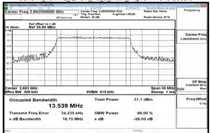
Band41_15MHz_QPSK_75_0_Main_HighCH41515-2682.5
