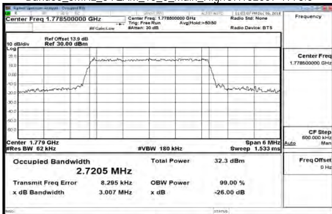
Band66_3MHz_64QAM_15_0_Main_HighCH132657-1778.5
