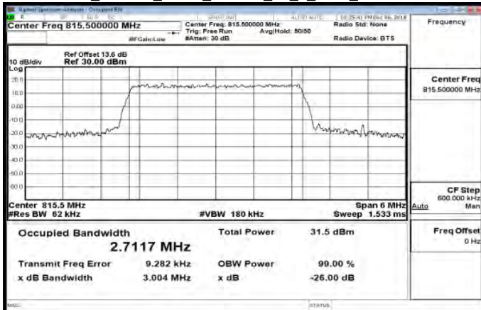
Band26_Part90s_3MHz_64QAM_15_0_Main_LowCH26705
