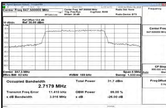
Band26_3MHz_64QAM_15_0_HighCH27025-847.5
