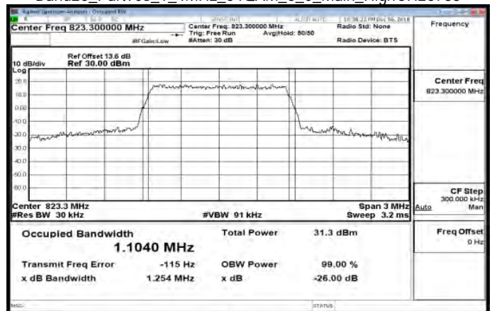
Band26_Part90s_1_4MHz_64QAM_6_0_Main_HighCH26783
