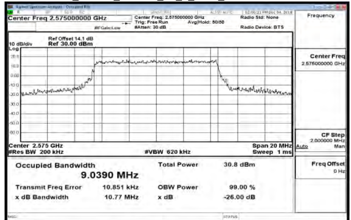
Band38_10MHz_16QAM_50_0_Main_LowCH37800-2575
