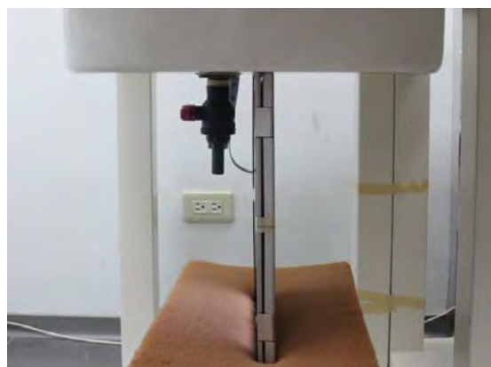
Fig.6 EUT Right side e to flat phantom
