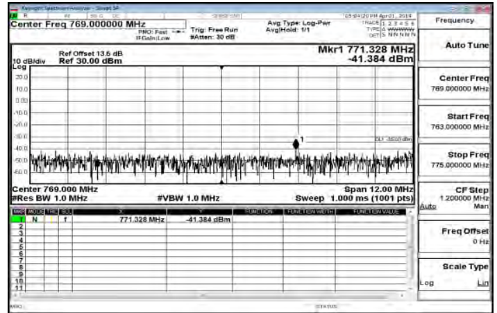
Inband-2_Band13_5MHz_QPSK_1_0_LowCH23205-779.5
