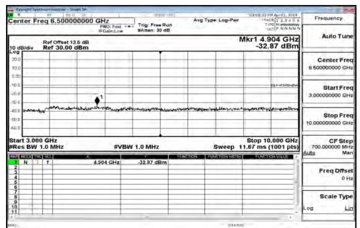
3GHz~10GHz_Band26_Part90s_5MHz_QPSK_1_0_LowCH26715-816.5
