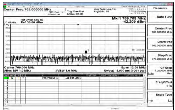
Inband-1_Band13_5MHz_QPSK_1_0_MidCH23230-782
