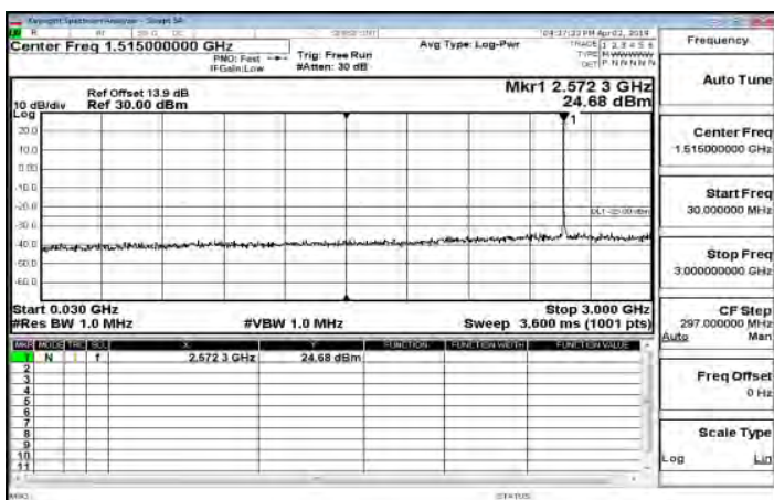
30MHz~3GHz_Band38_10MHz_QPSK_1_0_LowCH37800-2575
