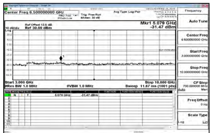
3GHz~10GHz_Band5_5MHz_QPSK_1_0_HighCH20625-846.5
