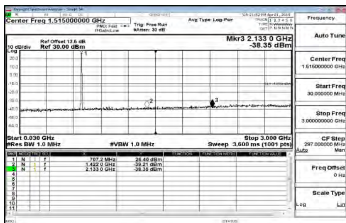
30MHz~3GHz_Band17_10MHz_QPSK_1_0_HighCH23800-711
