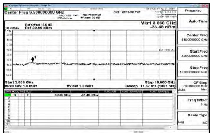
3GHz~10GHz_Band13_5MHz_QPSK_1_0_HighCH23255-784.5
