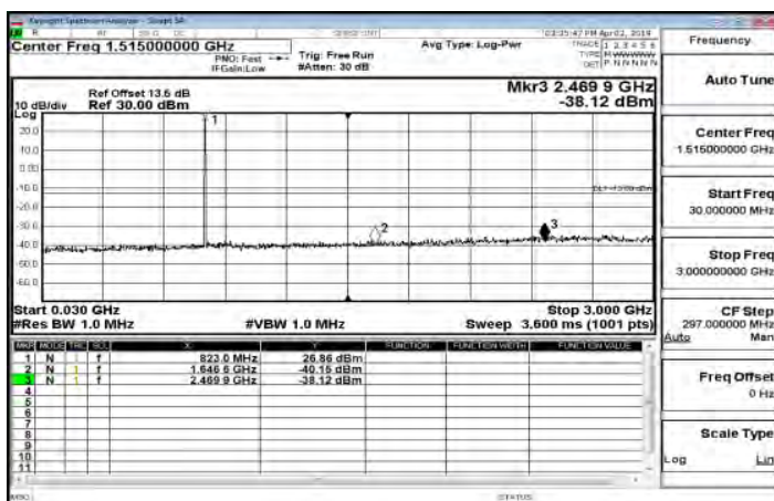
30MHz~3GHz_Band26_Part90s_1_4MHz_QPSK_1_0_HighCH26783-823.3
