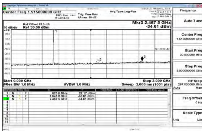
30MHz~3GHz_Band26_Part90s_3MHz_QPSK_1_0_HighCH26775-822.5
