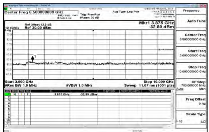
3GHz~10GHz_Band12_1_4MHz_QPSK_1_0_HighCH23173-715.3
