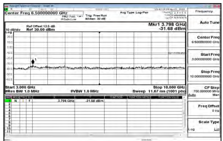
3GHz~10GHz_Band26_15MHz_QPSK_1_0_LowCH26865-831.5
