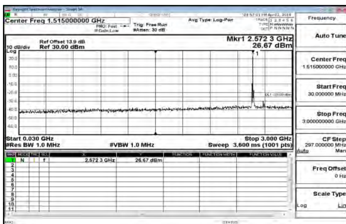
30MHz~3GHz_Band38_20MHz_QPSK_1_0_LowCH37850-2580
