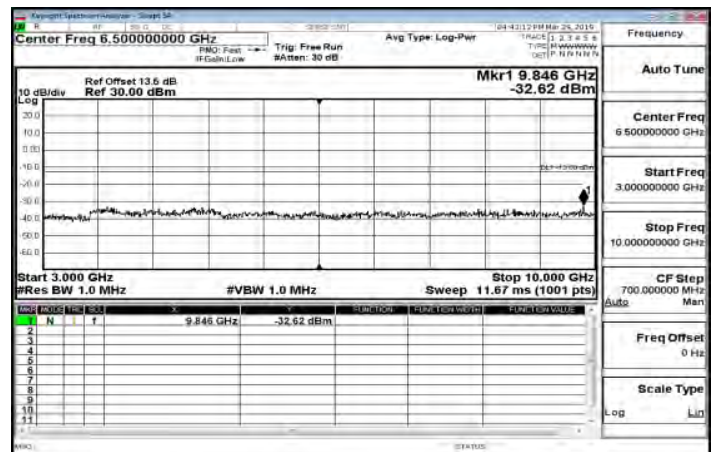
3GHz~10GHz_Band5_3MHz_QPSK_1_0_HighCH20635-847.5
