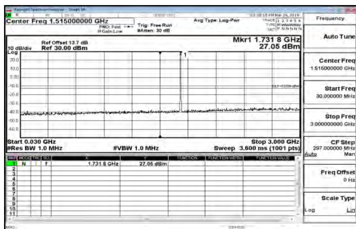
30MHz~3GHz_Band4_5MHz_QPSK_1_0_MidCH20175-1732.5
