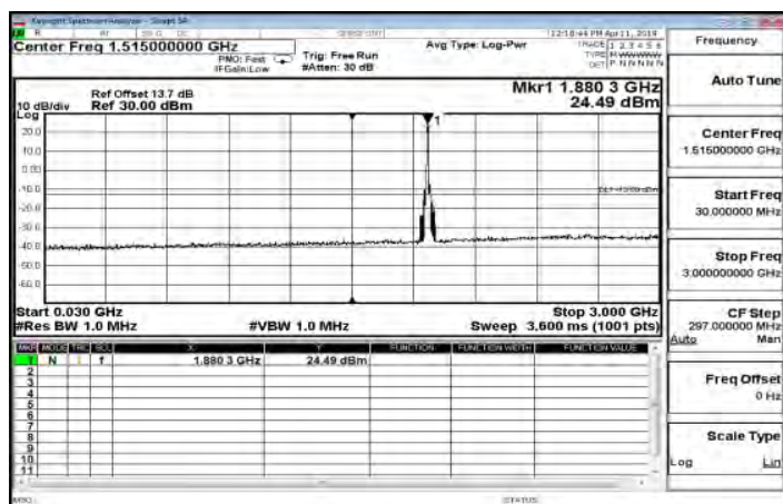
30MHz~3GHz_HSDPA_B2_MidCH9400-1880
