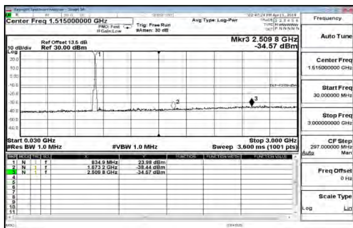
30MHz~3GHz_HSDPA_B5_MidCH4183-836.6
