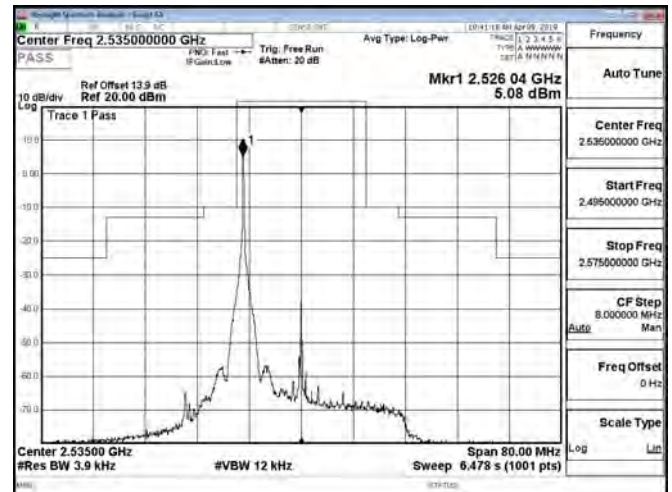
Band7_20MHz_16QAM_1_0_CH21350
