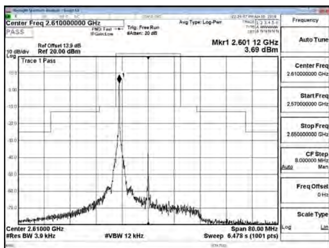
Band38_20MHz_QPSK_1_0_CH38150
