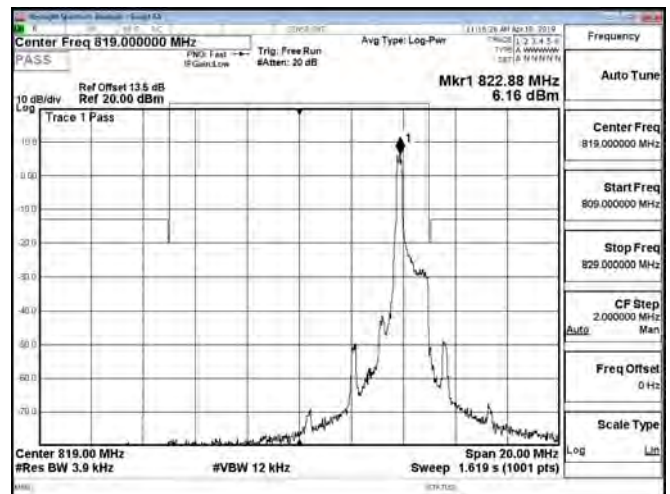
Band26_Part90s_1.4MHz_16QAM_1_0_CH26783
