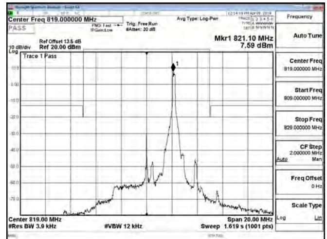
Band26_Part90s_5MHz_QPSK_1_24_CH26765
