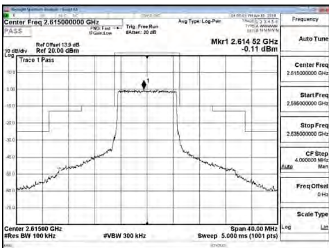
Band38_10MHz_QPSK_50_0_CH38200
