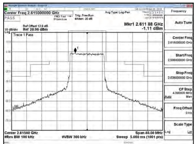
Band38_10MHz_16QAM_50_0_CH38200
