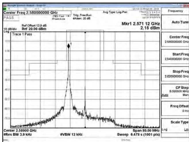
Band38_20MHz_QPSK_1_0_CH38000
