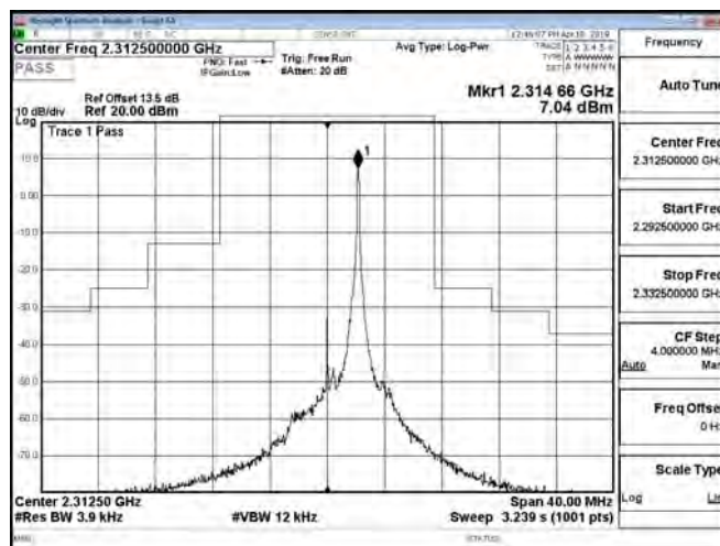
Band30_5MHz_QPSK_1_24_CH27735
