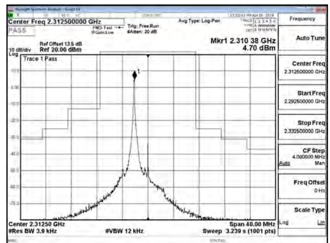
Band30_5MHz_16QAM_1_0_CH27735
