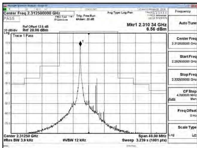
Band30_5MHz_QPSK_1_0_CH27735
