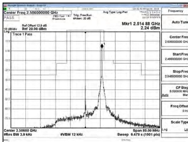
Band41_20MHz_QPSK_1_99_CH40620
