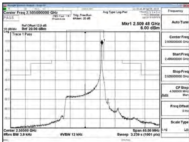
Band7_10MHz_16QAM_1_49_CH21100
