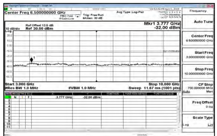
3GHz~10GHz_HSUPA_B5_HighCH4233-846.6
