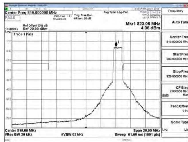
Band26_Part90s_1.4MHz_16QAM_6_0_CH26783
