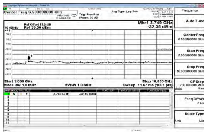
3GHz~10GHz_HSDPA_B5_HighCH4233-846.6
