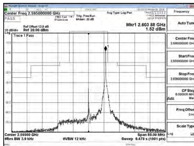
Band38_20MHz_QPSK_1_99_CH38150
