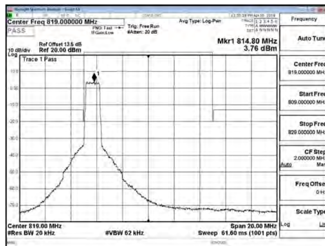
Band26_Part90s_1.4MHz_16QAM_6_0_CH26740
