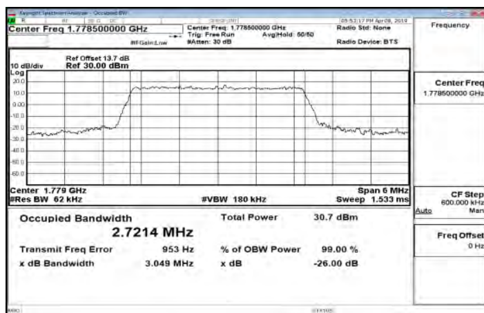
Band66_3MHz_QPSK_15_0_Main_HighCH132657-1778.5
