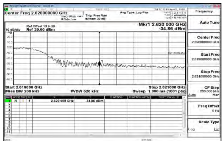
LTE\Band38_15MHz_QPSK_75_0_HighCH38175-2612.5
