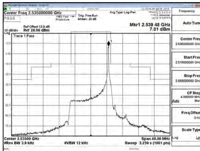
Band7_10MHz_QPSK_1_49_CH21400
