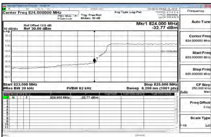
LTE\Band5_1_4MHz_QPSK_6_0_LowCH20407-824.7
