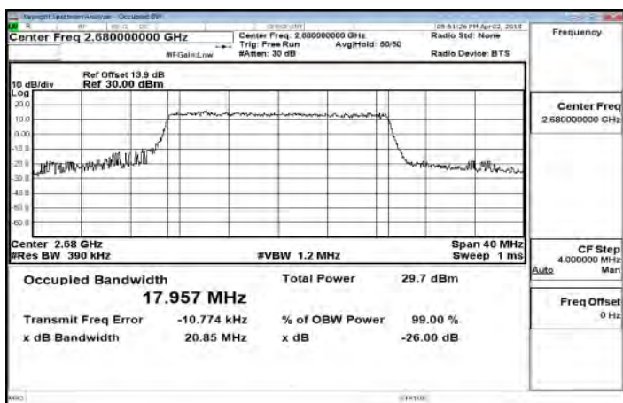
Band41_20MHz_16QAM_100_0_Main_HighCH41490-2680
