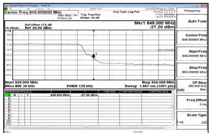
LTE\Band26_3MHz_QPSK_15_0_HighCH27025-847.5
