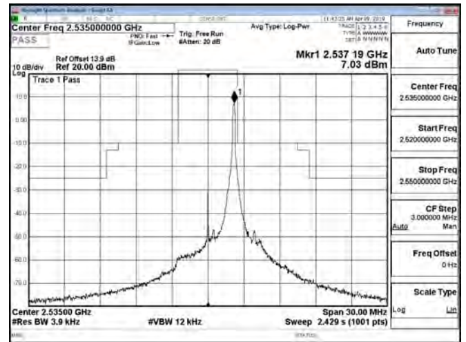
Band7_5MHz_QPSK_1_24_CH21425
