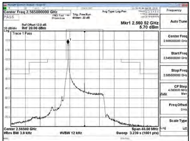
Band7_10MHz_16QAM_1_0_CH21400
