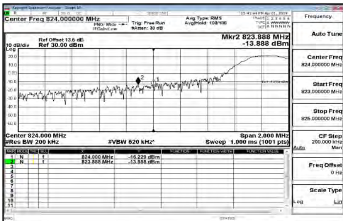
LTE\Band26_15MHz_QPSK_1_0_LowCH26865-831.5
