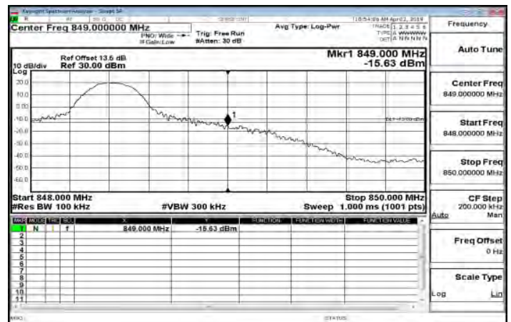
LTE\Band26_10MHz_QPSK_1_49_HighCH26990-844
