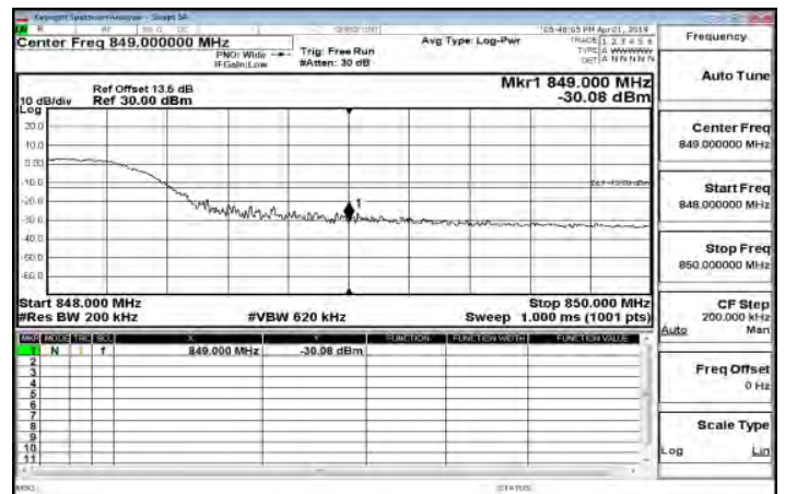
LTE\Band26_15MHz_QPSK_75_0_HighCH26965-841.5
