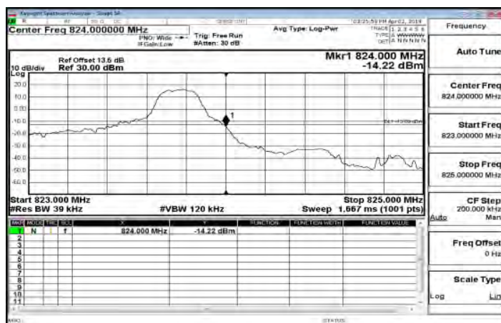
LTE\Band26_Part90s_3MHz_QPSK_1_14_HighCH26775-822.5
