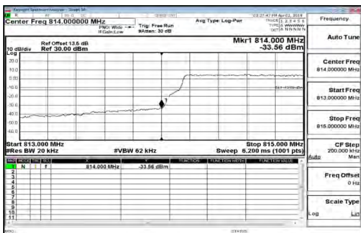
LTE\Band26_Part90s_1_4MHz_QPSK_6_0_LowCH26697-814.7
