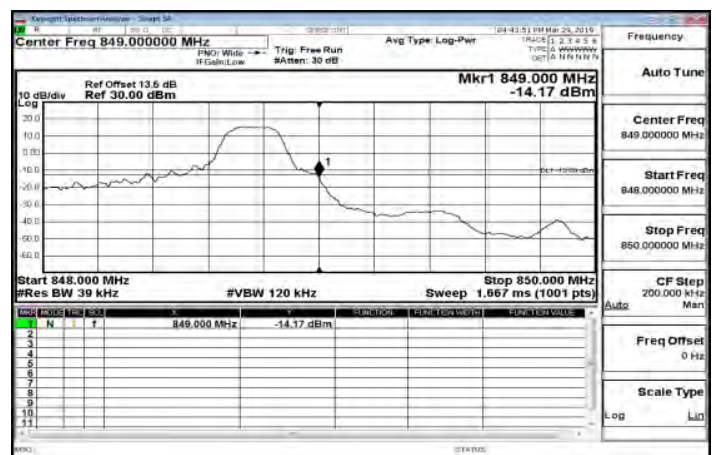
LTE\Band5_3MHz_QPSK_1_14_HighCH20635-847.5
