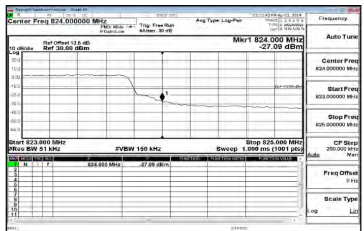
LTE\Band26_Part90s_5MHz_QPSK_25_0_HighCH26765-821.5
