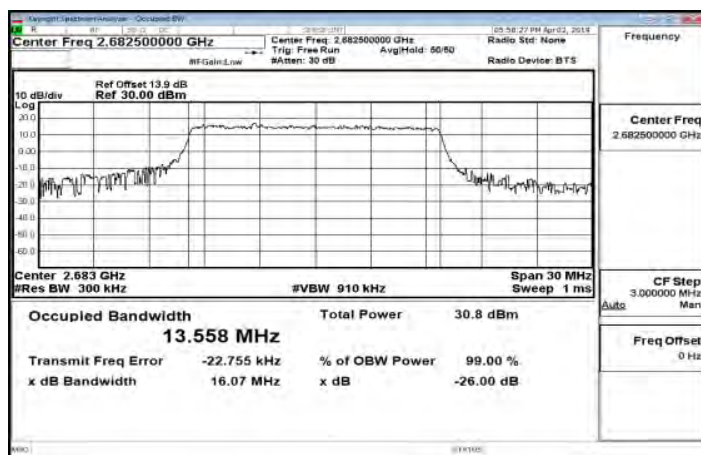
Band41_15MHz_QPSK_75_0_Main_HighCH41515-2682.5
