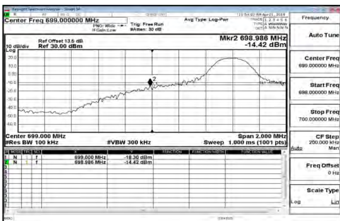
LTE\Band12_10MHz_QPSK_1_0_LowCH23060-704
