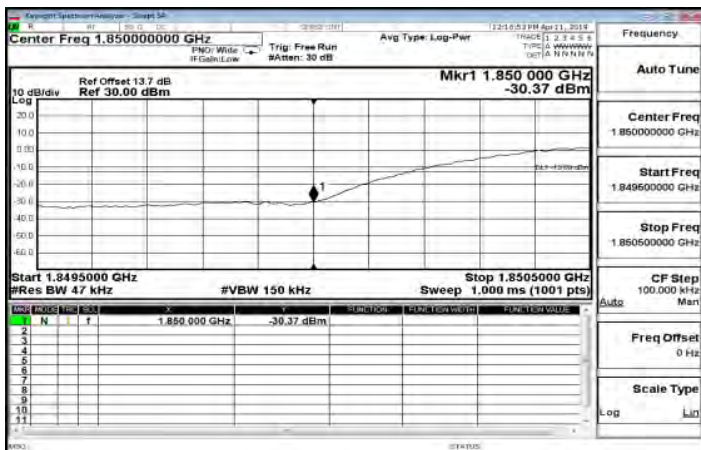
HSDPA_B2_LowCH9262-1852.4
