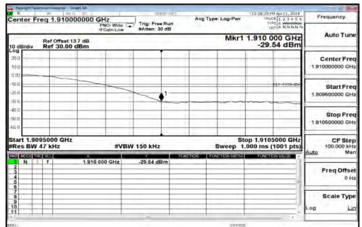
HSUPA_B2_HighCH9538-1907.6
