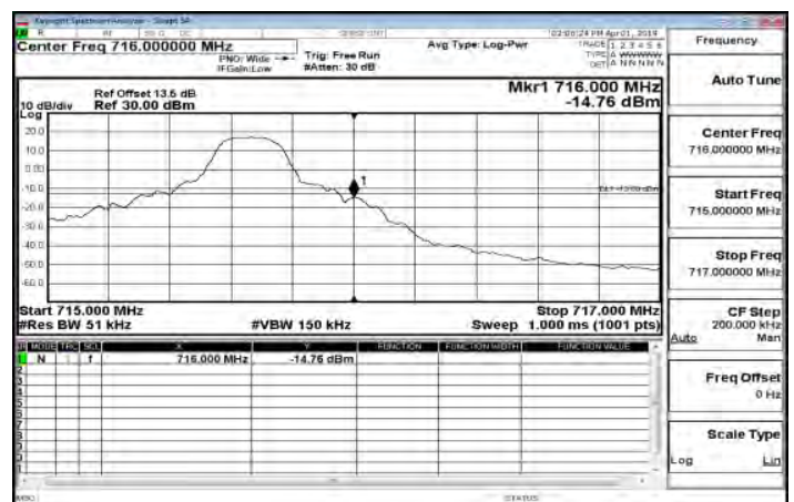
LTE\Band12_5MHz_QPSK_1_24_HighCH23155-713.5
