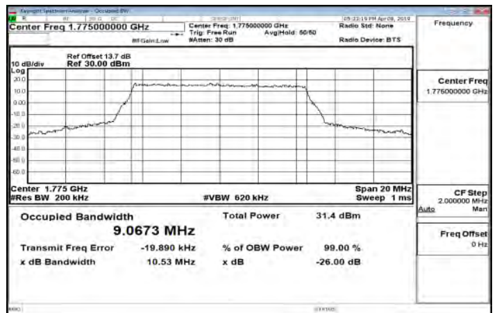
Band66_10MHz_QPSK_50_0_Main_HighCH132622-1775
