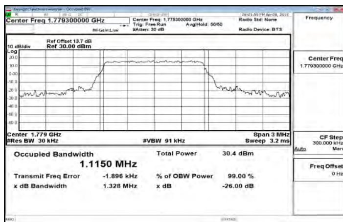
Band66_1_4MHz_QPSK_6_0_Main_HighCH132665-1779.3
