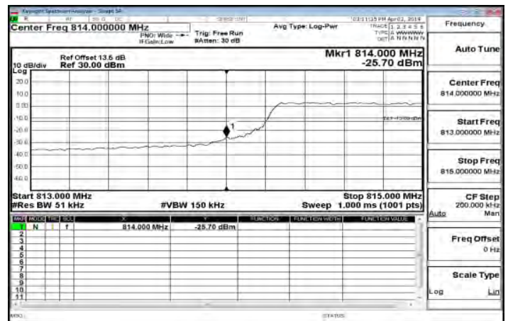
LTE\Band26_Part90s_5MHz_QPSK_25_0_HighCH26765-821.5
