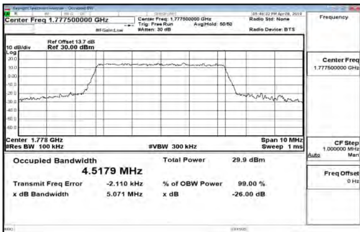
Band66_5MHz_16QAM_25_0_Main_HighCH132647-1777.5
