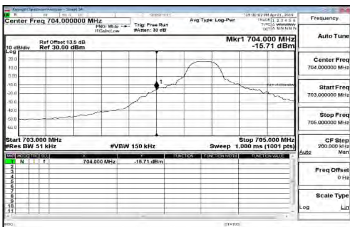
LTE\Band17_5MHz_QPSK_1_0_LowCH23755-706.5
