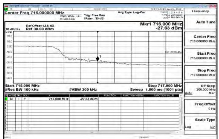
LTE\Band12_10MHz_QPSK_50_0_HighCH23130-711
