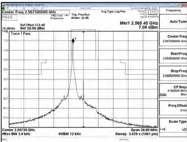
Band7_5MHz_QPSK_1_0_CH21425
