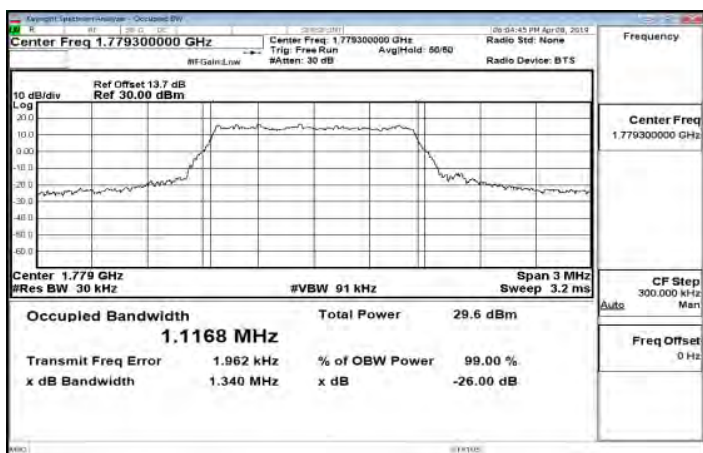
Band66_1_4MHz_16QAM_6_0_Main_HighCH132665-1779.3
