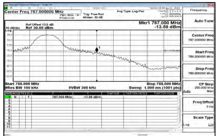
LTE\Band13_10MHz_QPSK_1_49_HighCH23230-782
