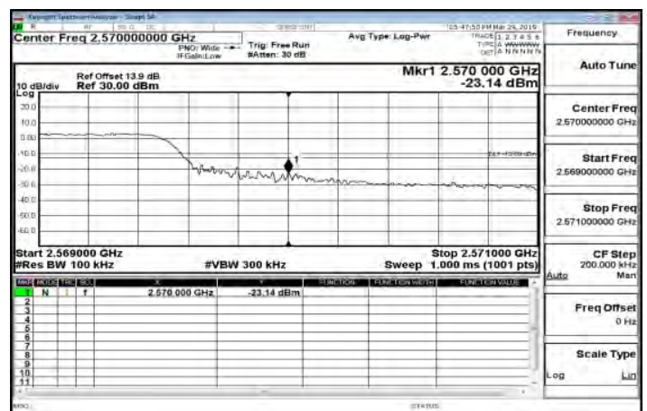
LTE\Band7_10MHz_QPSK_50_0_HighCH21400-2565
