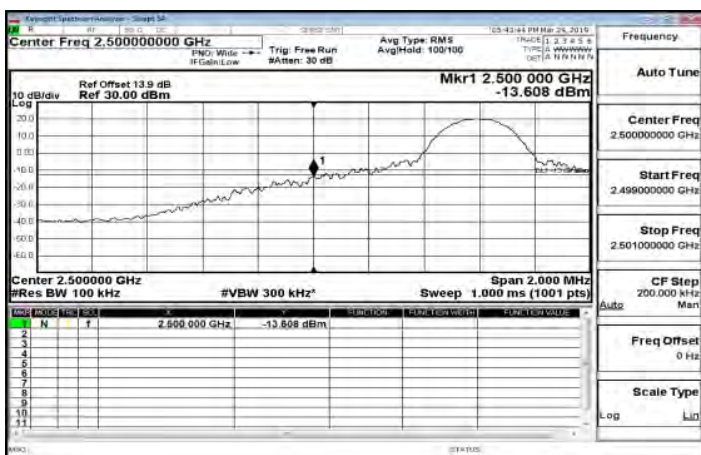
LTE\Band7_10MHz_QPSK_1_0_LowCH20800-2505
