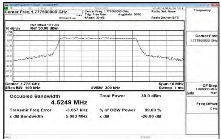
Band66_5MHz_QPSK_25_0_Main_HighCH132647-1777.5
