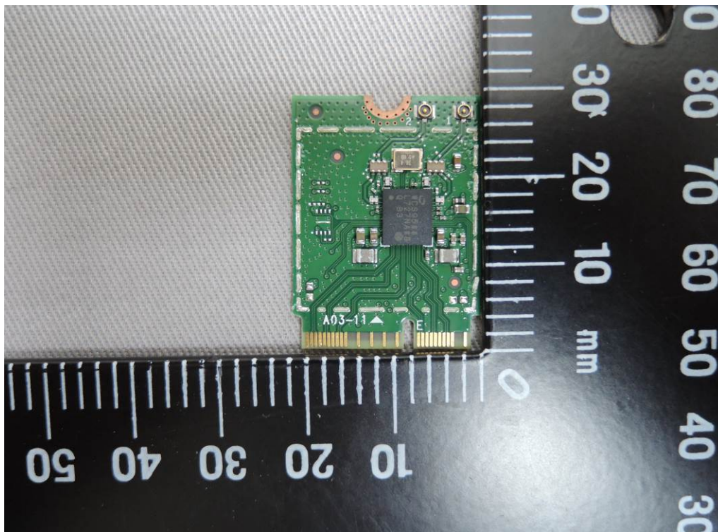
WLAN / BT Module-1 (Model No.: AX200NGW)
