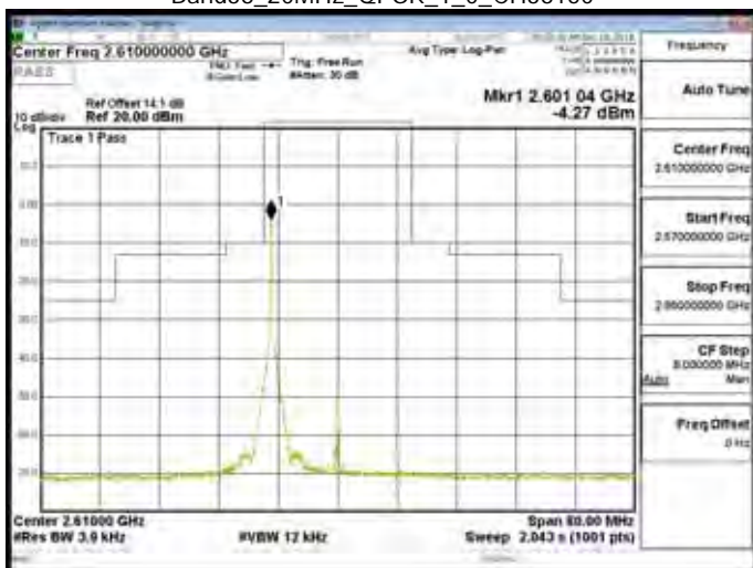
Band38_20MHz_QPSK_1_0_CH38150
