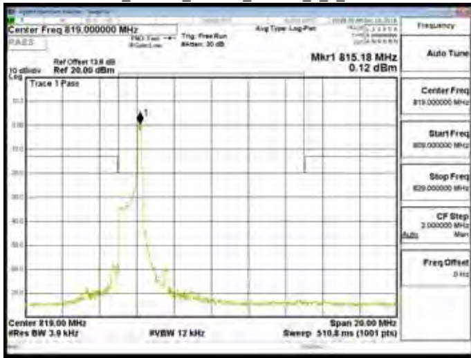
Band26_Part90s_1.4MHz_16QAM_1_5_CH26740
