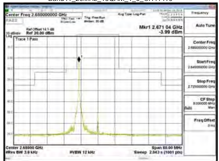
Band41_20MHz_16QAM_1_0_CH41490
