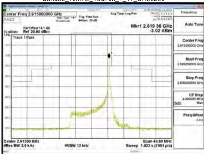
Band38_10MHz_16QAM_1_49_CH38200
