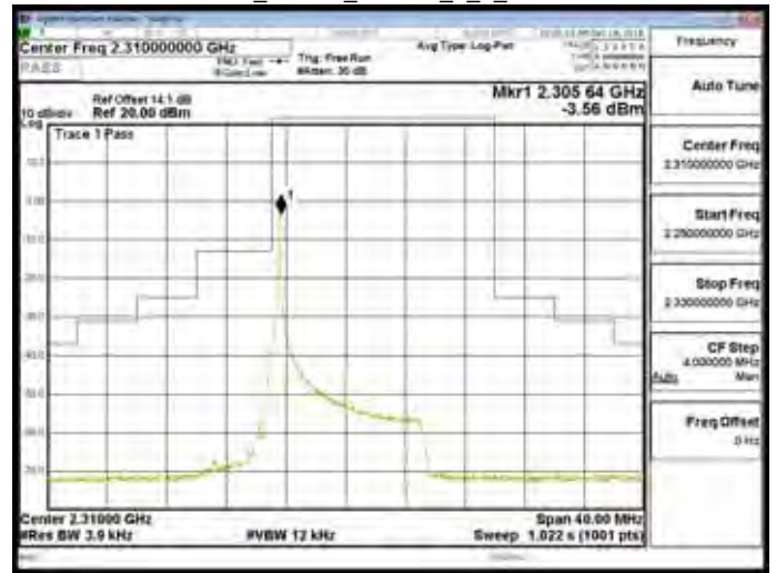
Band30_10MHz_16QAM_1_49_CH27710
