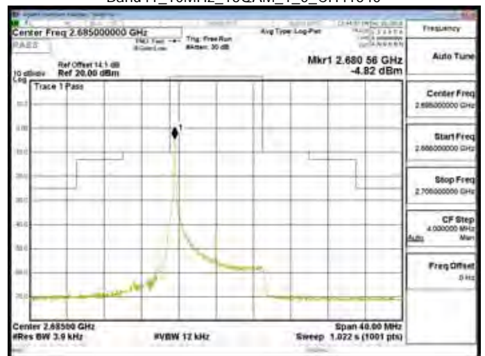
Band41_10MHz_16QAM_1_0_CH41540
