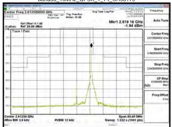
Band38_15MHz_QPSK_1_74_CH38175
