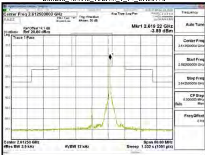
Band38_15MHz_16QAM_1_74_CH38175
