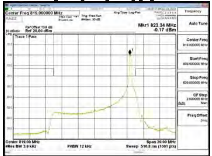
Band26_Part90s_10MHz_16QAM_50_0_CH26740
