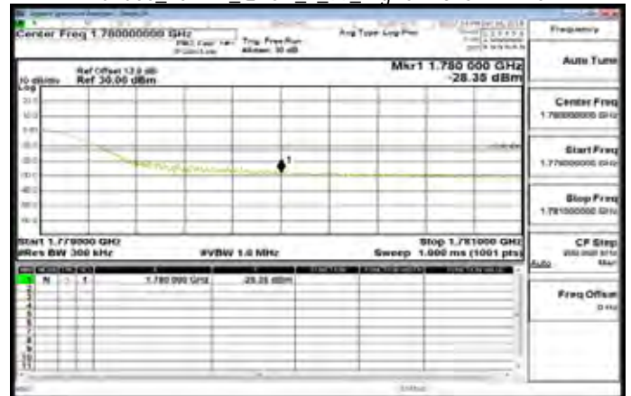
Band66_20MHz_QPSK_1_99_HighCH132572-1770
