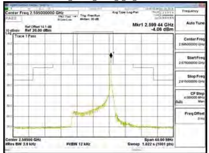
Band38_10MHz_QPSK_1_49_CH38200
