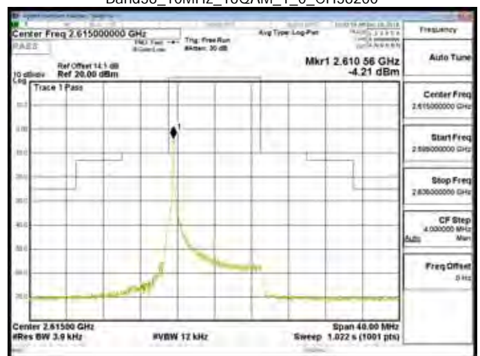
Band38_10MHz_16QAM_1_0_CH38200
