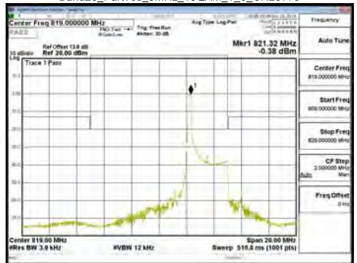
Band26_Part90s_3MHz_16QAM_1_0_CH26775
