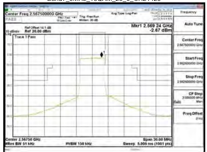
Band7_5MHz_16QAM_25_0_CH21425
