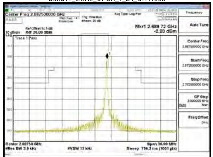
Band41_5MHz_QPSK_1_24_CH41565
