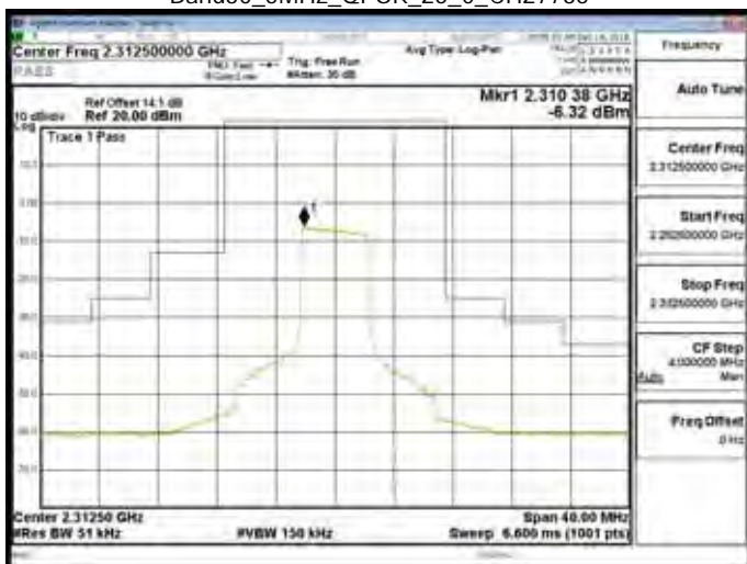
Band30_5MHz_QPSK_25_0_CH27735
