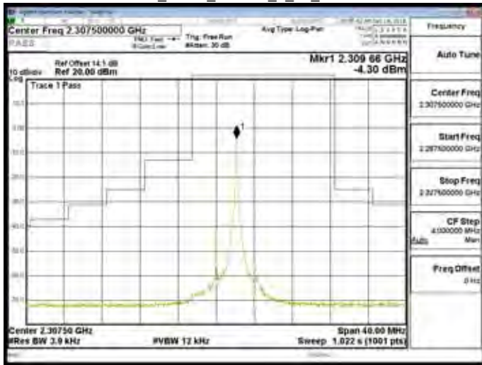
Band30_5MHz_16QAM_1_24_CH27710
