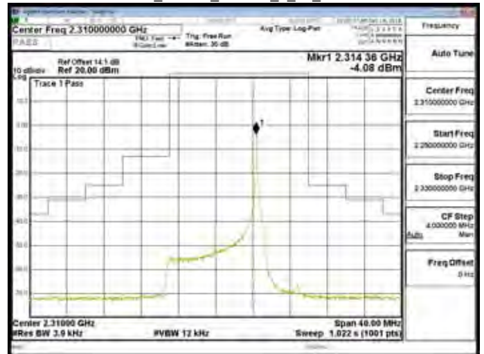
Band30_10MHz_16QAM_50_0_CH27710
