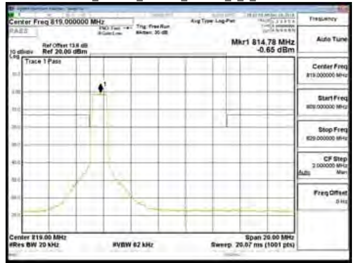
Band26_Part90s_1.4MHz_16QAM_6_0_CH26740
