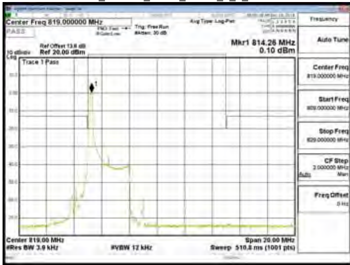
Band26_Part90s_3MHz_QPSK_1_0_CH26740
