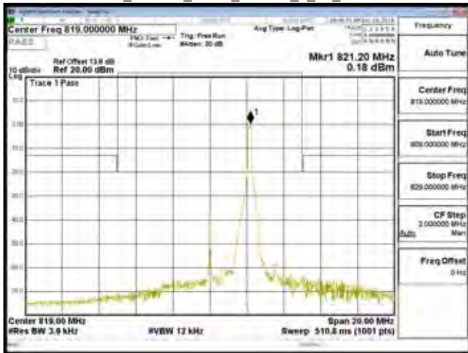
Band26_Part90s_5MHz_16QAM_1_24_CH26765
