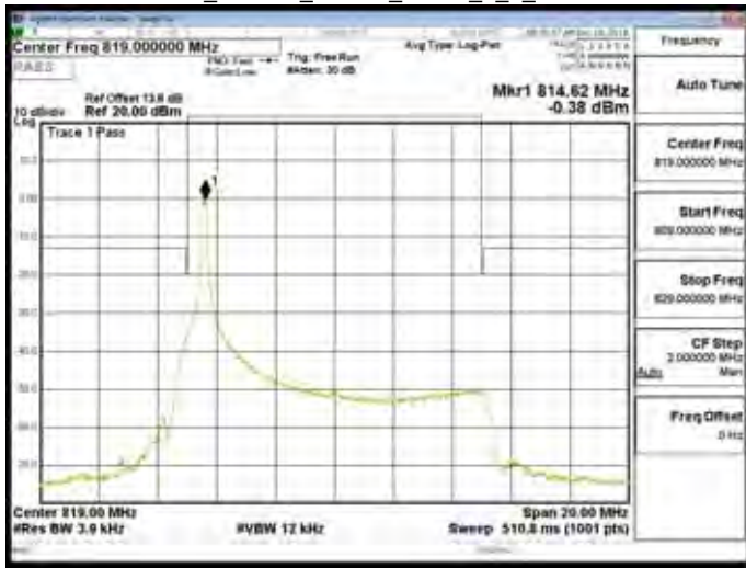
Band26_Part90s_10MHz_QPSK_1_49_CH26740
