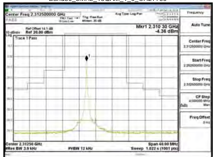
Band30_5MHz_16QAM_1_0_CH27735
