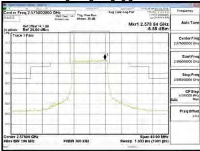
Band38_10MHz_QPSK_50_0_CH38000
