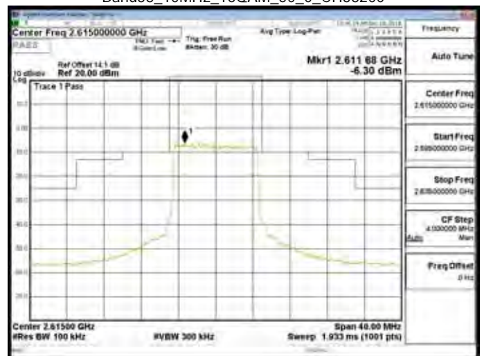
Band38_10MHz_16QAM_50_0_CH38200
