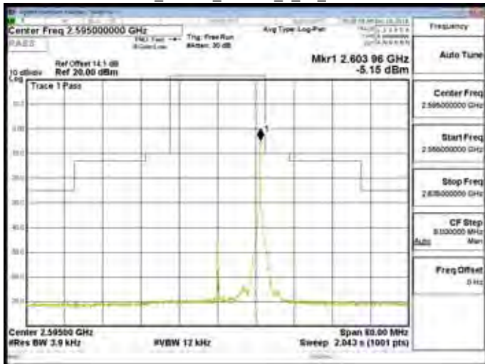
Band38_20MHz_16QAM_1_99_CH38150
