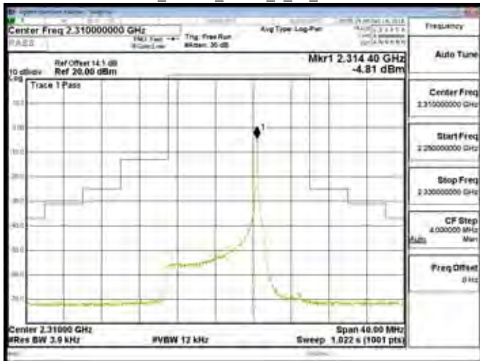
Band30_10MHz_QPSK_50_0_CH27710
