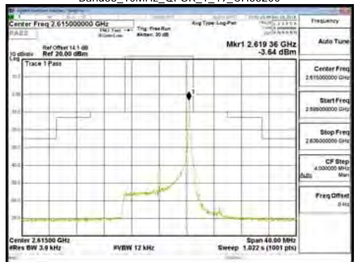
Band38_10MHz_QPSK_1_49_CH38200
