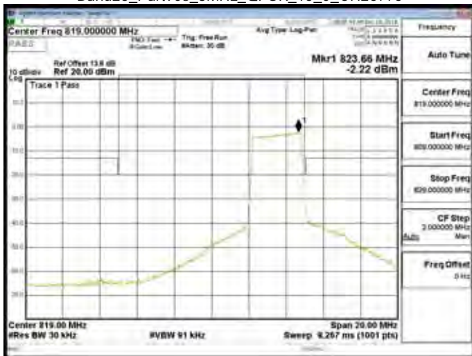
Band26_Part90s_3MHz_QPSK_15_0_CH26775
