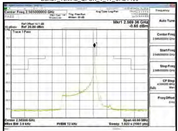
Band7_10MHz_QPSK_1_49_CH21400
