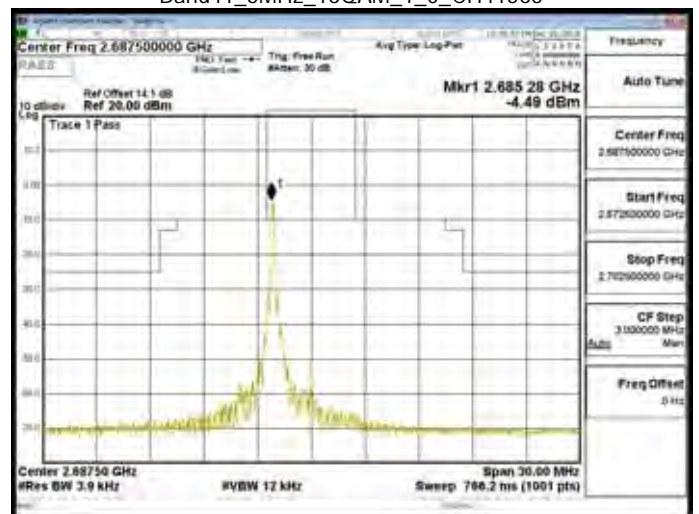
Band41_5MHz_16QAM_1_0_CH41565
