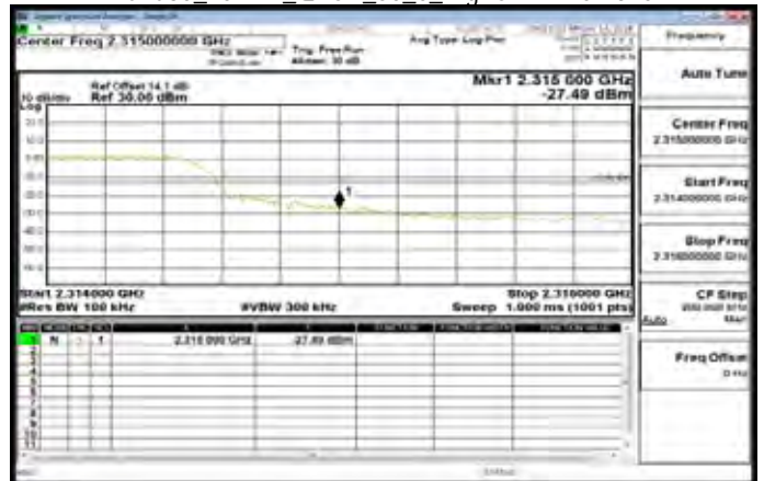
Band30_10MHz_QPSK_50_0_HighCH27710-2310
