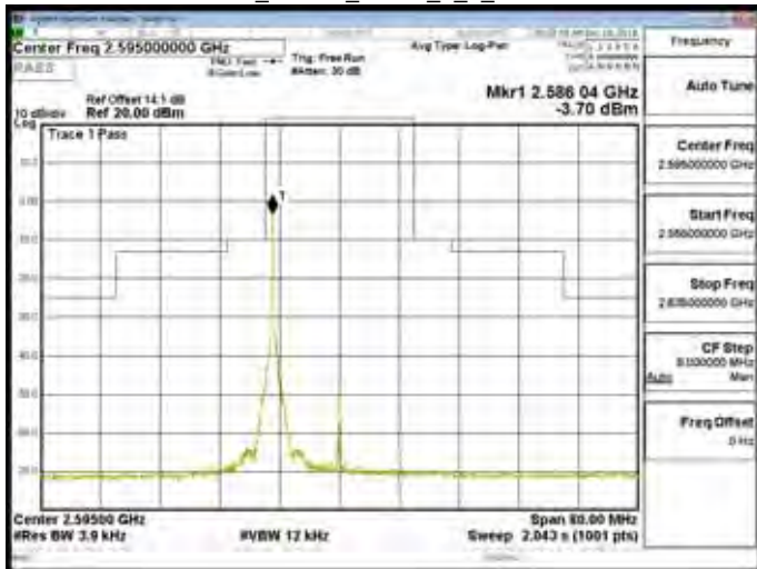
Band38_20MHz_QPSK_1_0_CH38150
