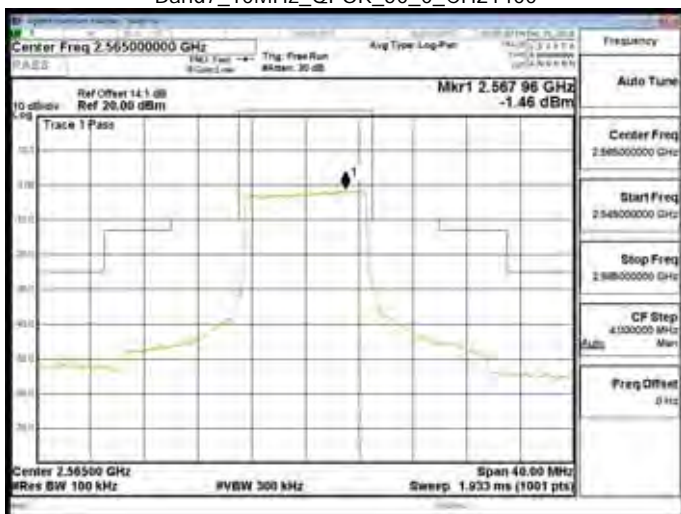
Band7_10MHz_QPSK_50_0_CH21400
