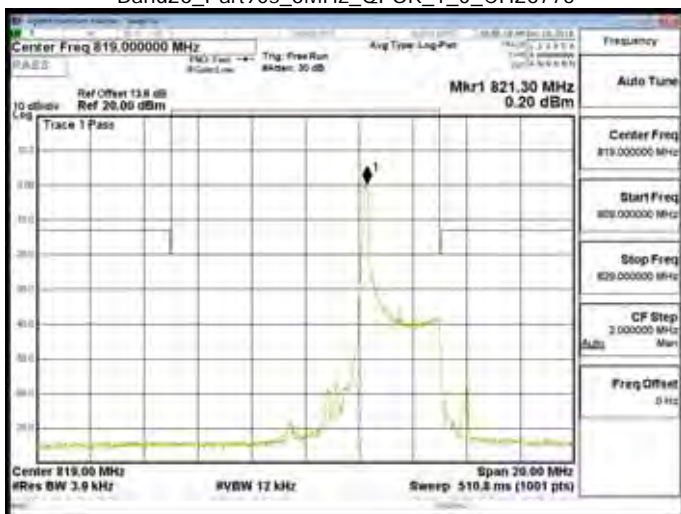
Band26_Part90s_3MHz_QPSK_1_0_CH26775
