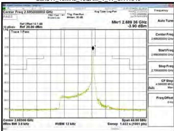
Band41_10MHz_16QAM_1_49_CH41540
