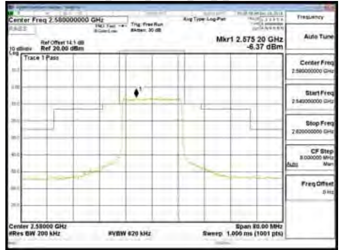
Band38_20MHz_16QAM_100_0_CH38000
