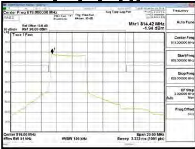
Band26_Part90s_5MHz_QPSK_25_0_CH26740
