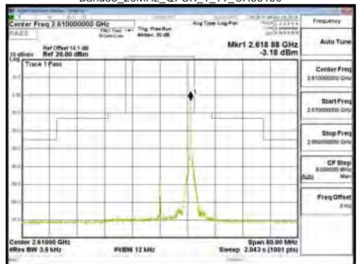
Band38_20MHz_QPSK_1_99_CH38150
