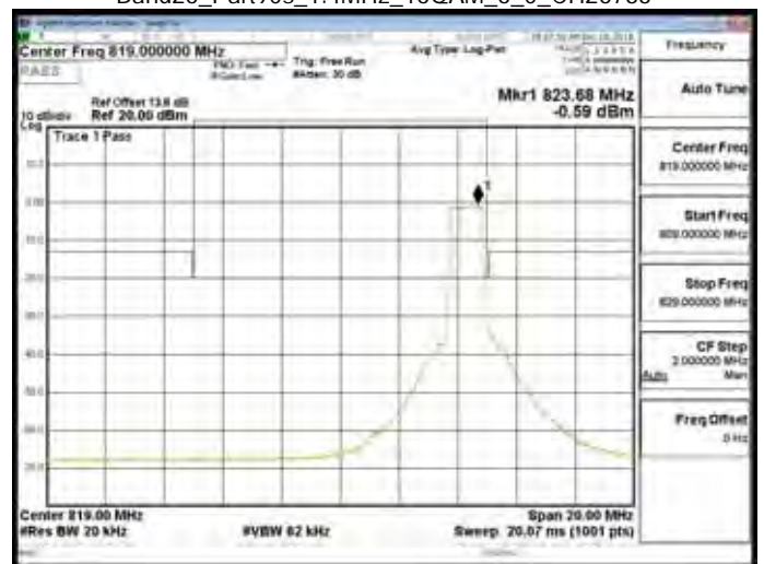
Band26_Part90s_1.4MHz_16QAM_6_0_CH26783
