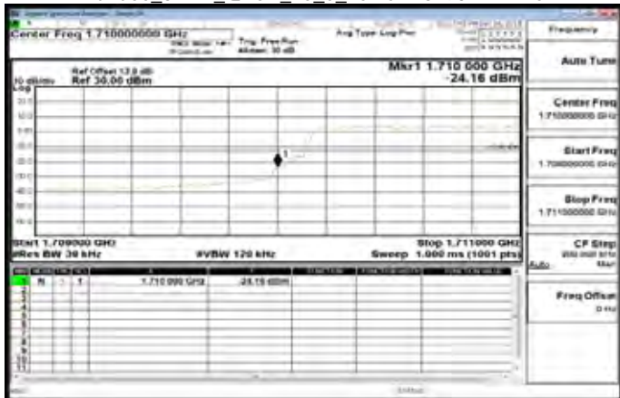
Band66_3MHz_QPSK_15_0_LowCH131987-1711.5
