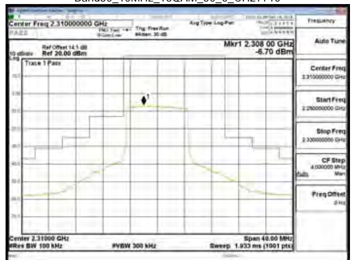
Band30_10MHz_16QAM_50_0_CH27710
