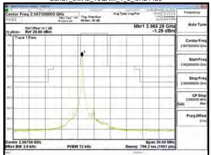
Band7_5MHz_16QAM_1_0_CH21425
