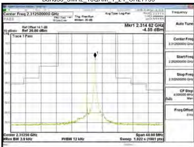
Band30_5MHz_16QAM_1_24_CH27735
