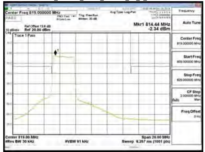
Band26_Part90s_3MHz_16QAM_15_0_CH26740
