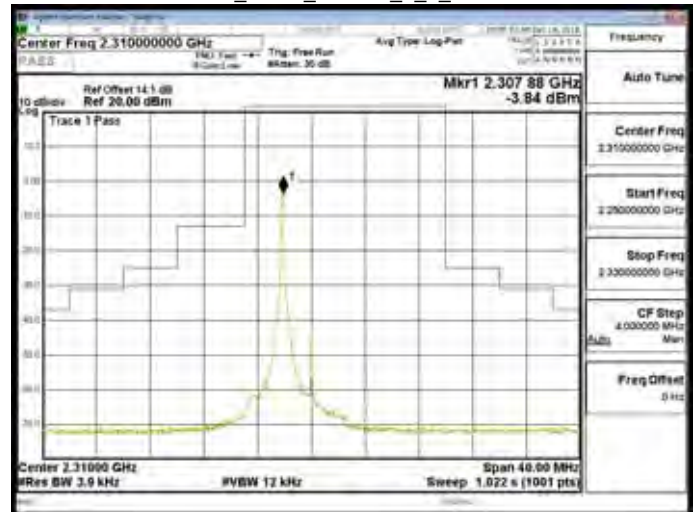
Band30_5MHz_16QAM_1_0_CH27735
