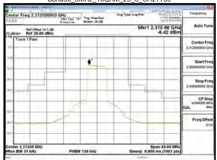
Band30_5MHz_16QAM_25_0_CH27735
