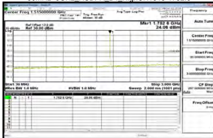
30MHz~3GHz_HSDPA_B4_HighCH1513-1752.6
