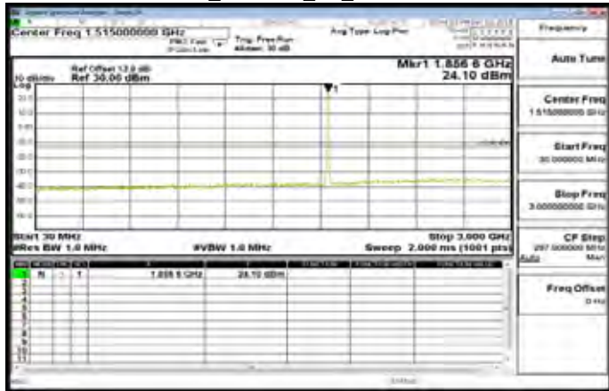
30MHz~3GHz_WCDMA_B2_LowCH9262-1852.4
