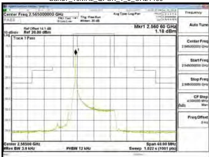
Band7_10MHz_QPSK_1_0_CH21400
