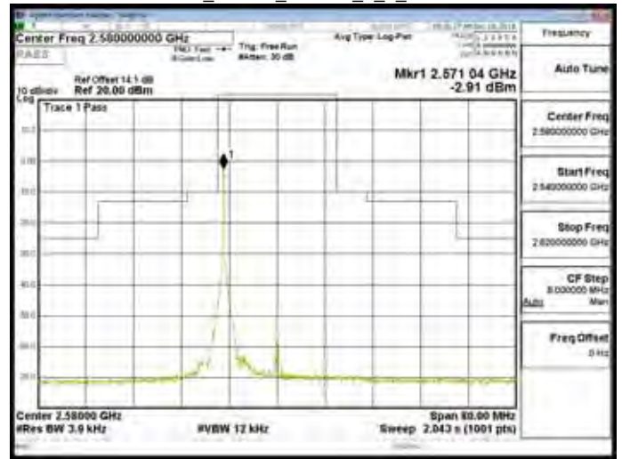
Band38_20MHz_16QAM_1_0_CH38000
