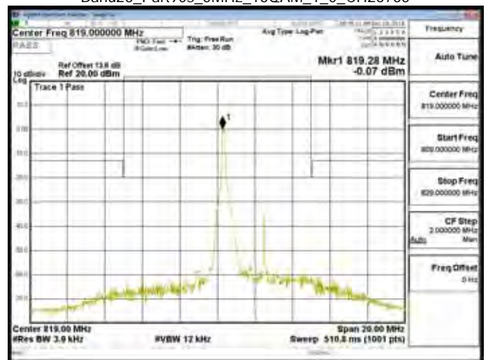
Band26_Part90s_5MHz_16QAM_1_0_CH26765
