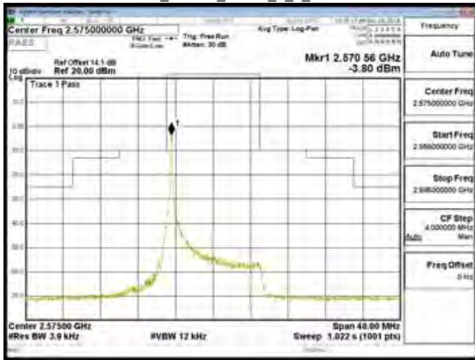
Band38_10MHz_QPSK_1_0_CH38000
