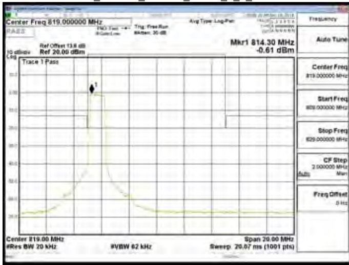
Band26_Part90s_1.4MHz_QPSK_6_0_CH26740
