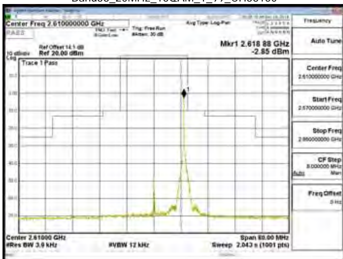
Band38_20MHz_16QAM_1_99_CH38150
