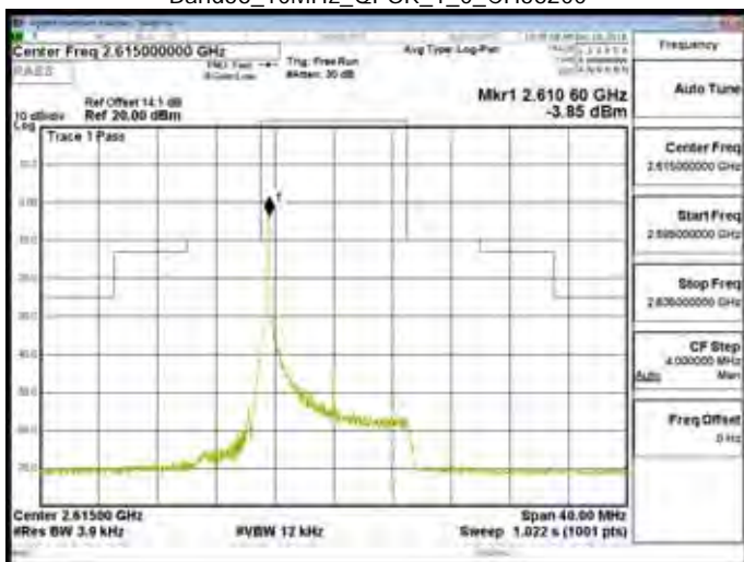
Band38_10MHz_QPSK_1_0_CH38200
