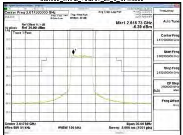
Band38_5MHz_16QAM_25_0_CH38225
