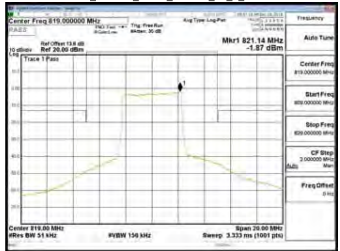
Band26_Part90s_5MHz_16QAM_25_0_CH26765
