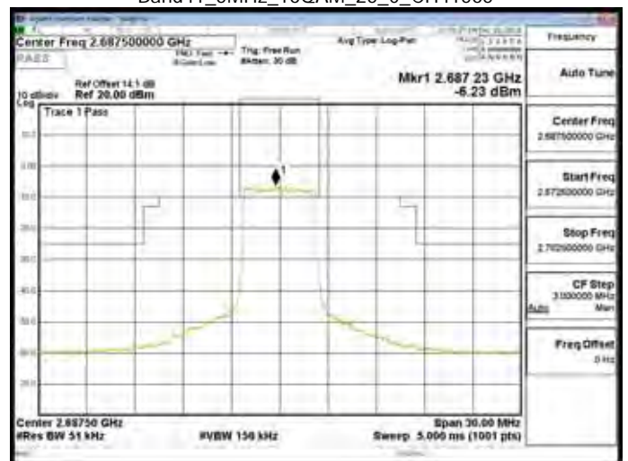
Band41_5MHz_16QAM_25_0_CH41565
