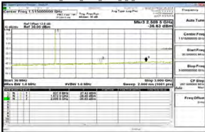
30MHz-3GHz_Band5_3MHz_OPSK_1_0_MidCH20525-836.5
