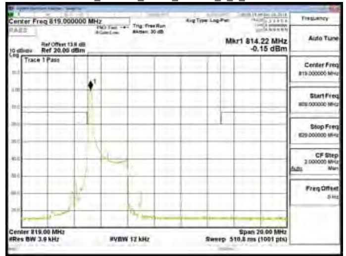
Band26_Part90s_3MHz_16QAM_1_0_CH26740
