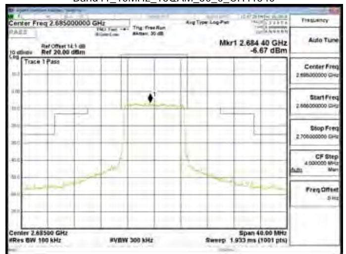
Band41_10MHz_16QAM_50_0_CH41540
