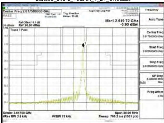
Band38_5MHz_16QAM_1_24_CH38225
