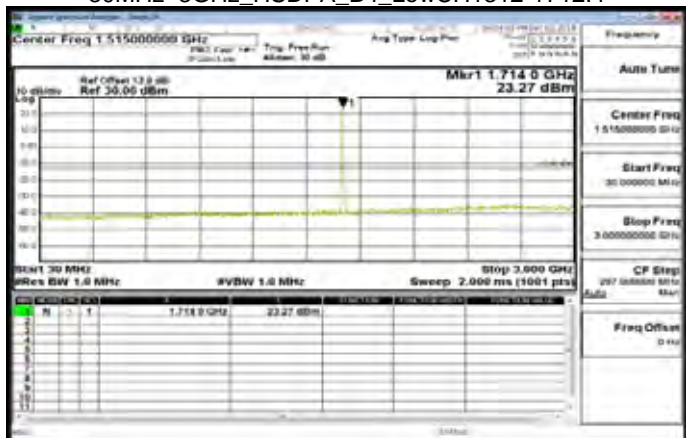
30MHz~3GHz_HSDPA_B4_LowCH1312-1712.4
