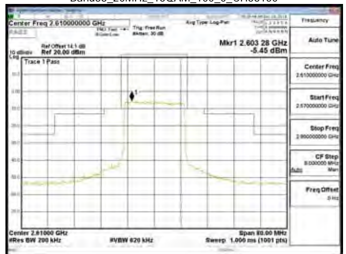
Band38_20MHz_16QAM_100_0_CH38150
