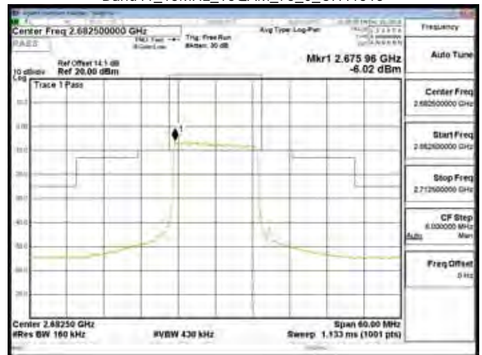
Band41_15MHz_16QAM_75_0_CH41515
