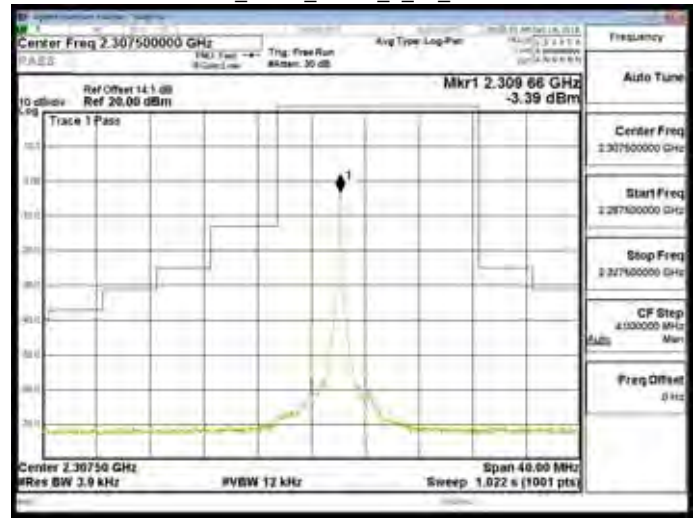
Band30_5MHz_QPSK_1_24_CH27710
