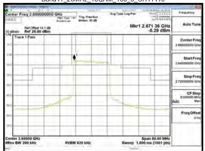
Band41_20MHz_16QAM_100_0_CH41490
