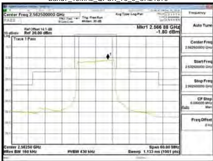
Band7_15MHz_QPSK_75_0_CH21375
