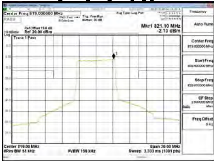
Band26_Part90s_5MHz_QPSK_25_0_CH26765
