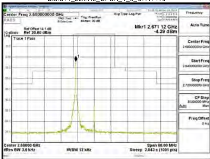
Band41_20MHz_QPSK_1_0_CH41490
