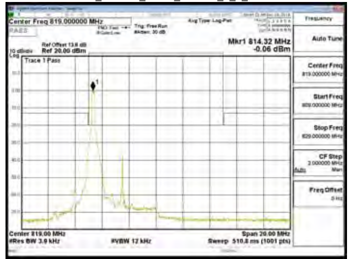
Band26_Part90s_5MHz_16QAM_1_0_CH26740
