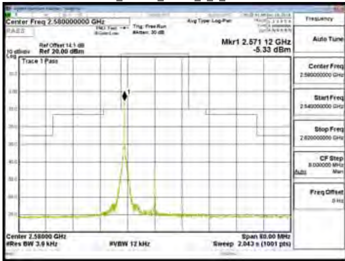
Band38_20MHz_QPSK_1_0_CH38000
