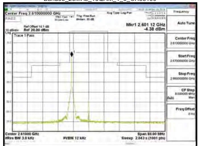
Band38_20MHz_16QAM_1_0_CH38150
