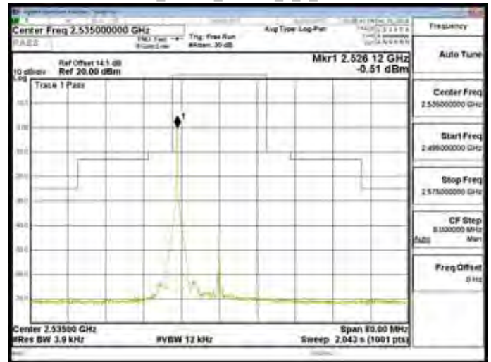
Band7_20MHz_16QAM_1_0_CH21350
