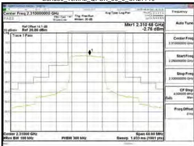
Band30_10MHz_QPSK_50_0_CH27710
