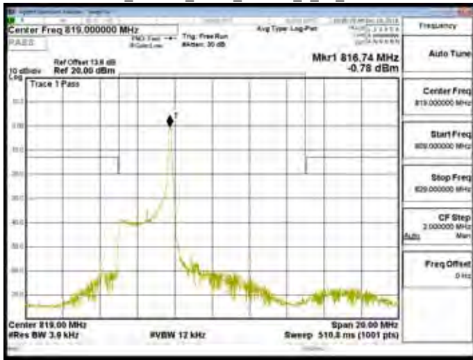
Band26_Part90s_3MHz_16QAM_1_14_CH26740
