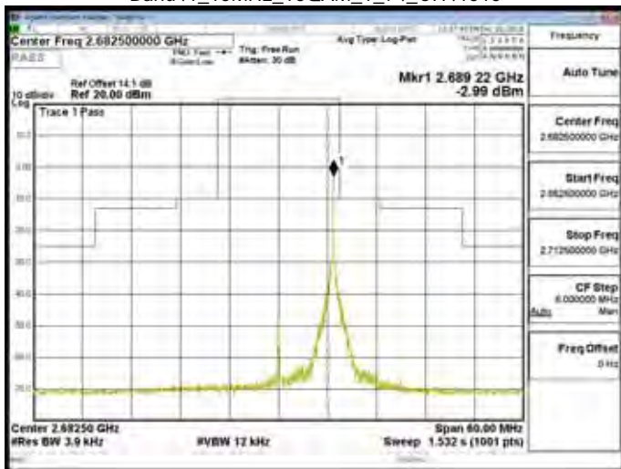
Band41_15MHz_16QAM_1_74_CH41515
