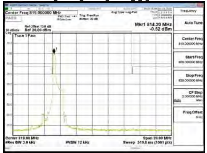
Band26_Part90s_1.4MHz_16QAM_1_0_CH26740
