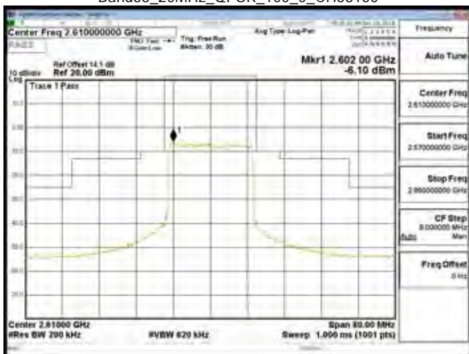
Band38_20MHz_QPSK_100_0_CH38150
