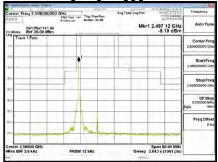
Band41_20MHz_16QAM_1_0_CH40620
