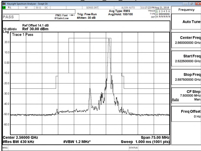
Band 7_QPSK_20M_RB100,0
