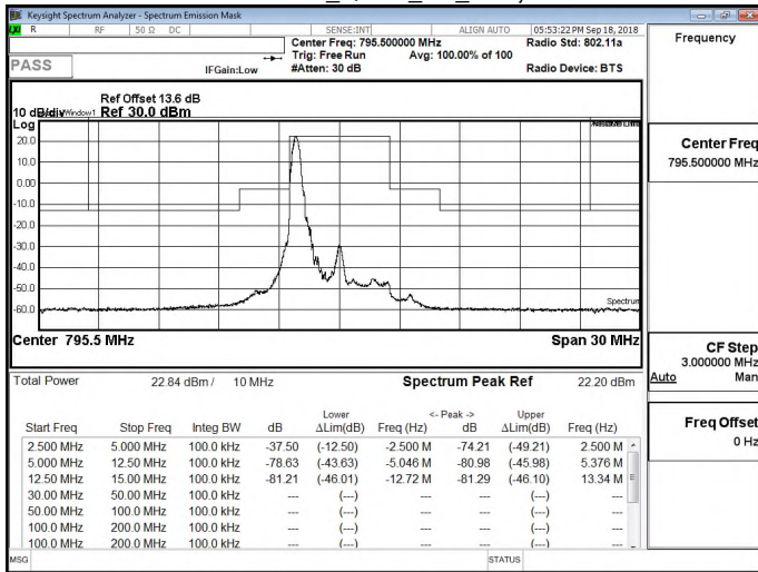
Band 14 QPSK_5M_RB1,24
