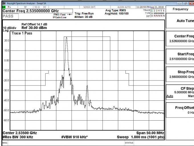
Band 7_16QAM_15M_RB1,74
