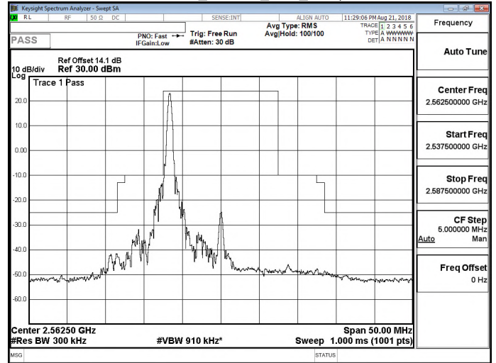
Band 7_16QAM_15M_RB1,74
