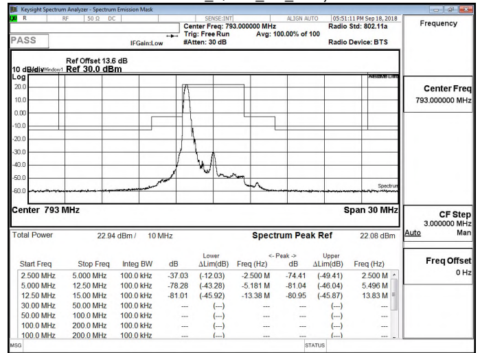
Band 14 QPSK_5M_RB1,24
