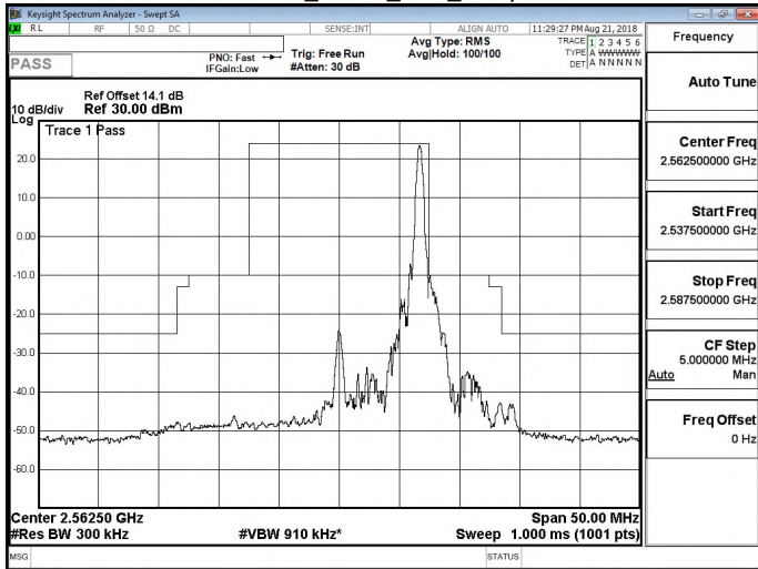
Band 7_QPSK_15M_RB75,0
