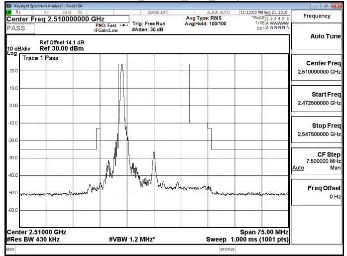
Band 7_16QAM_20M_RB1,99
