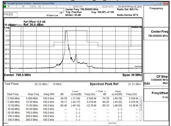
Band 14 16QAM_5M_RB1,24
