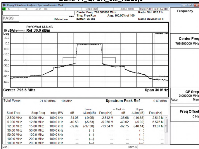
Band 14 QPSK_5M_RB25,0
