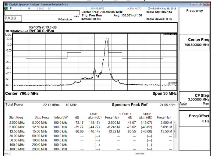
Band 14 16QAM_5M_RB25,0
