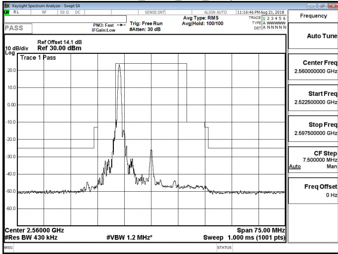
Band 7_QPSK_20M_RB1,99
