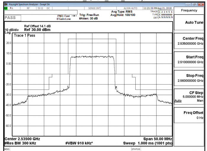
Band 7_QPSK_15M_RB75,0
