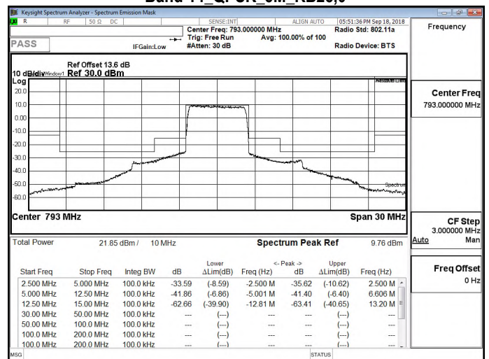
Band 14 QPSK_5M_RB25,0
